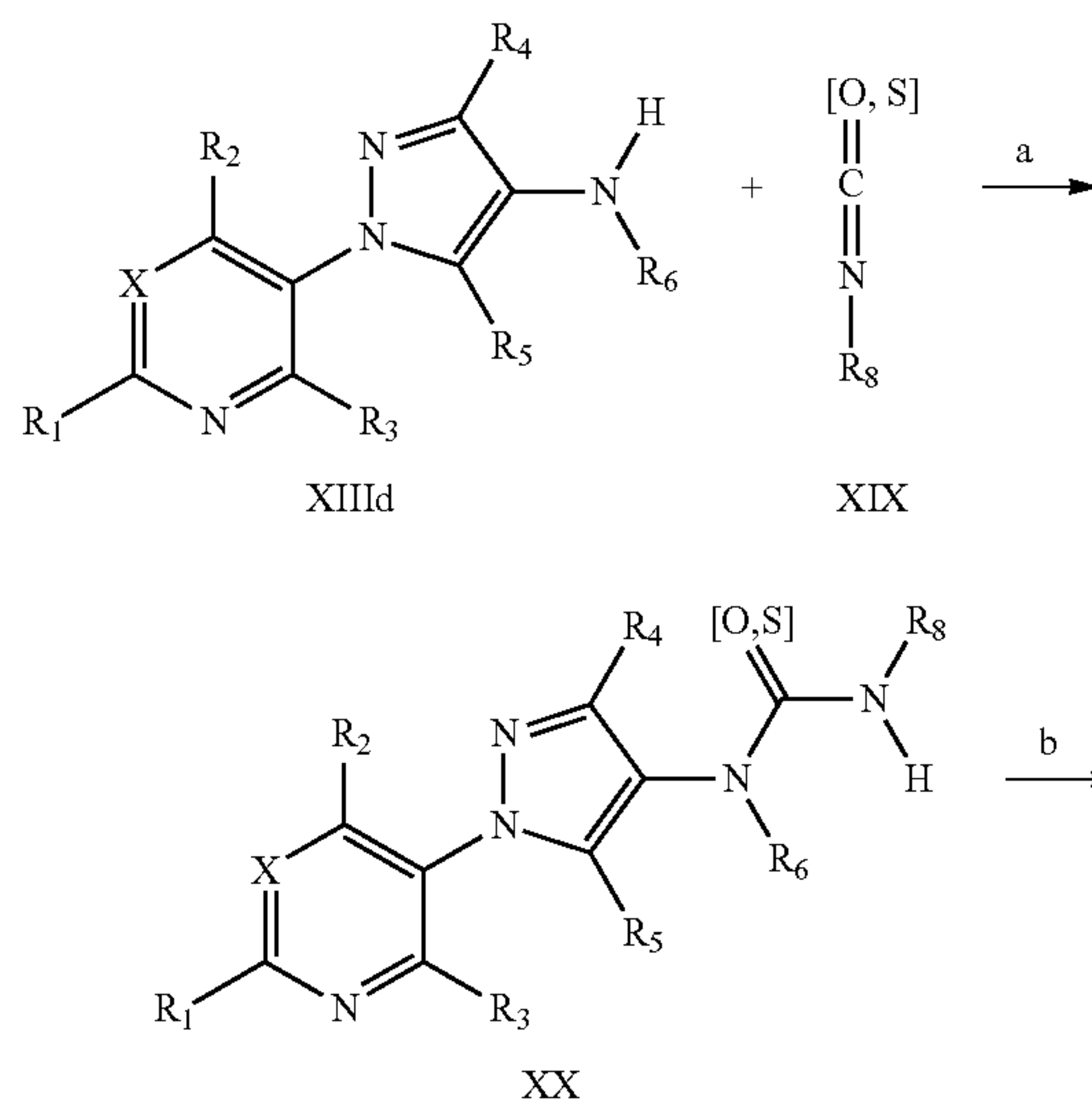
Scheme X
