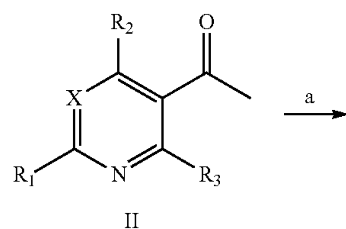
Scheme I
