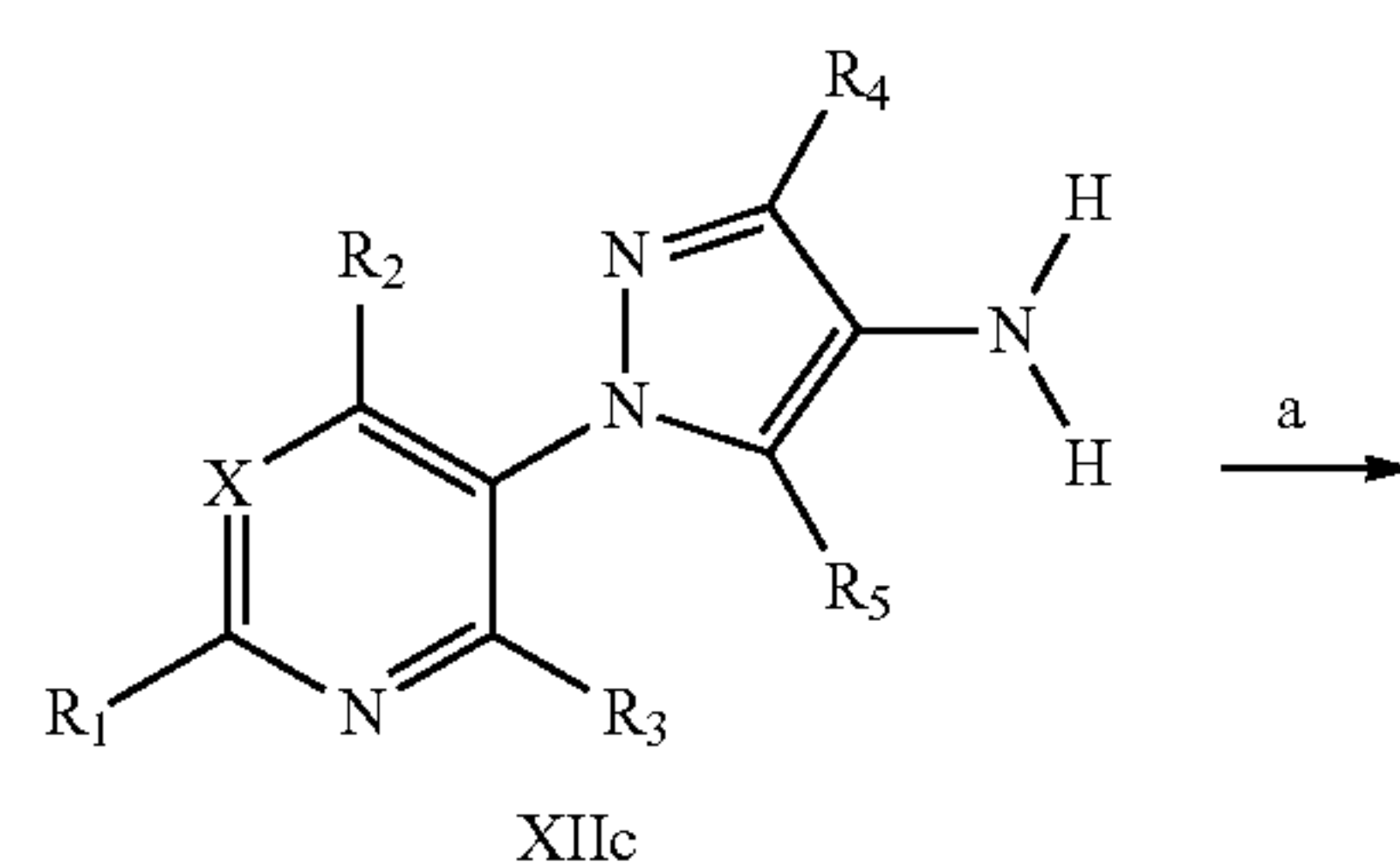
Scheme VIII
