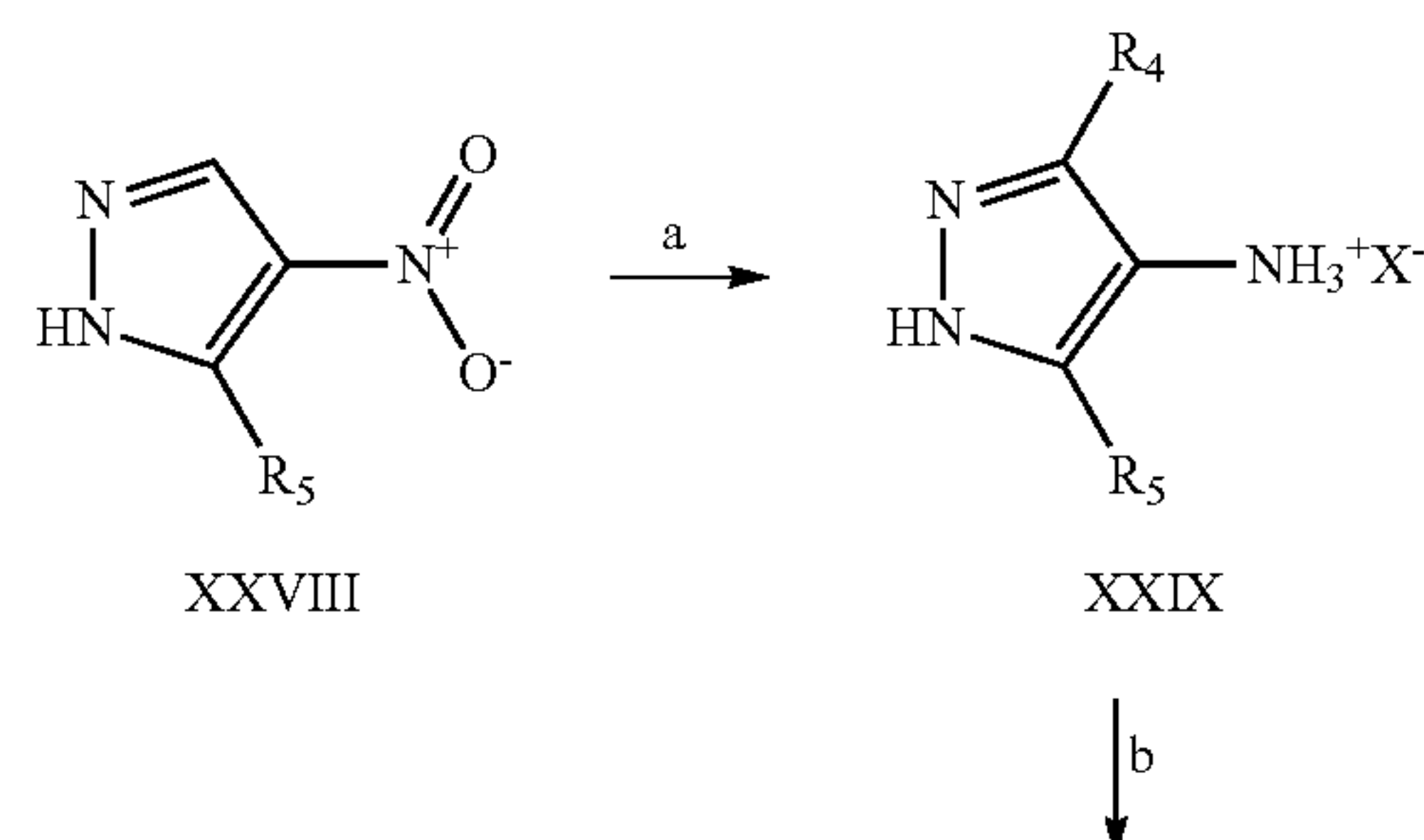
Scheme XIV
