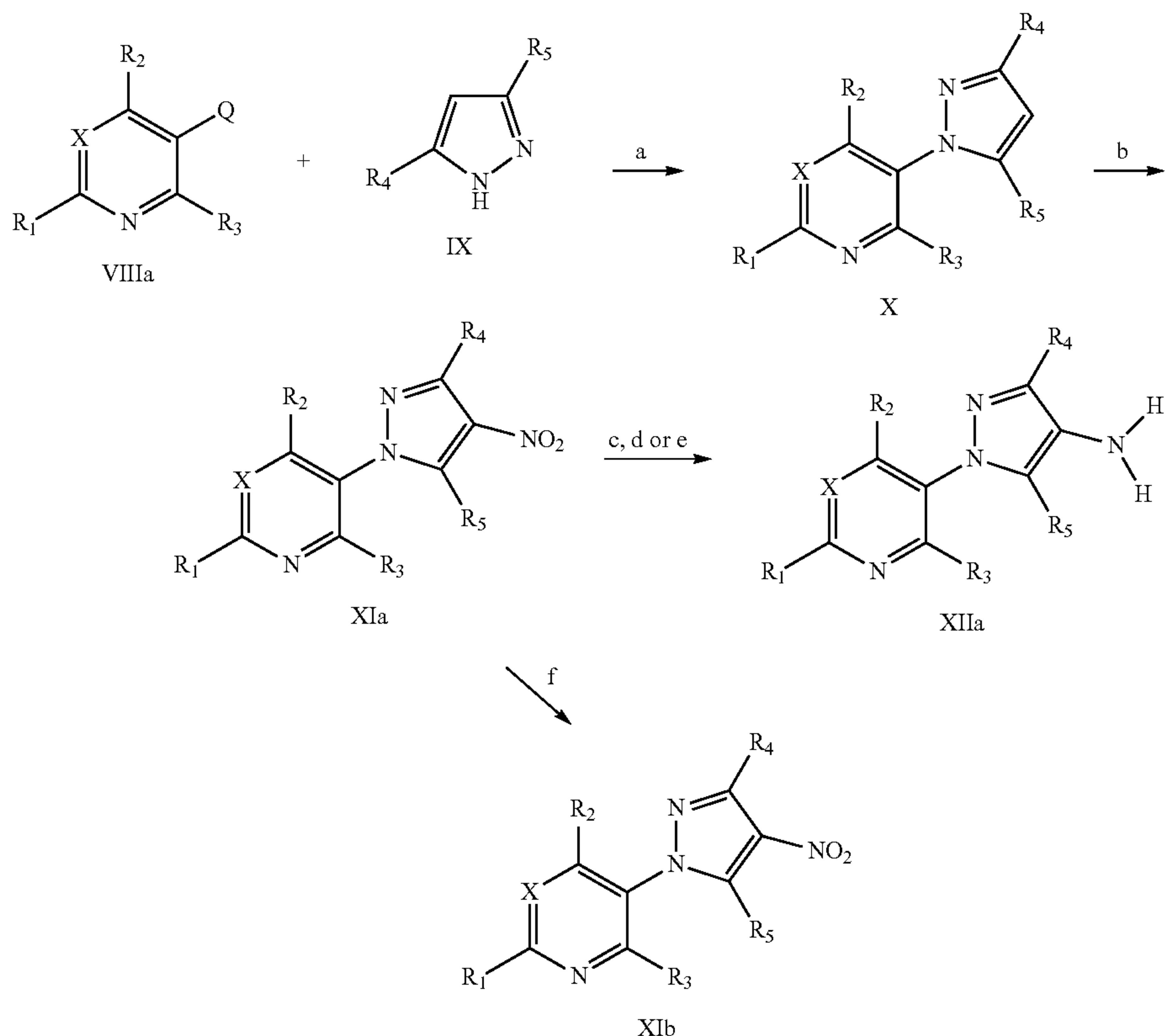
Scheme III
