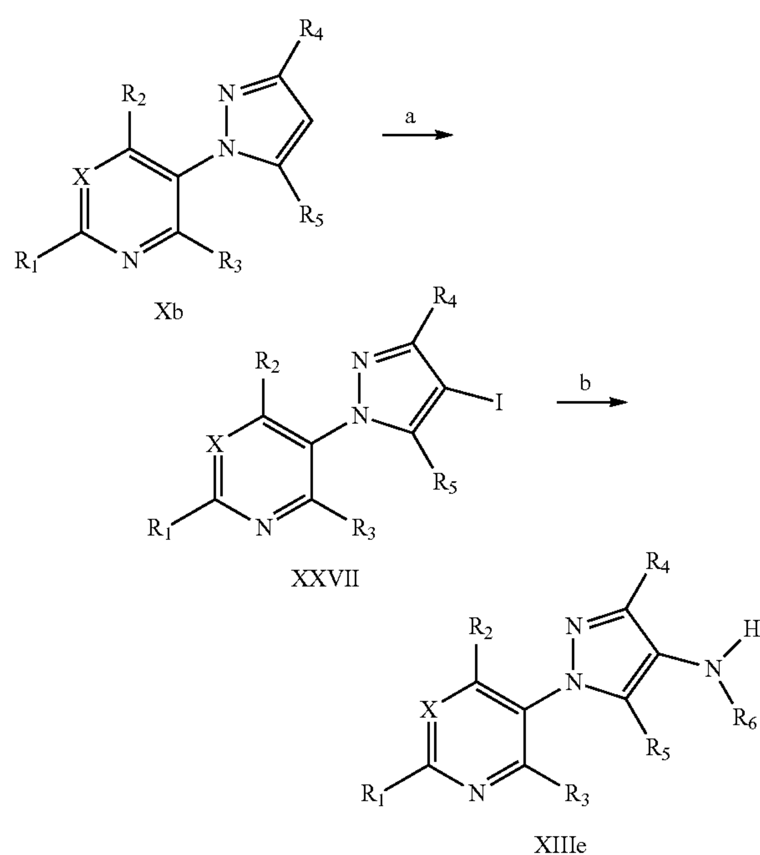
Scheme XIII
