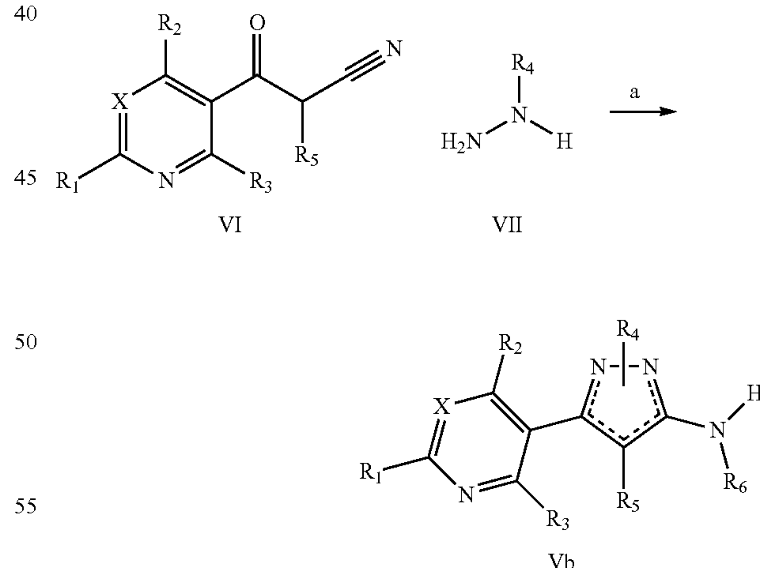
Scheme II
