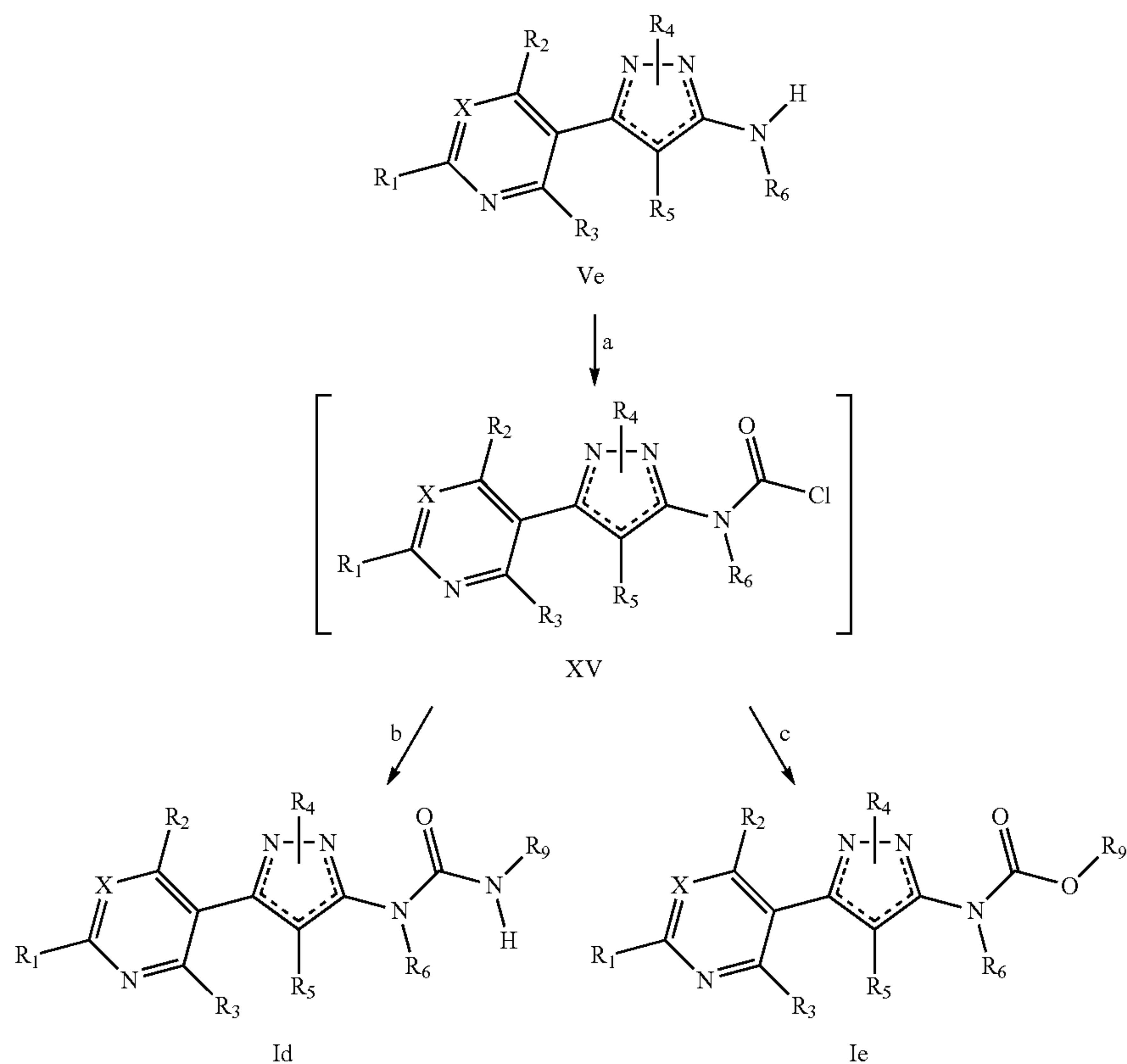
Scheme VII
