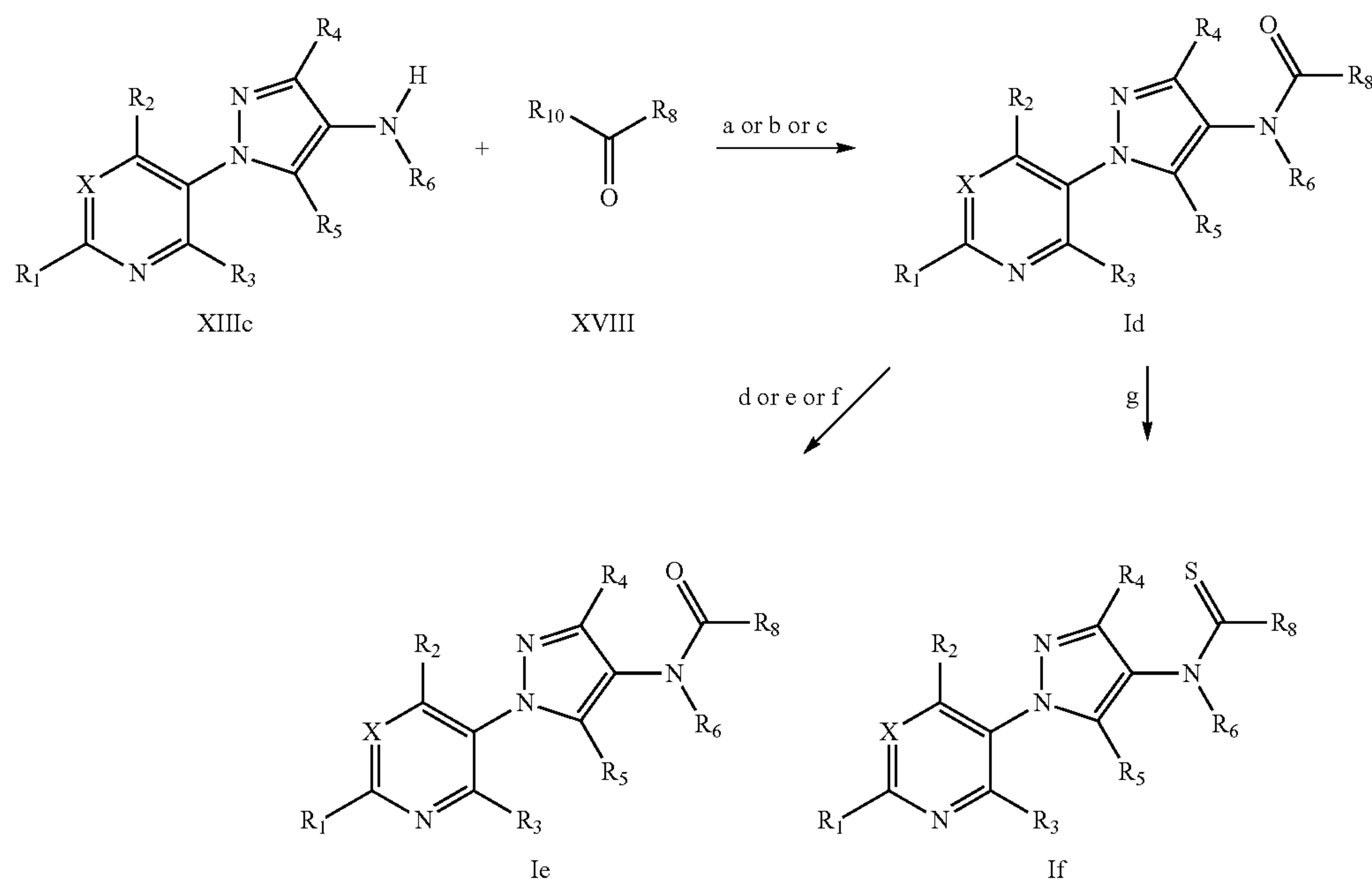
Scheme IX
