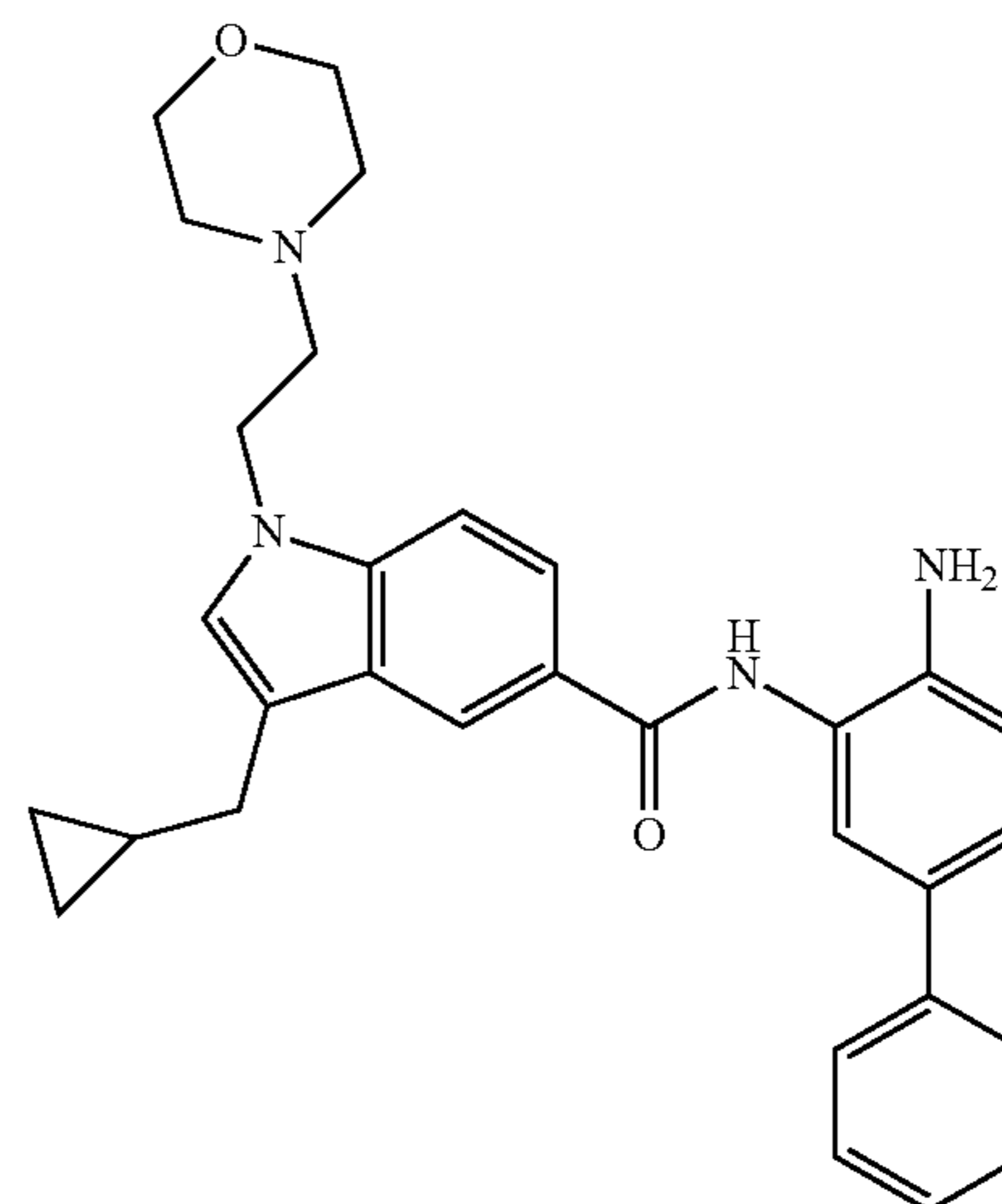
N-(4-amino-[1,1'-biphenyl]-3-yl)-3-(cyclopropylmethyl)-1-(2-morpholinoethyl)-1H-indole-5-carboxamide
