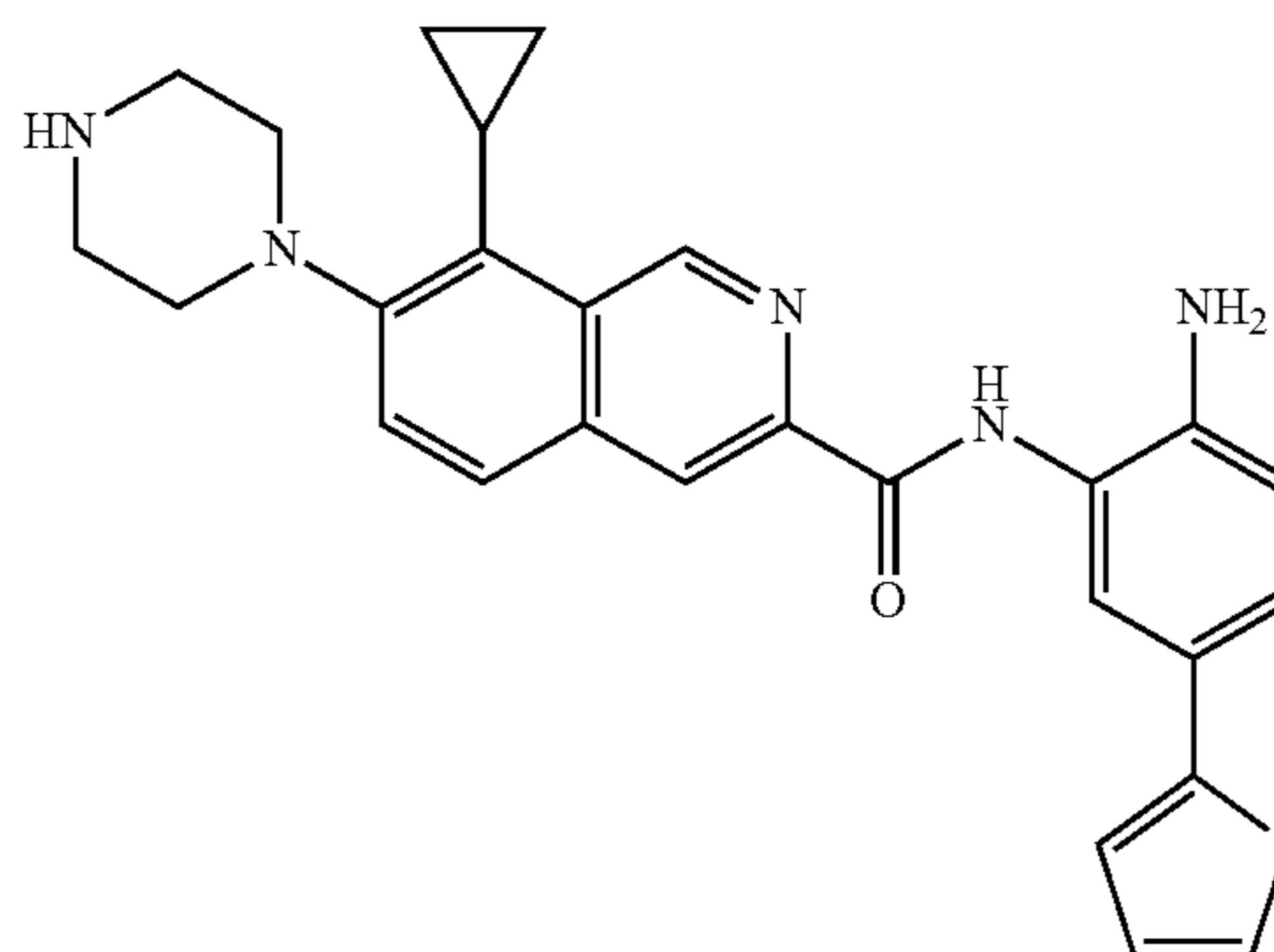
N-(2-amino-5-(thiophen-2-yl)phenyl)-8- cyclopropyl-7-(piperazin-1-yl)isoquinoline-3- carboxamide
