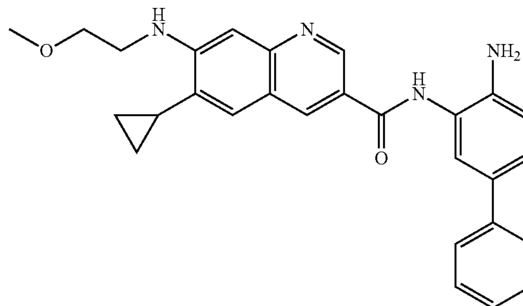
N-(4-amino-[1,1'-biphenyl]-3-yl)-6-cyclopropyl-7-((2-methoxyethyl)amino)quinoline-3-carboxamide
