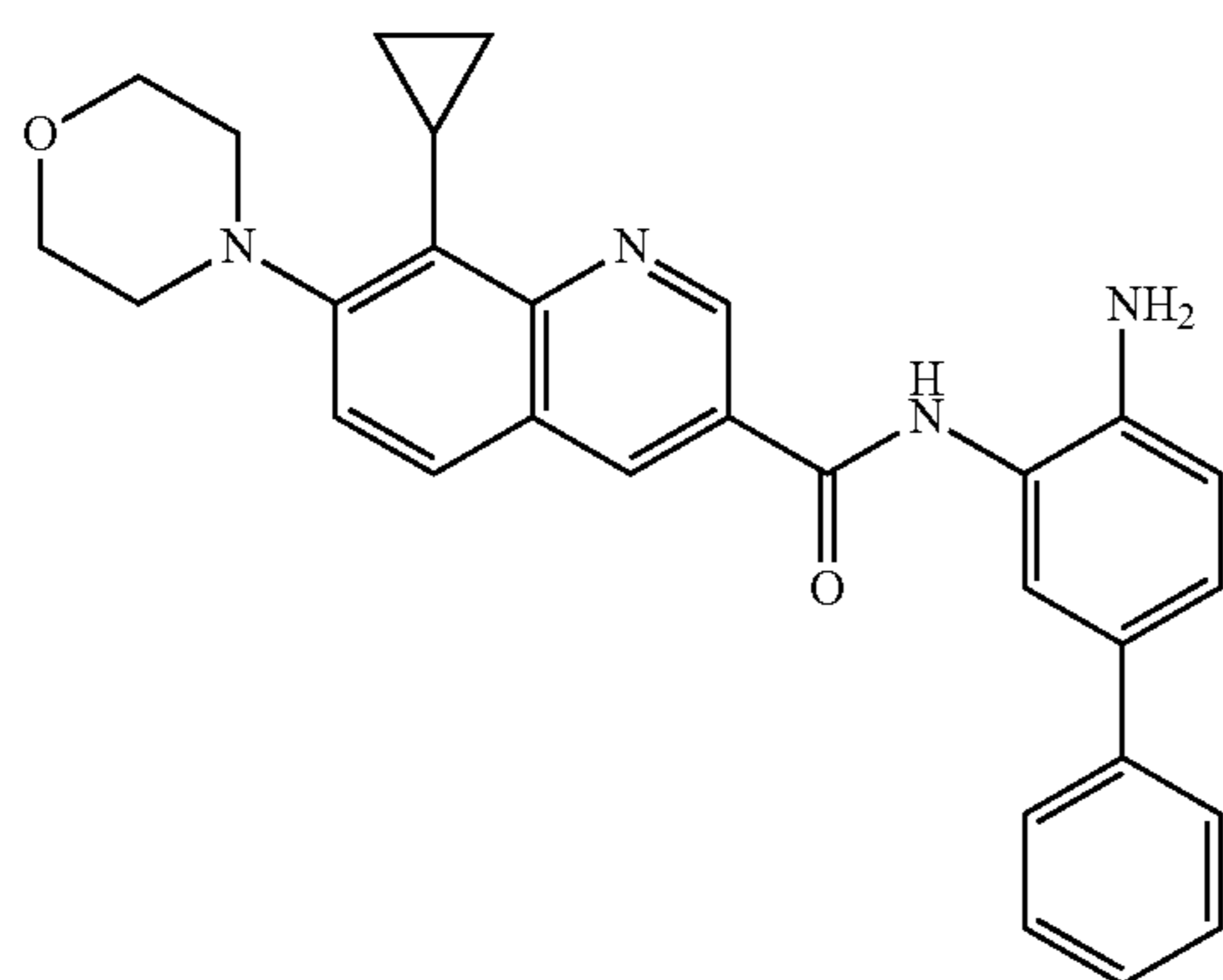
N-(4-amino-[1,1'-biphenyl]-3-yl)-8-cyclopropyl-7-morpholinoquinoline-3-carboxamide IC_{50} (nM) HDAC1 = 295 HDAC2 = 799 HDAC3 = >2,000
