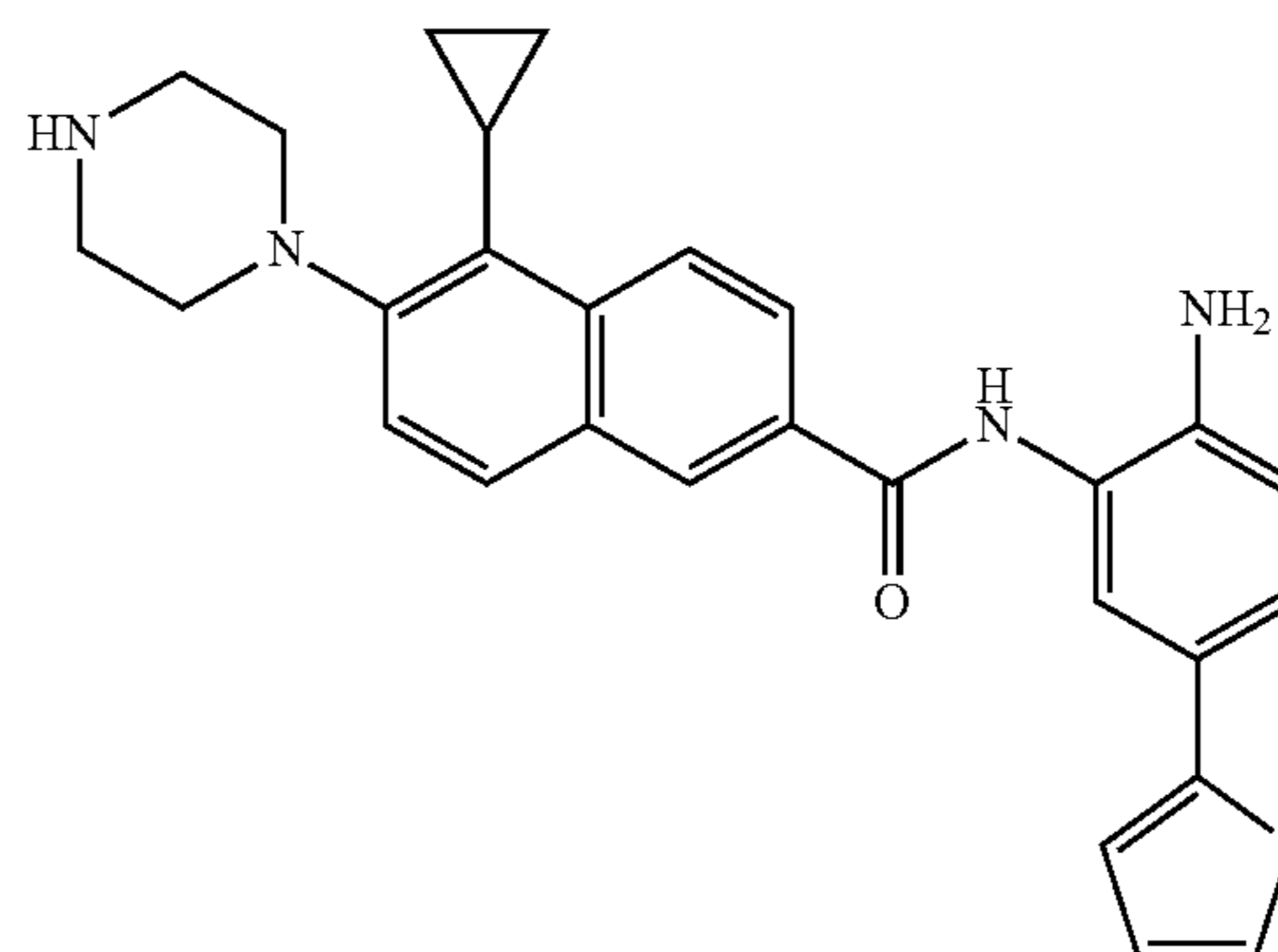
N-(2-amino-5-(thiophen-2-yl)phenyl)-5-cyclopropyl-6-(piperazin-1-yl)-2-naphthamide
