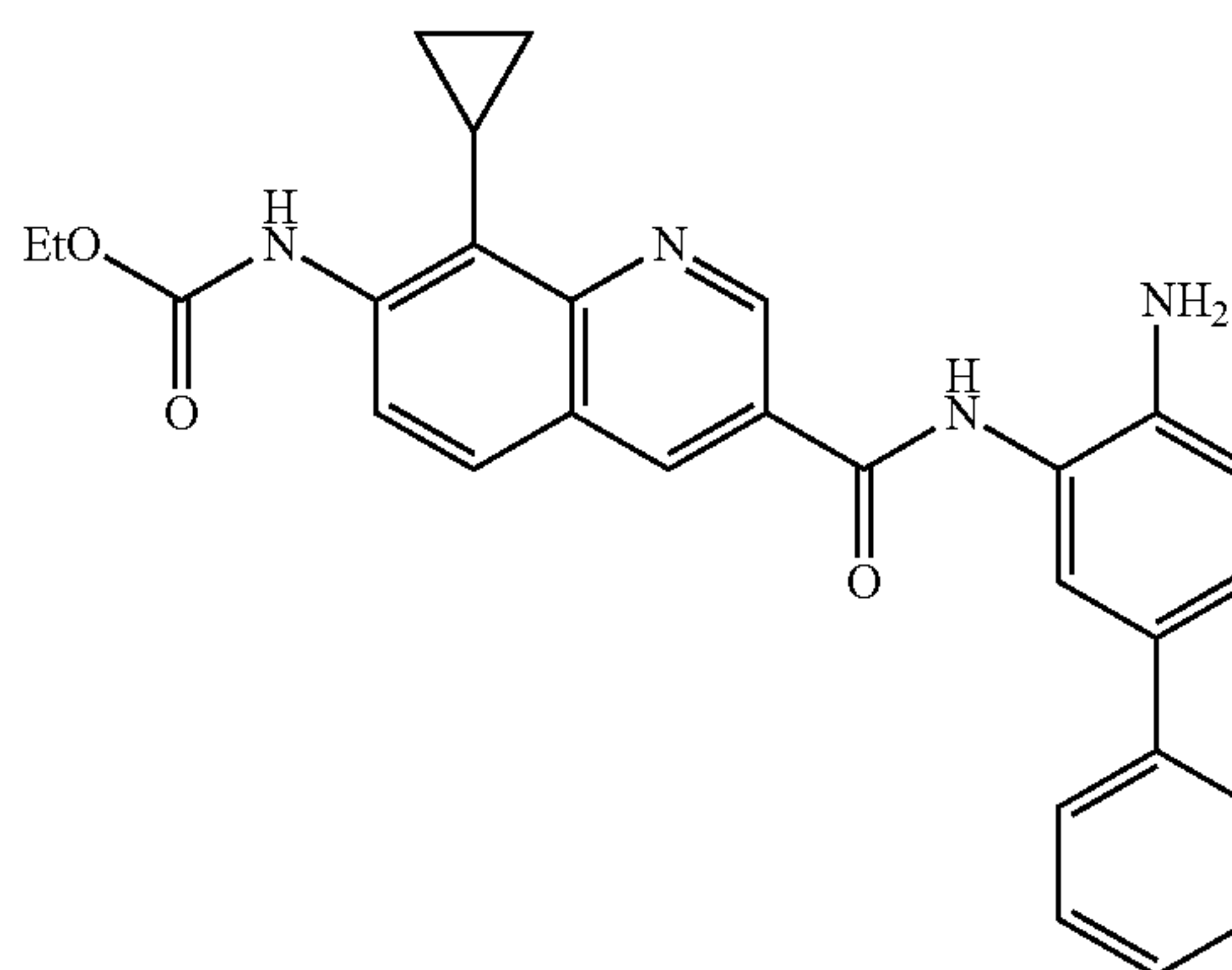
ethyl 3-((4-amino-[1,1'-biphenyl]-3-yl)carbamoyl)-8-cyclopropylquinolin-7-yl)carbamate
