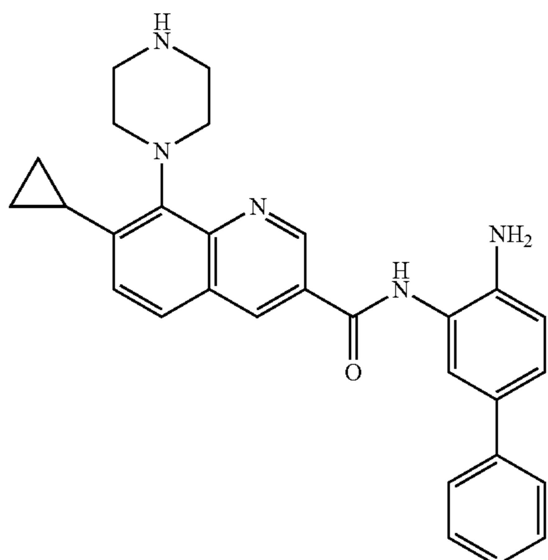
N-(4-amino-[1,1'-biphenyl]-3-yl)-7-cyclopropyl-8-(piperazin-1-yl)quinoline-3-carboxamide IC_{50}(nM) HDAC1 = 103 HDAC2 = 56 HDAC3 = 257
