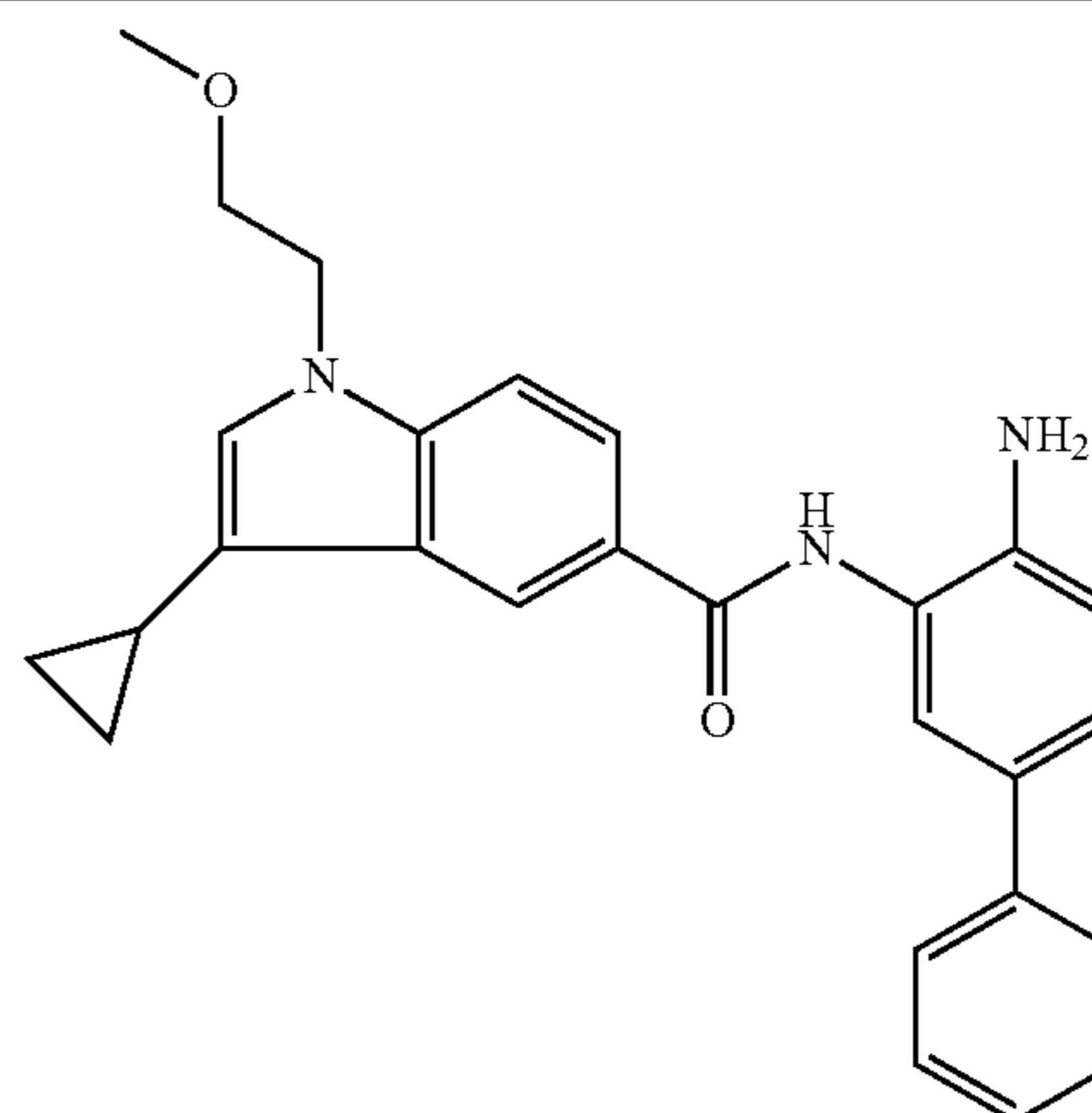
N-(4-amino-[1,1'-biphenyl]-3-yl)-3-cyclopropyl-1-(2-methoxyethyl)-1H-indole-5-carboxamide IC_{50} (nM) HDAC1 = >2,000 HDAC2 = >2,000 HDAC3 = >2,000
