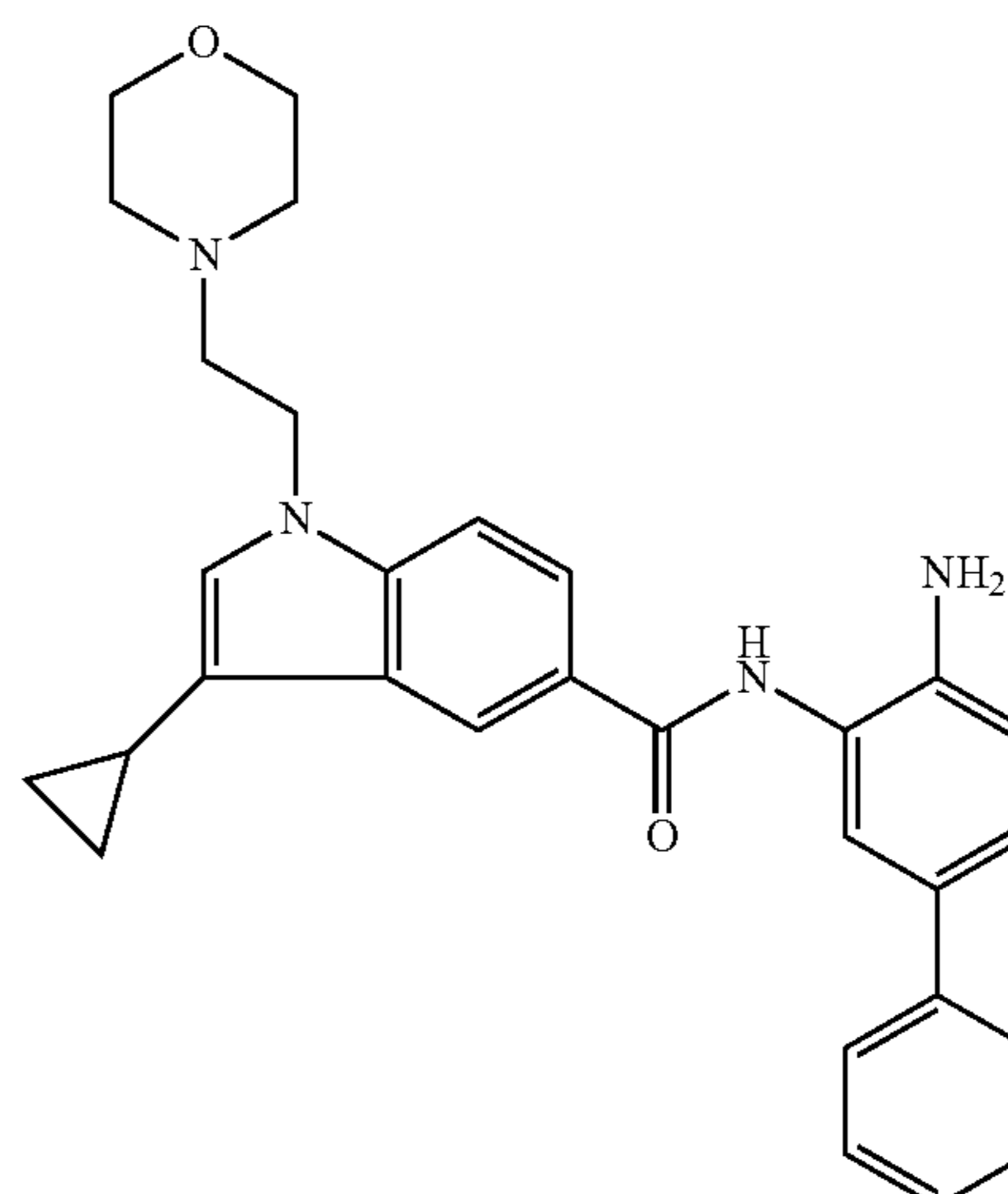
N-(4-amino-[1,1'-biphenyl]-3-yl)-3-cyclopropyl-1-(2-morpholinoethyl)-1H-indole-5-carboxamide
