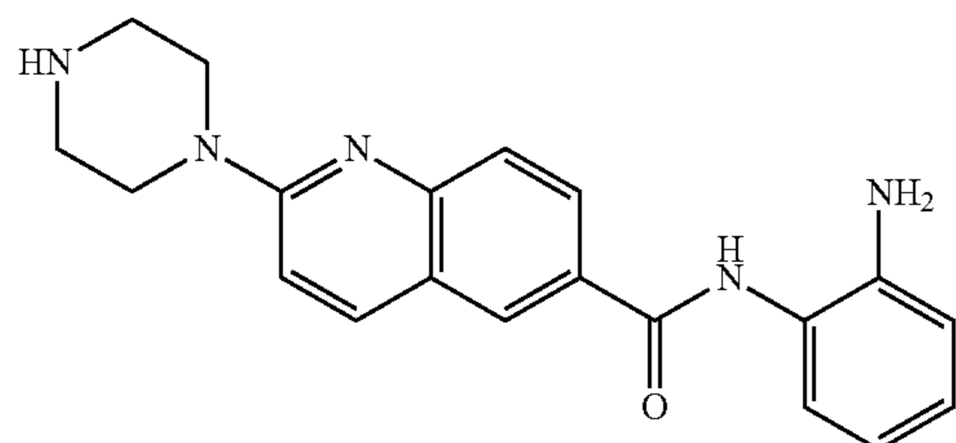
N-(2-aminophenyl)-2-(piperazin-1-yl)quinoline-6-carboxamide IC_{50} (nM) HDAC1 = >2,000 HDAC2 = 624 HDAC3 = 104
