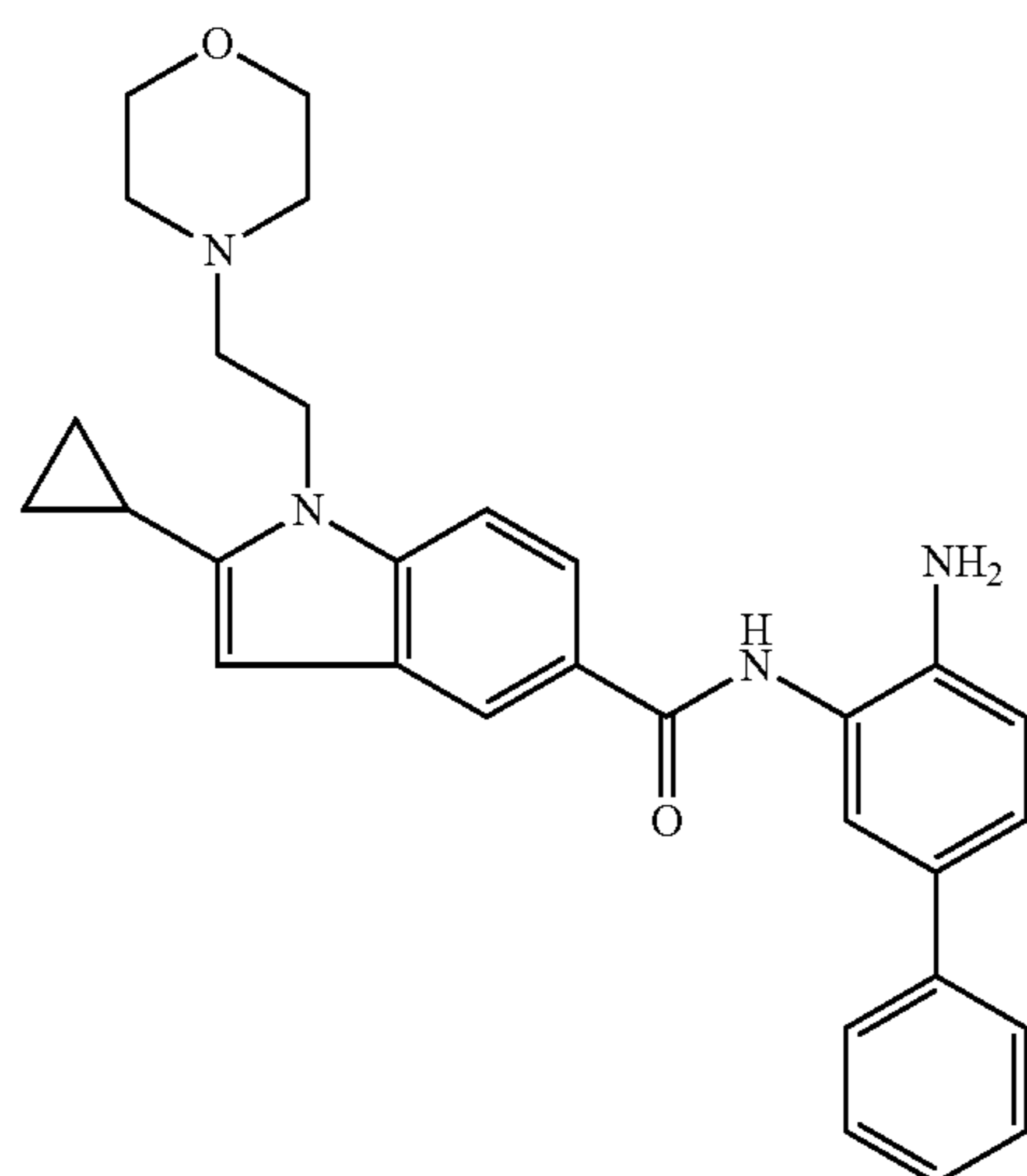
N-(4-amino-[1,1'-biphenyl]-3-yl)-2-cyclopropyl-1-(2-morpholinoethyl)-1H-indole-5-carboxamide
