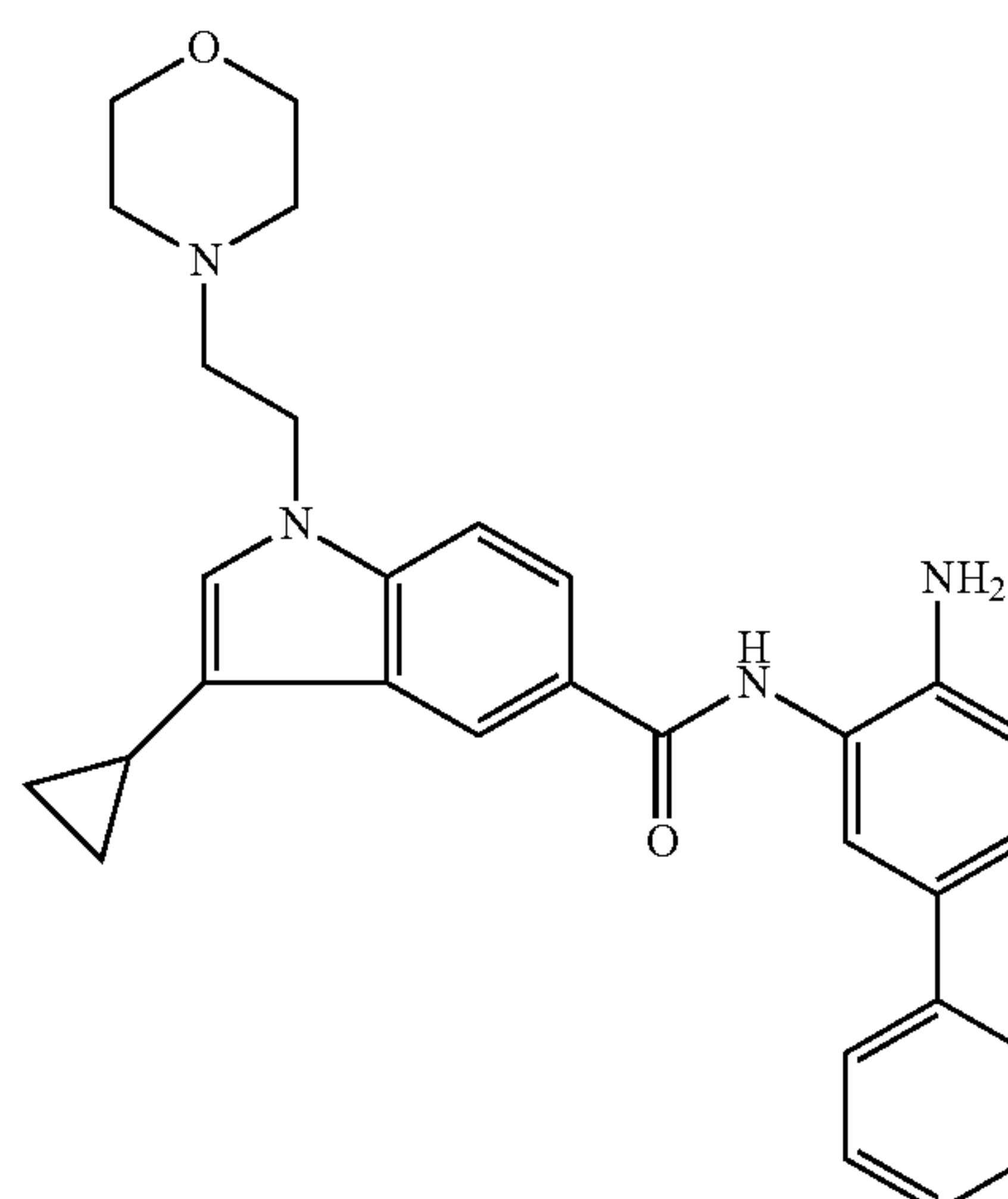
N-(4-amino-[1,1'-biphenyl]-3-yl)-3-cyclopropyl-1-(2-morpholinoethyl)-1H-indole-5-carboxamide
