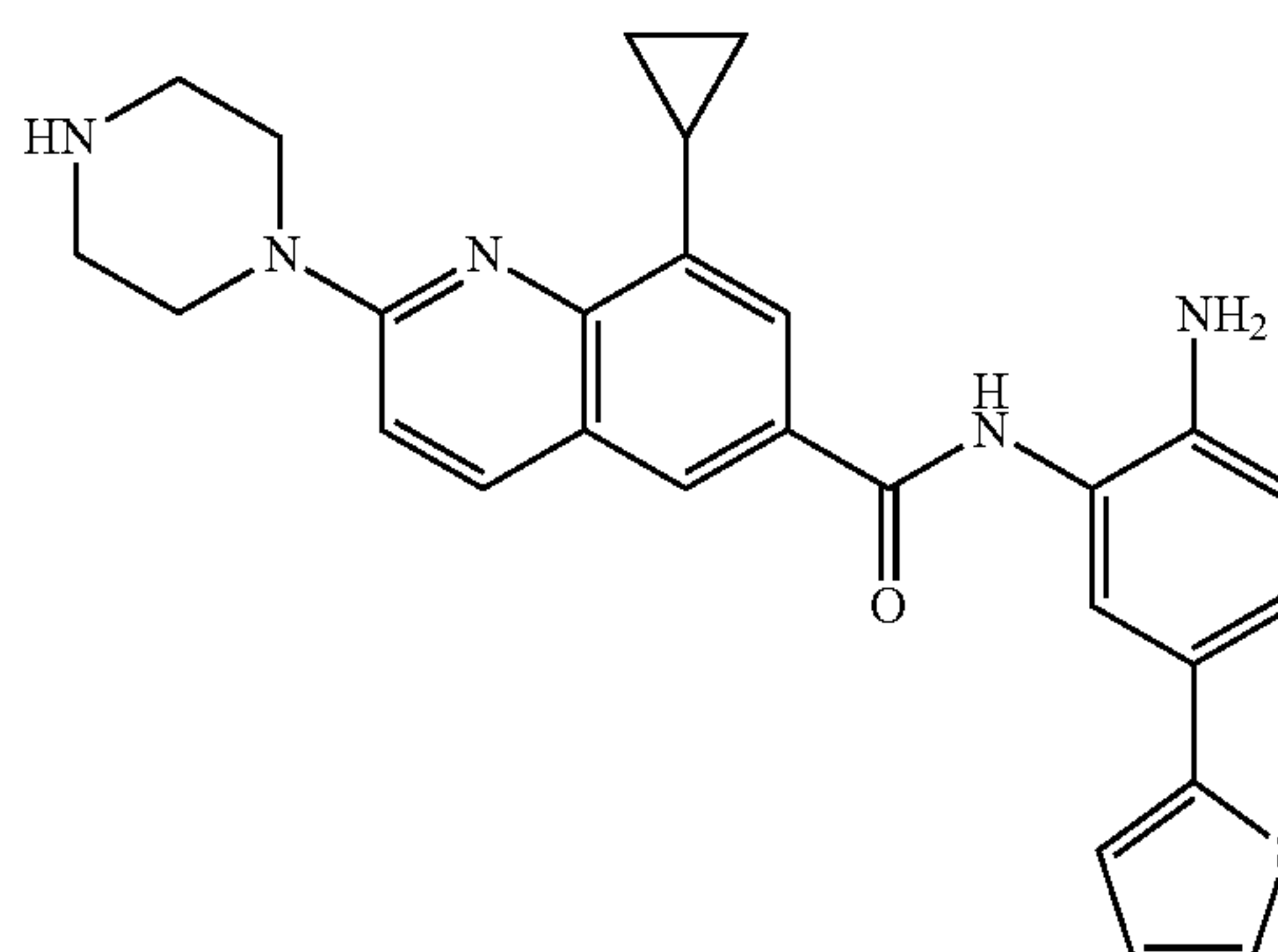
N-(2-amino-5-(thiophen-2-yl)phenyl)-8-cyclopropyl-2-(piperazin-1-yl)quinoline-6-carboxamide
