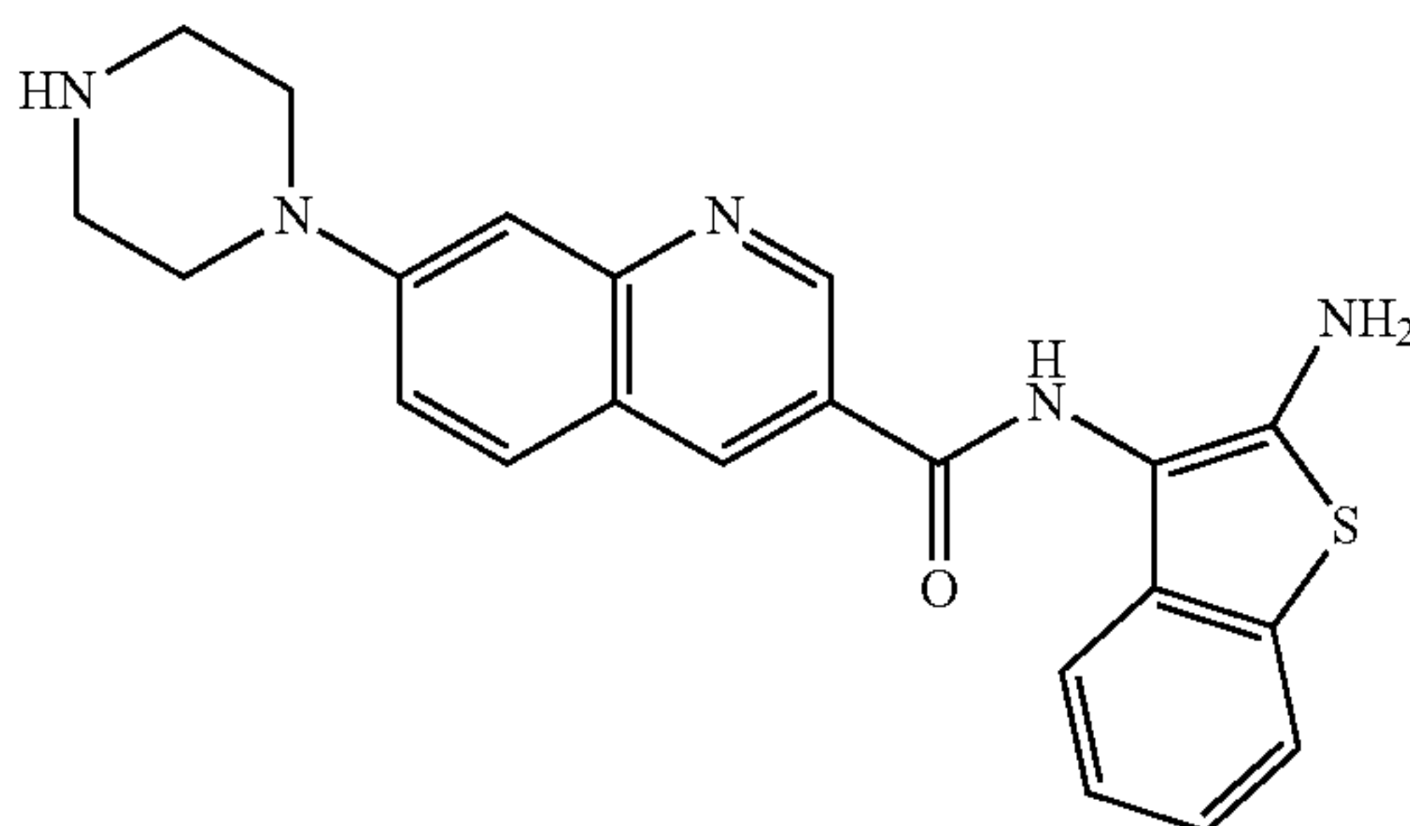
N-(2-aminobenzo[b]thiophen-3-yl)-7-(piperazin-1-yl)quinoline-3-carboxamide
