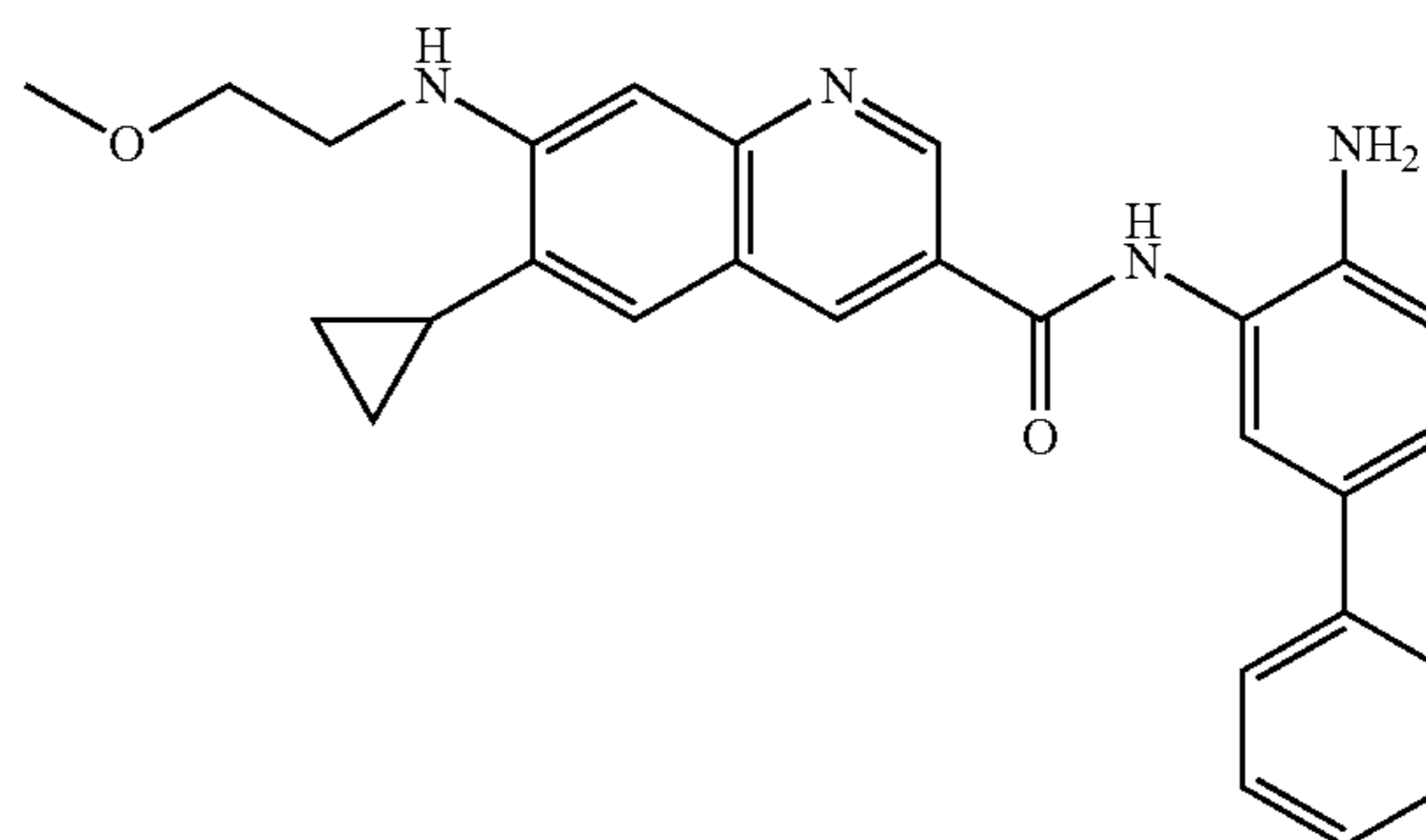
N-(4-amino-[1,1'-biphenyl]-3-yl)-6-cyclopropyl-7-((2-methoxyethyl)amino)quinoline-3-carboxamide
