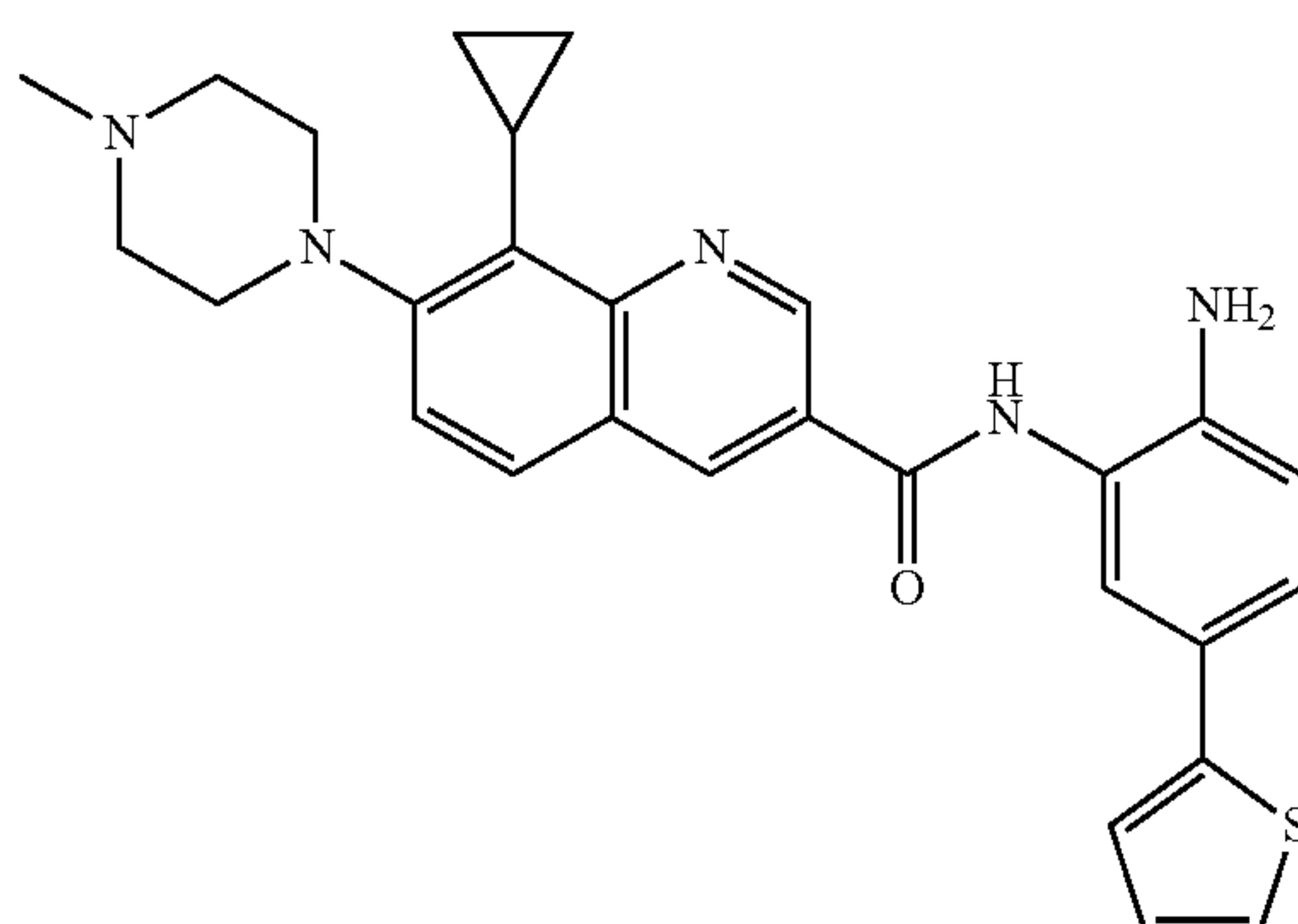
N-(2-amino-5-(thiophen-2-yl)phenyl)-8-cyclopropyl-7-(4-methylpiperazin-1-yl)quinoline-3-carboxamide
