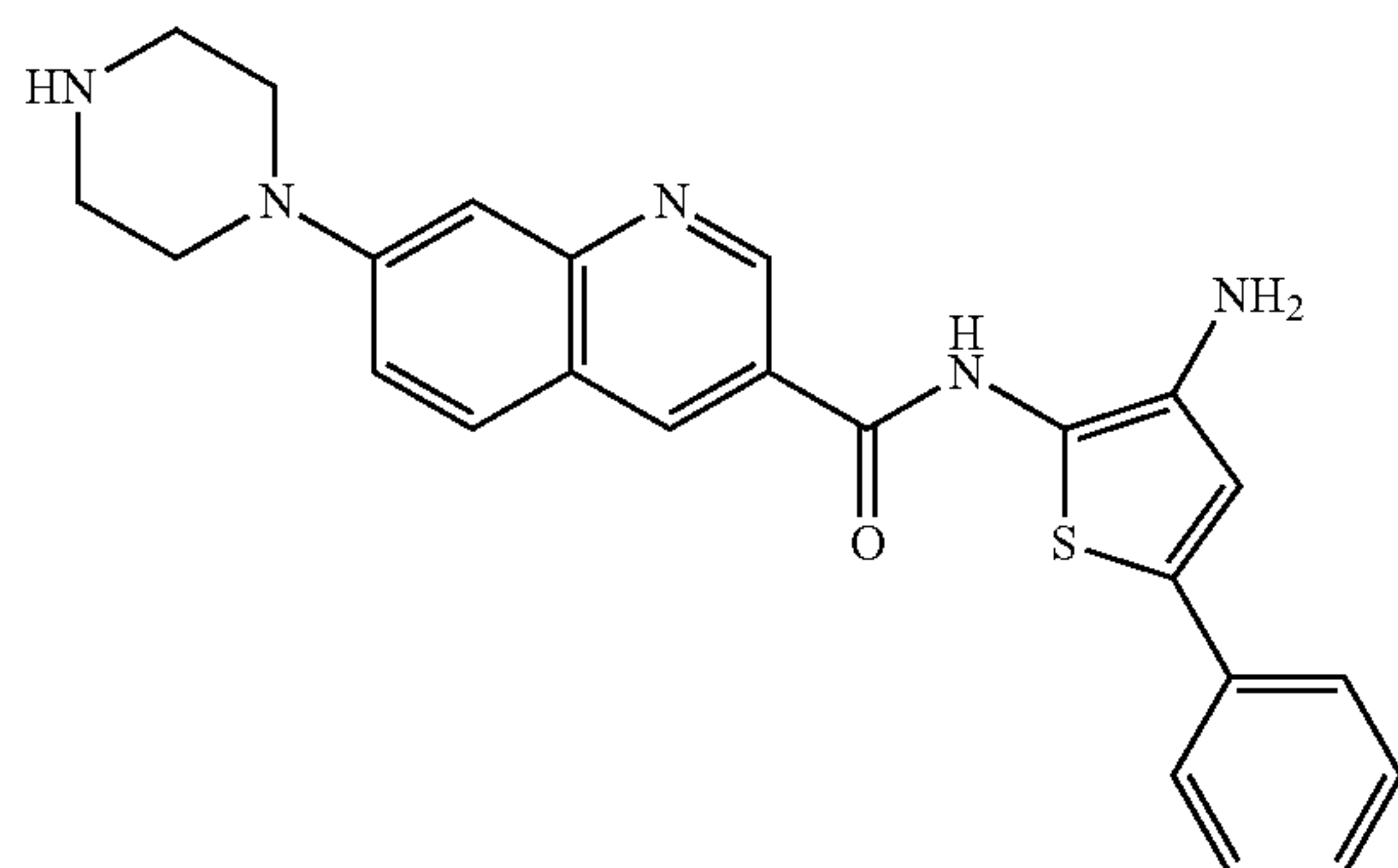
N-(3-amino-5-phenylthiophen-2-yl)-7-(piperazin-1-yl)quinoline-3-carboxamide
