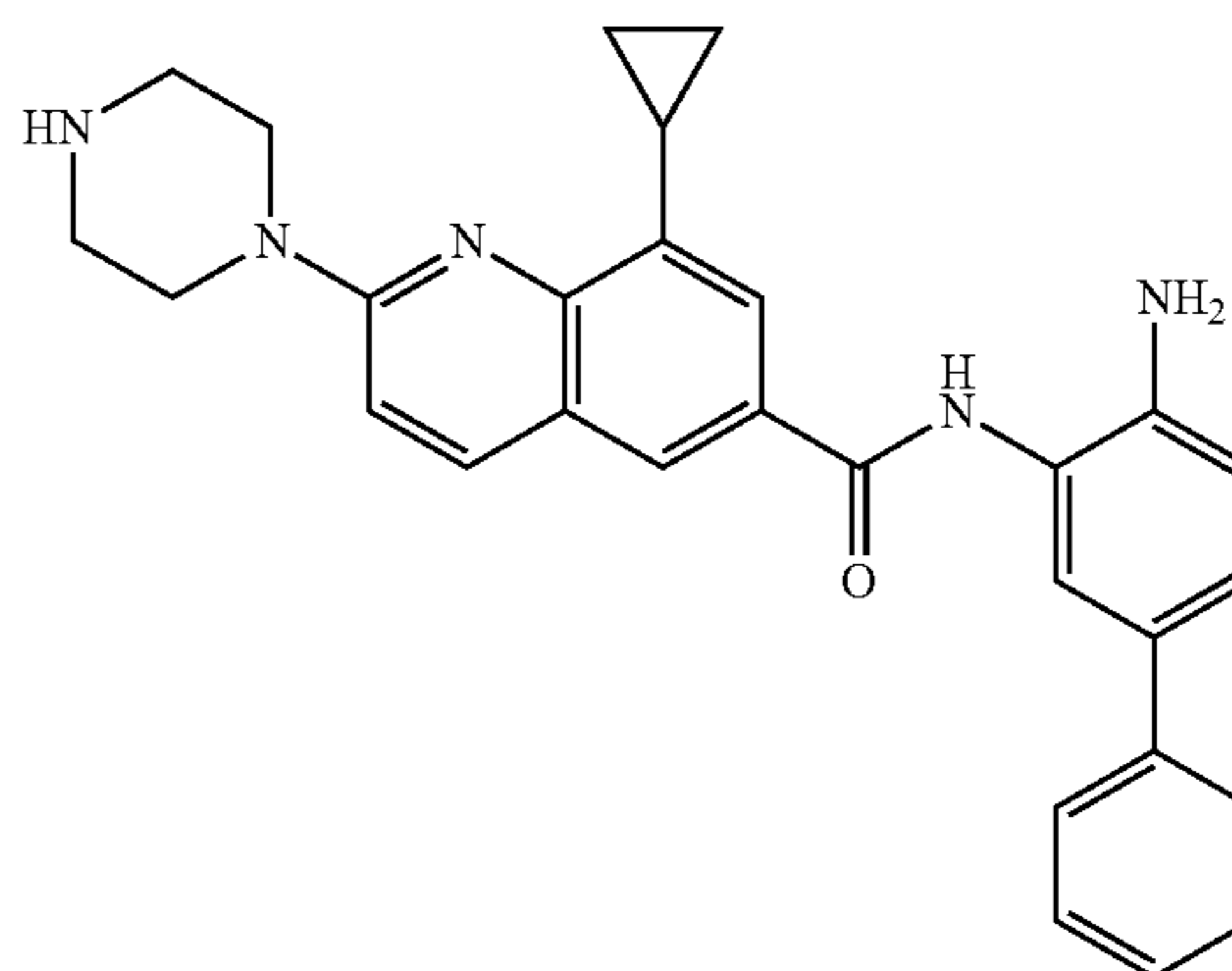
N-(4-amino-[1,1'-biphenyl]-3-yl)-8- cyclopropyl-2-(piperazin-1-yl)quinoline-6- carboxamide
