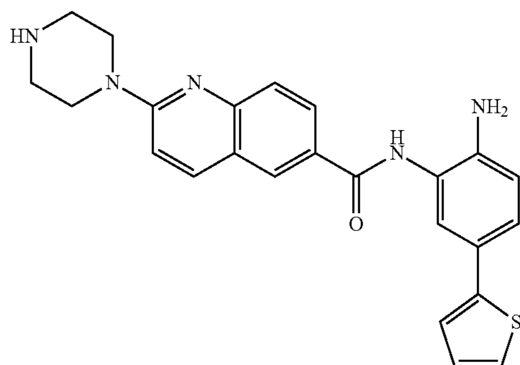
N-(2-amino-5-(thiophen-2-yl)phenyl)-2-(piperazin-1-yl)quinoline-6-carboxamide, Compound 001 IC_{50}(nM) HDAC1 = 4 HDAC2 = 15 HDAC3 = 114
