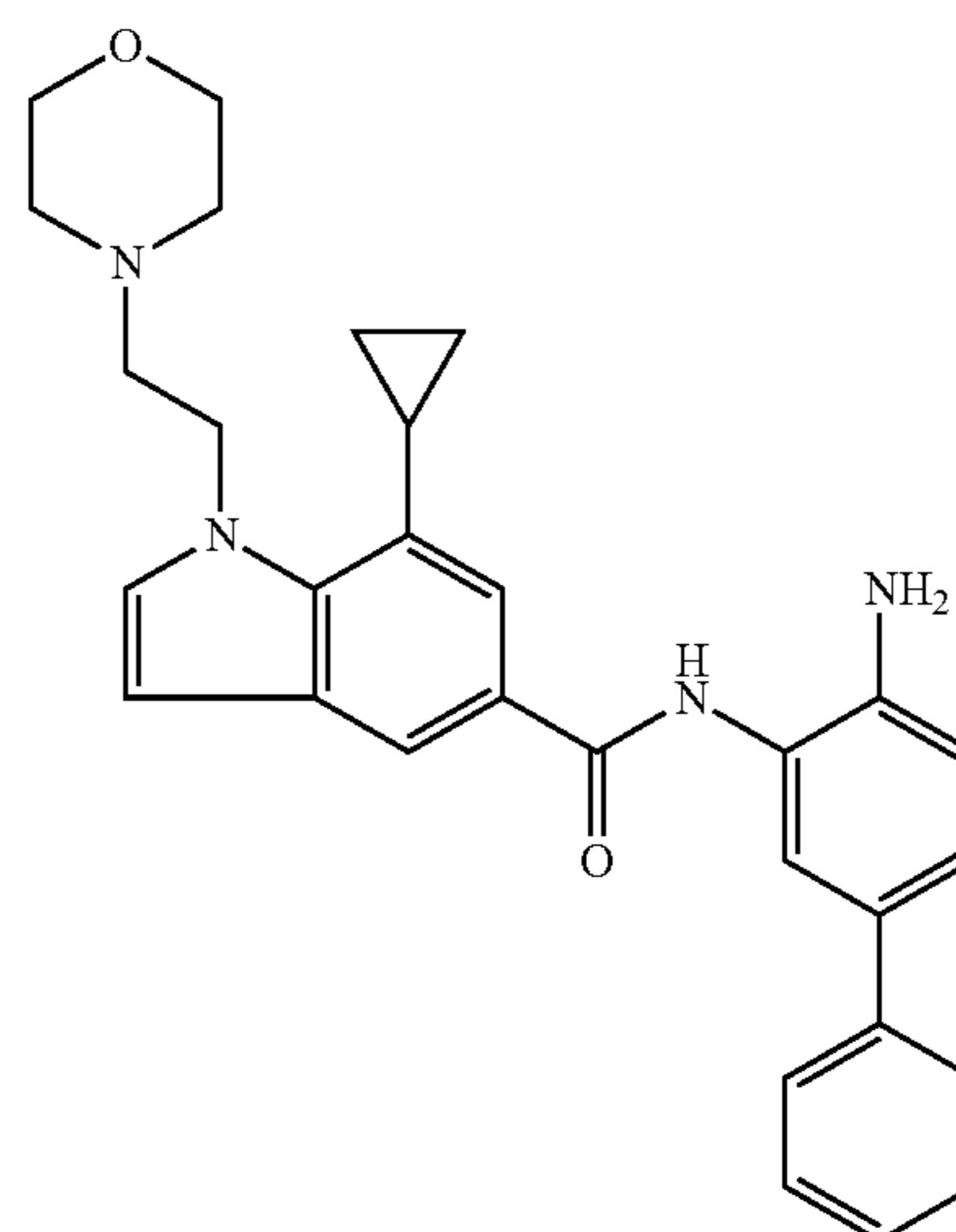
N-(4-amino-[1,1'-biphenyl]-3-yl)-7-cyclopropyl-1-(2-morpholinoethyl)-1H-indole-5-carboxamide
