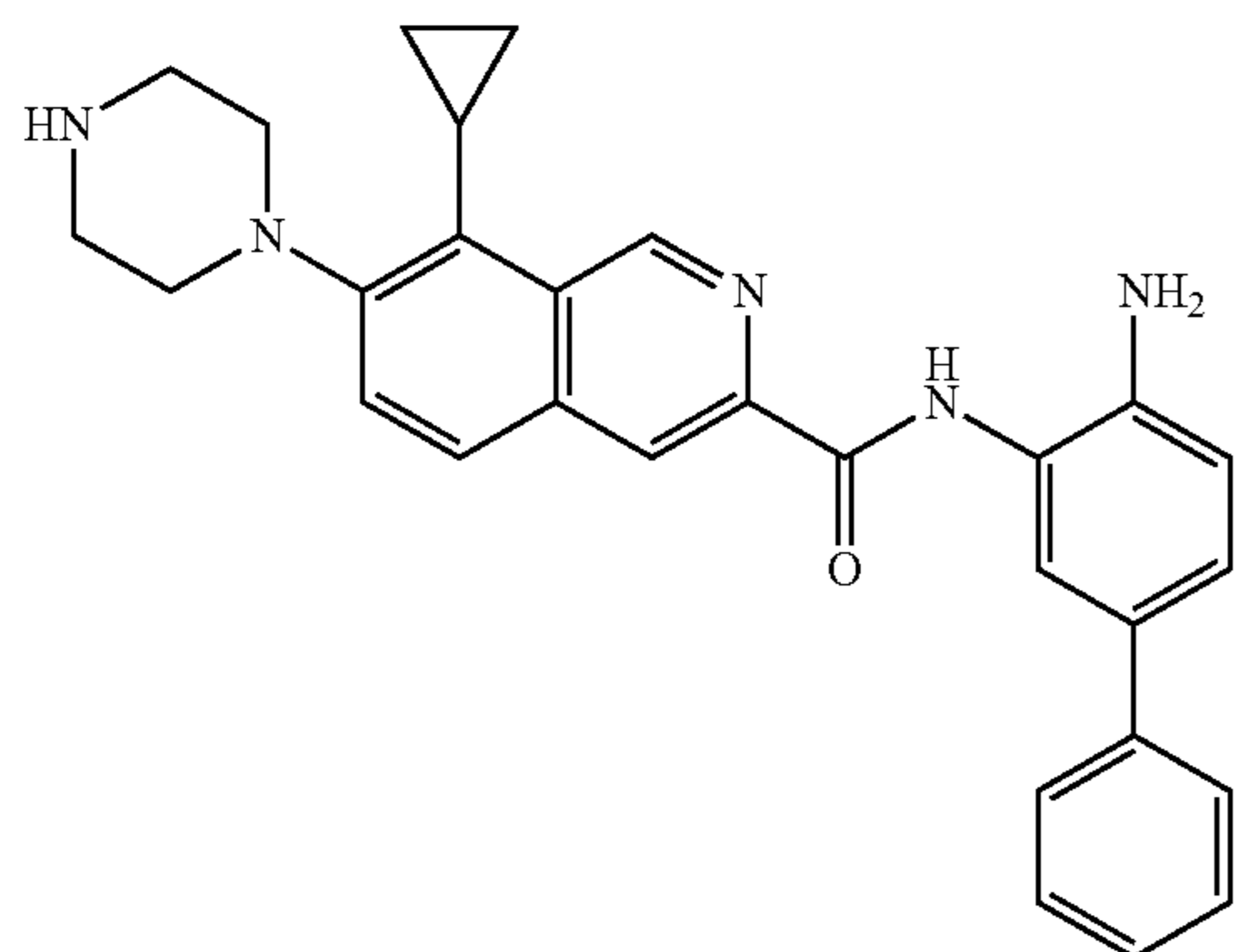
N-(4-amino-[1,1'-biphenyl]-3-yl)- cyclopropyl-7-(piperazin-1-yl)isoquinoline-3- carboxamide
