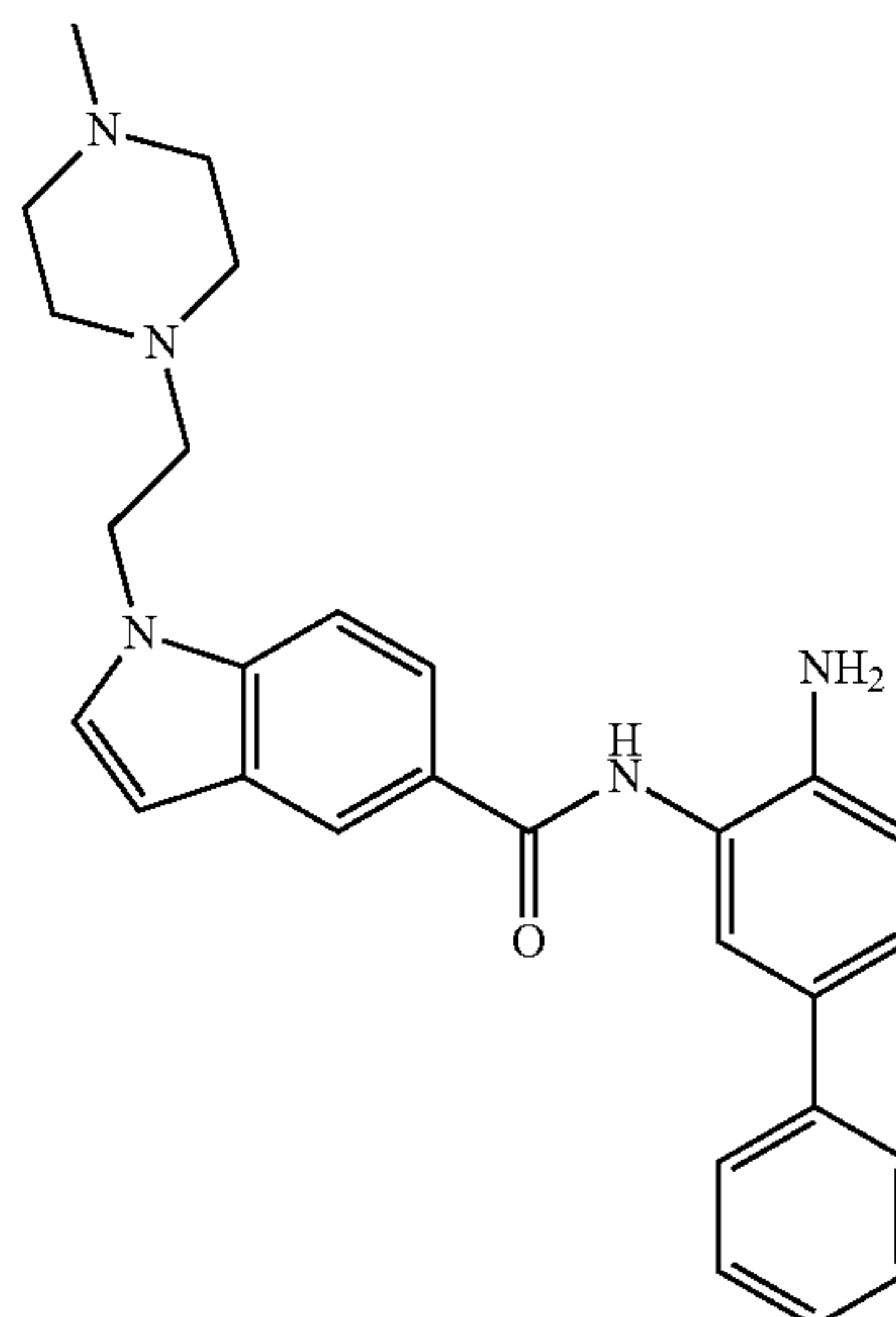
N-(4-amino-[1,1'-biphenyl]-3-yl)-1-(2-(4-methylpiperazin-1-yl)ethyl)-1H-indole-5-carboxamide
