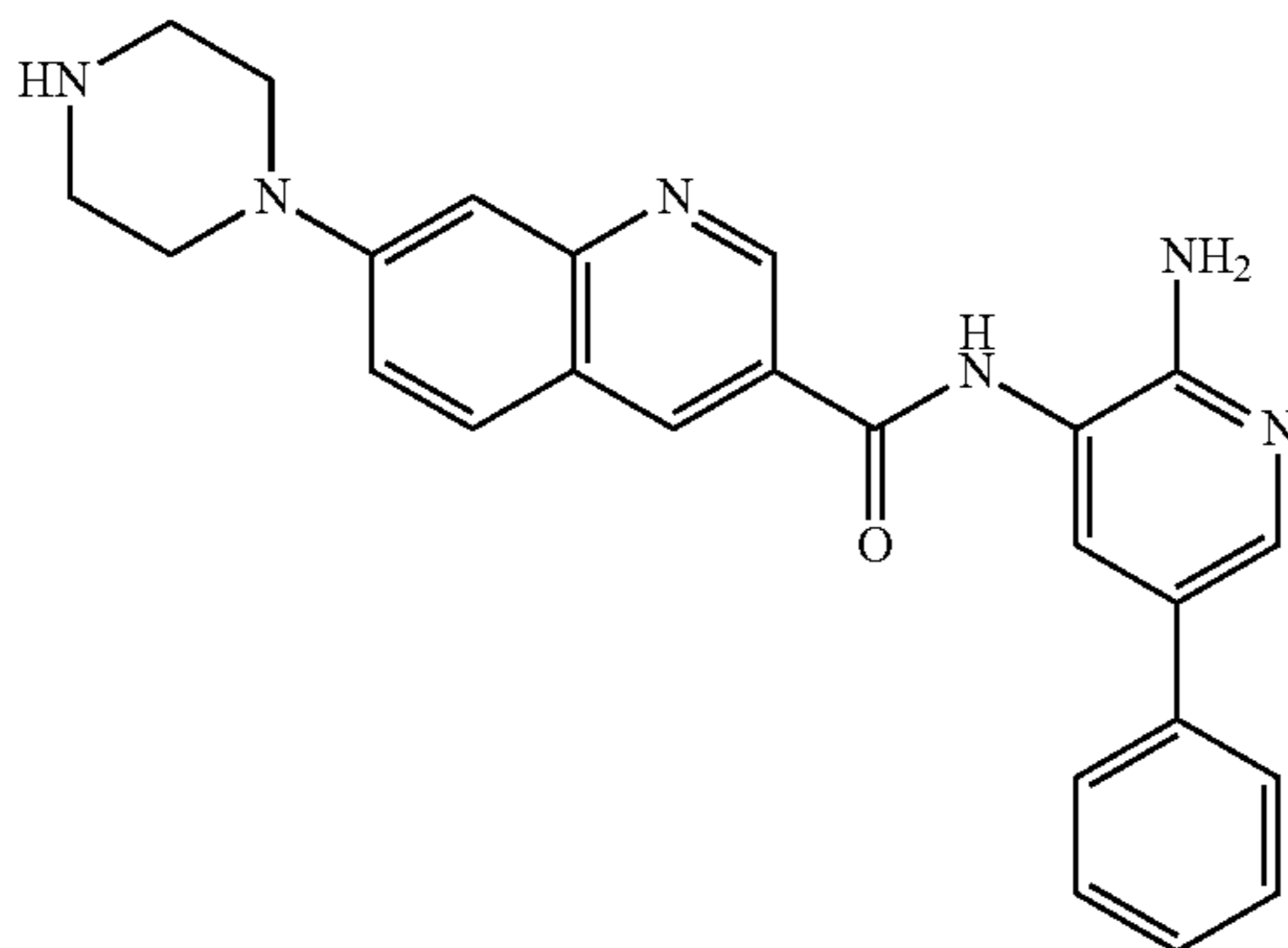
N-(2-amino-5-phenylpyridin-3-yl)-7-(piperazin-1-yl)quinoline-3-carboxamide
