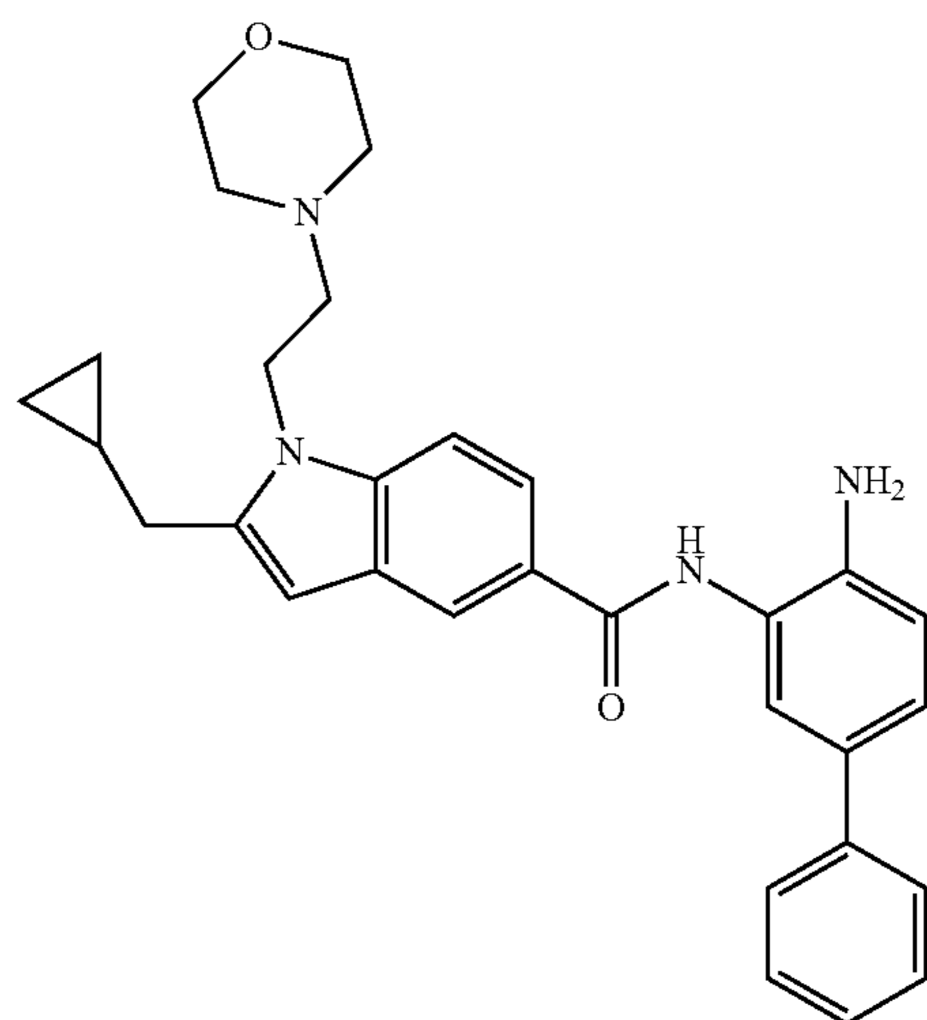
N-(4-amino-[1,1'-biphenyl]-3-yl)-2- (cyclopropylmethyl)-1-(2-morpholinoethyl)- 1H-indole-5-carboxamide
