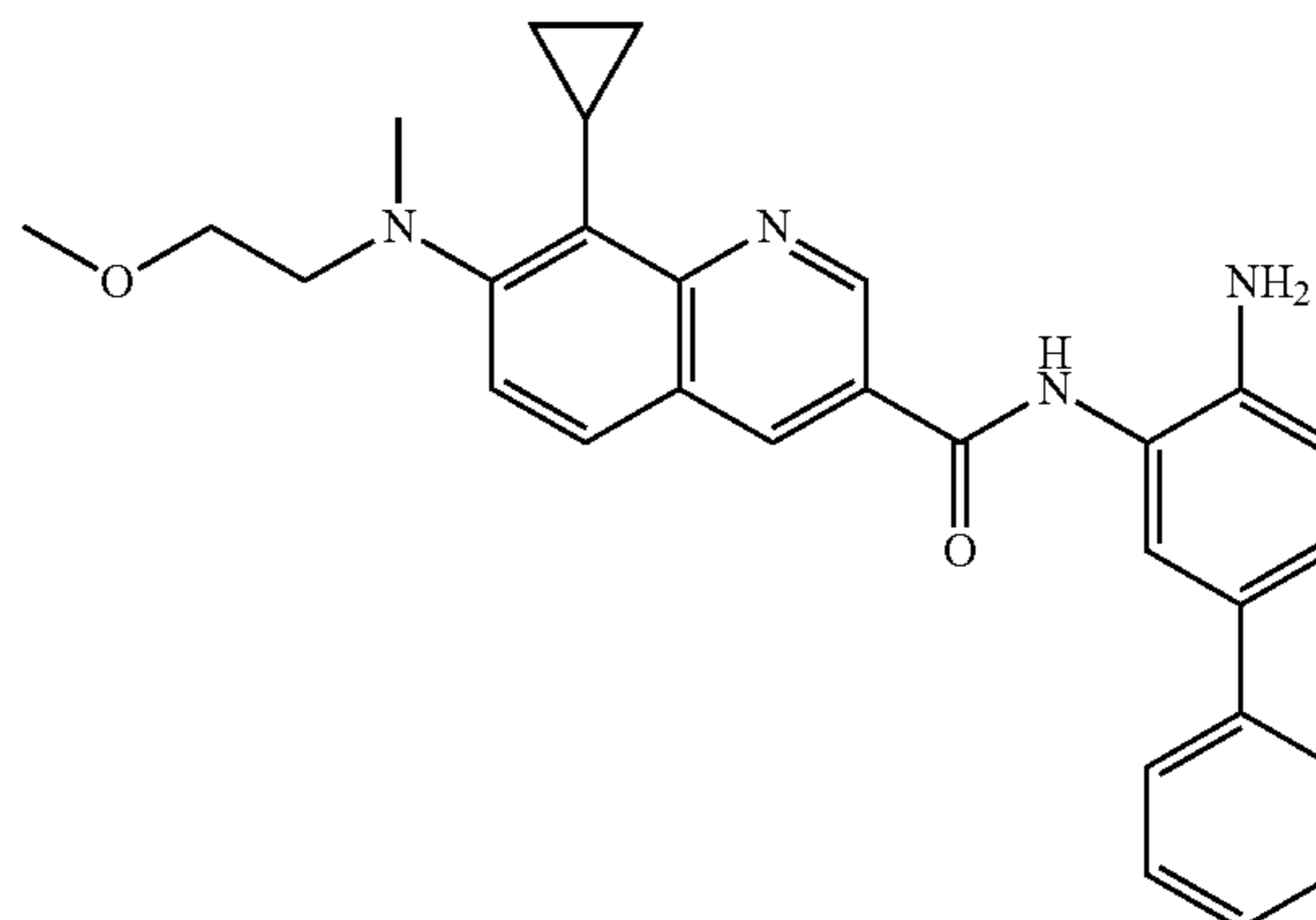
N-(4-amino-[1,1'-biphenyl]-3-yl)-8-cyclopropyl-7-((2-methoxyethyl)(methyl)amino)quinoline-3-carboxamide
