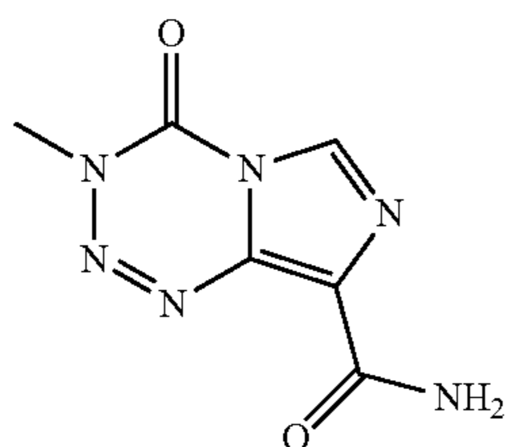
Temozolomide (TMZ)
