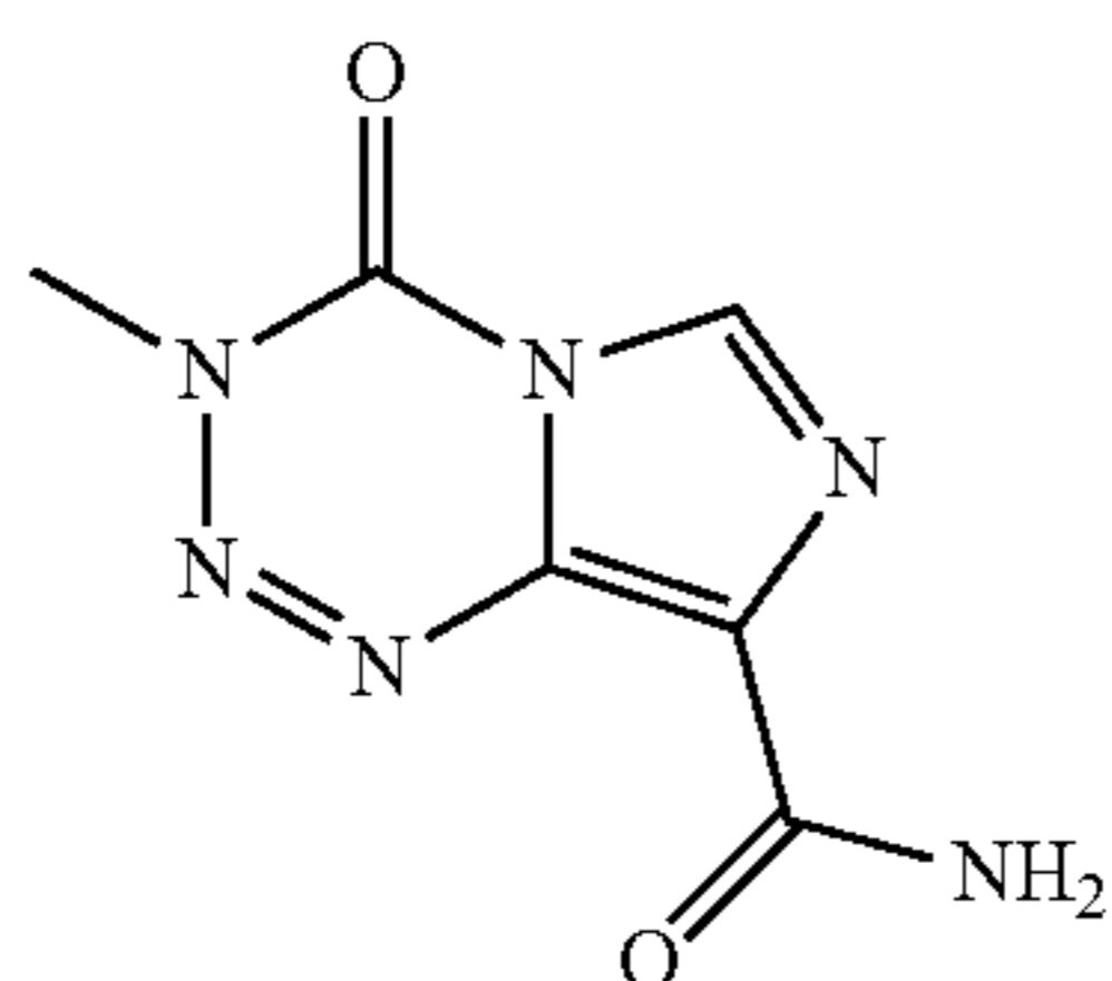
Temozolomide (TMZ)
