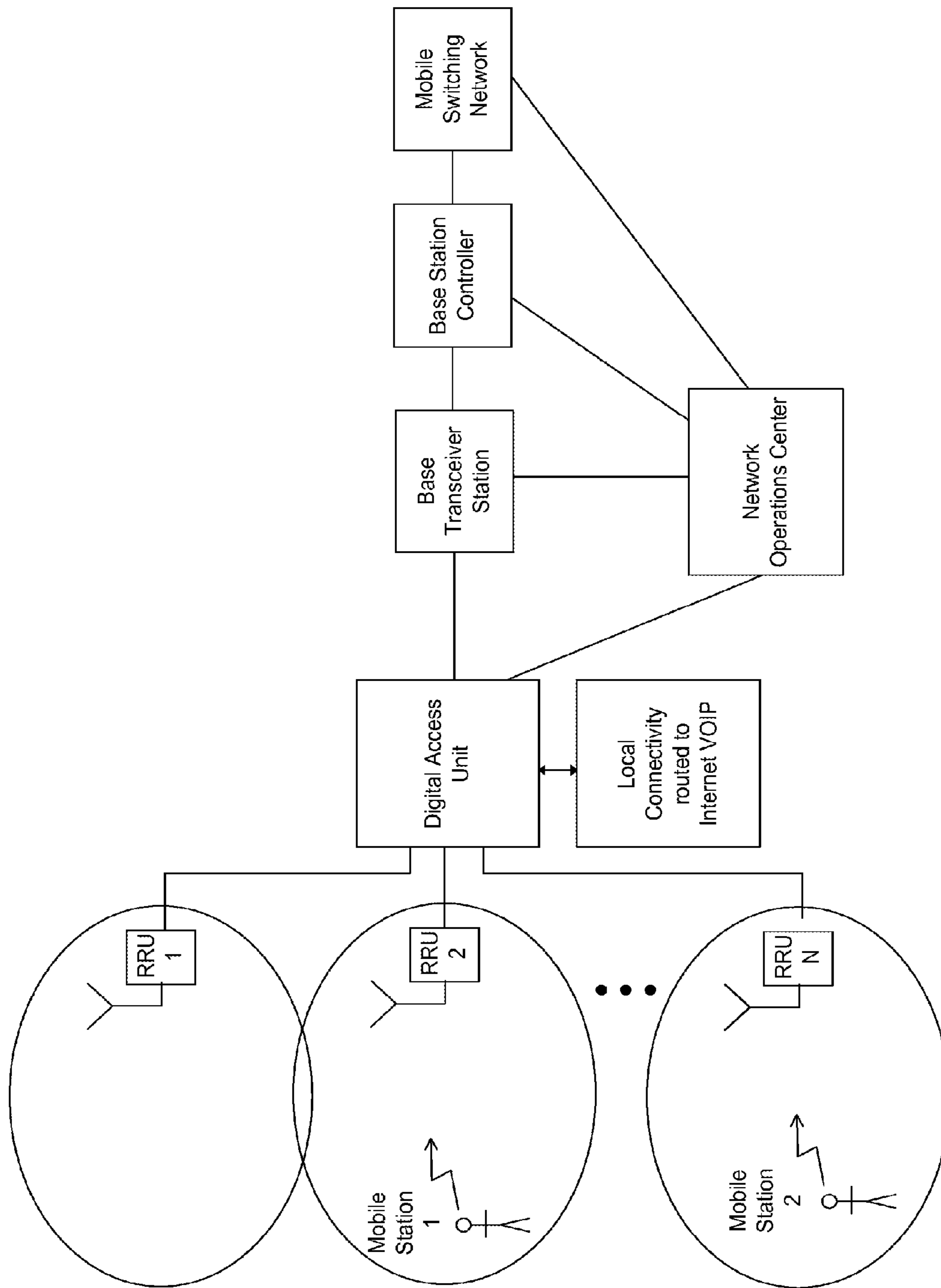
Figure 6 Local Connectivity
