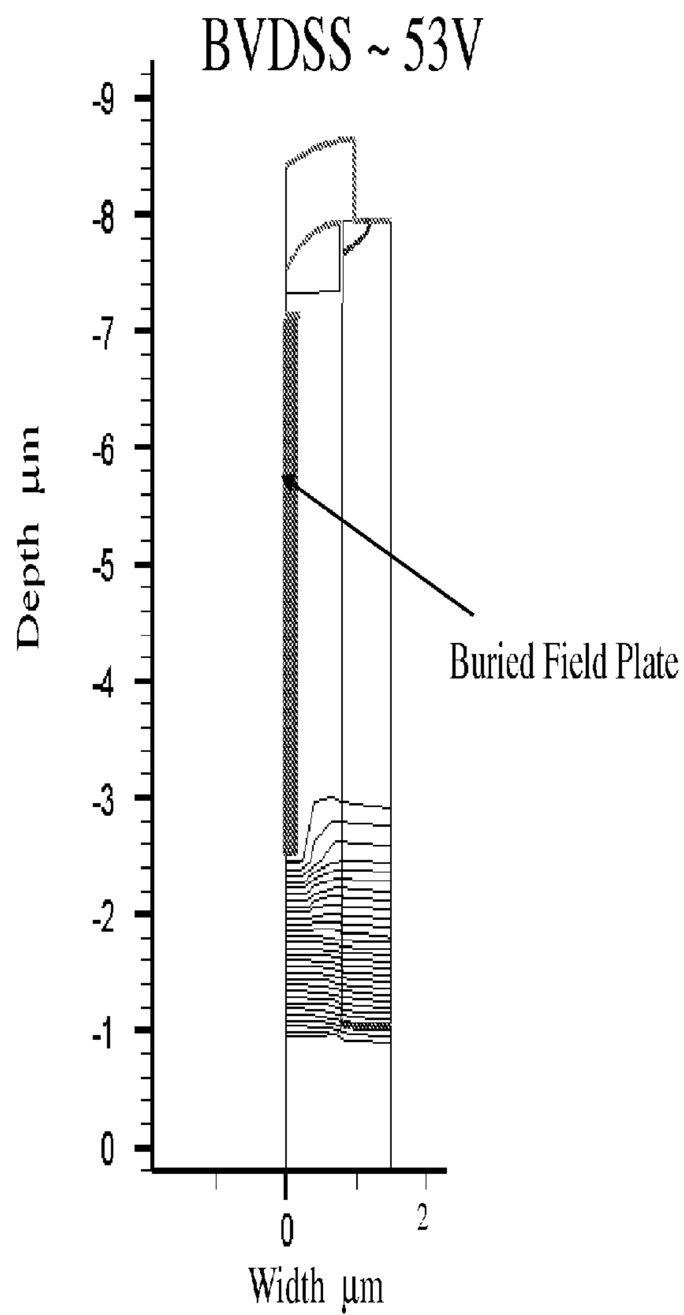
Figure 3C MOSFET with buried field plate and low Q_F
