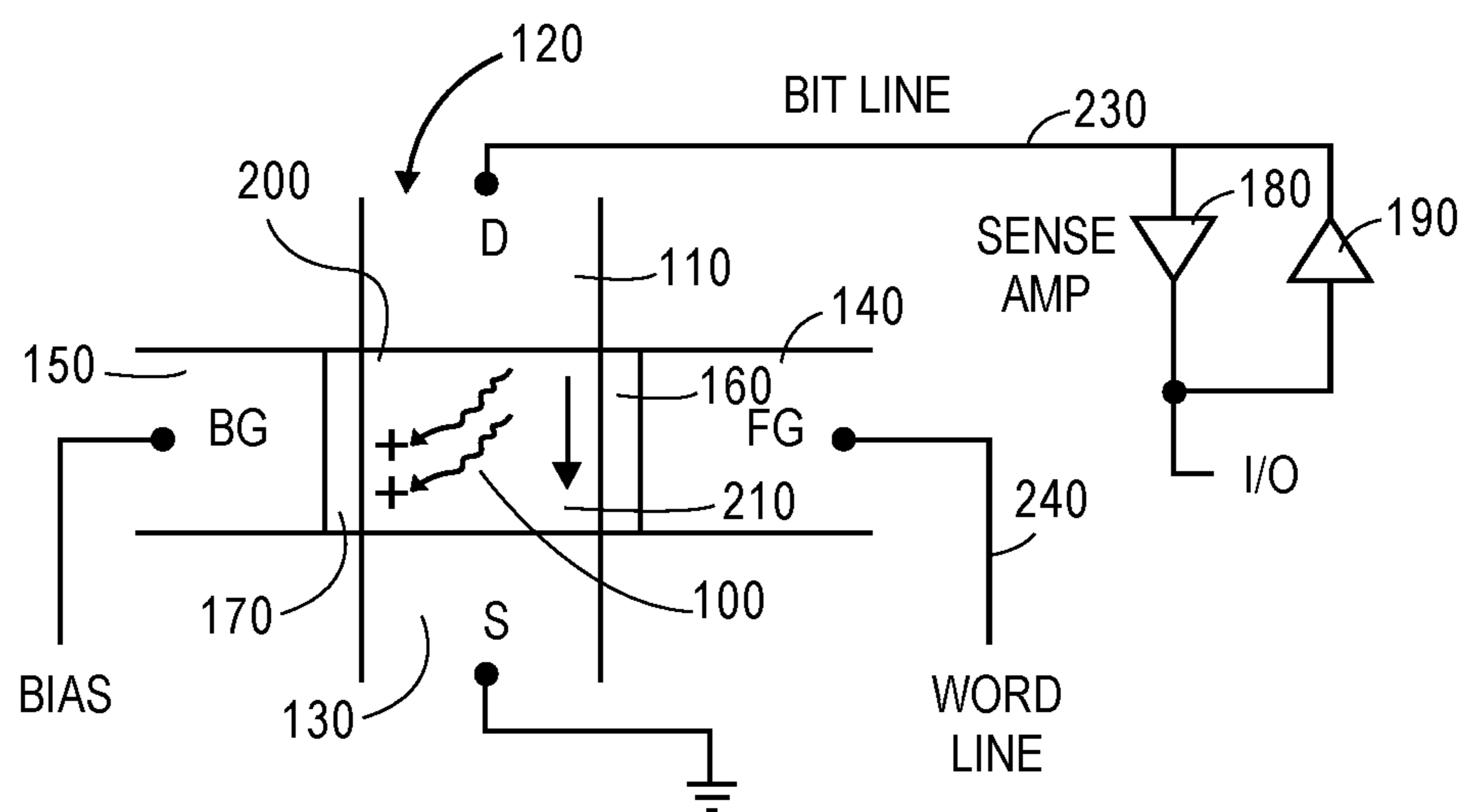
FIG. 1 (PRIOR ART)
