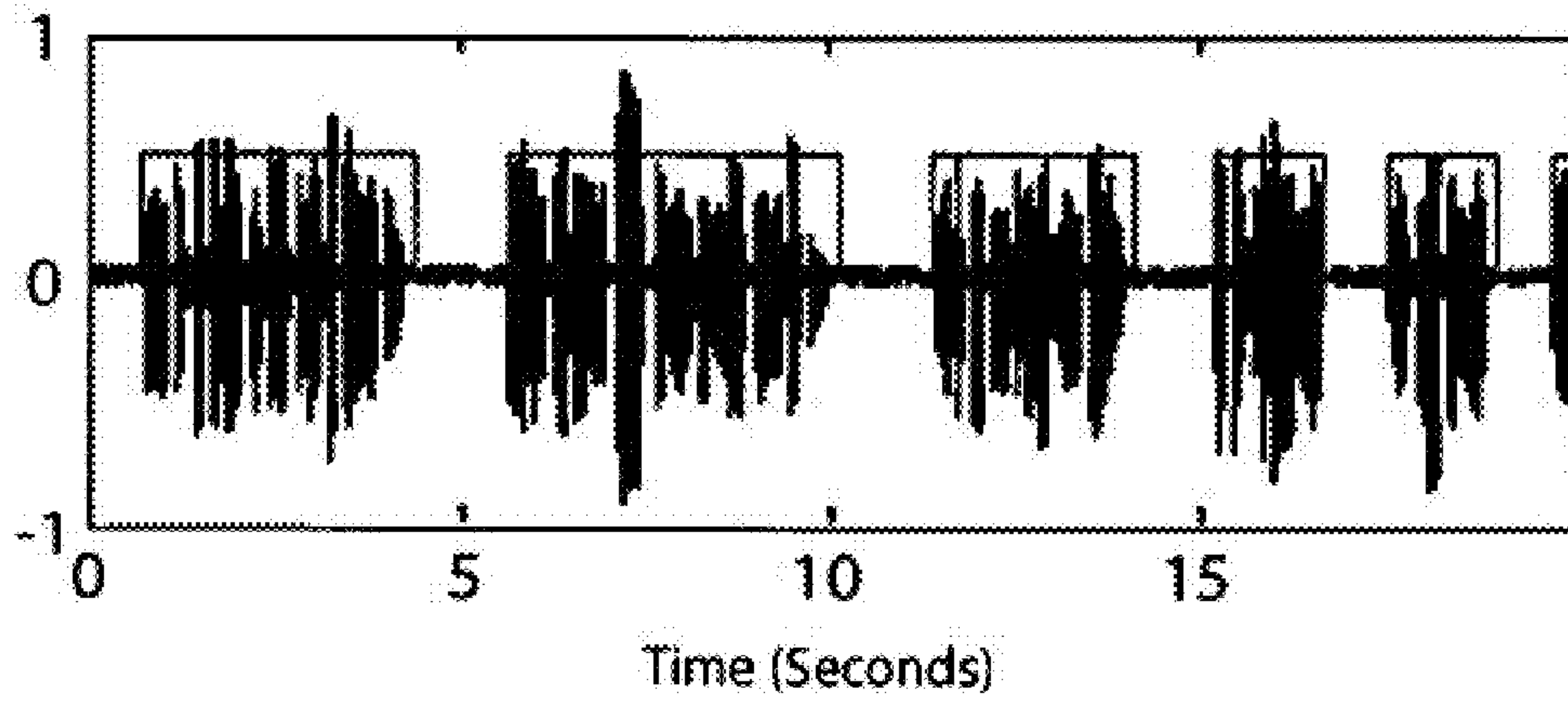
Energy-based Algorithm
