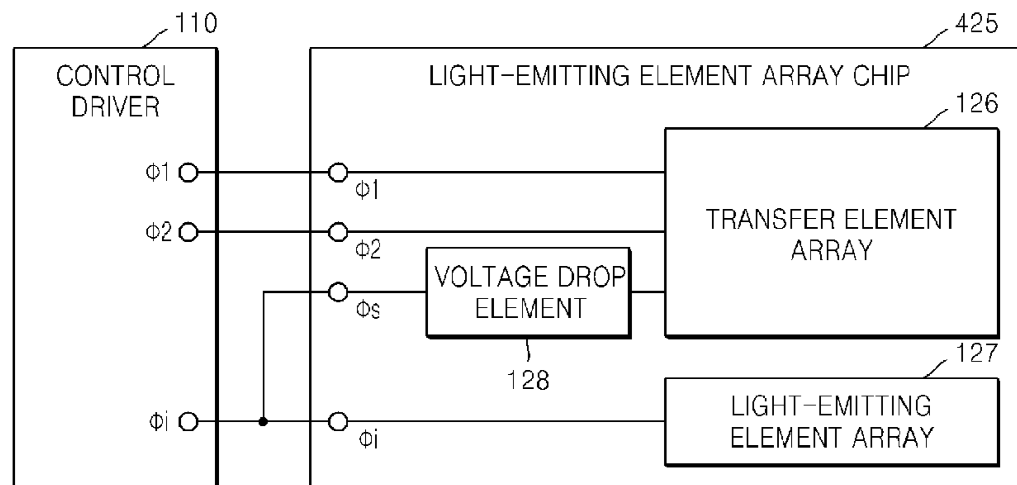
LIGHT-EMITTING ELEMENT ARRAY MODULE 400
