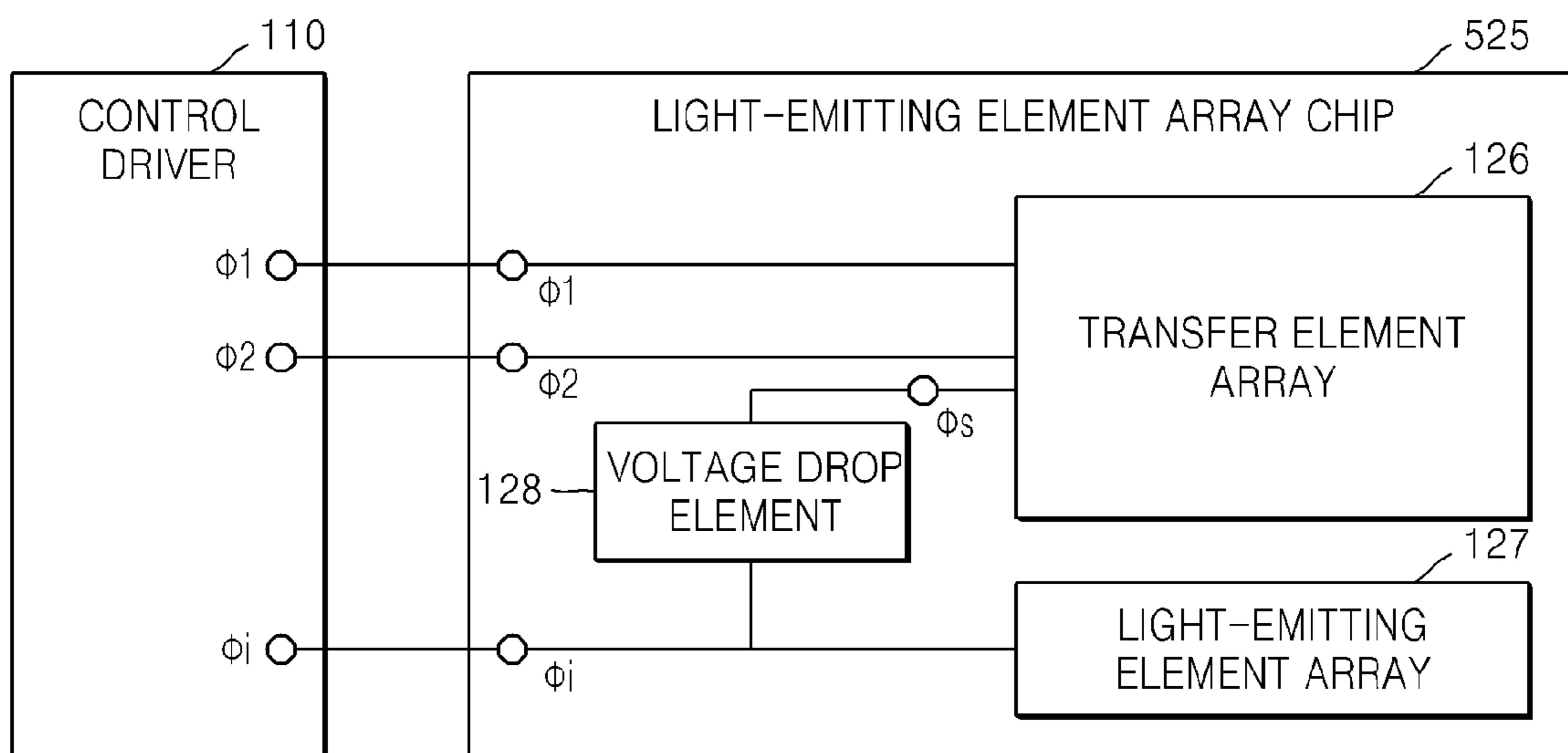
LIGHT-EMITTING ELEMENT ARRAY MODULE 500
