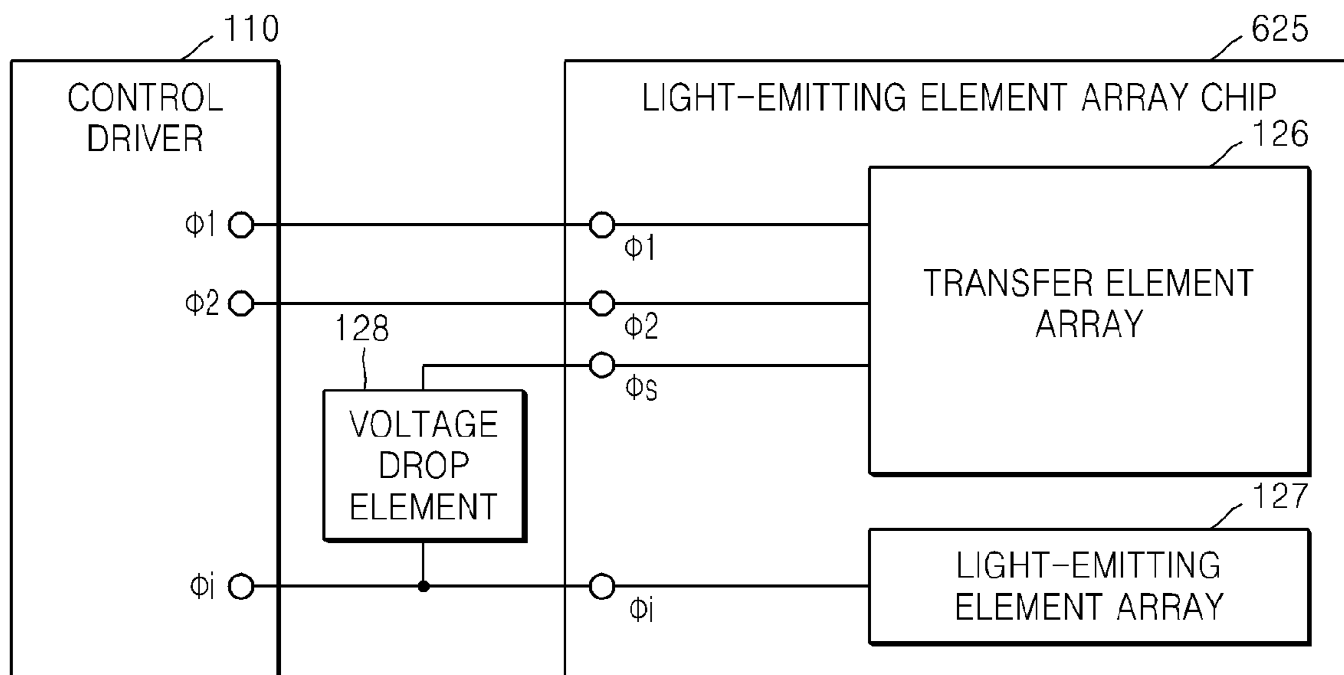
LIGHT-EMITTING ELEMENT ARRAY MODULE 600
