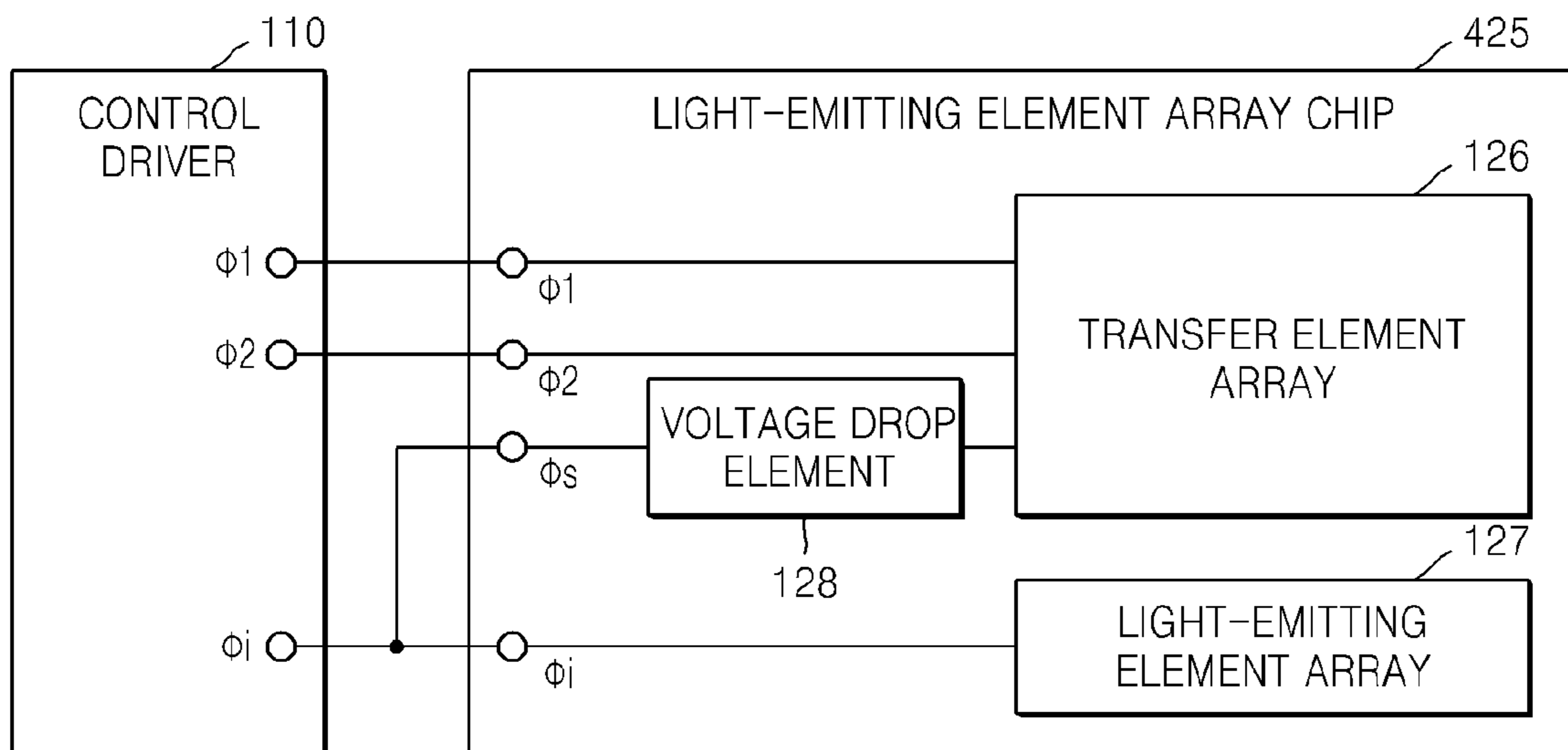
LIGHT-EMITTING ELEMENT ARRAY MODULE 400
