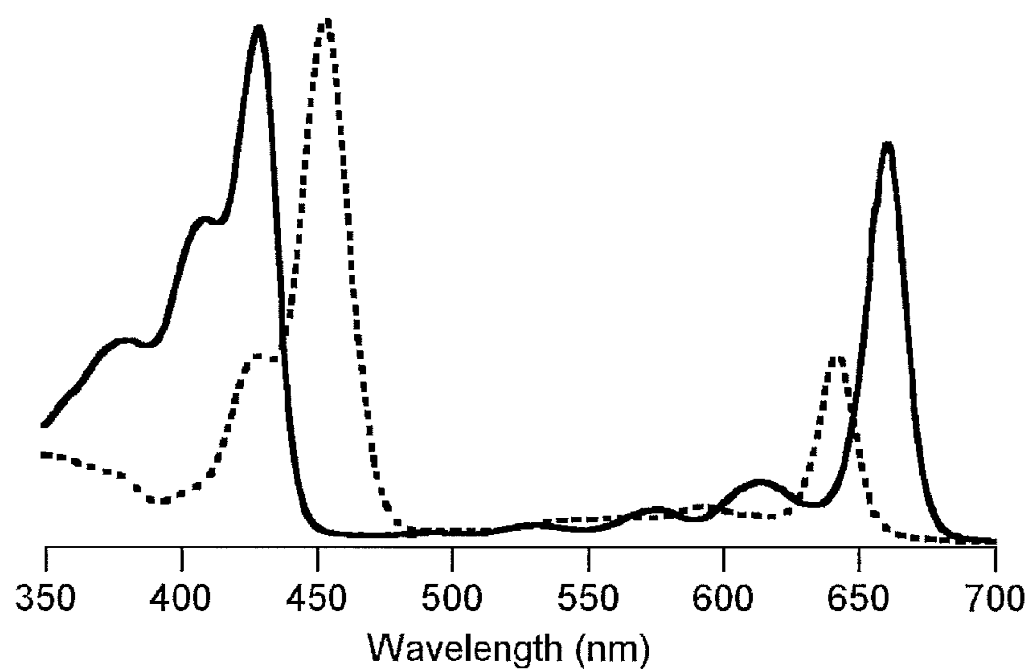
Figure 3. Absorption spectra of chlorophylls a and b.
