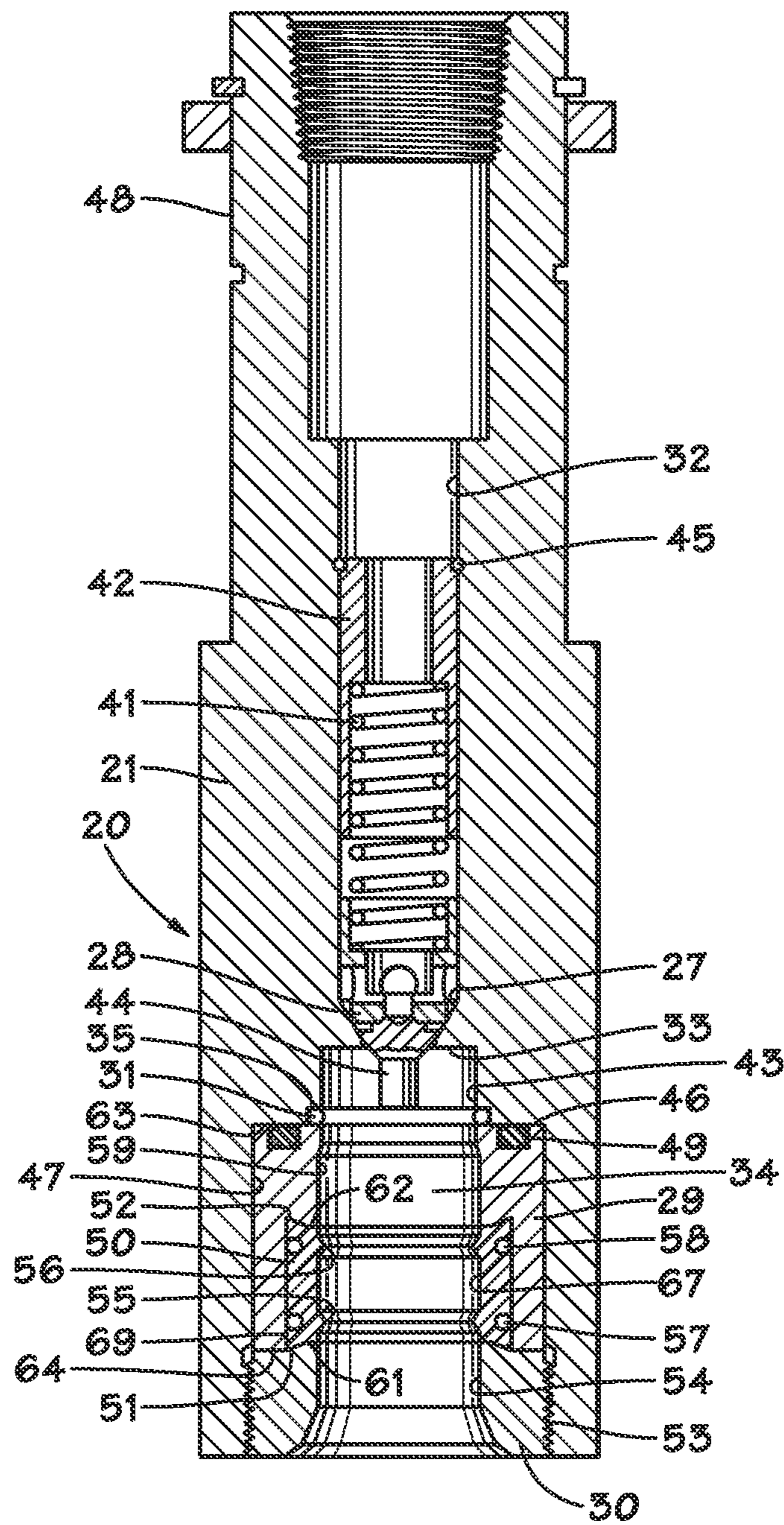
FIG. 1 (PRIOR ART)
