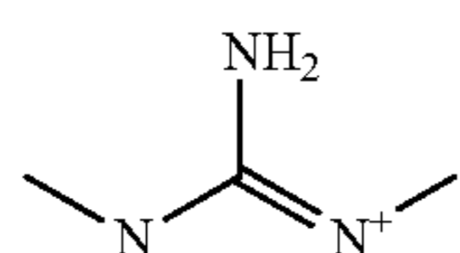
[Amino(methylamino)methylene]-methyl-ammonium
