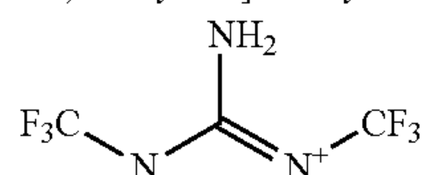
[Amino-(trifluoromethylamino)methylene]-(trifluoromethyl)ammonium
