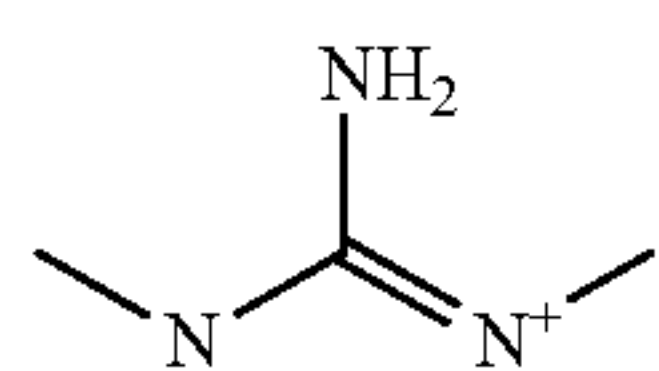
[Amino(methylamino)methylene]-methyl-ammonium
