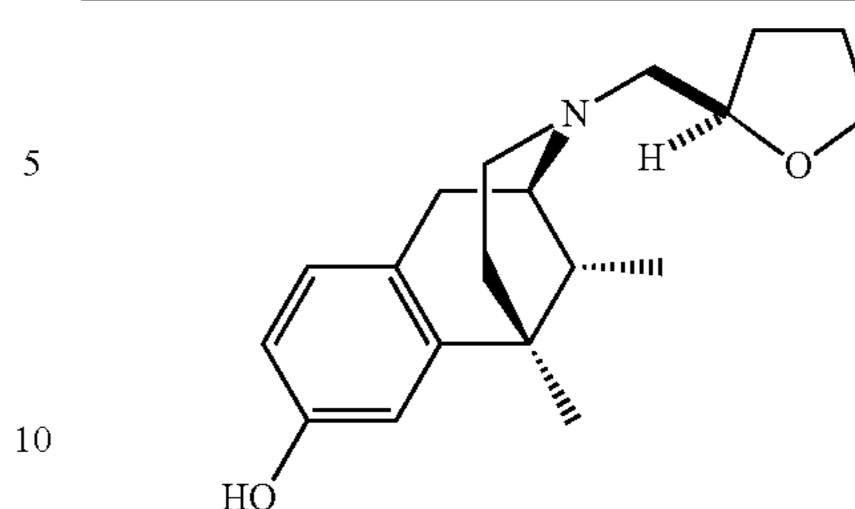
Compound 18
