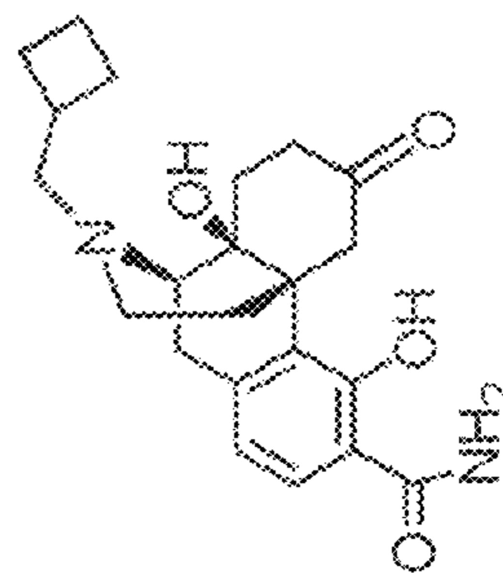
Compound A
