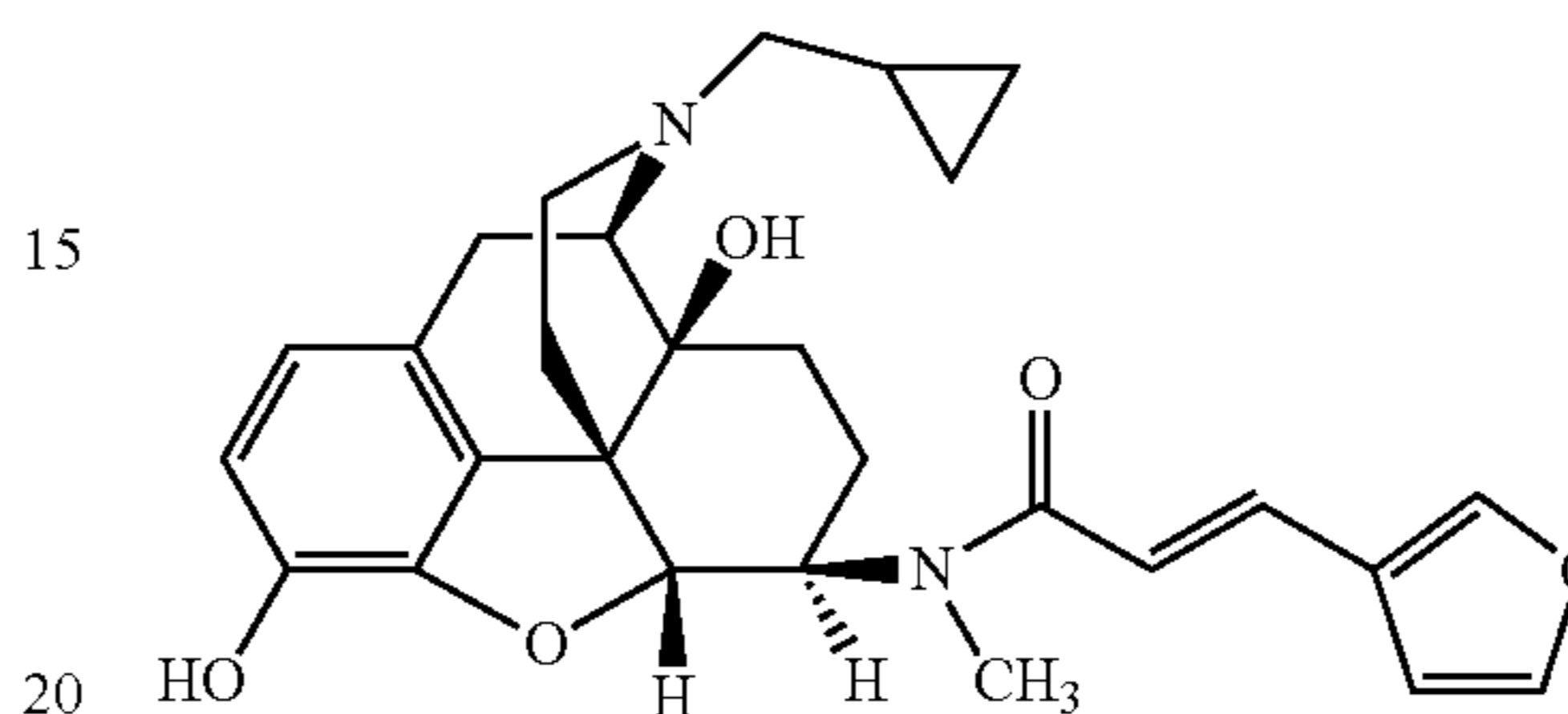
Compound 19
