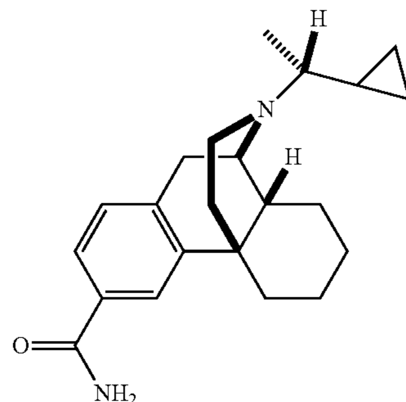
Compound 1
