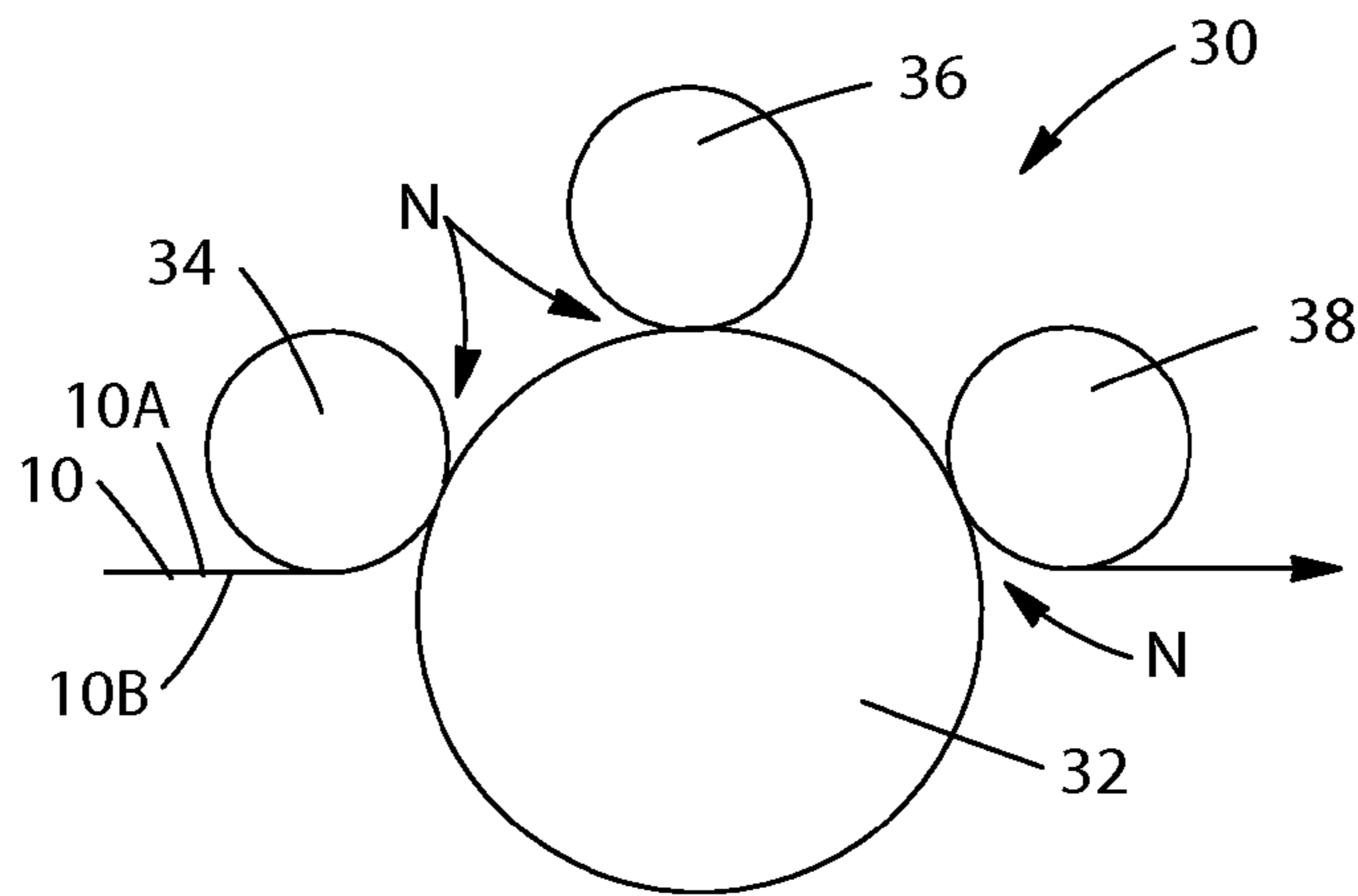
Fig. 2 Prior Art
