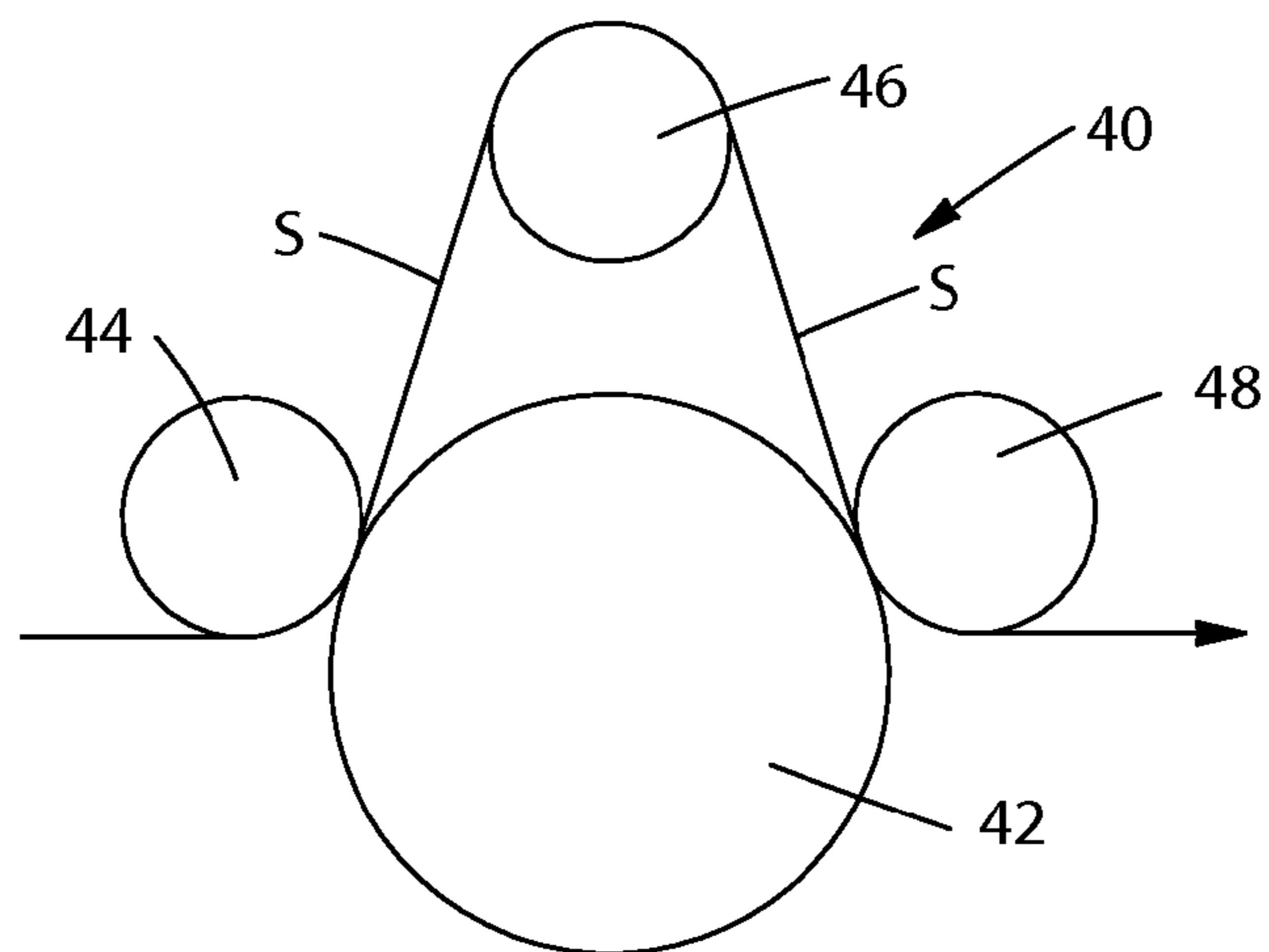
Fig. 3 Prior Art
