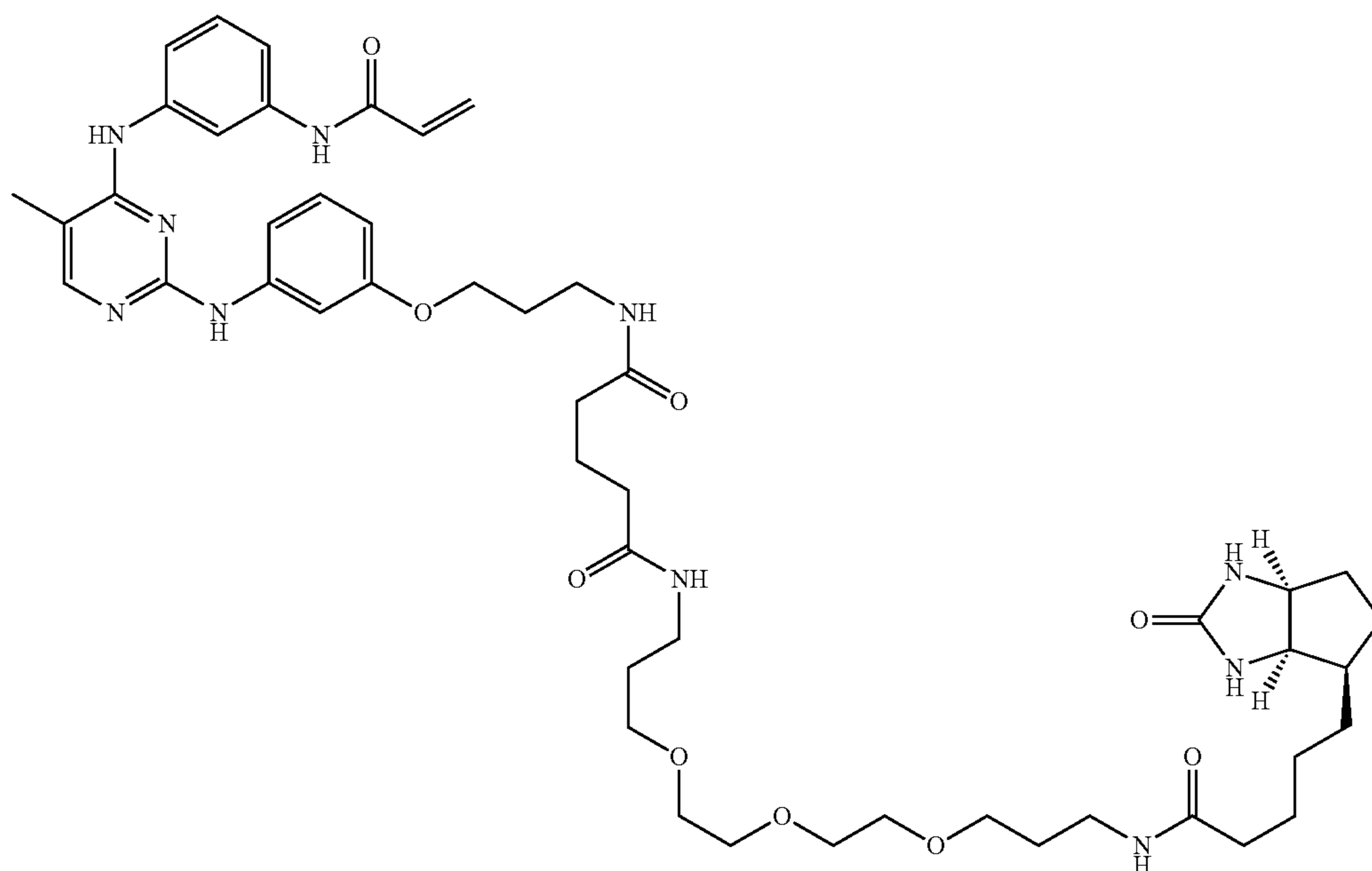
Covalent Probe
