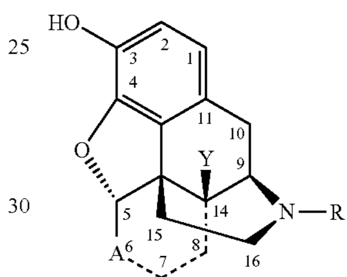
Formula 11
