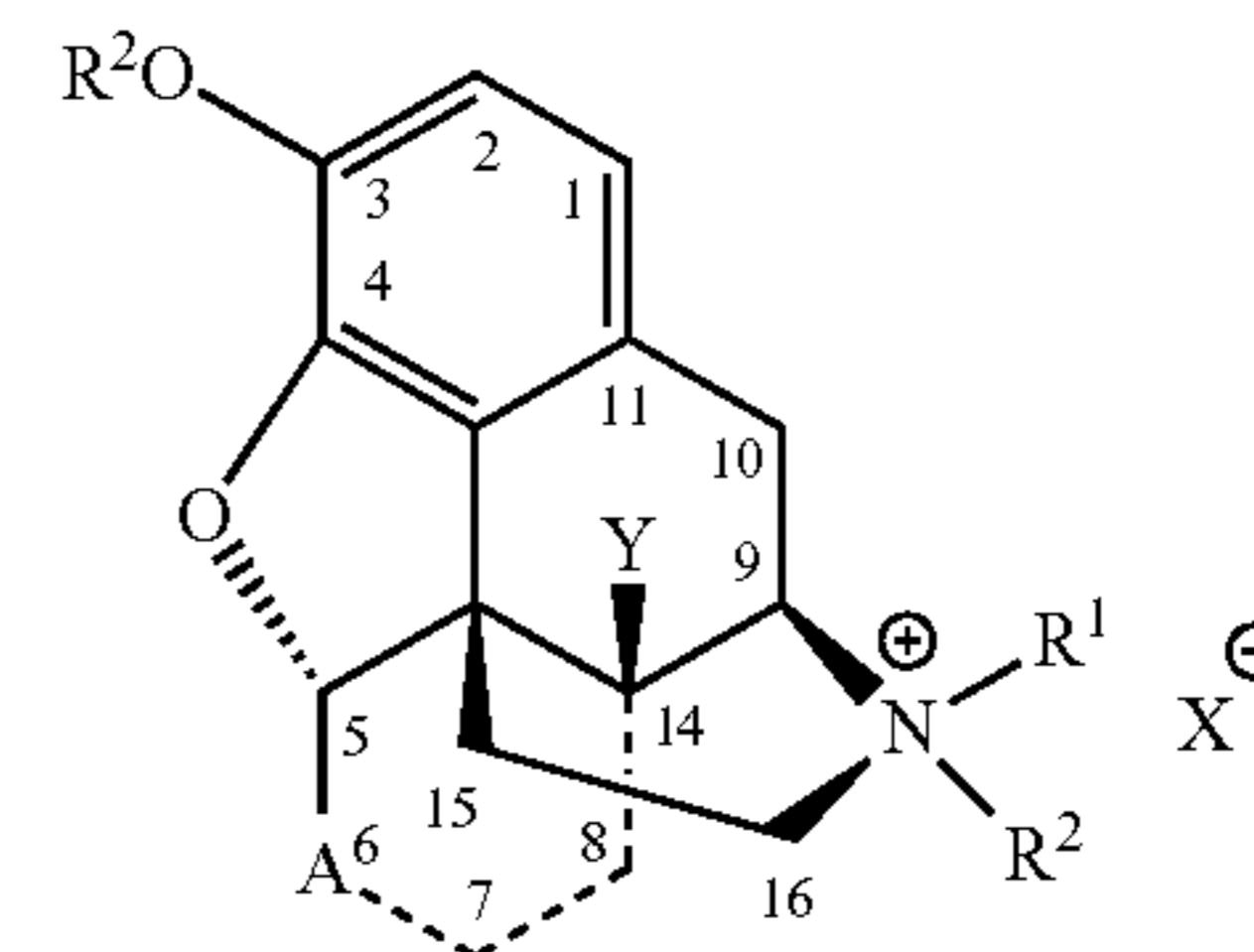
Formula 11C
