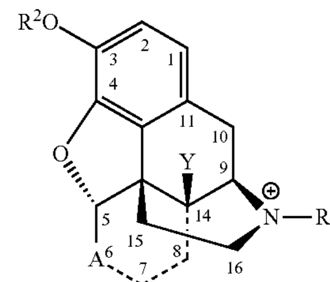
Formula 11B
