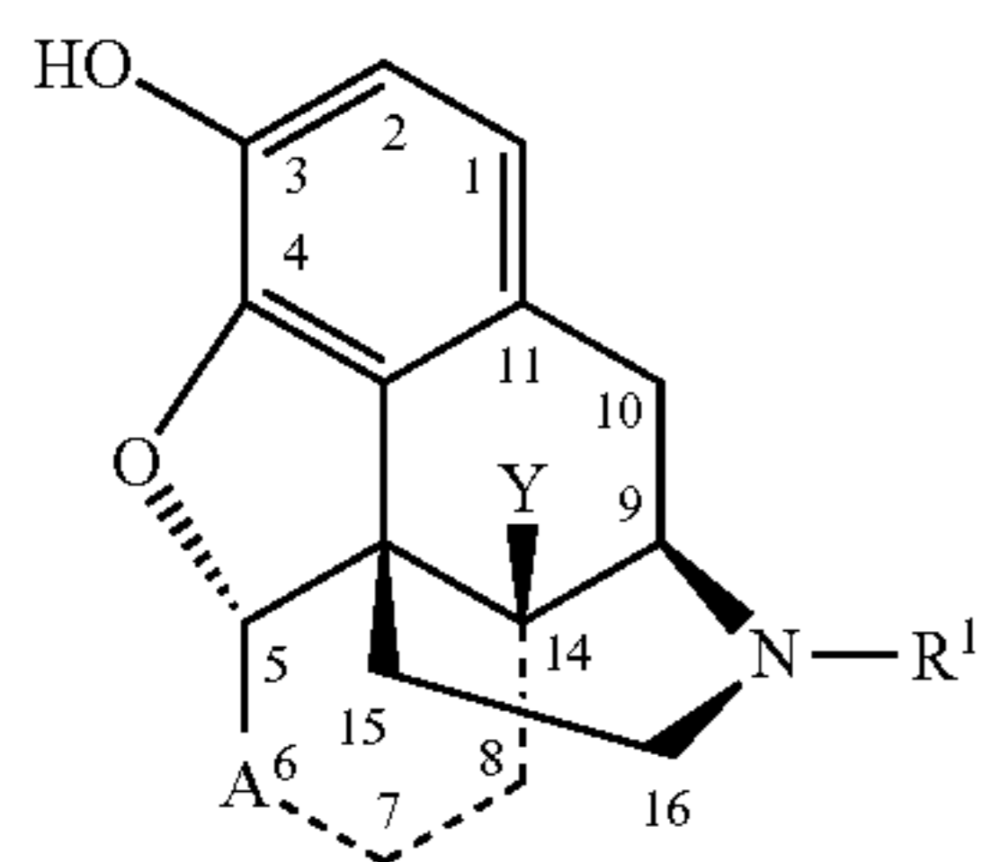
Formula 11
