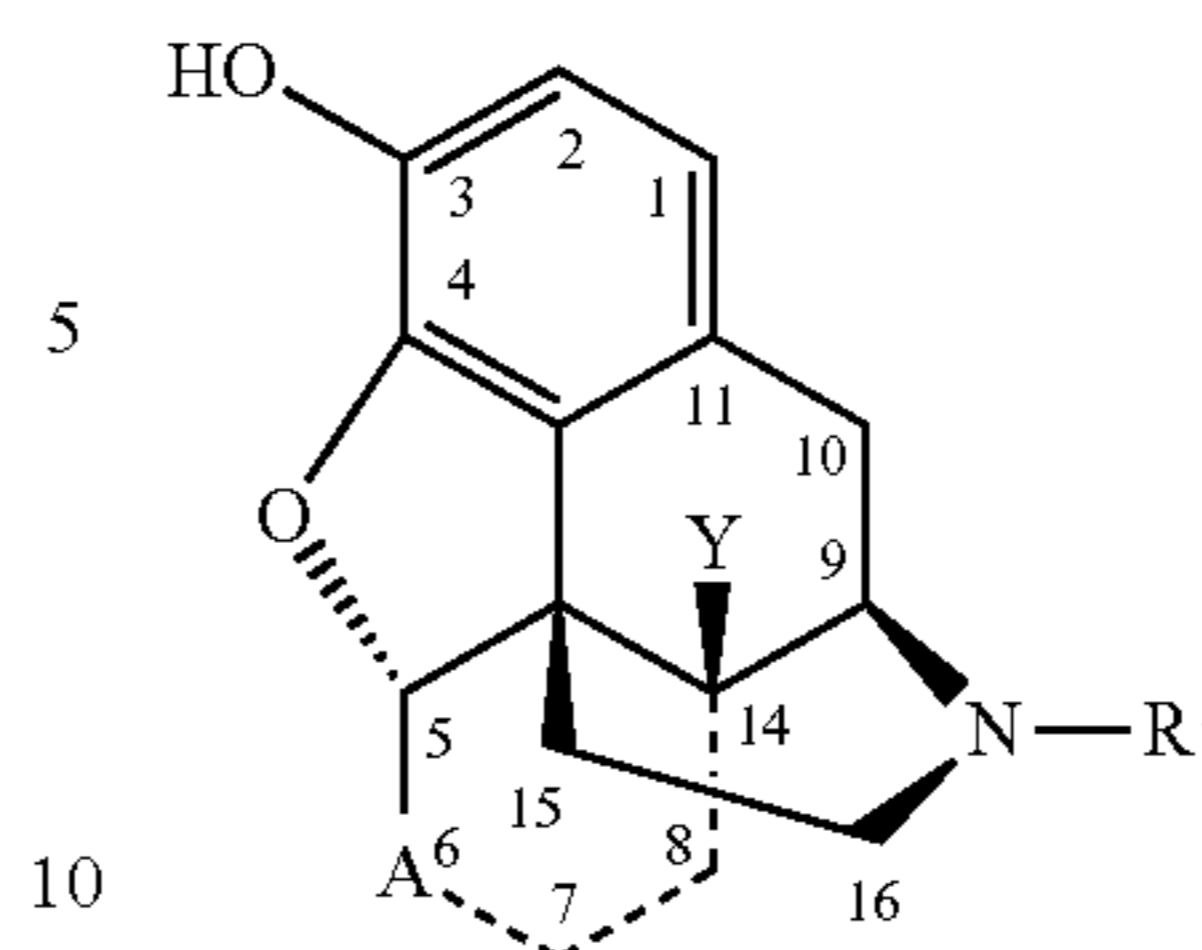
Formula 11
