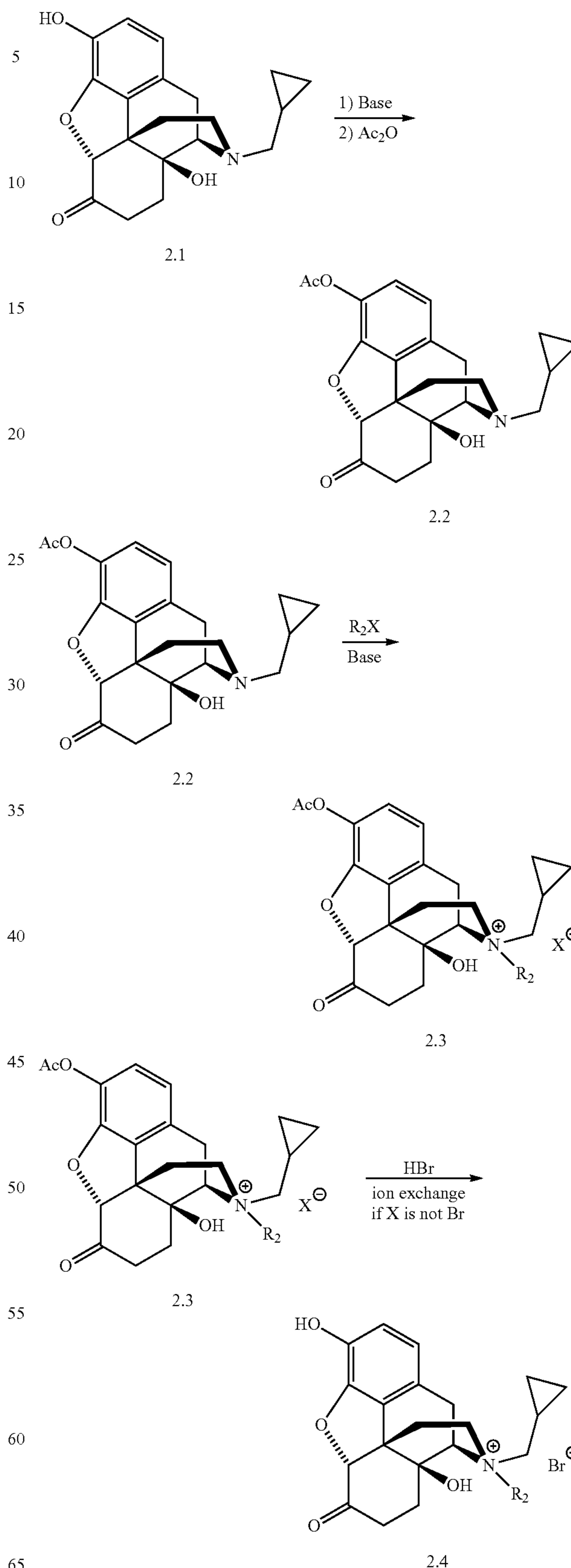
Scheme 2
