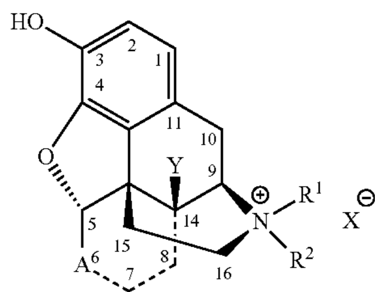
Formula 11A
