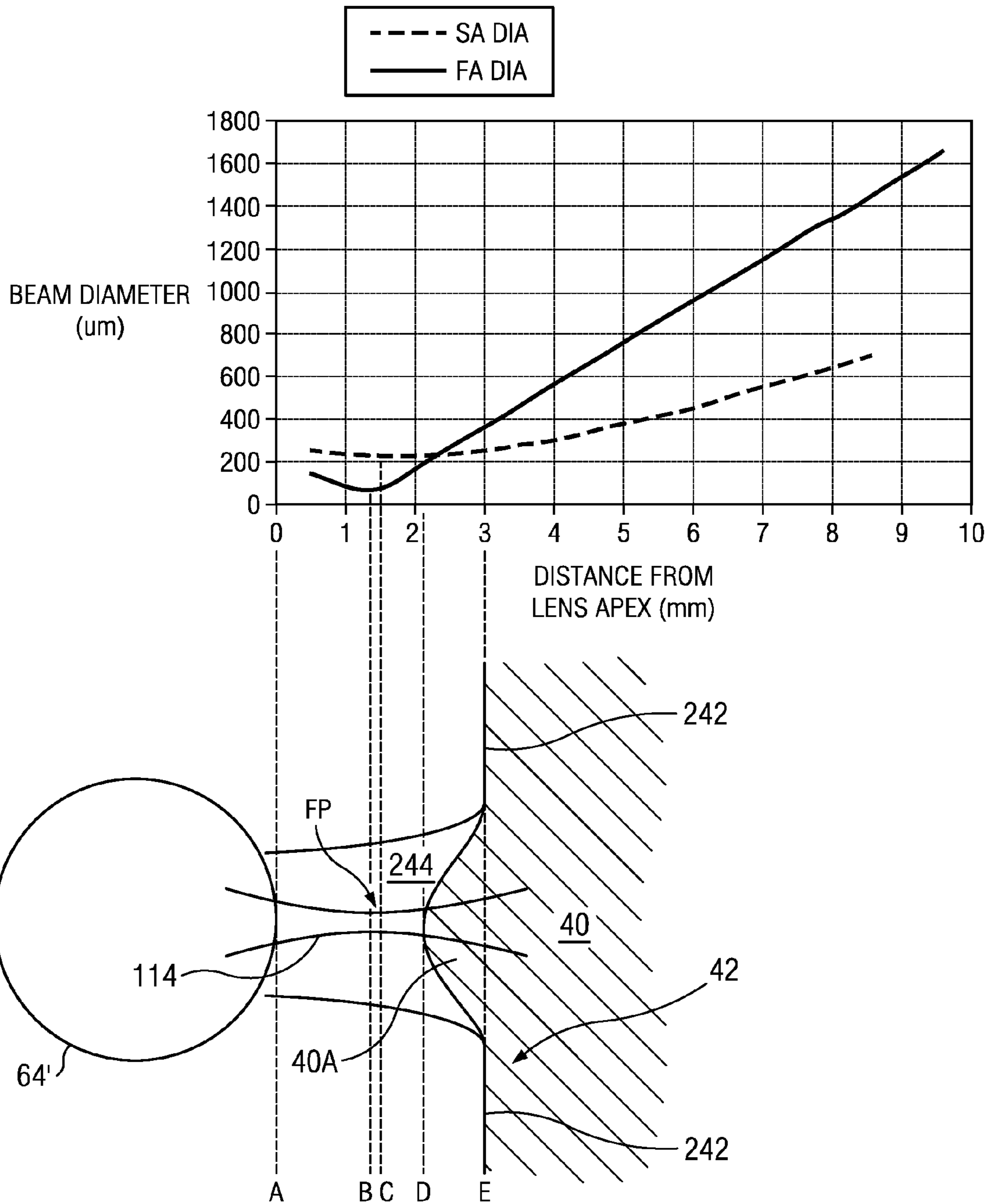
FA AND SA BEAM DIAMETER VS DISTANCE FROM 5mm ROD LENS
