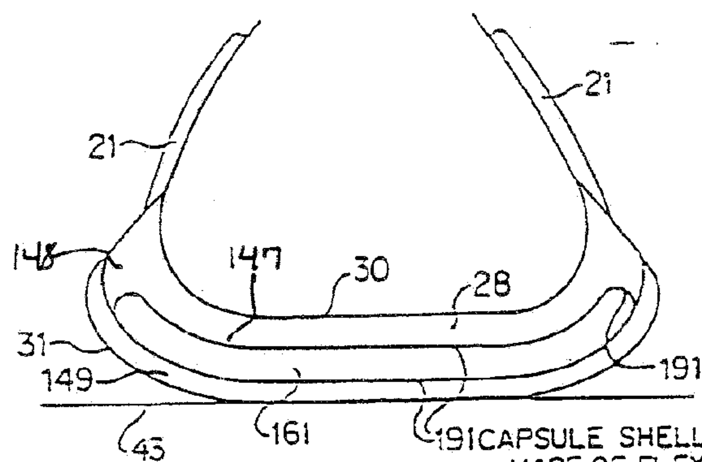
FIG. 59E CAPSULE SHELL MADE OF FLEXIBLE INELASTIC FIBER STRANDS
