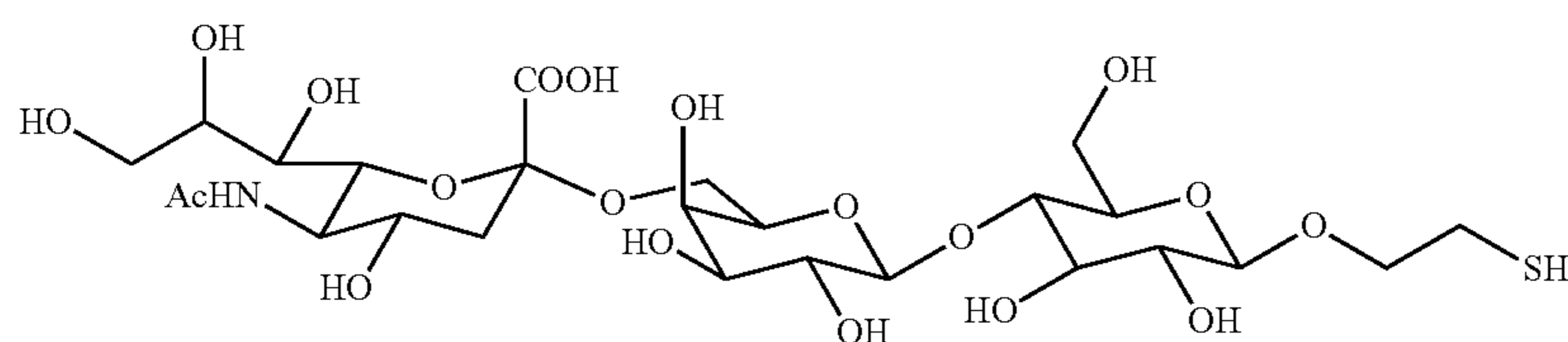
NeuAc \alpha 2,6Gal \beta 1,4Glc \beta
