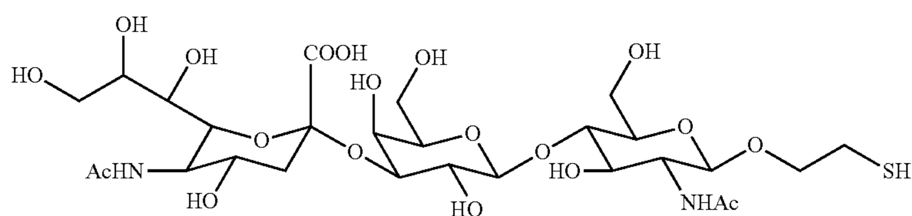
NeuAc \alpha 2,3Gal \beta 1,4GlcNac \beta
