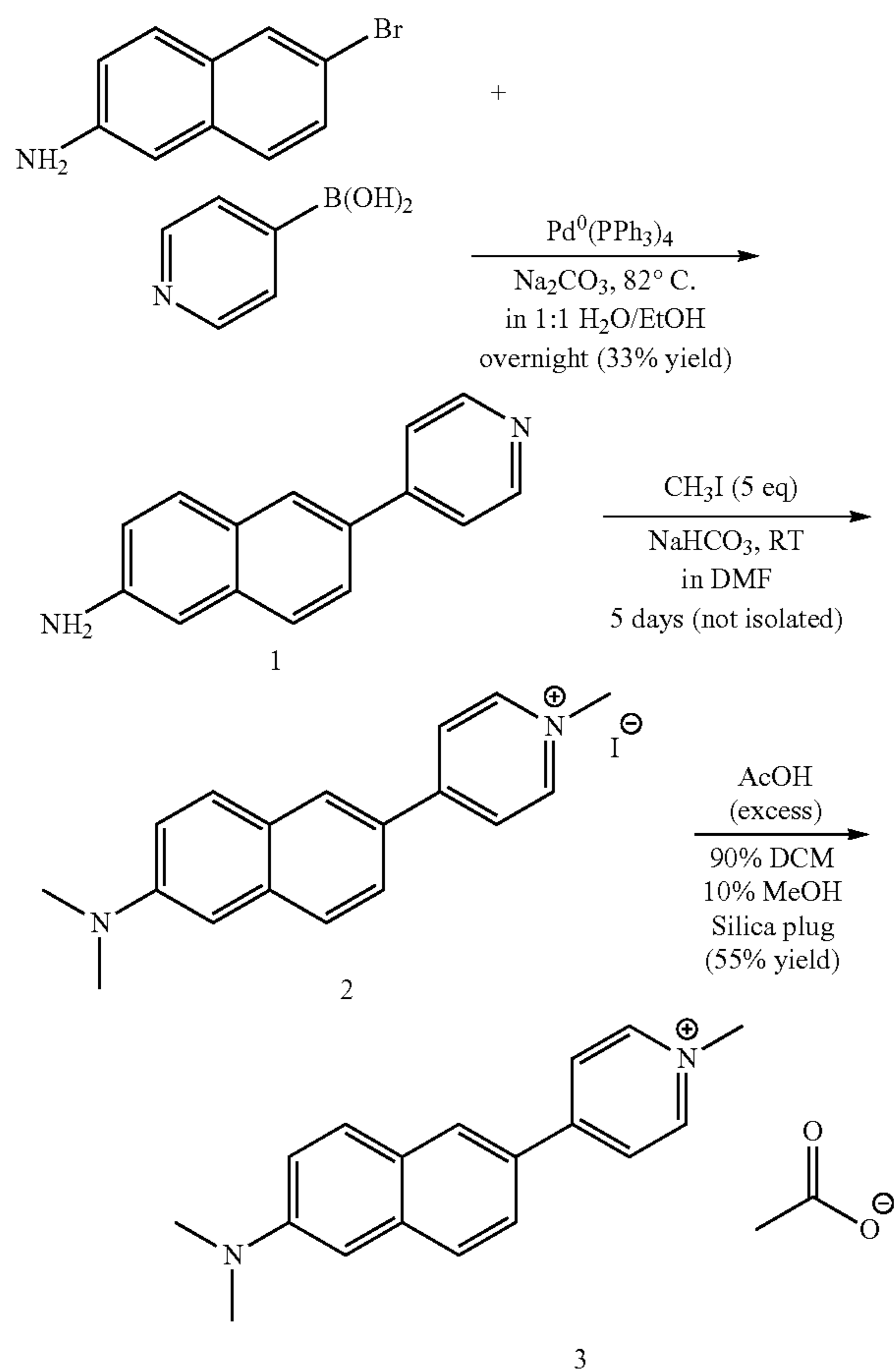
Scheme 4. Example synthesis of fluorescent dye LL-1 (or DANPY-1)
