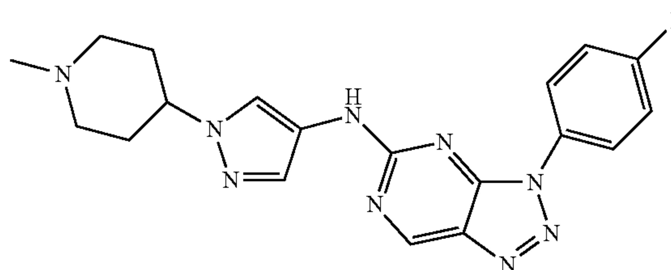
3-(4-fluorophenyl)-N-[1-(1-methyl-4-piperidyl)pyrazol-4-yl]triazolo[4,5-d]pyrimidin-5-amine
