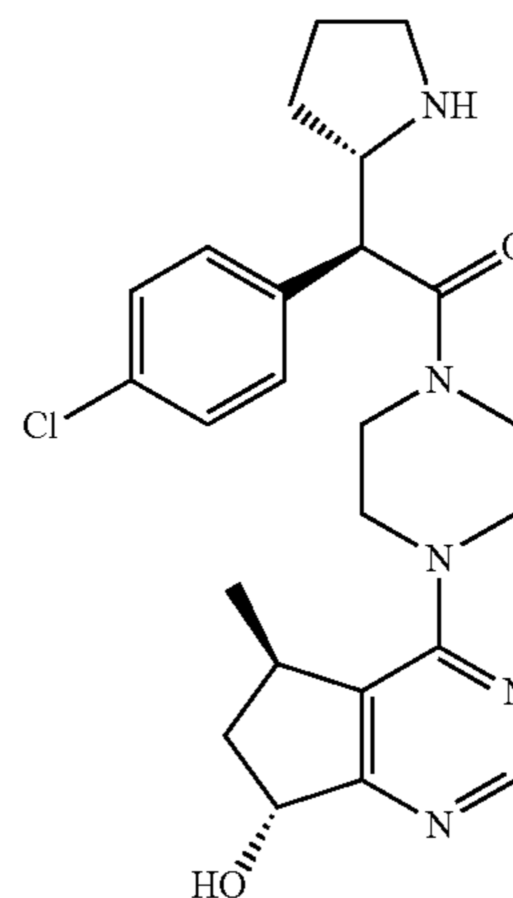
(S)-2-(4-chlorophenyl)-1-(4-((5R,7R)-7-hydroxy-5-methyl-6,7-dihydro-5H-cyclopenta[d]pyrimidin-4-yl)piperazin-1-yl)-2-((S)-pyrrolidin-2-yl)ethanone
