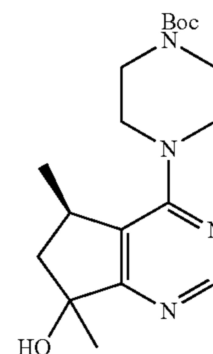
tert-butyl 4-((5R)-7-hydroxy-5,7-dimethyl-6,7-dihydro-5H-cyclopenta[d]pyrimidin-4-yl)piperazine-1-carboxylate
