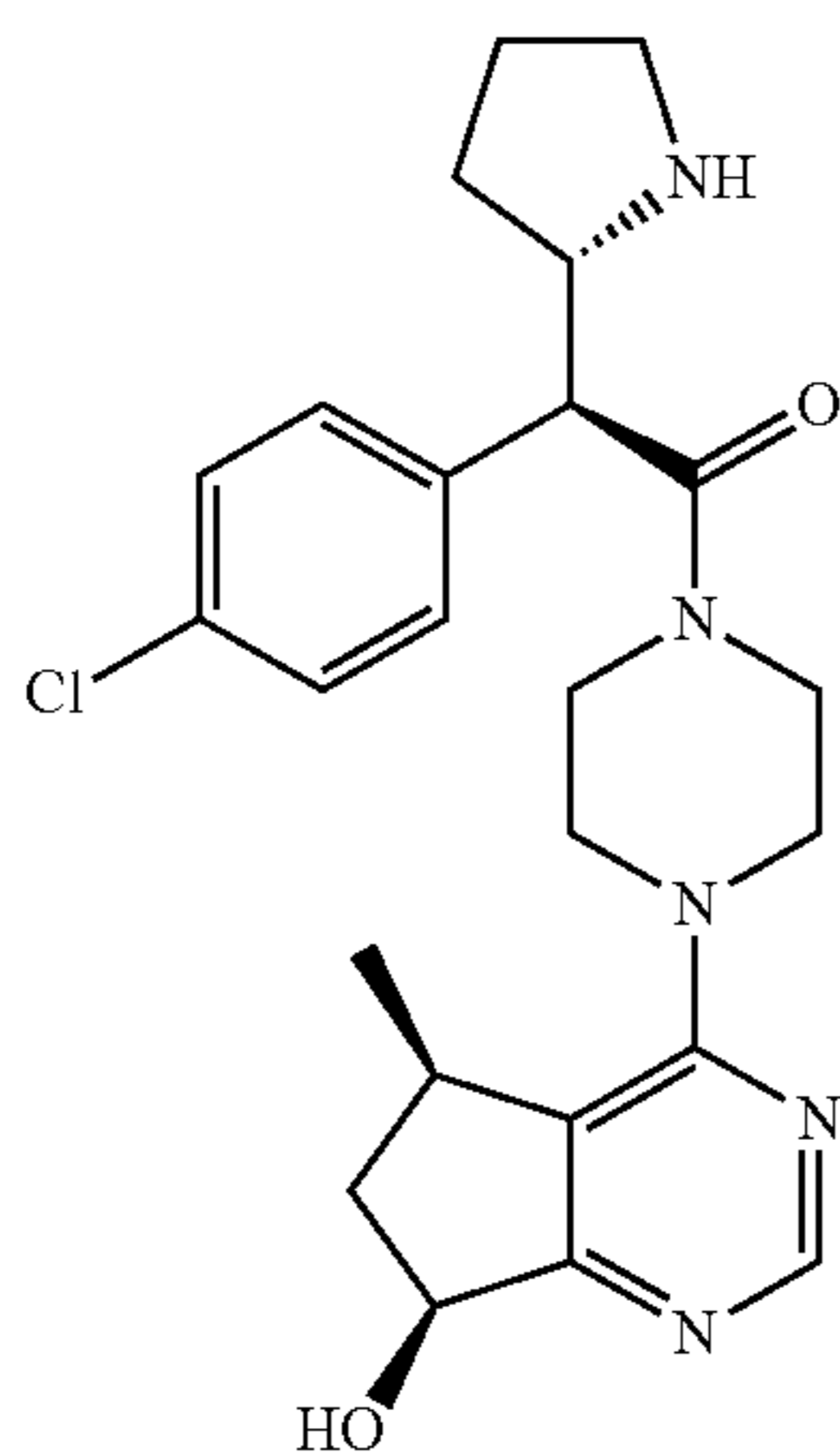
(S)-2-(4-chlorophenyl)-1-(4-((5R,7S)-7-hydroxy-5-methyl-6,7-dihydro-5H-cyclopenta[d]pyrimidin-4-yl)piperazin-1-yl)-2-((S)-pyrrolidin-2-yl)ethanone
