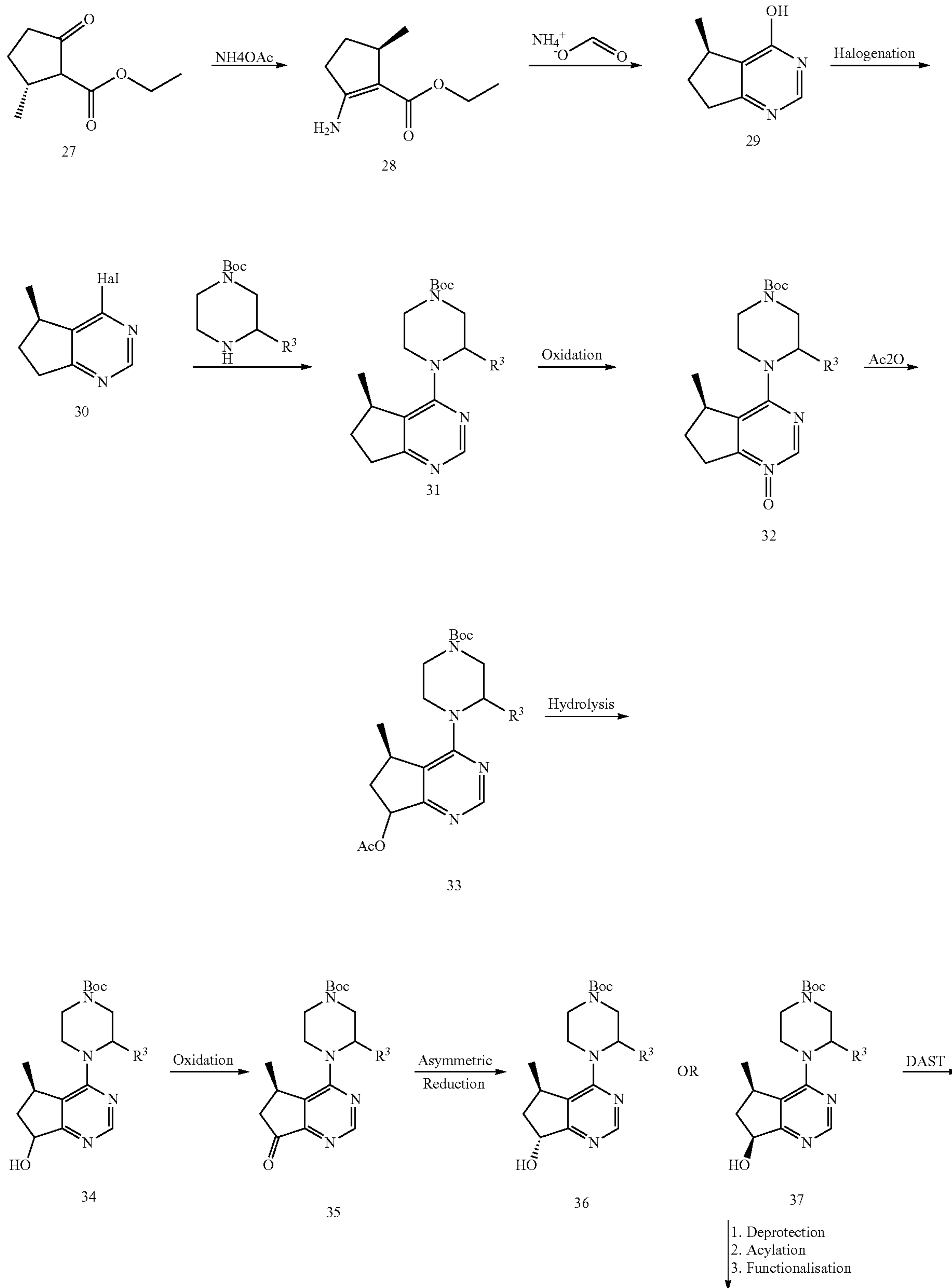
Scheme 4
