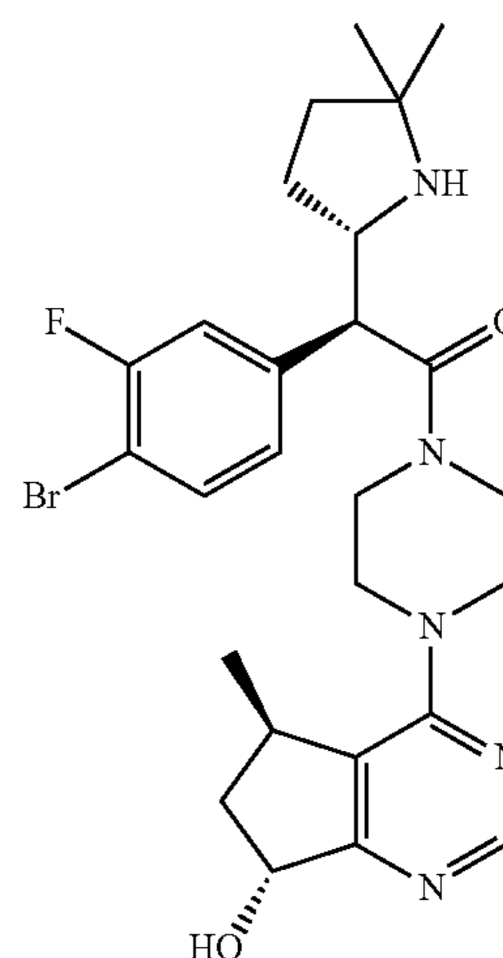
(S)-2-(4-bromo-3-fluorophenyl)-2-((S)-5,5-dimethylpyrrolidin-2-yl)-1-(4-((5R,7R)-7-hydroxy-5-methyl-6,7-dihydro-5H-cyclopenta[d]pyrimidin-4-yl)piperazin-1-yl)ethanone
