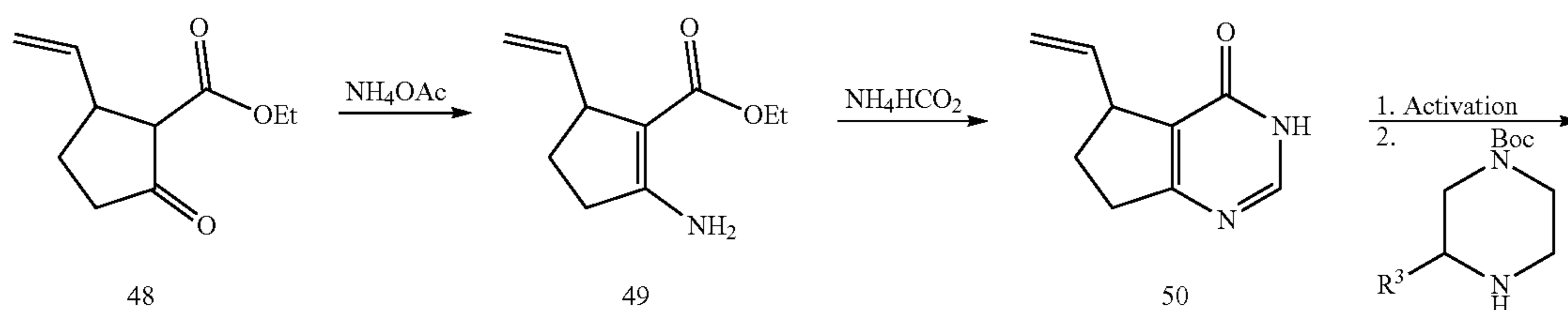
Scheme 6
