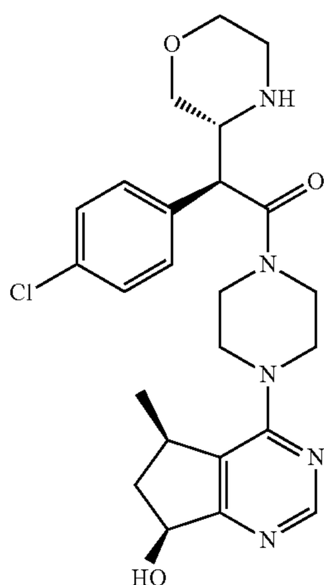
(S)-2-(4-chlorophenyl)-1-(4-((5R,7S)-7-hydroxy-5-methyl-6,7-dihydro-5H-cyclopenta[d]pyrimidin-4-yl)piperazin-1-yl)-2-((R)-morpholin-3-yl)ethanone
