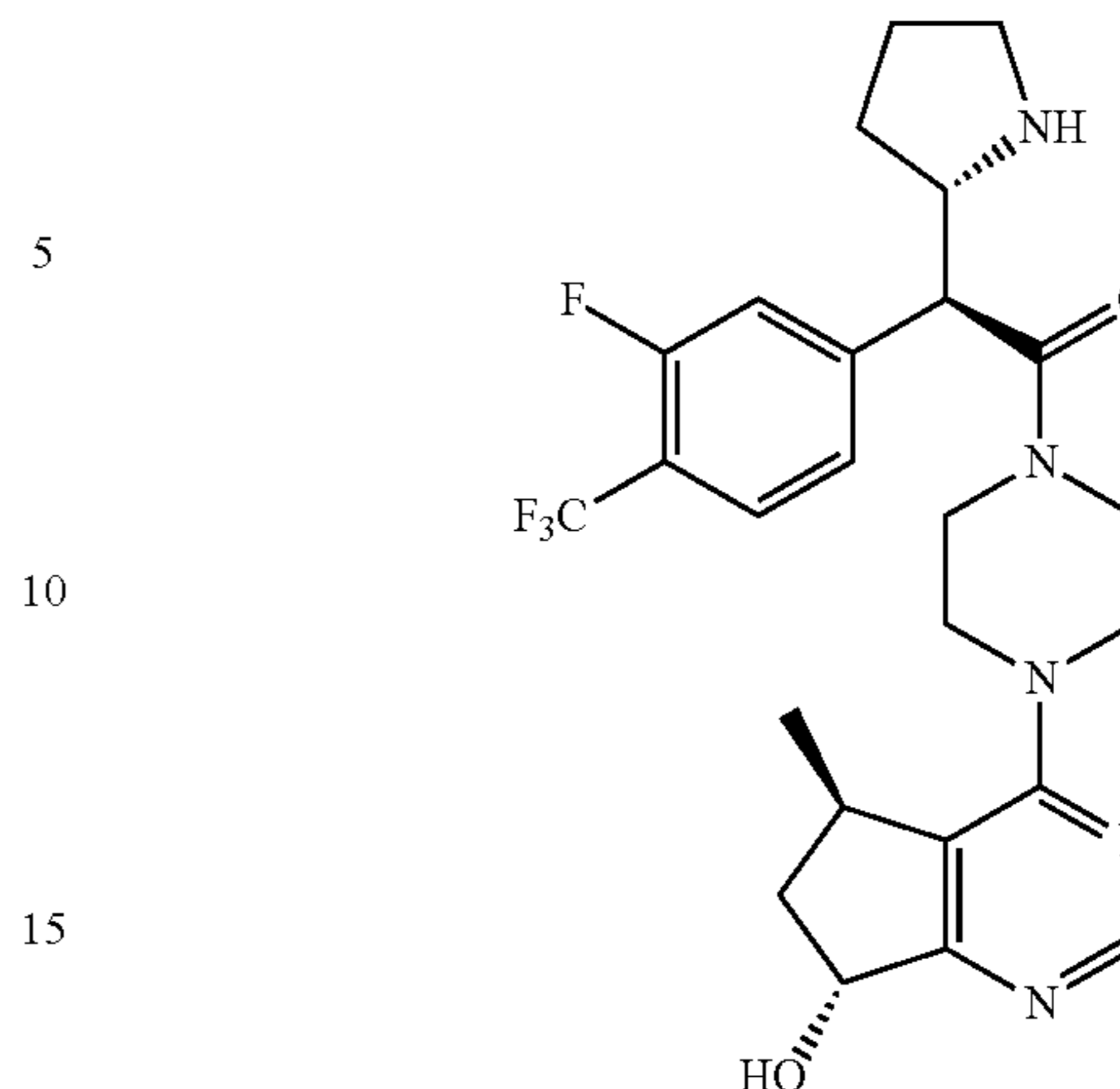
(S)-2-(3-fluoro-4-(trifluoromethyl)phenyl)-1-(4-((5R,7R)-7-hydroxy-5-methyl-6,7-dihydro-5H-cyclopenta[d]pyrimidin-4-yl)piperazin-1-yl)-2-((S)-pyrrolidin-2-yl)ethanone
