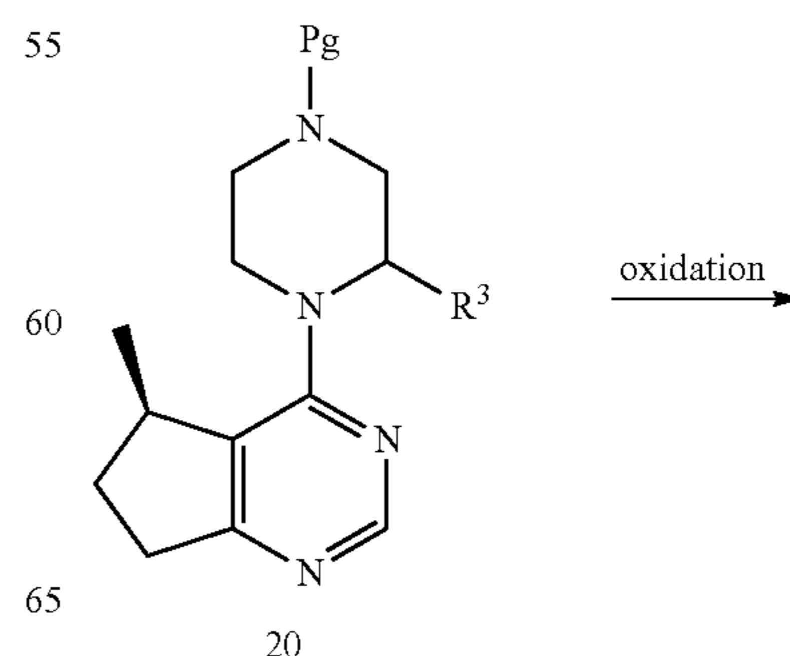
Scheme 3
