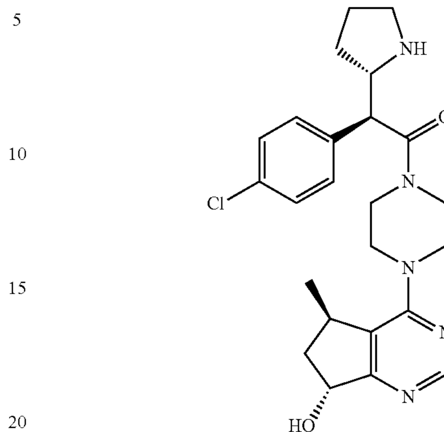
(S)-2-(4-chlorophenyl)-1-(4-((5R,7R)-7-hydroxy-5-methyl-6,7-dihydro-5H-cyclopenta[d]pyrimidin-4-yl)piperazin-1-yl)-2-((S)-pyrrolidin-2-yl)ethanone
