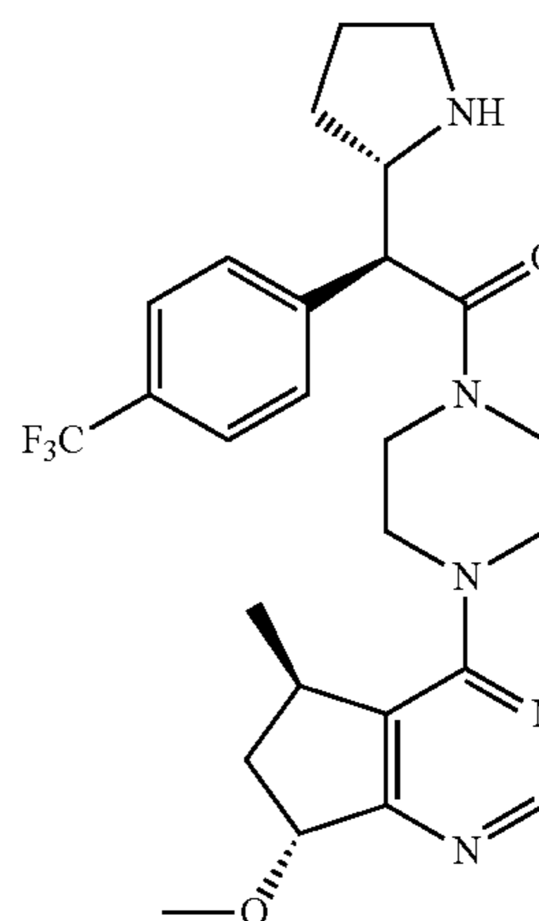
(S)-1-(4-((5R,7R)-7-methoxy-5-methyl-6,7-dihydro-5H-cyclopenta[d]pyrimidin-4-yl)piperazin-1-yl)-2-((S)-pyrrolidin-2-yl)-2-(4-(trifluoromethyl)phenyl)ethanone
