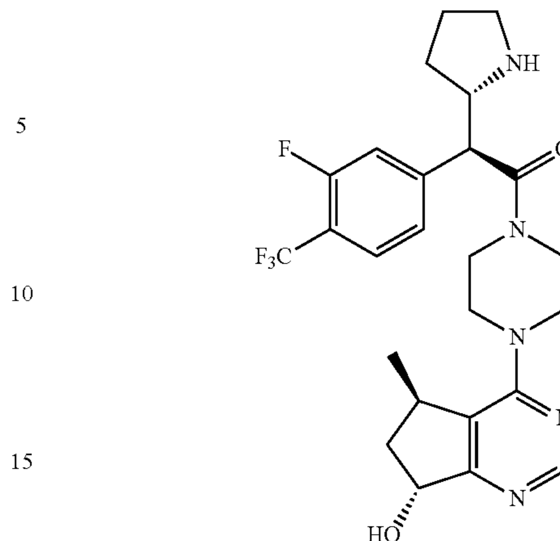
(S)-2-(3-fluoro-4-(trifluoromethyl)phenyl)-1-(4-((5R,7R)-7-hydroxy-5-methyl-6,7-dihydro-5H-cyclopenta[d]pyrimidin-4-yl)piperazin-1-yl)-2-((S)-pyrrolidin-2-yl)ethanone
