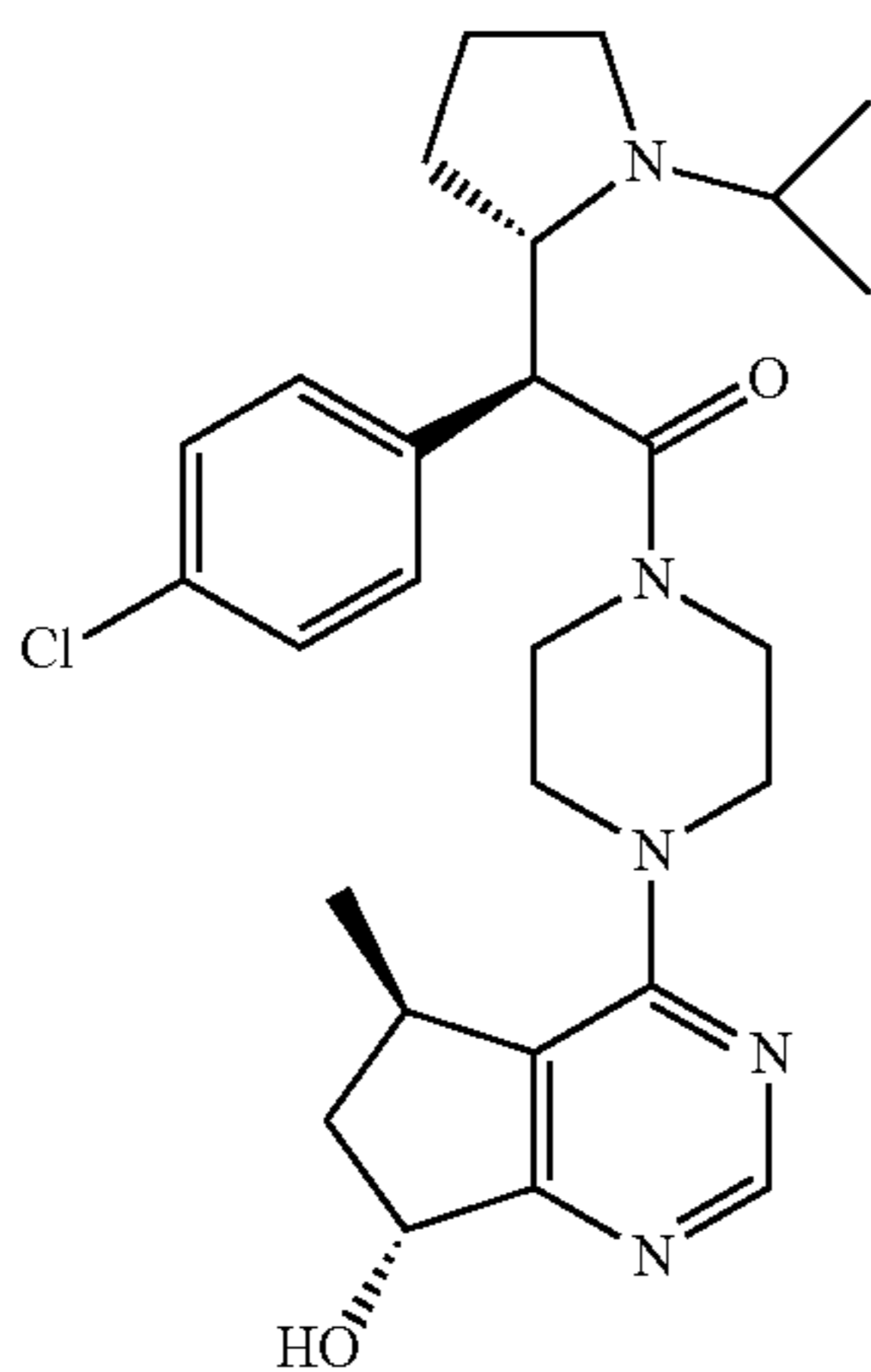
(S)-2-(4-chlorophenyl)-1-(4-((5R,7R)-7-hydroxy-5-methyl-6,7-dihydro-5H-cyclopenta[d]pyrimidin-4-yl)piperazin-1-yl)-2-((S)-1-isopropylpyrrolidin-2-yl)ethanone
