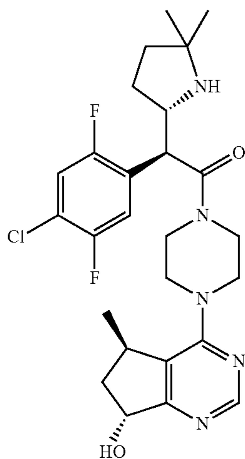
(S)-2-(4-chloro-2,5-difluorophenyl)-2-((S)-5,5-dimethylpyrrolidin-2-yl)-1-(4-((5R,7R)-7-hydroxy-5-methyl-6,7-dihydro-5H-cyclopenta[d]pyrimidin-4-yl)piperazin-1-yl)ethanone
