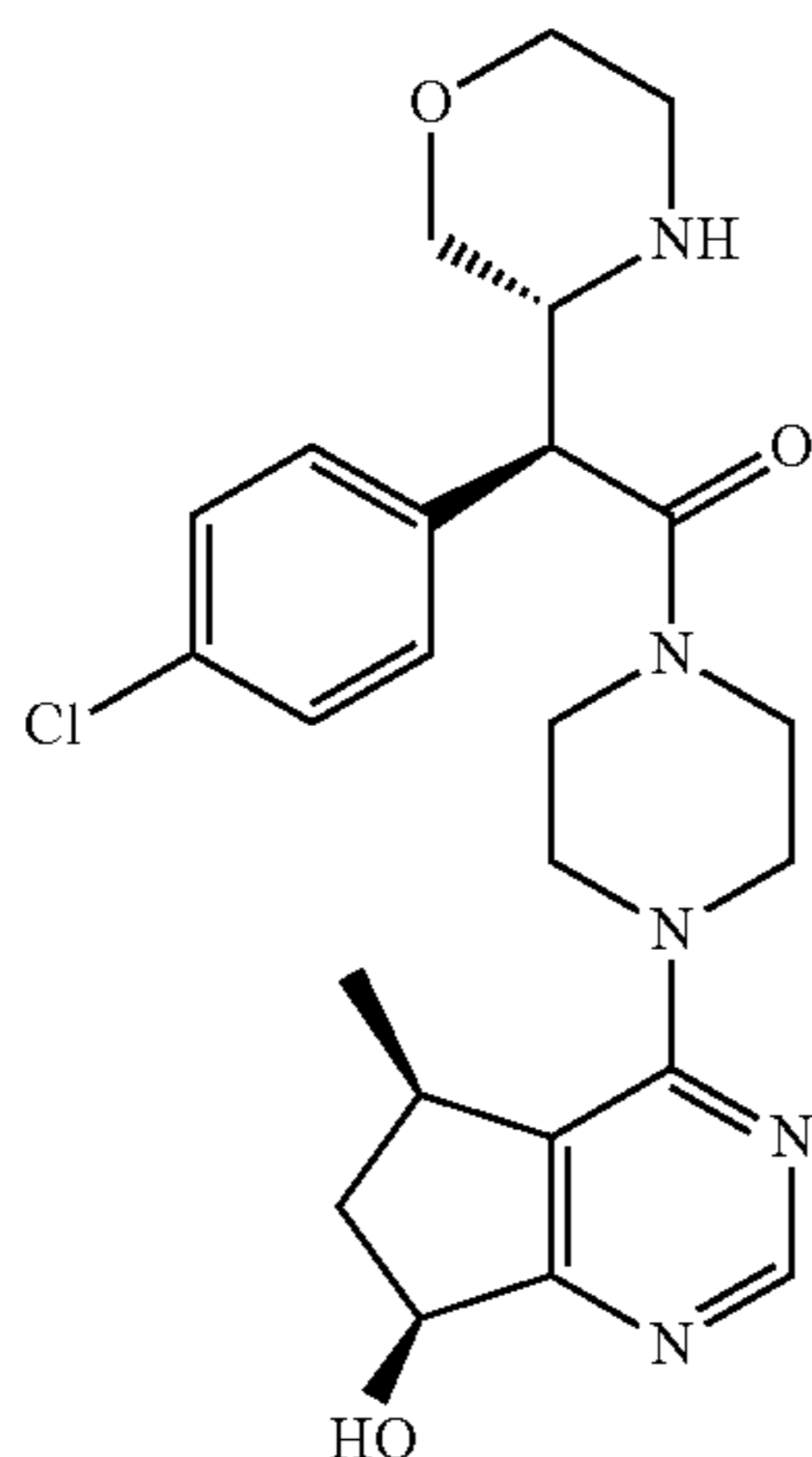
(S)-2-(4-chlorophenyl)-1-(4-((5R,7S)-7-hydroxy-5-methyl-6,7-dihydro-5H-cyclopenta[d]pyrimidin-4-yl)piperazin-1-yl)-2-((R)-morpholin-3-yl)ethanone
