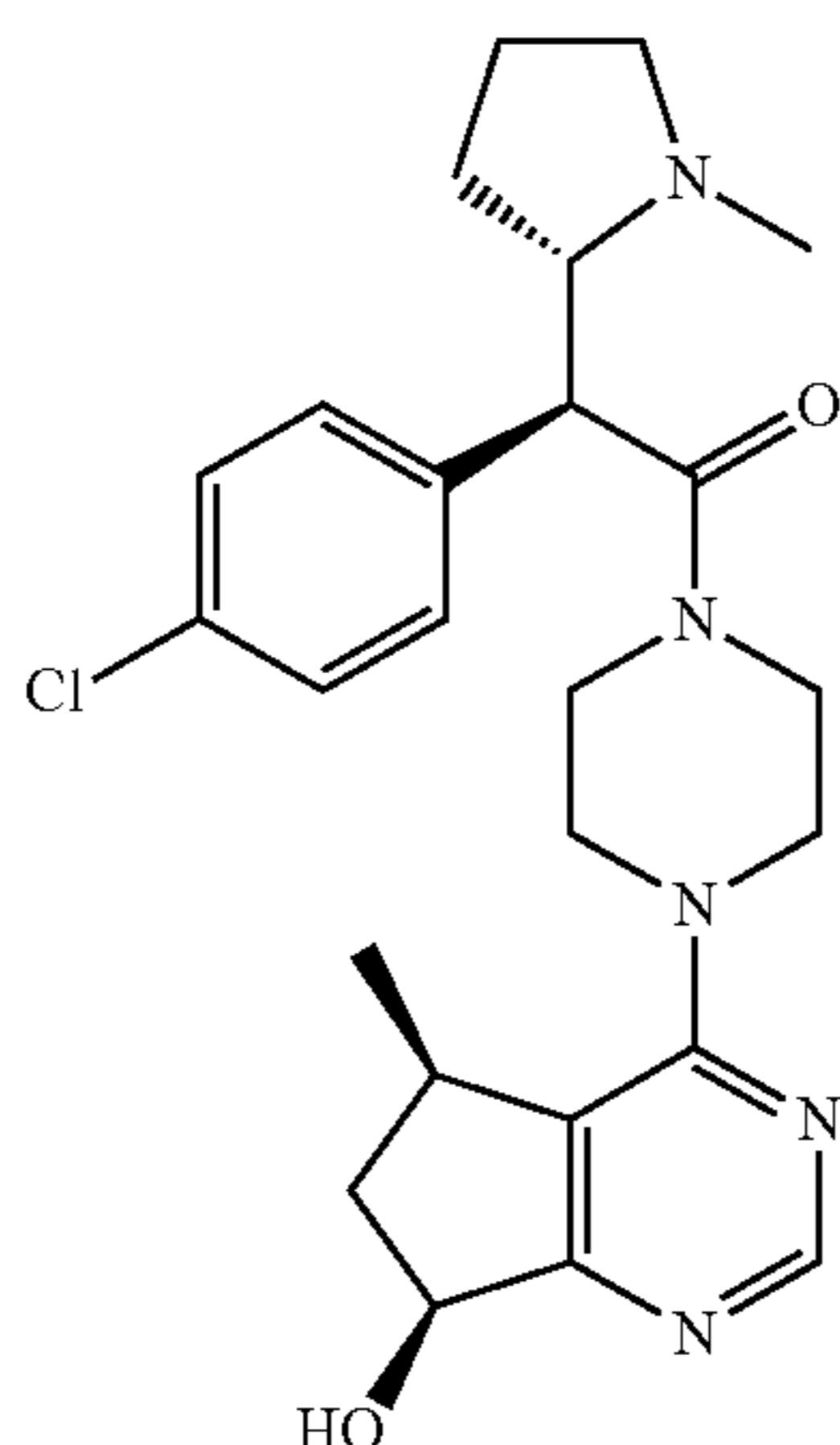
(S)-2-(4-chlorophenyl)-1-(4-((5R,7S)-7-hydroxy-5-methyl-6,7-dihydro-5H-cyclopenta[d]pyrimidin-4-yl)piperazin-1-yl)-2-((S)-1-methylpyrrolidin-2-yl)ethanone
