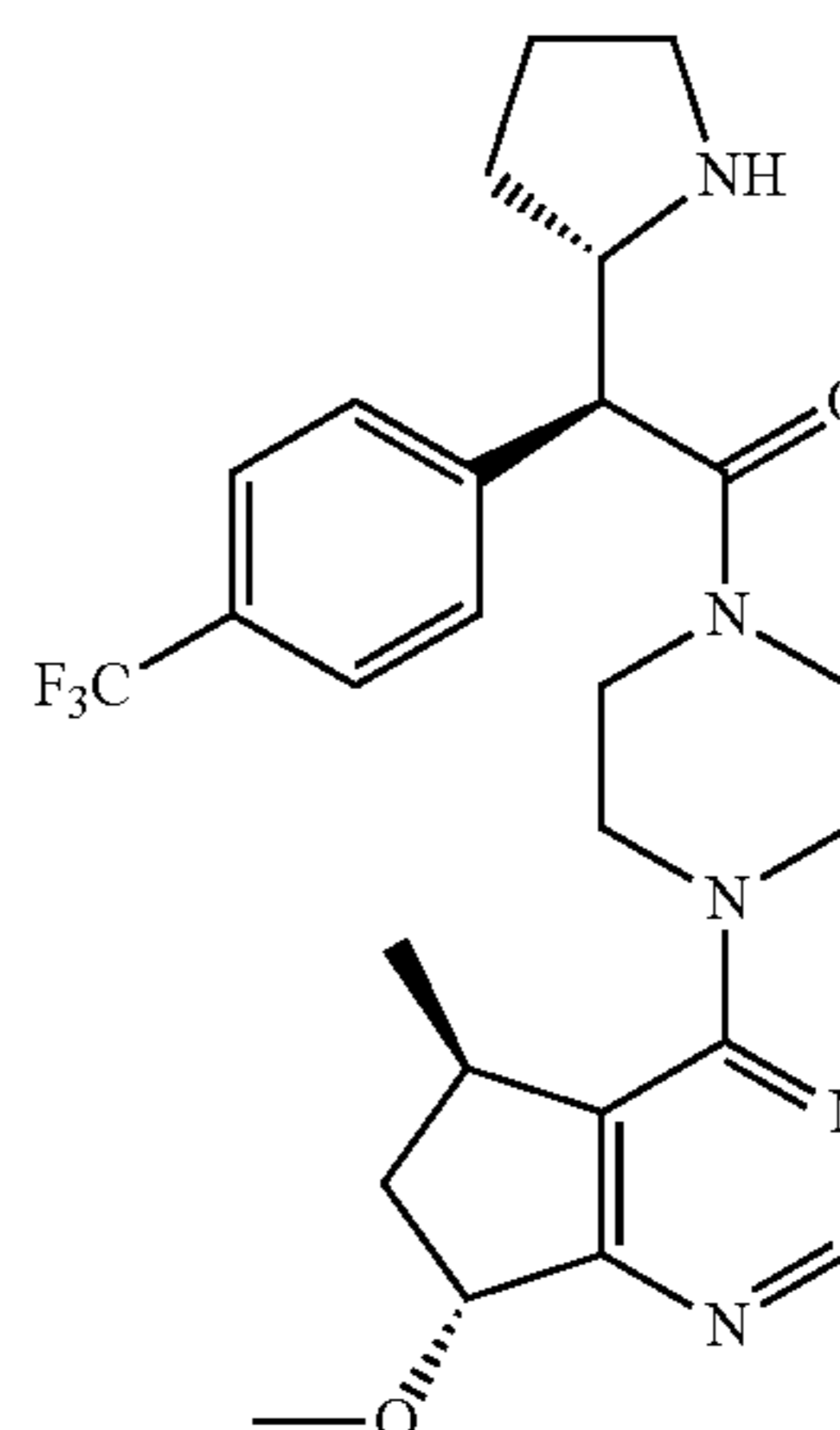
(S)-1-(4-((5R,7R)-7-methoxy-5-methyl-6,7-dihydro-5H-cyclopenta[d]pyrimidin-4-yl)piperazin-1-yl)-2-((S)-pyrrolidin-2-yl)-2-(4-(trifluoromethyl)phenyl)ethanone
