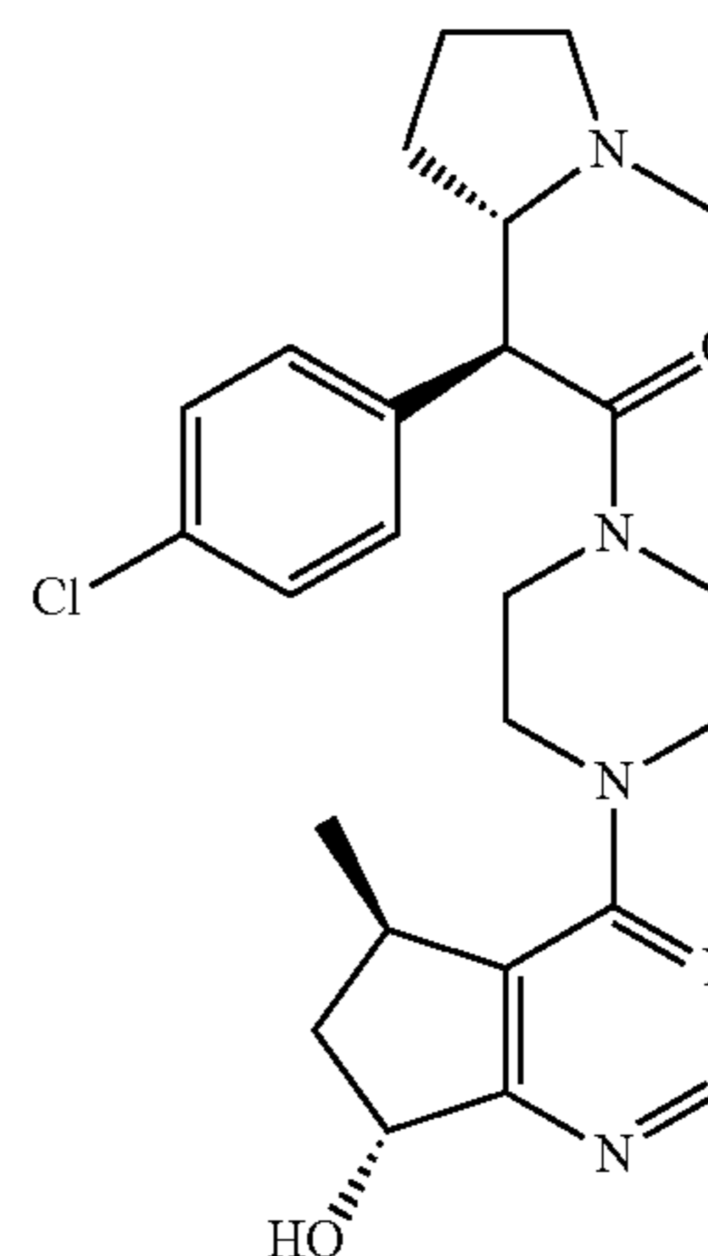
(S)-2-(4-chlorophenyl)-1-(4-((5R,7R)-7-hydroxy-5-methyl-6,7-dihydro-5H-cyclopenta[d]pyrimidin-4-yl)piperazin-1-yl)-2-((S)-1-methylpyrrolidin-2-yl)ethanone
