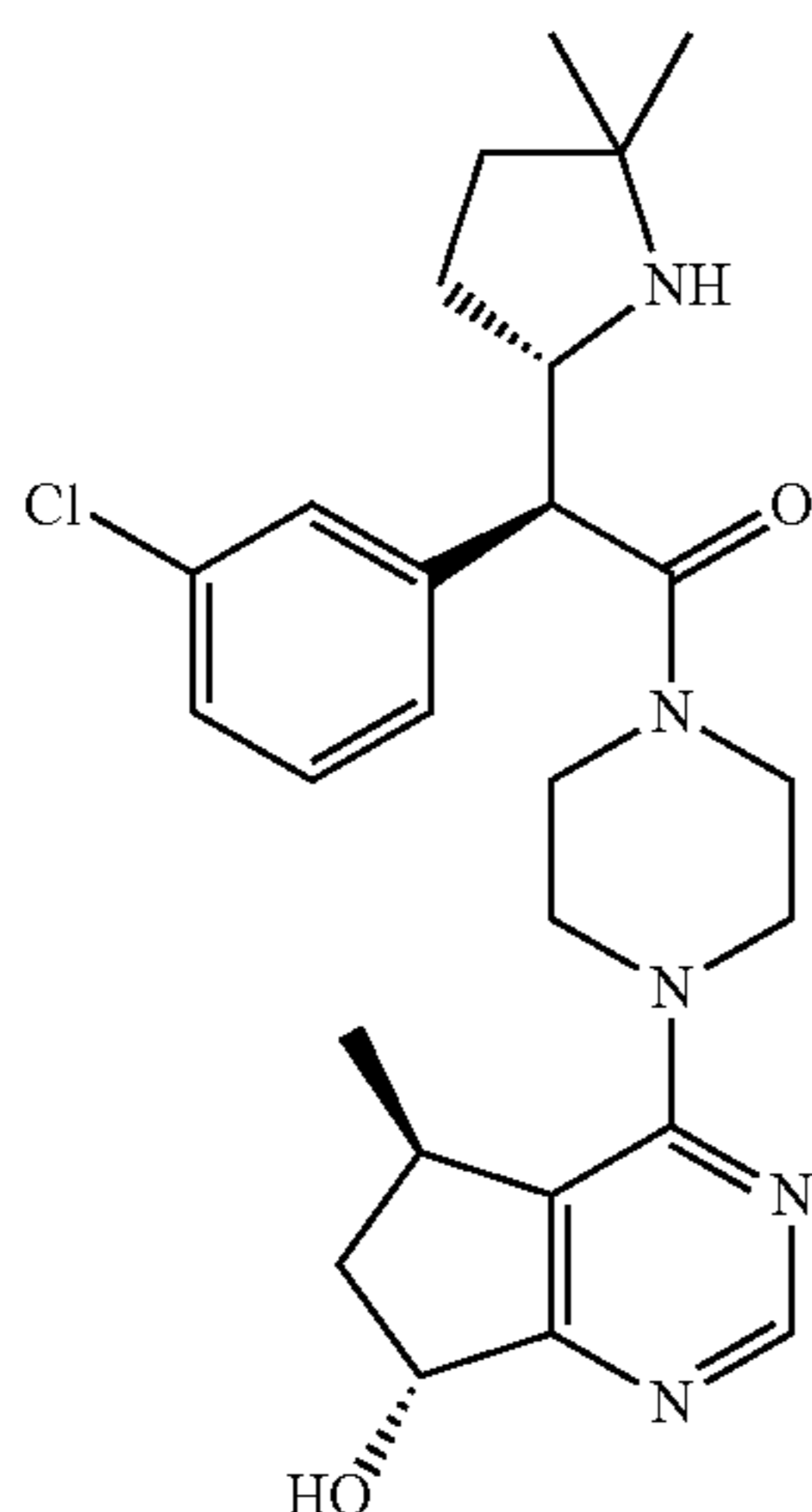
(S)-2-(3-chlorophenyl)-2-((S)-5,5-dimethylpyrrolidin-2-yl)-1-(4-((5R,7R)-7-hydroxy-5-methyl-6,7-dihydro-5H-cyclopenta[d]pyrimidin-4-yl)piperazin-1-yl)ethanone
