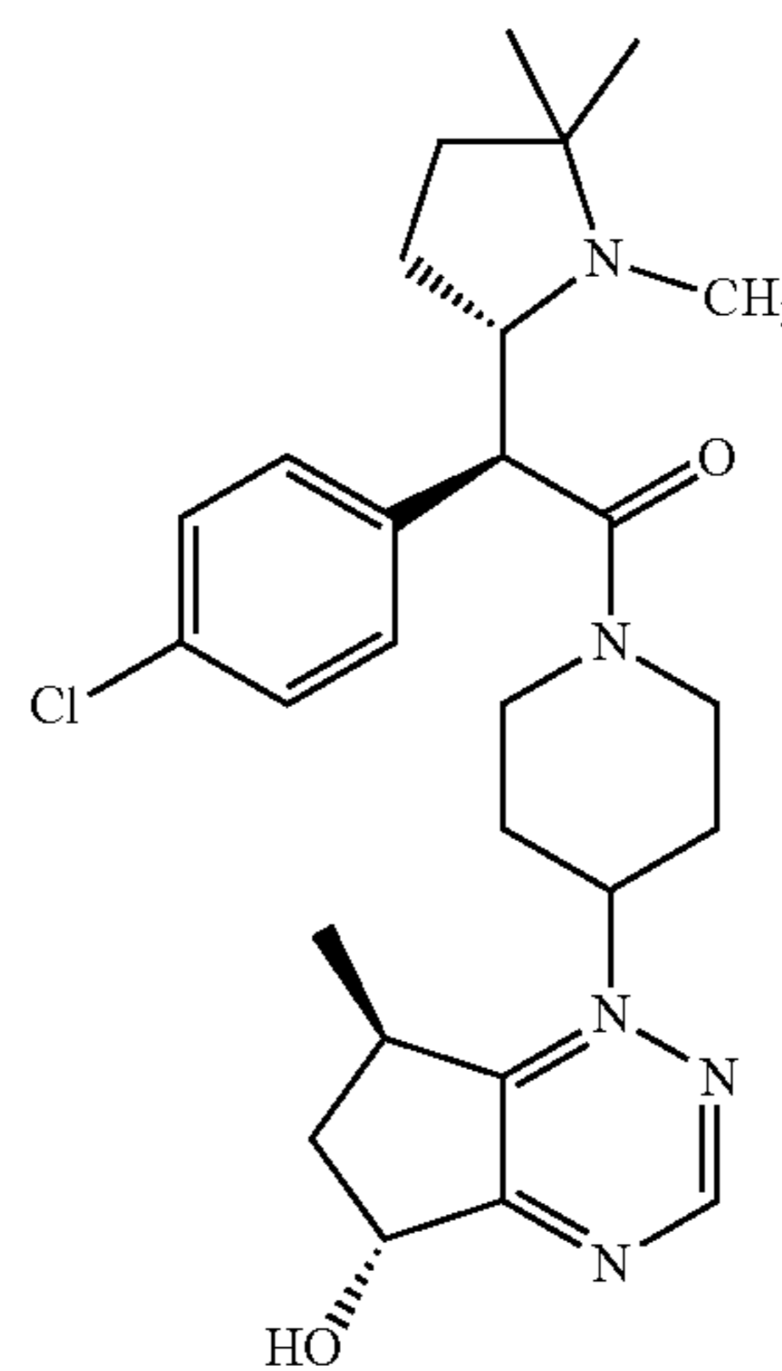
(S)-2-(4-chlorophenyl)-1-(4-((5R,7R)-7-hydroxy-5-methyl-6,7-dihydro-5H-cyclopenta[d]pyrimidin-4-yl)piperazin-1-yl)-2-((S)-1,5,5-trimethylpyrrolidin-2-yl)ethanone
