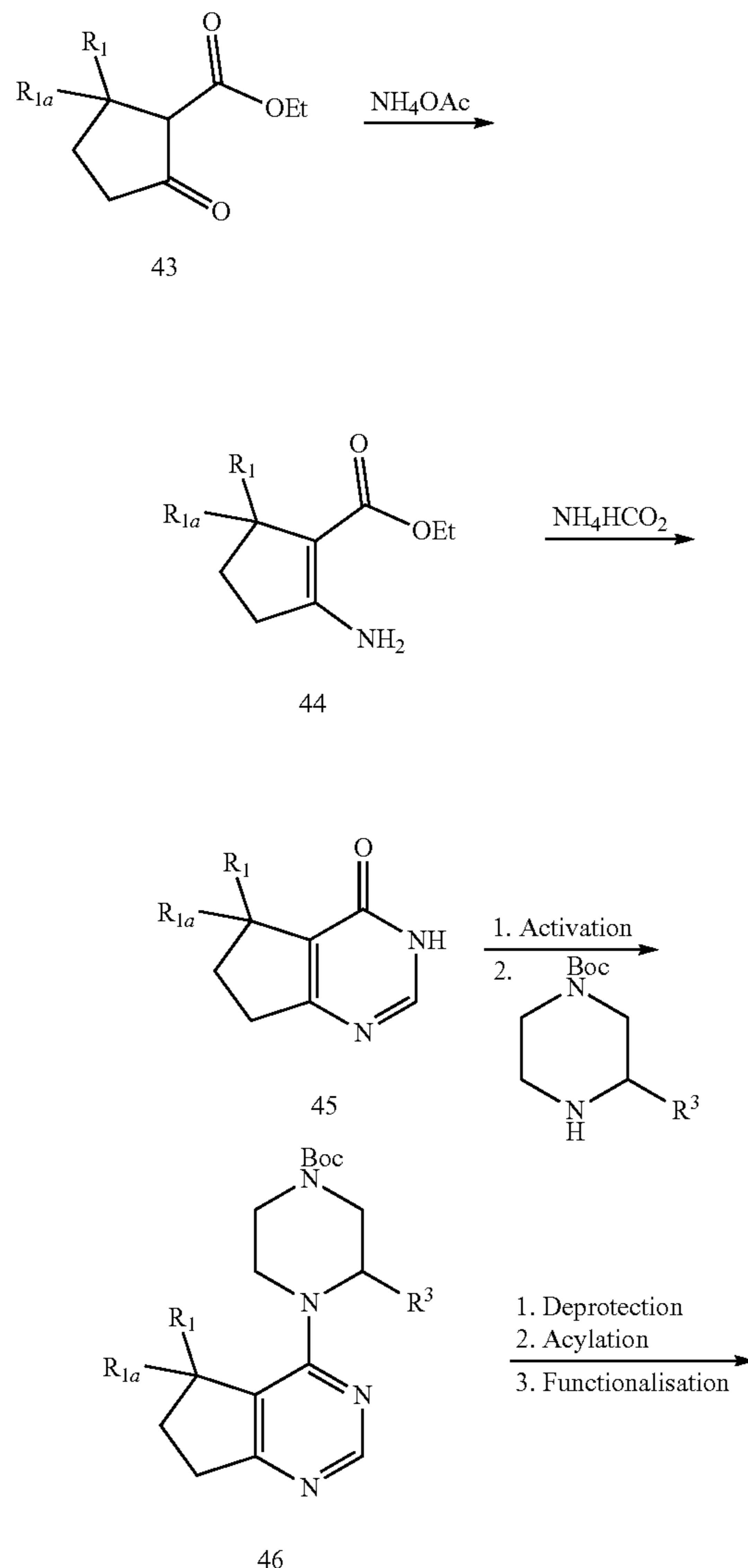
Scheme 5
