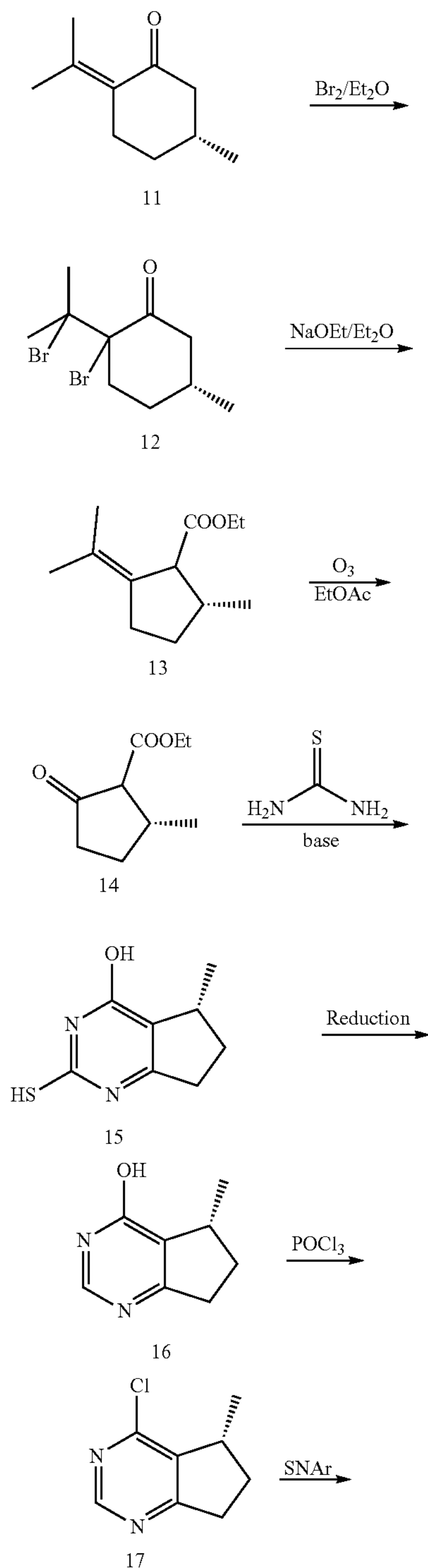
Scheme 2
