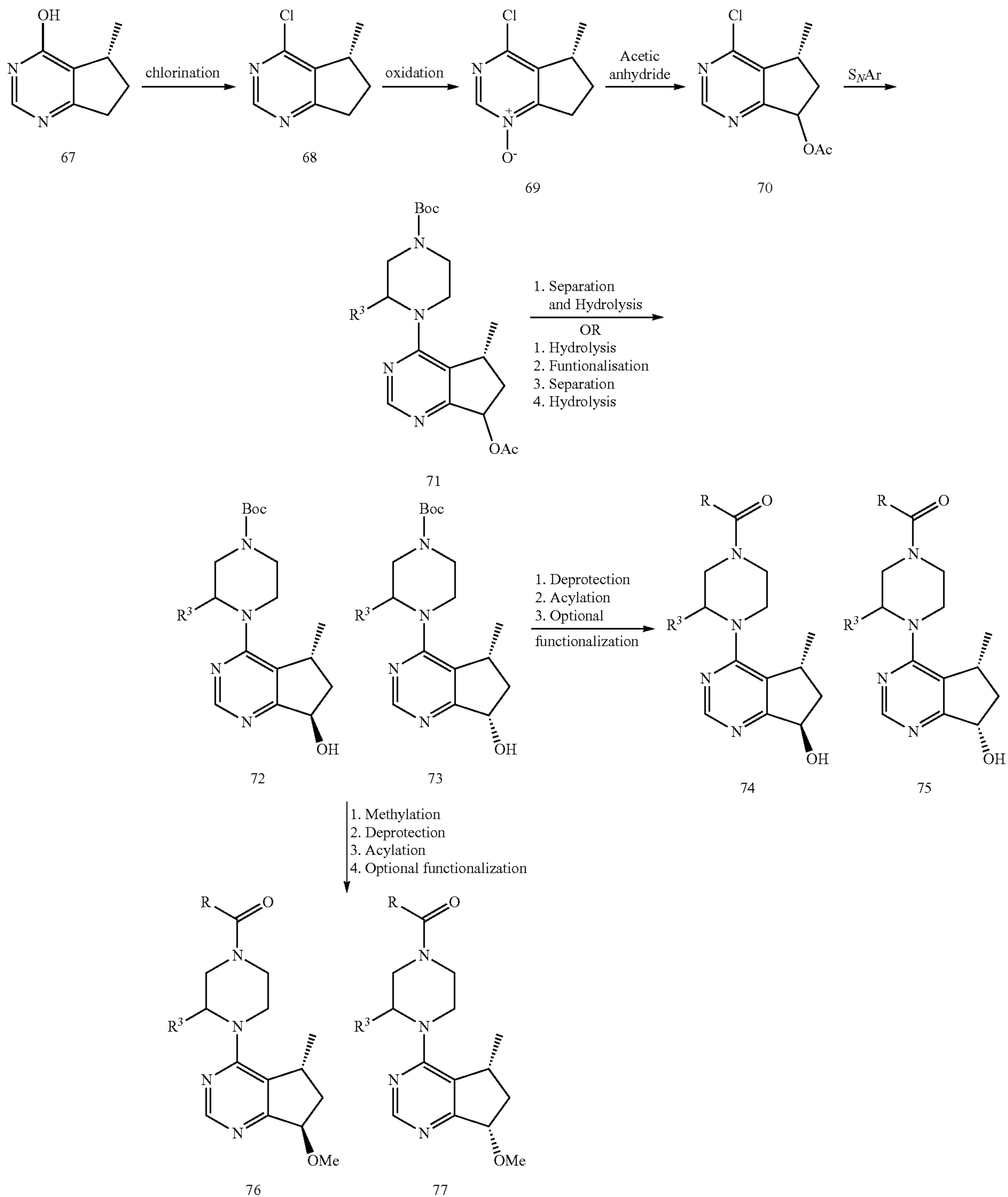
Scheme 8
