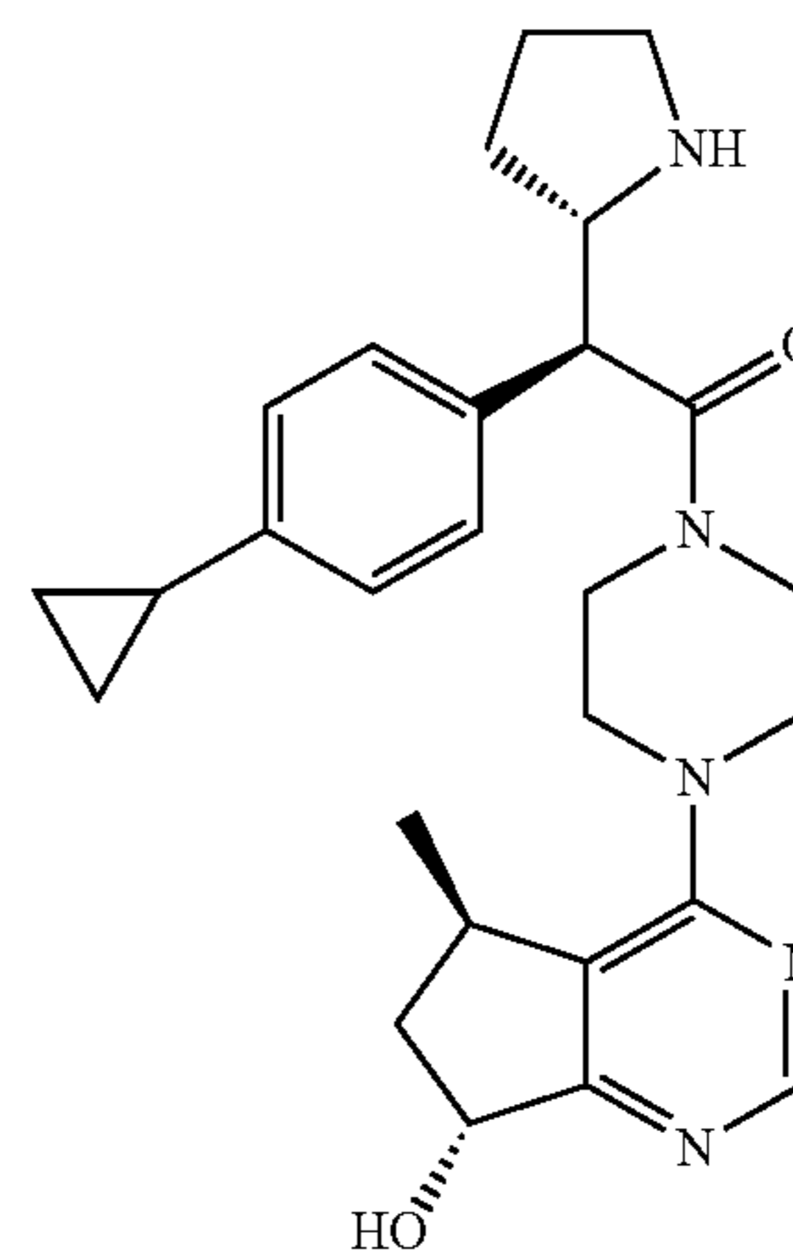
(S)-2-(4-cyclopropylphenyl)-1-(4-((5R,7R)-7-hydroxy-5-methyl-6,7-dihydro-5H-cyclopenta[d]pyrimidin-4-yl)piperazin-1-yl)-2-((S)-pyrrolidin-2-yl)ethanone
