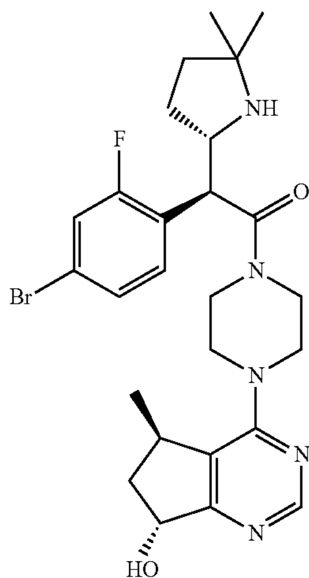
(S)-2-(4-bromo-2-fluorophenyl)-2-((S)-5,5-dimethylpyrrolidin-2-yl)-1-(4-((5R,7R)-7-hydroxy-5-methyl-6,7-dihydro-5H-cyclopenta[d]pyrimidin-4-yl)piperazin-1-yl)ethanone
