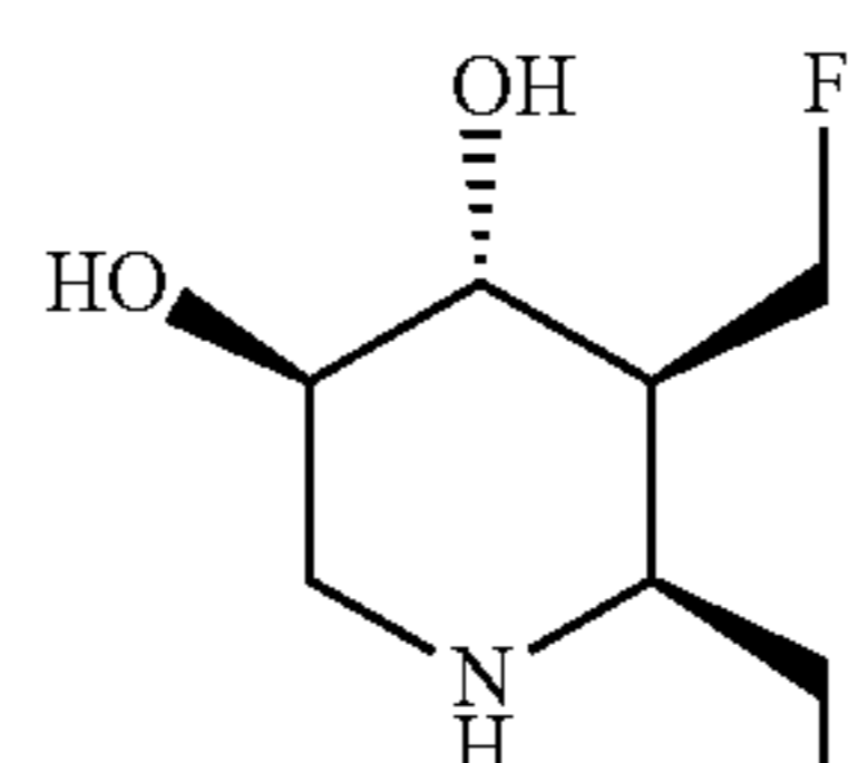
(3R,4R,5S,6R)-6-ethyl-5-(fluoromethyl)piperidine-3,4-diol
