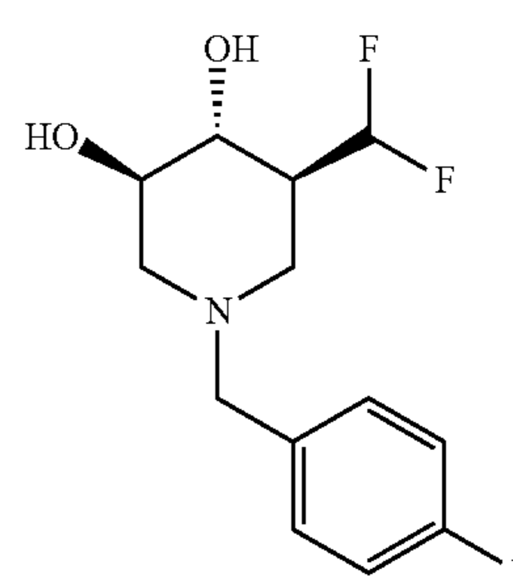
(3R,4R,5S)-5-(difluoromethyl)-1-(4-fluorobenzyl)piperidine-3,4-diol
