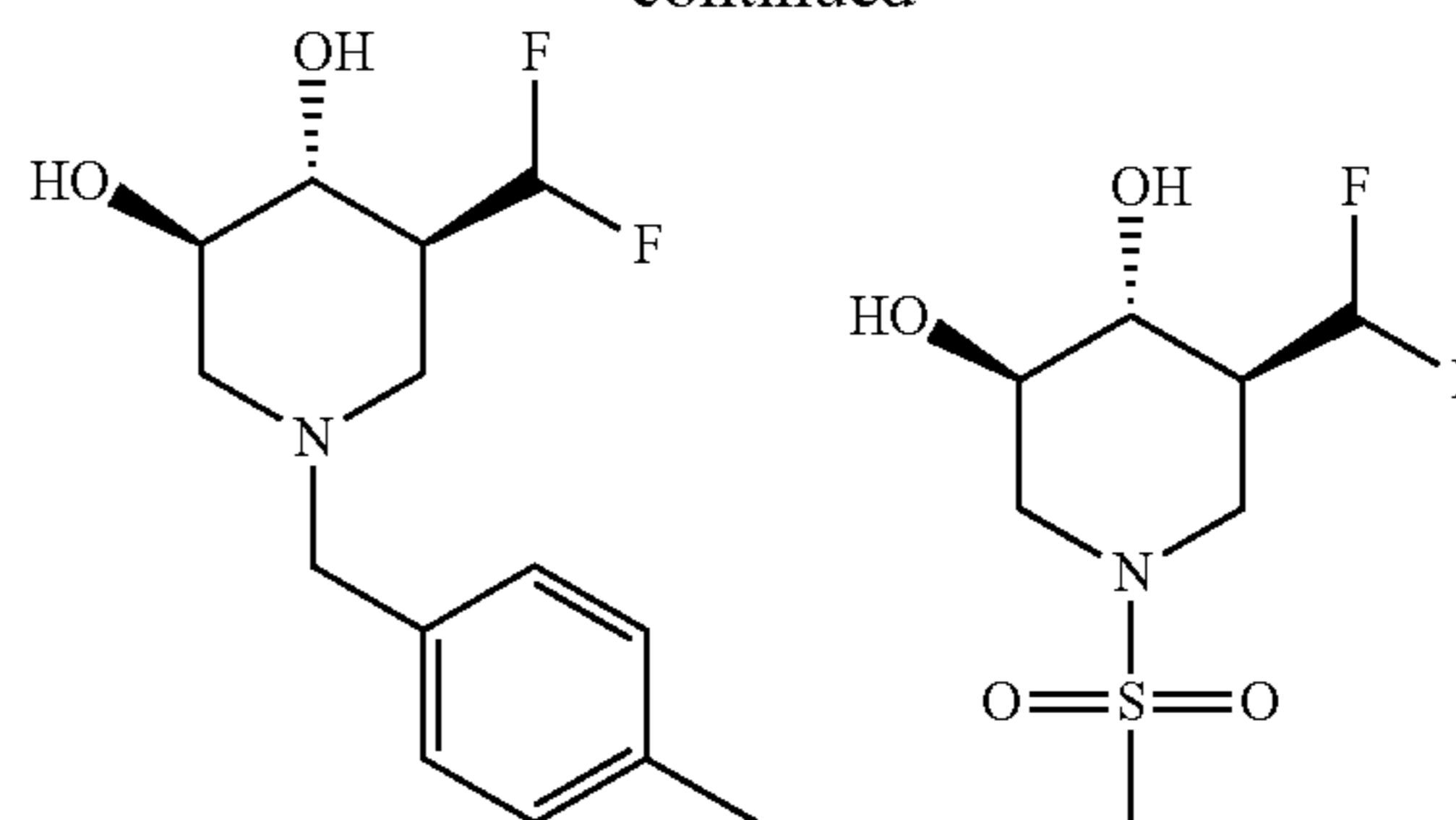
(3R,4R,5S)-5-(difluoromethyl)-1-(4-methylbenzyl)piperidine-3,4-diol
