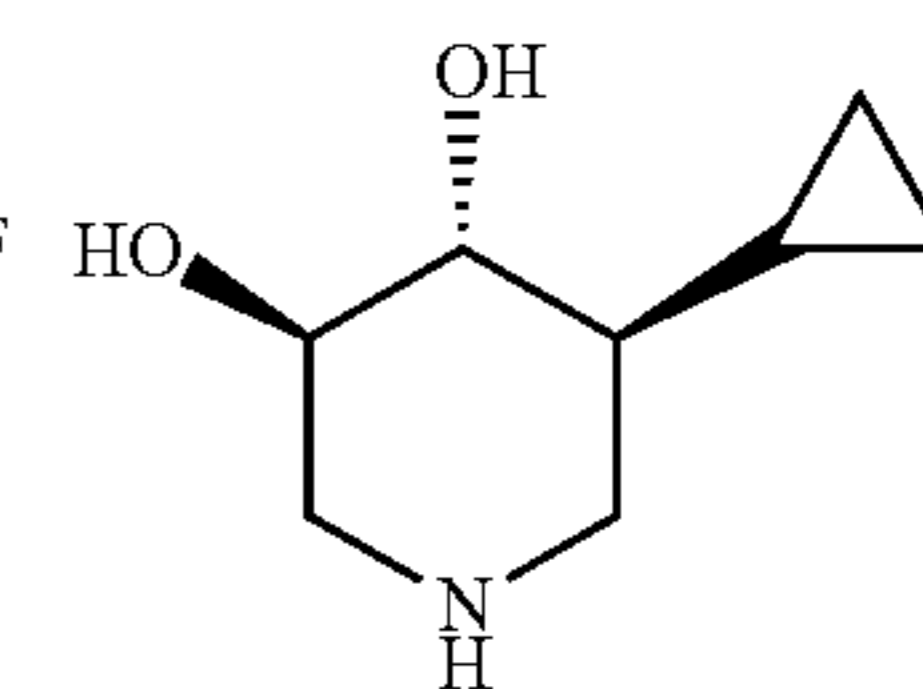
(3R,4R,5S)-5-cyclopropylpiperidine-3,4-diol
