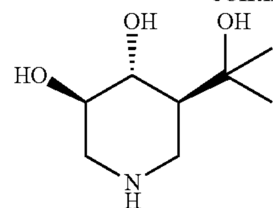
(3R,4R,5S)-5-(2-hydroxypropan-2-yl)piperidine-3,4-diol
