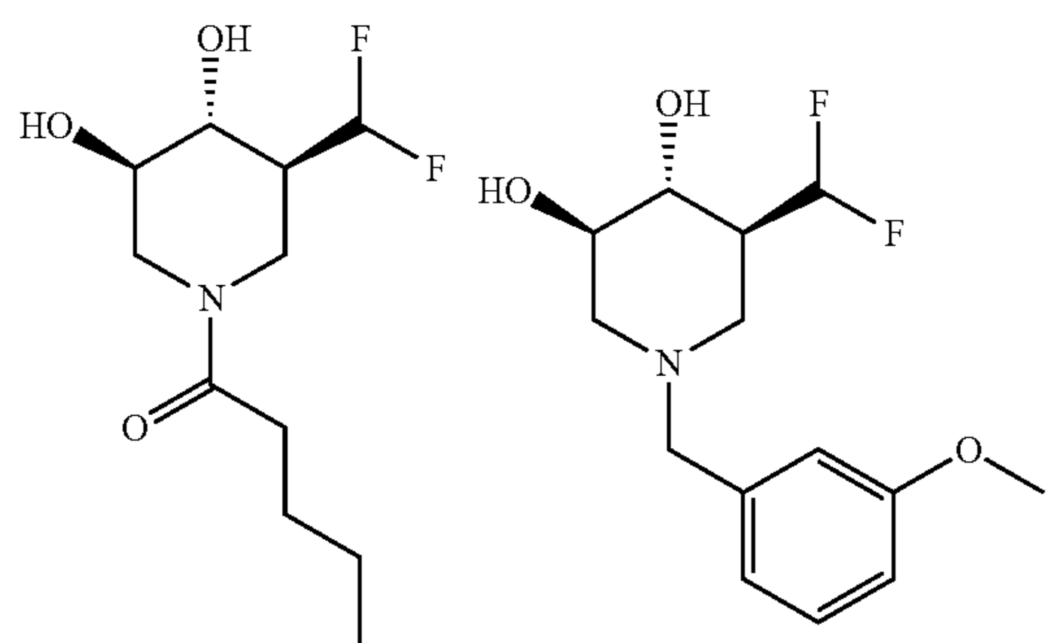
(3R,4R,5S)-5-(difluoromethyl)-1-(3-methoxybenzyl)piperidine-3,4-diol
