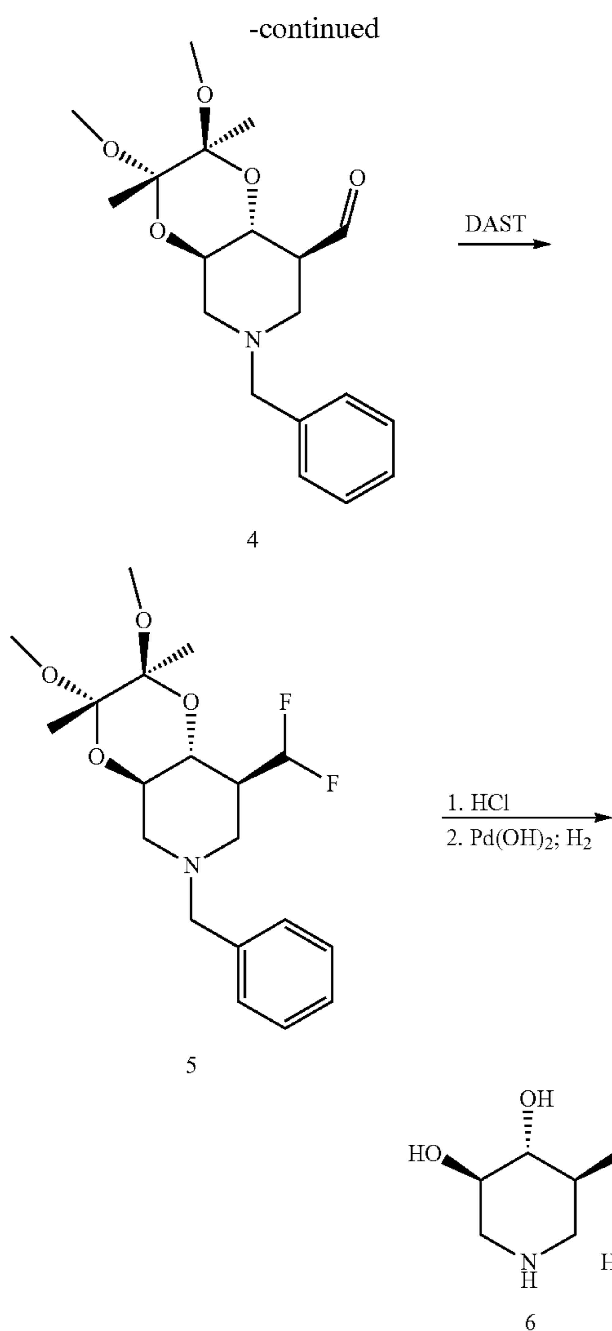
((2S,3S,4aR,8R,8aR)-2,3-Dimethoxy-2,3-dimethyloctahydro-[1,4]dioxino[2,3-c]pyridin-8-yl)methanol Hydrochloride(2)
