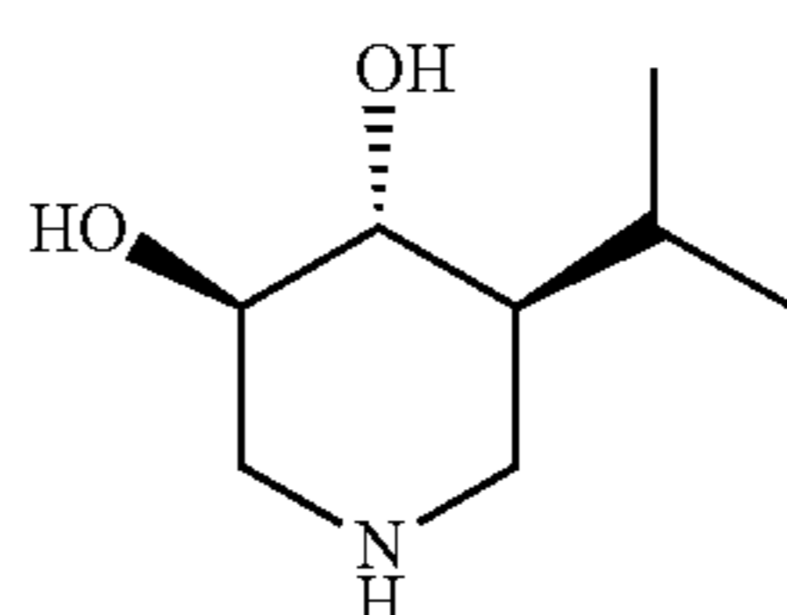
(3R,4R,5S)-5-isopropylpiperidine-3,4-diol
