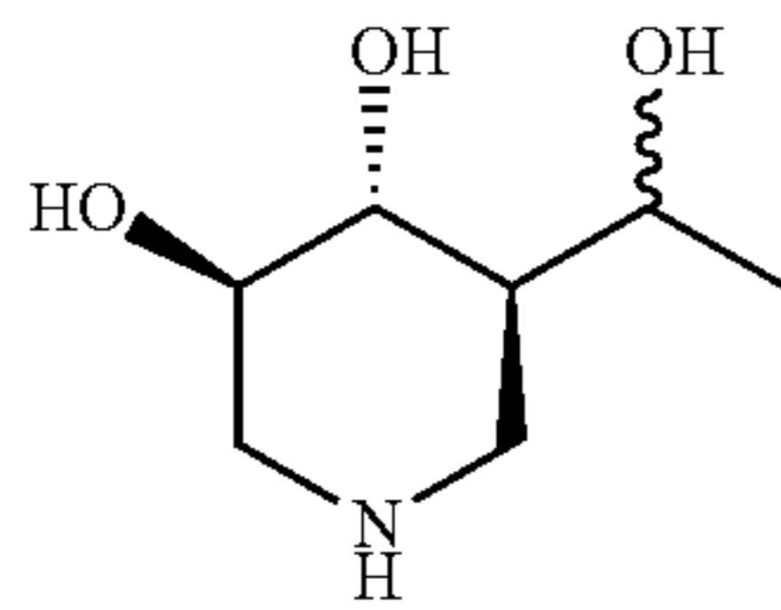
(3R,4R,5R)-5-(1-hydroxyethyl)piperidine-3,4-diol
