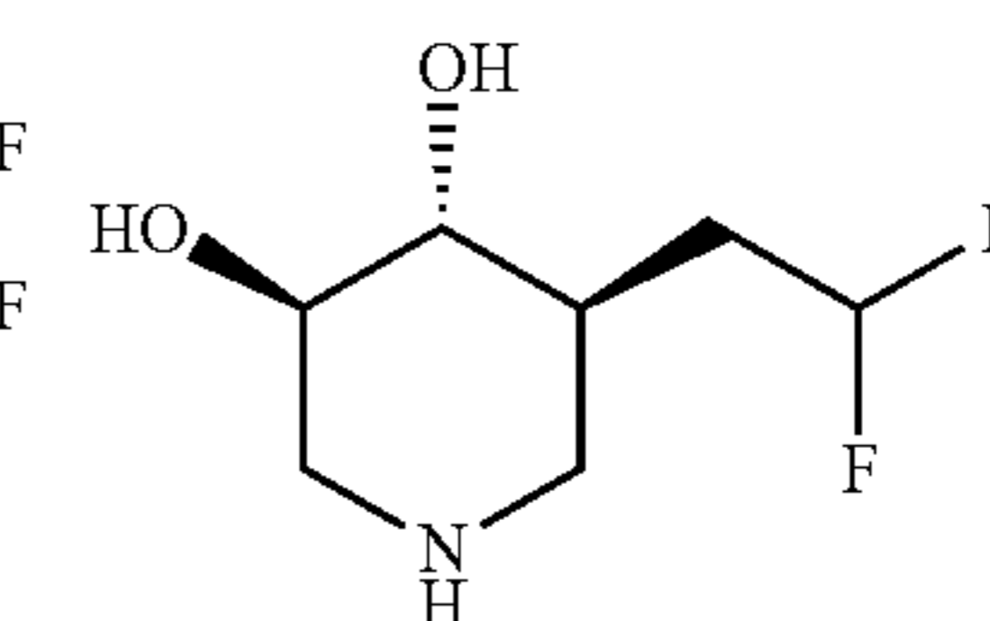
(3R,4R,5S)-5-(2,2-difluoroethyl)piperidine-3,4-diol
