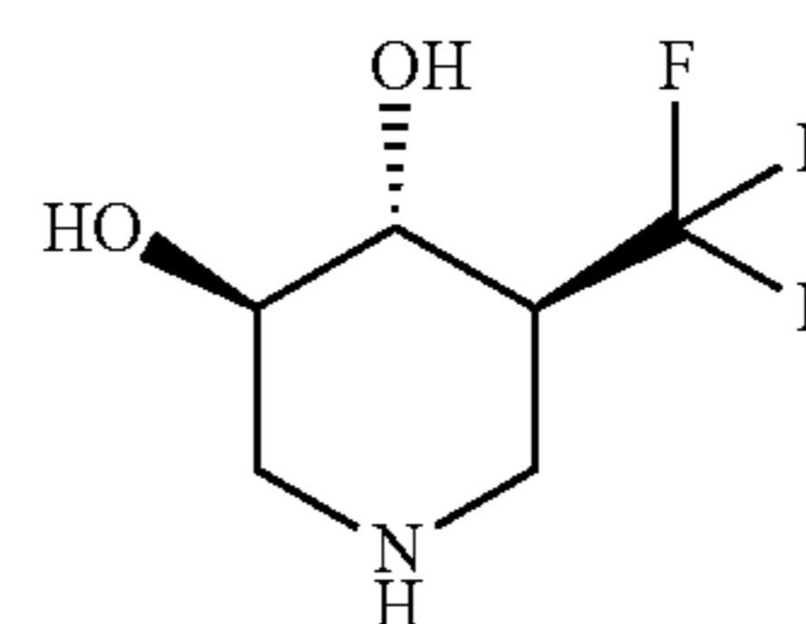
(3R,4R,5S)-5-(trifluoromethyl)piperidine-3,4-diol
