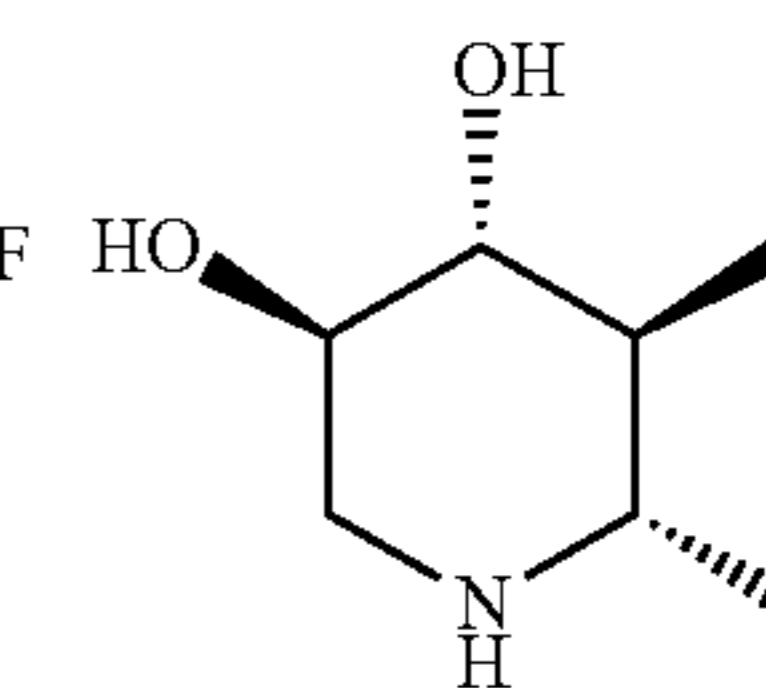
(3R,4R,5S,6S)-6-ethyl-5-(fluoromethyl)piperidine-3,4-diol
