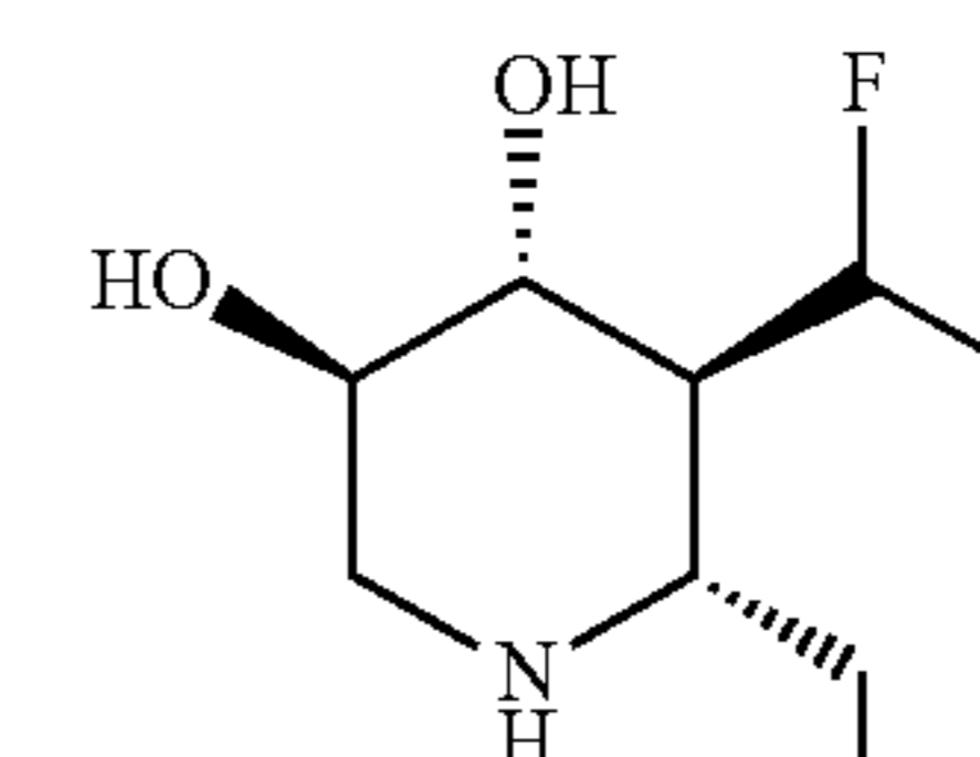
(3R,4R,5S,6S)-5-(difluoromethyl)-6-ethylpiperidine-3,4-diol
