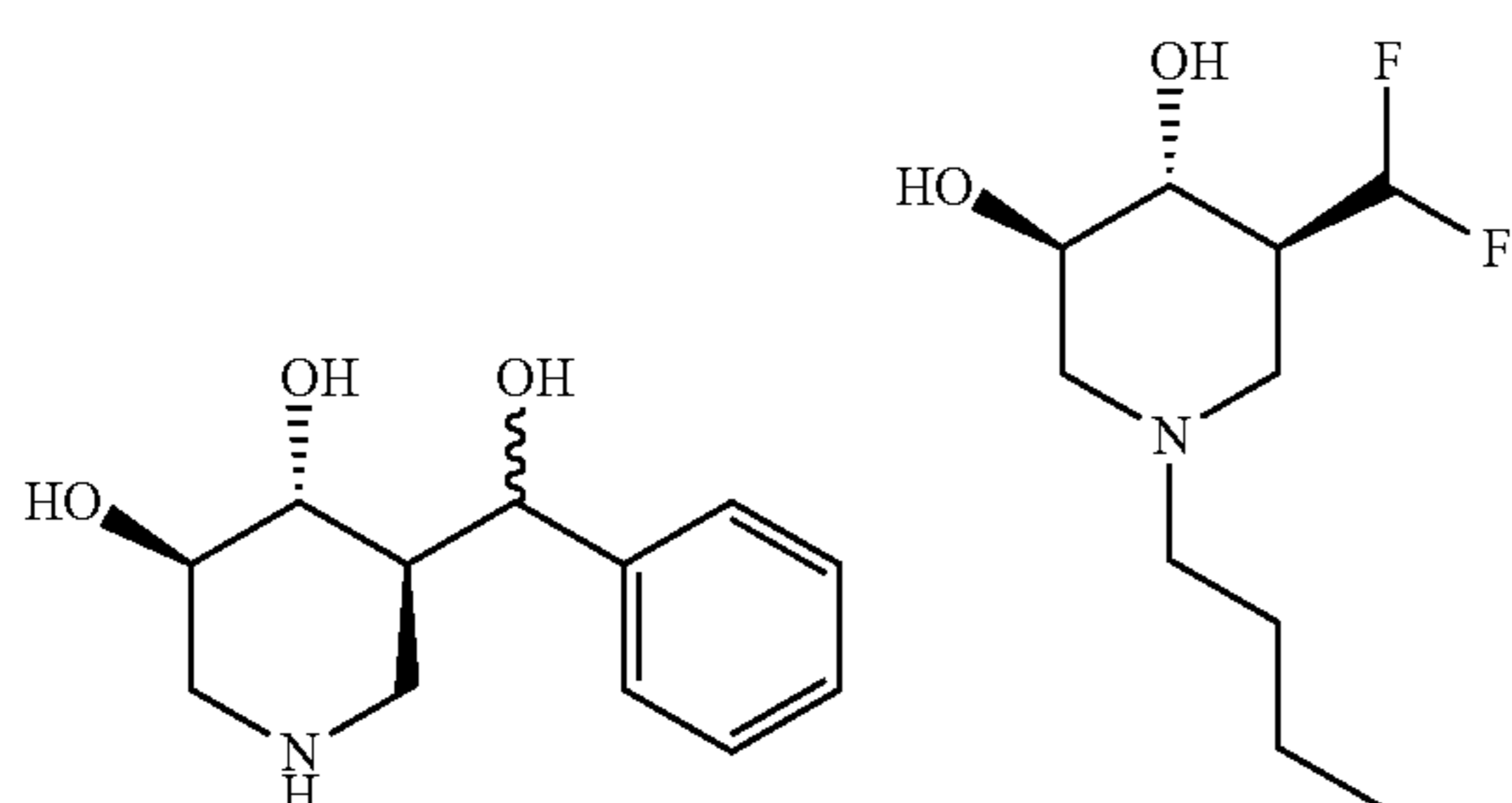
(3R,4R,5R)-5-((S)-hydroxy(phenyl)methyl)piperidine-3,4-diol
