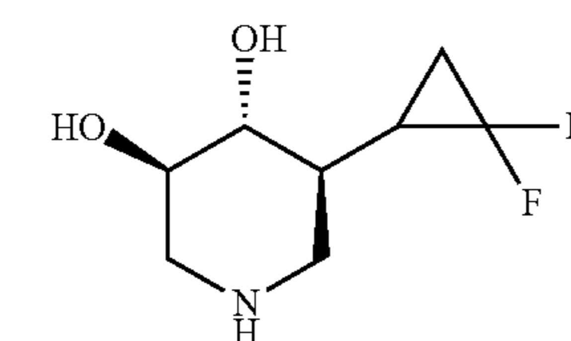
(3R,4R,5S)-5-(2,2-difluorocyclopropyl)piperidine-3,4-diol
