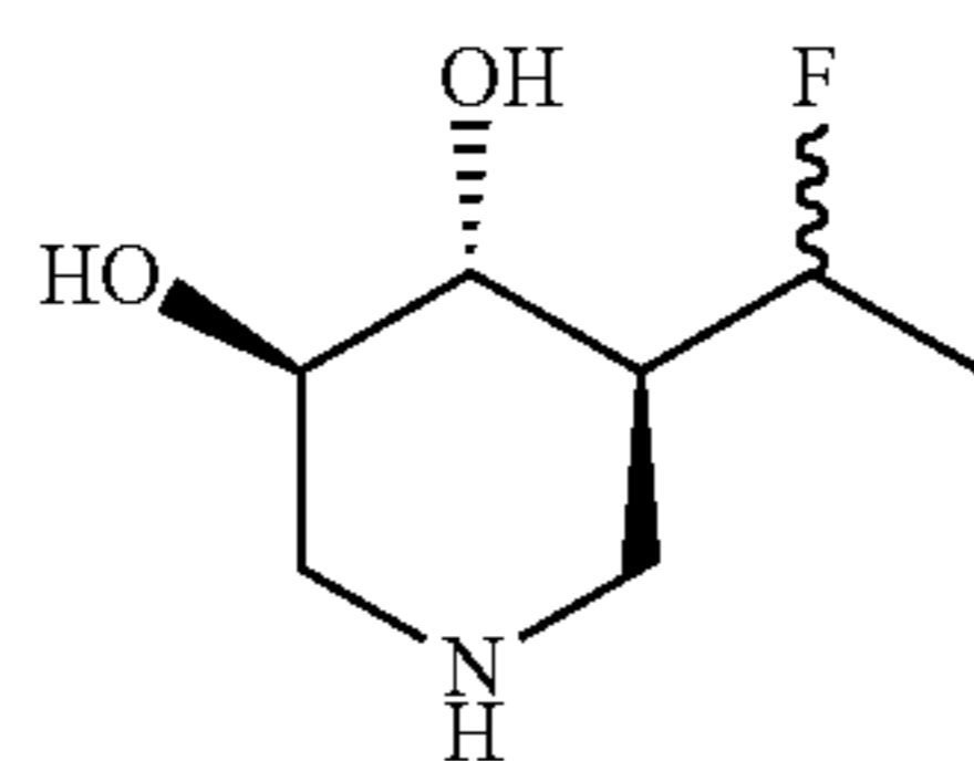
(3R,4R,5S)-5-(1-fluoroethyl)piperidine-3,4-diol
