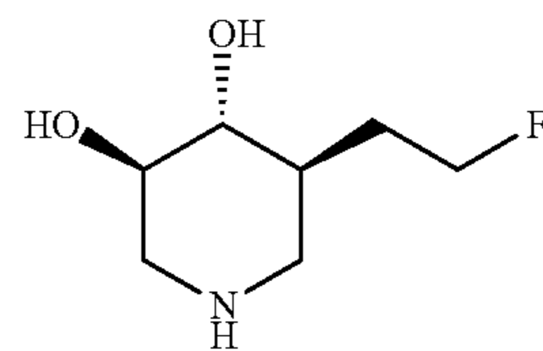
(3R,4R,5S)-5-(2-fluoroethyl)piperidine-3,4-diol
