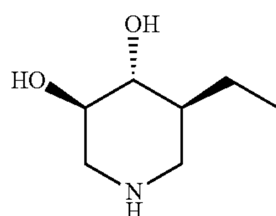
(3R,4R,5S)-5-ethylpiperidine-3,4-diol
