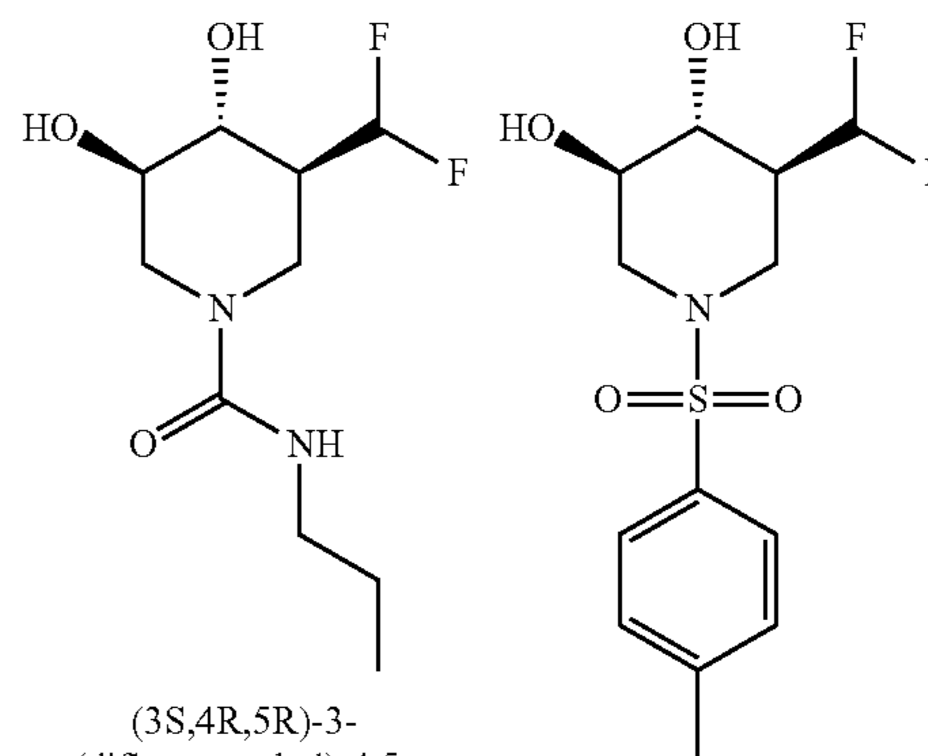
(3R,4R,5S)-5-(difluoromethyl)-1-tosylpiperidine-3,4-diol
