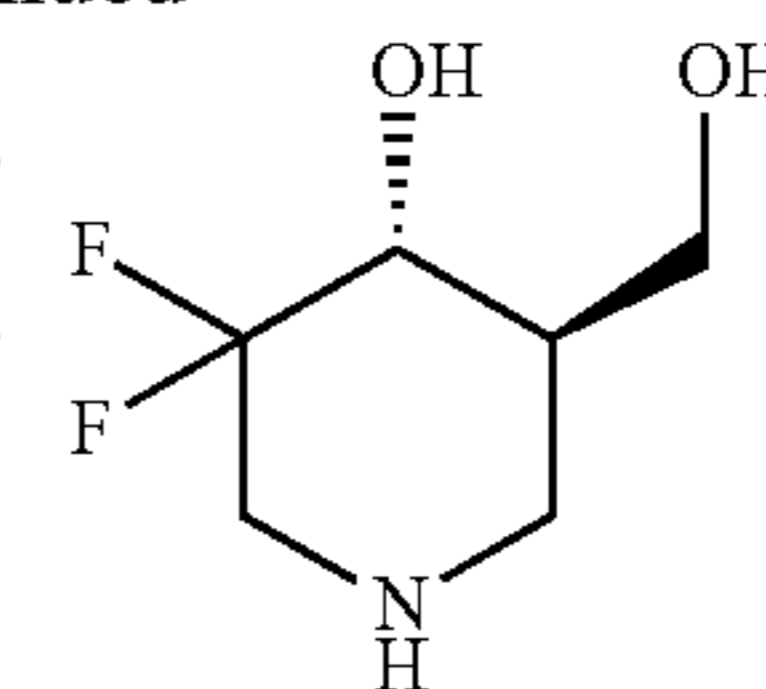
(4R,5R)-3,3-difluoro-5-(hydroxymethyl)piperidine-4-ol
