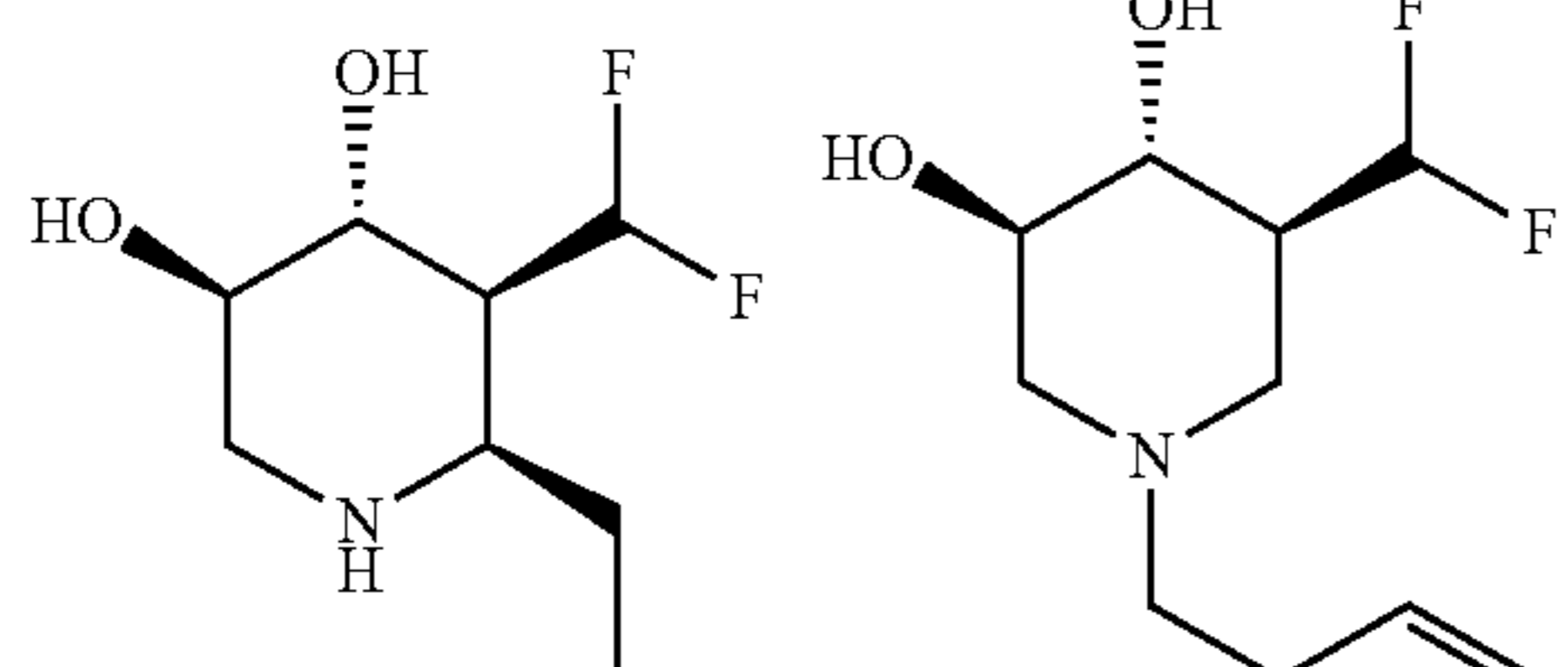
(3R,4R,5S,6R)-5-(difluoromethyl)-6-ethylpiperidine-3,4-diol
