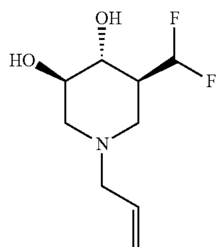
(3R,4R,5S)-1-allyl-5-(difluoromethyl)piperidine-3,4-diol
