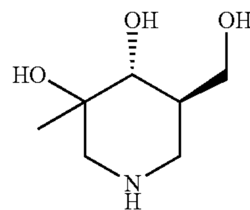
(4R,5R)-5-(hydroxymethyl)-3-methylpiperidine-3,4-diol
