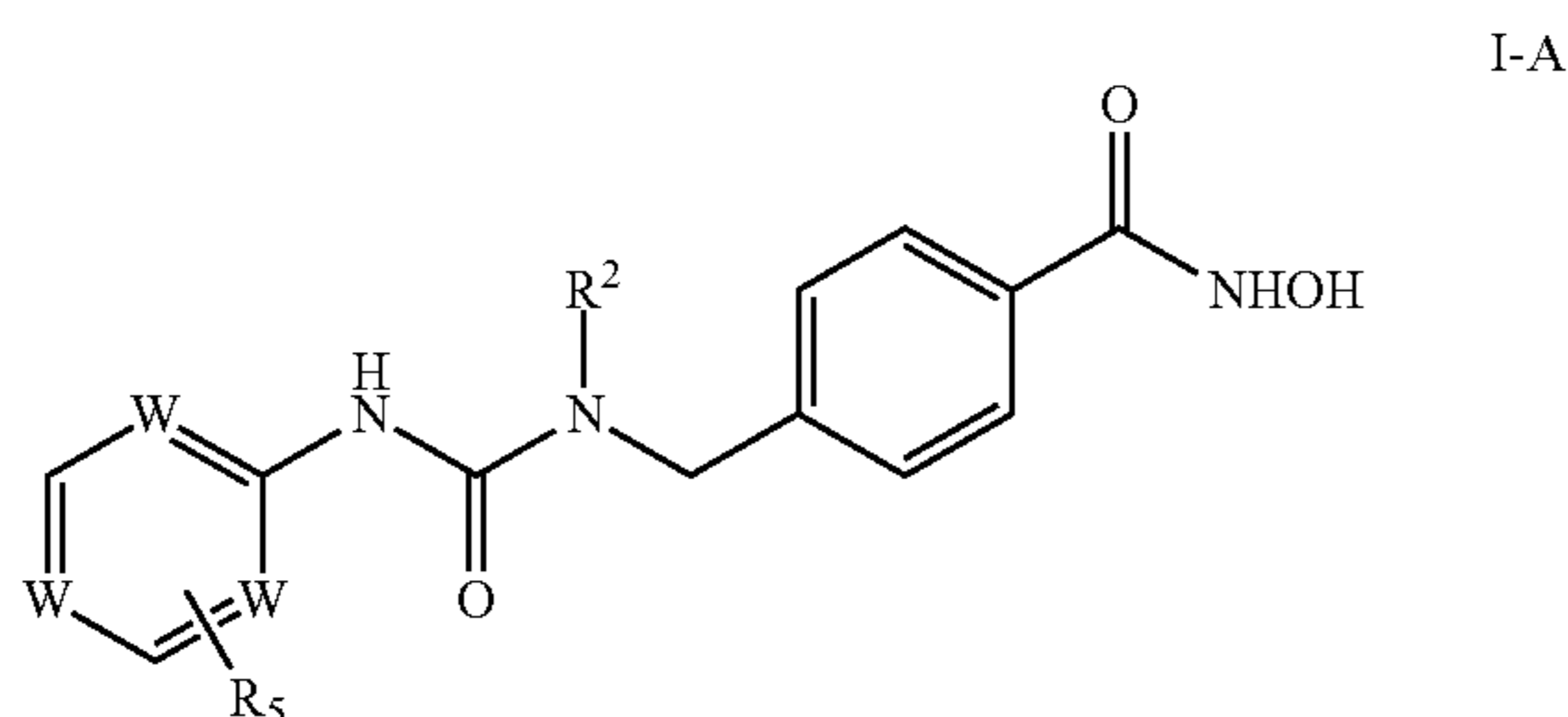
Scheme 1: Synthesis of proximal N-substituted hydroxamic acids
