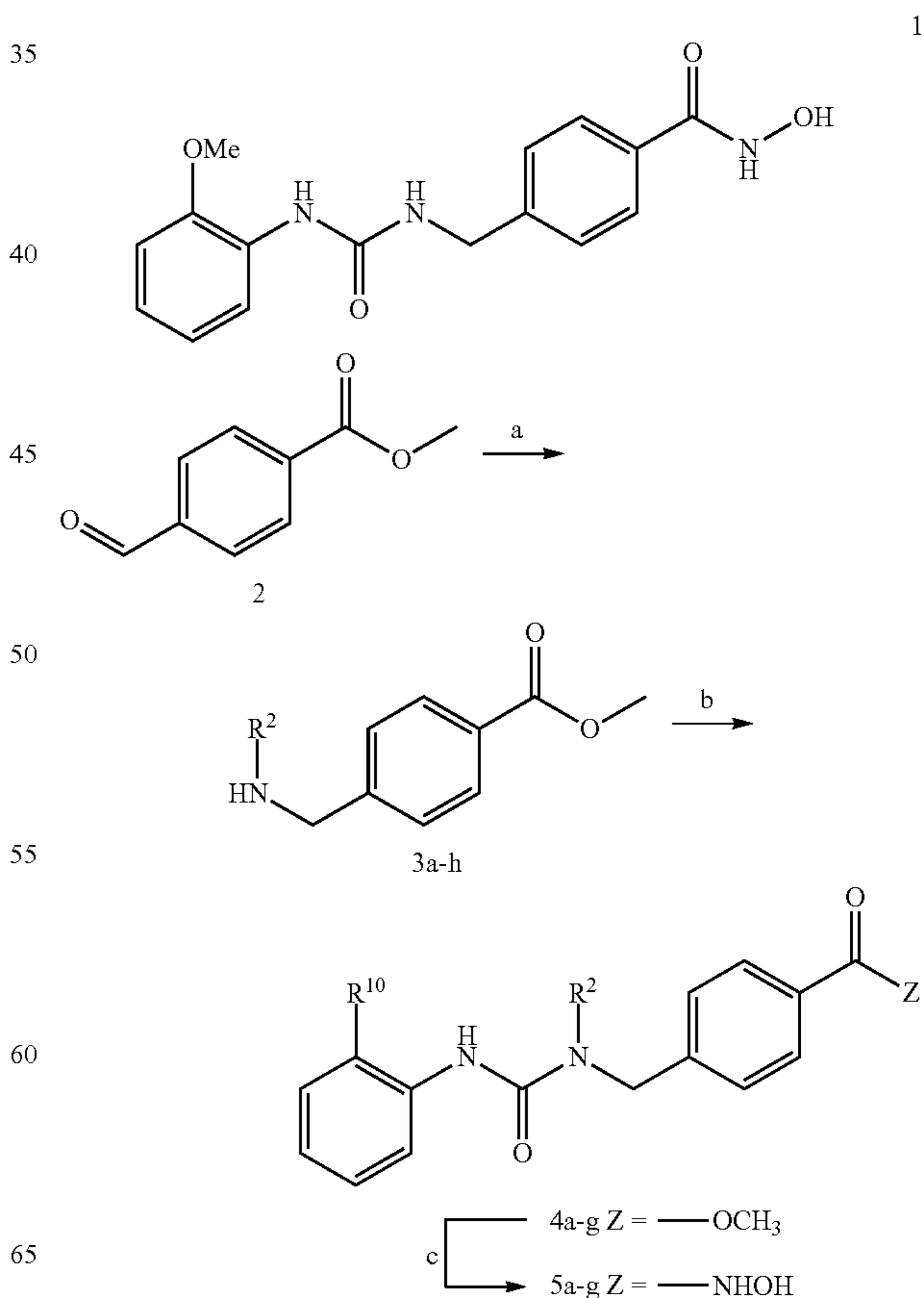
Scheme 1: Synthesis of proximal N-substituted hydroxamic acids
