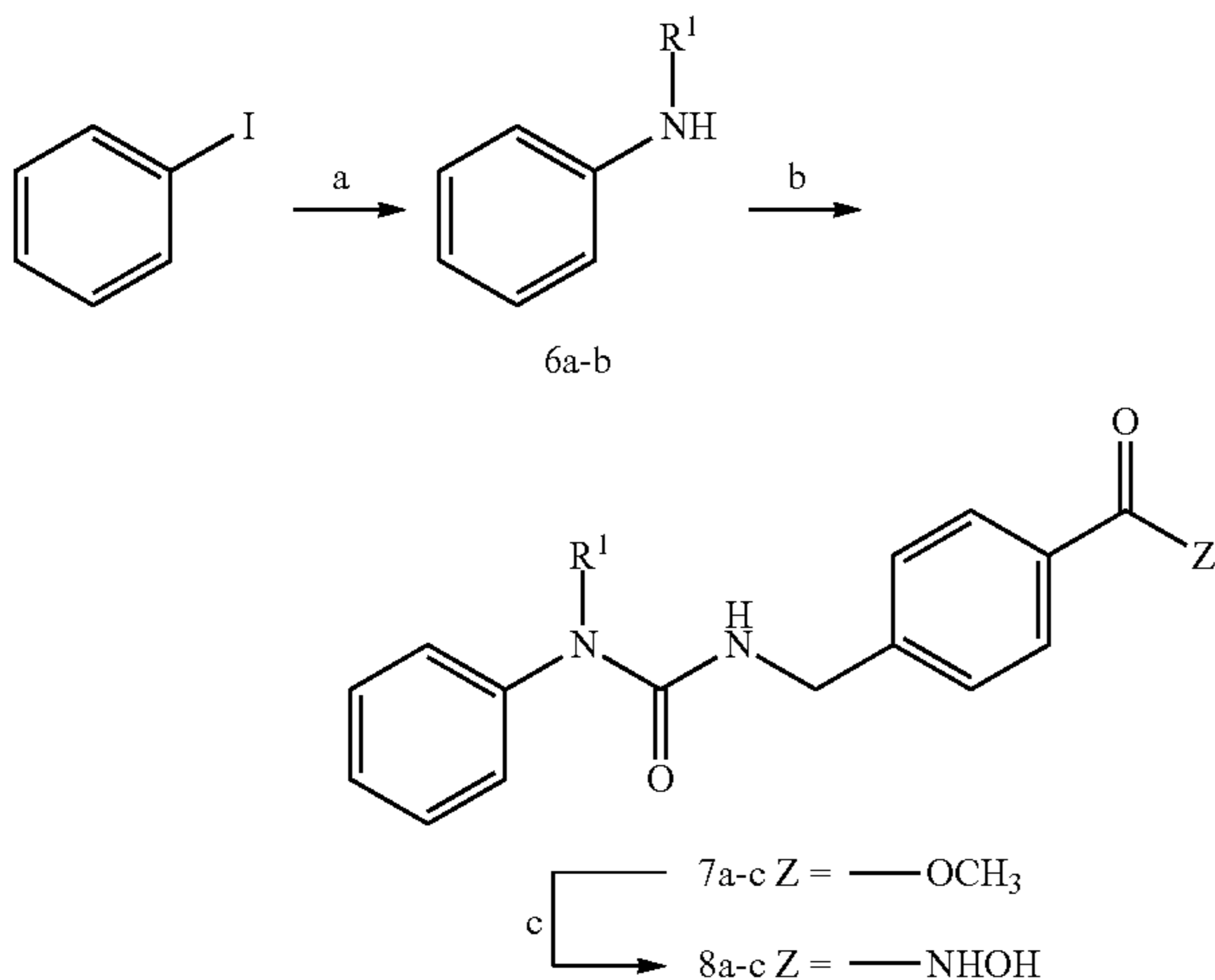
Scheme 2: Synthesis of distal N-substituted hydroxamic acids
