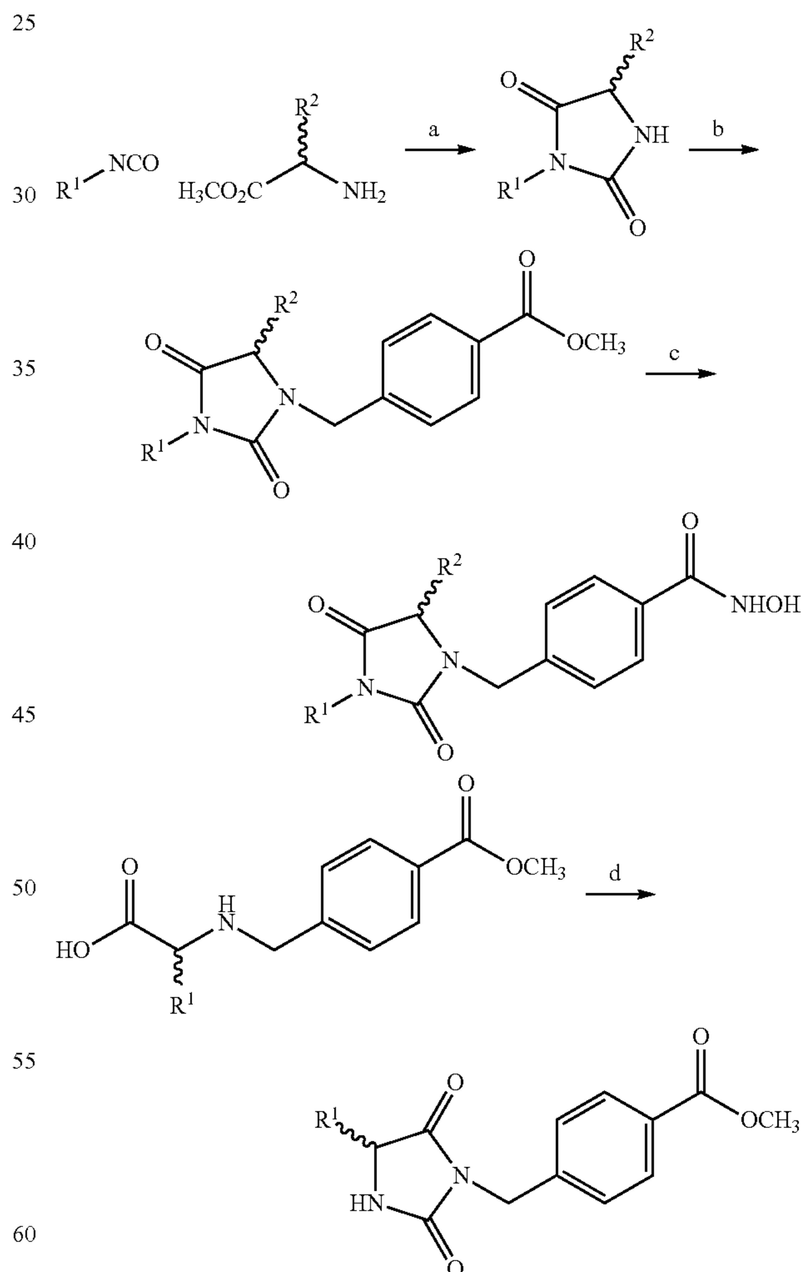
Scheme 3: Synthesis of cyclic urea hydroxamic acids
