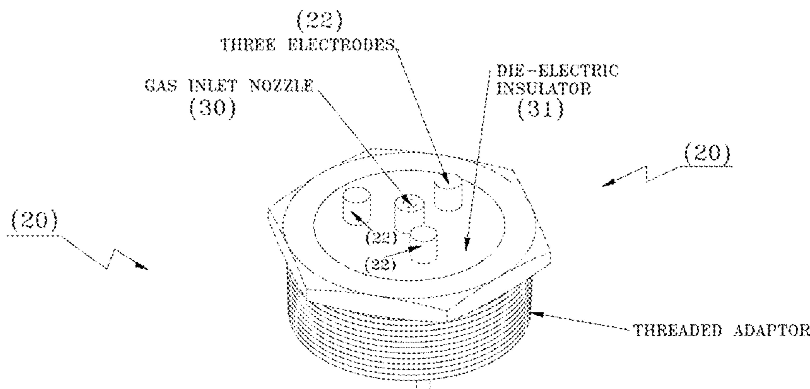
THREE ELECTRODE SPARK PLUG
