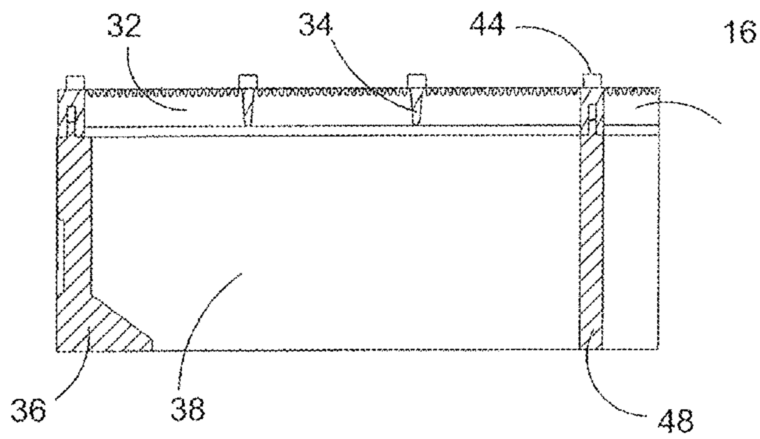
SECTION B-B
