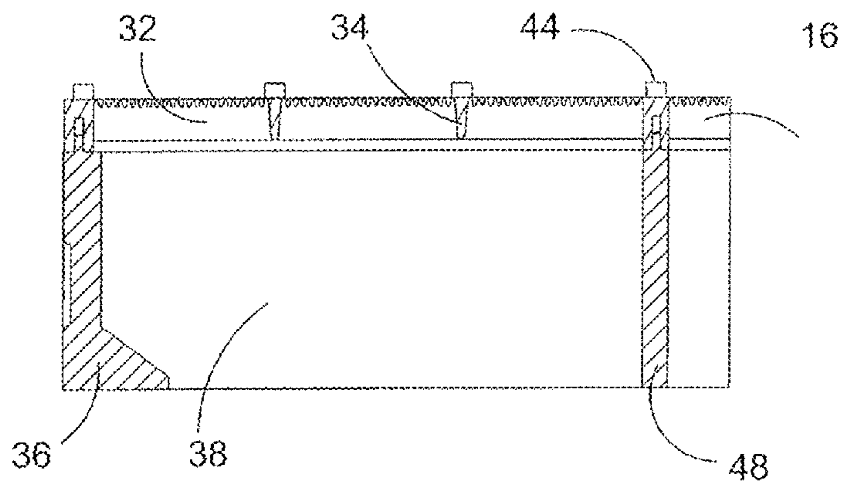
SECTION B-B
