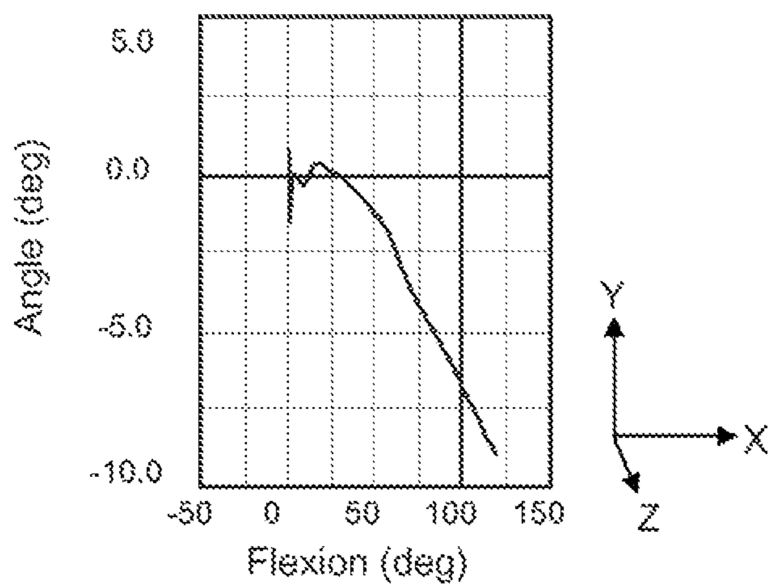
KNEE VARUS ANGLE vs FLEXION
