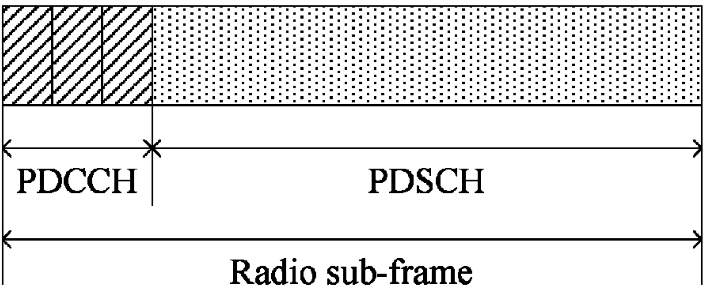
FIG. 4 (Prior Art)
