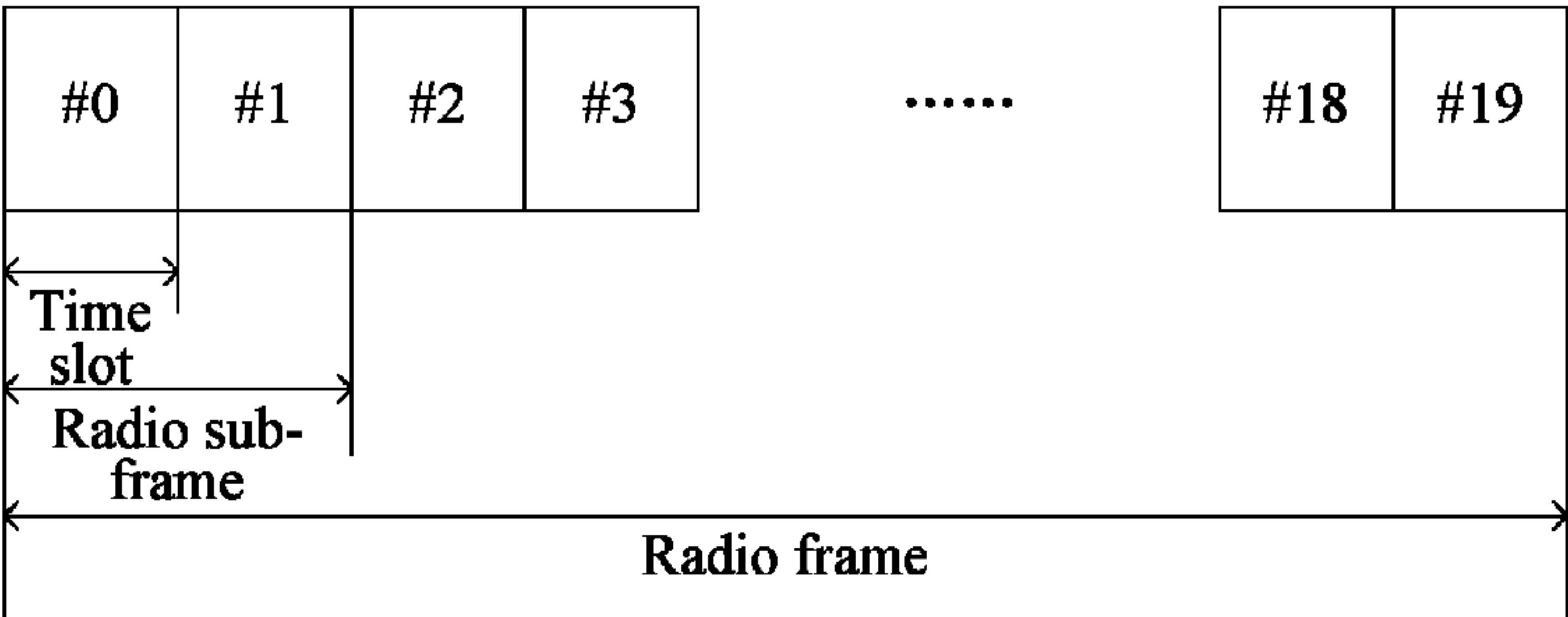
FIG. 3 (Prior Art)
