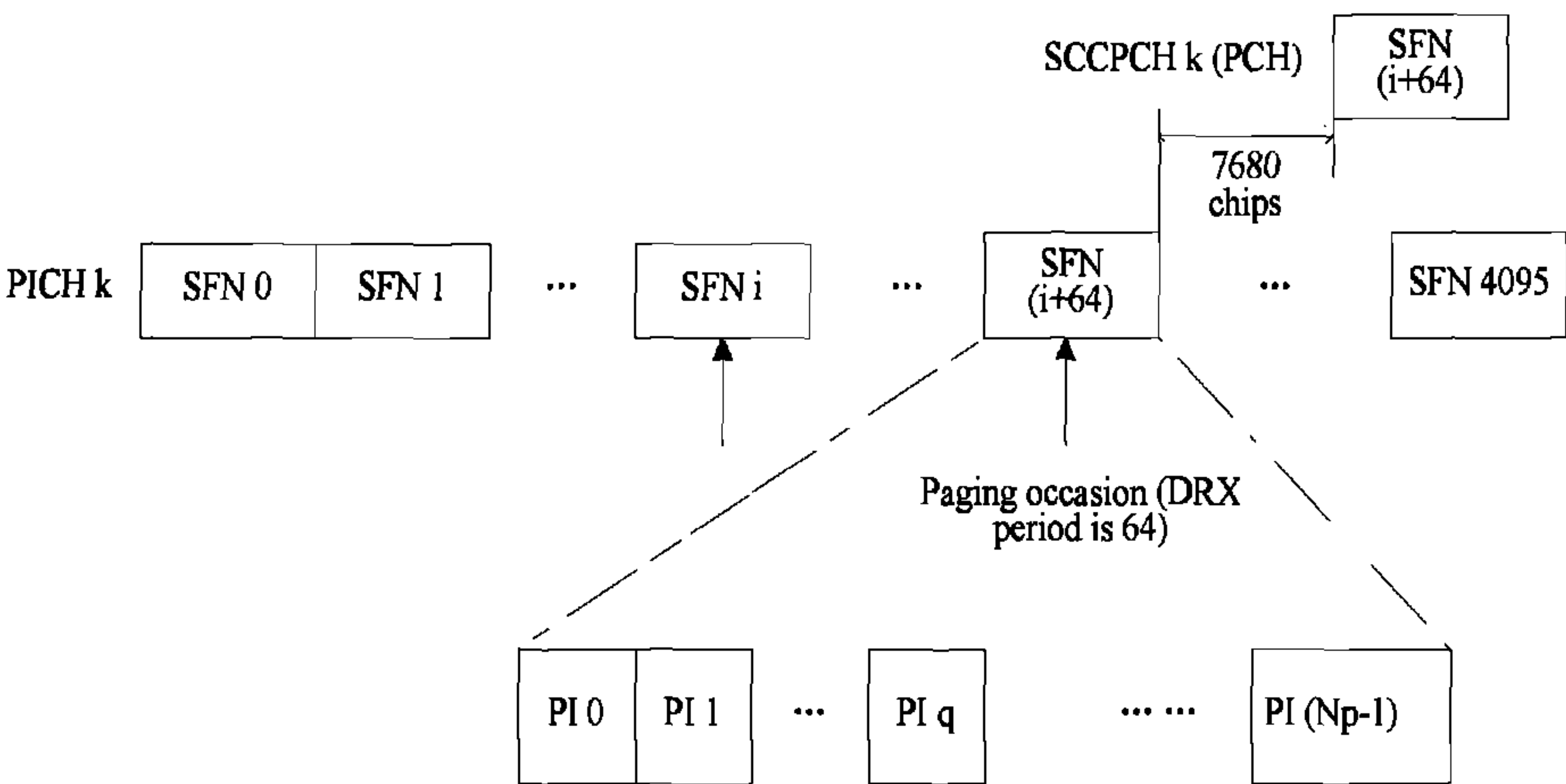
FIG. 2 (Prior Art)
