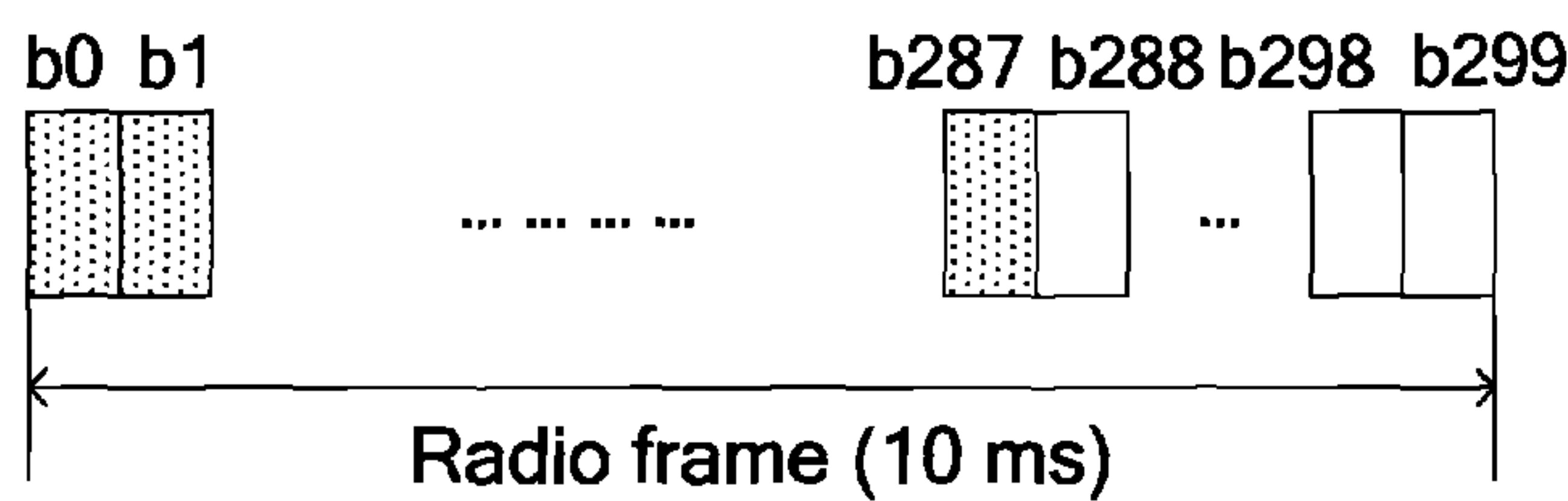
FIG. 1 (Prior Art)
