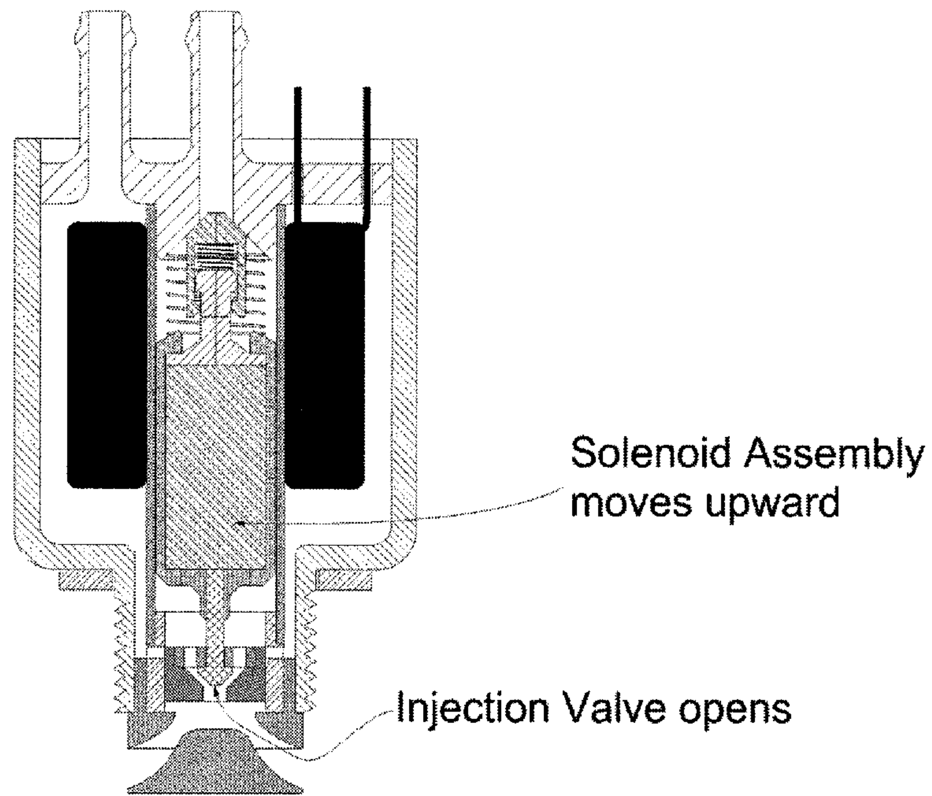
Figure 6 Solenoid Activation
