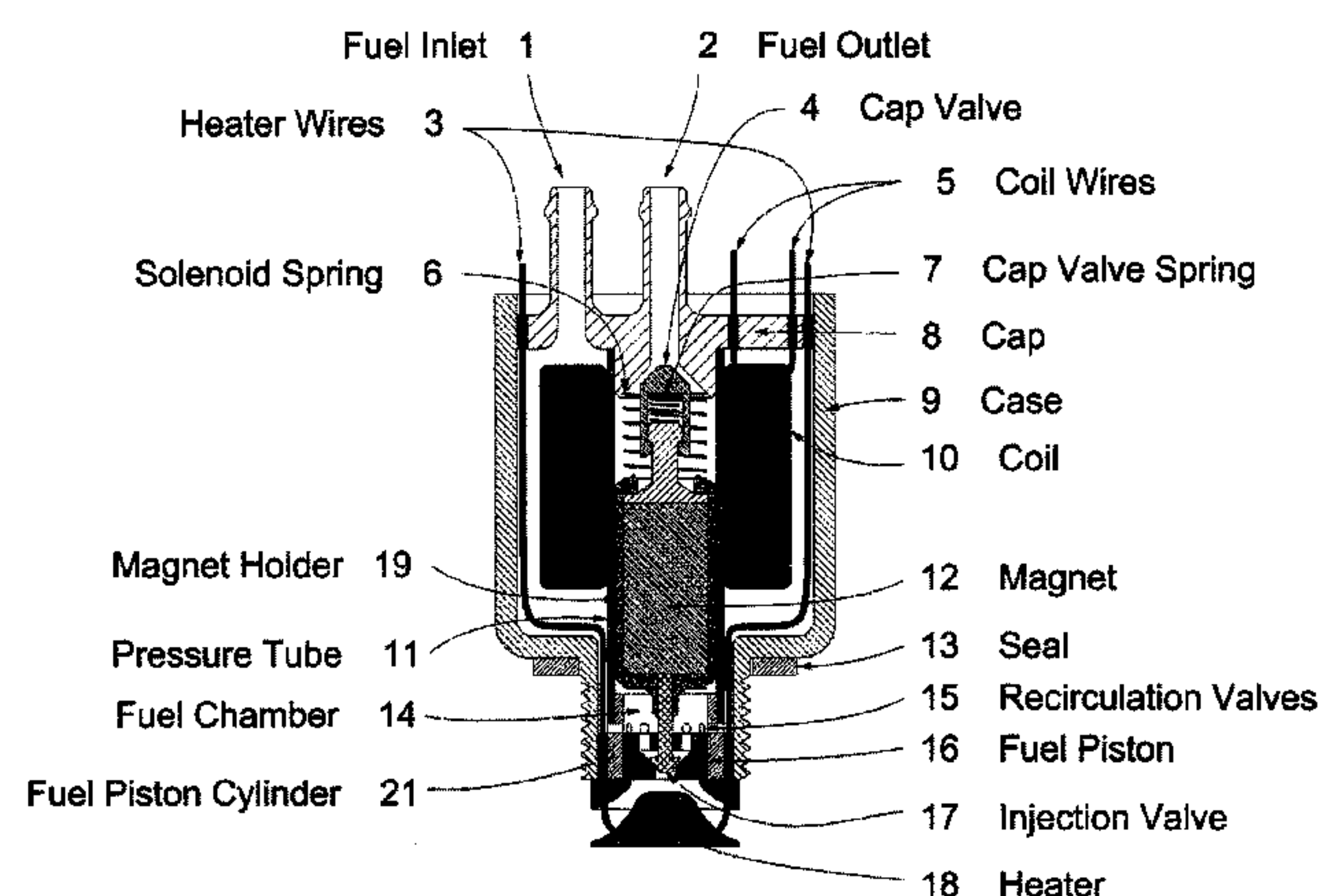
Injector Assembly
