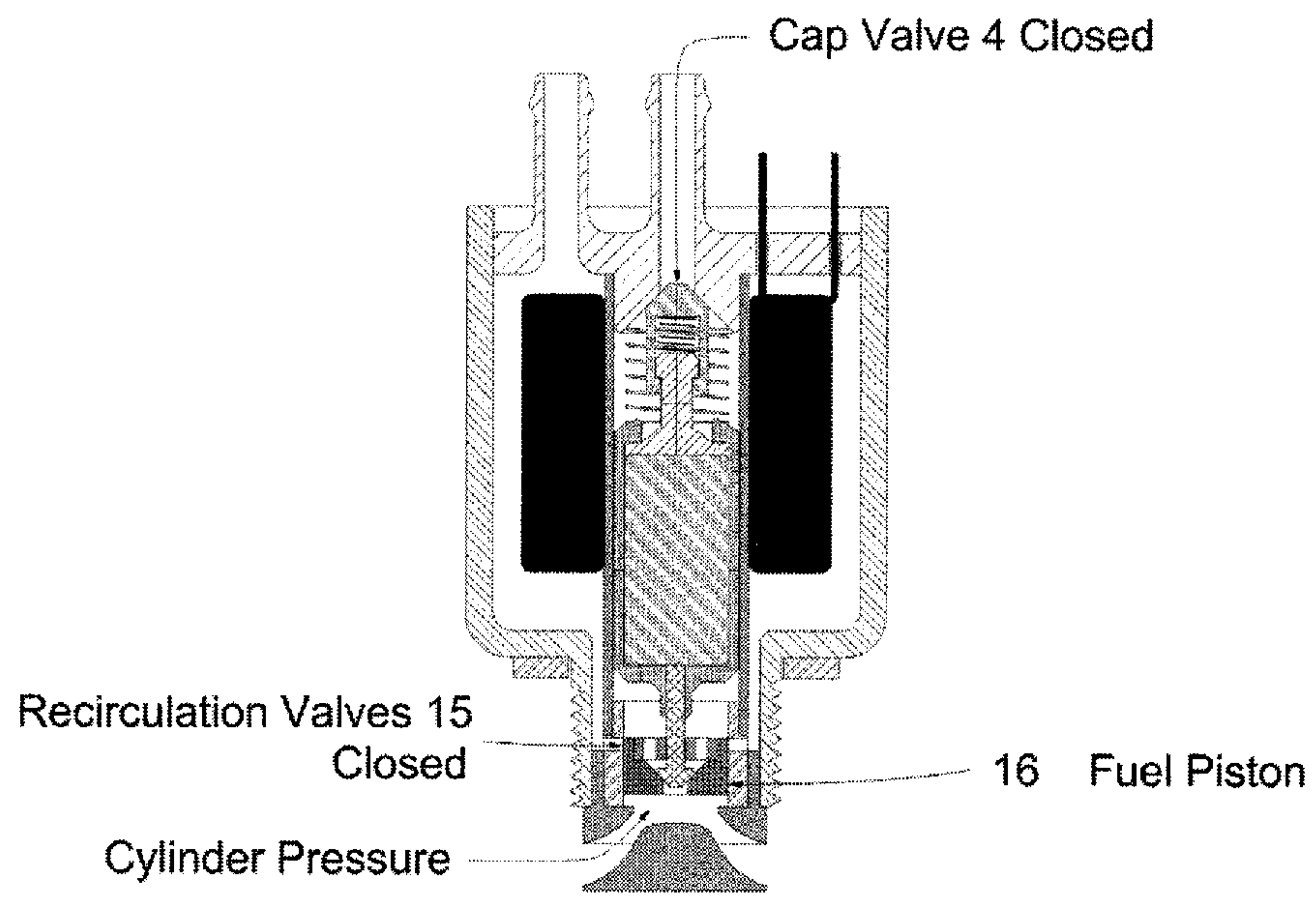
Figure 5 Cylinder Pressure Valve Closure
