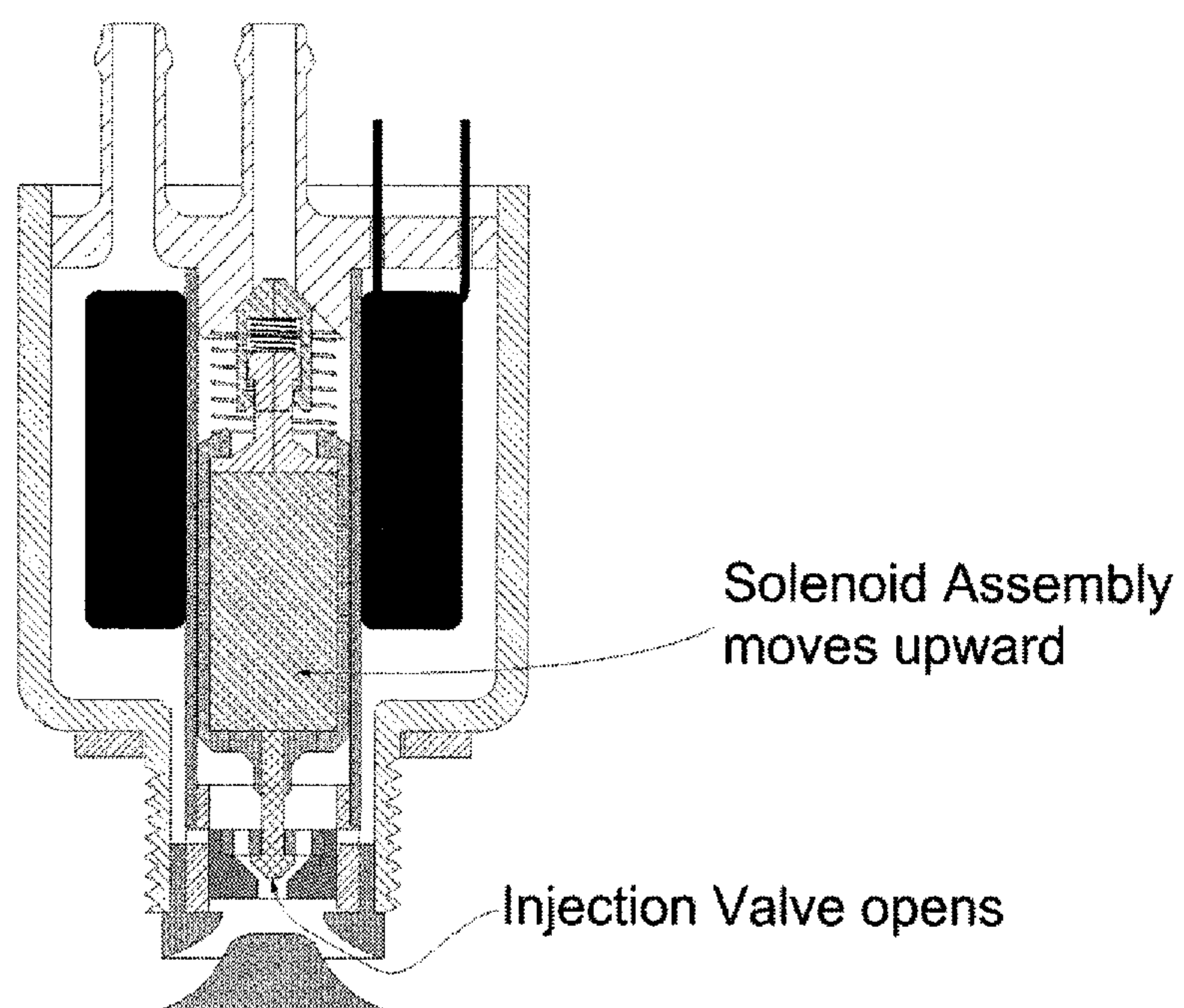
Figure 6 Solenoid Activation
