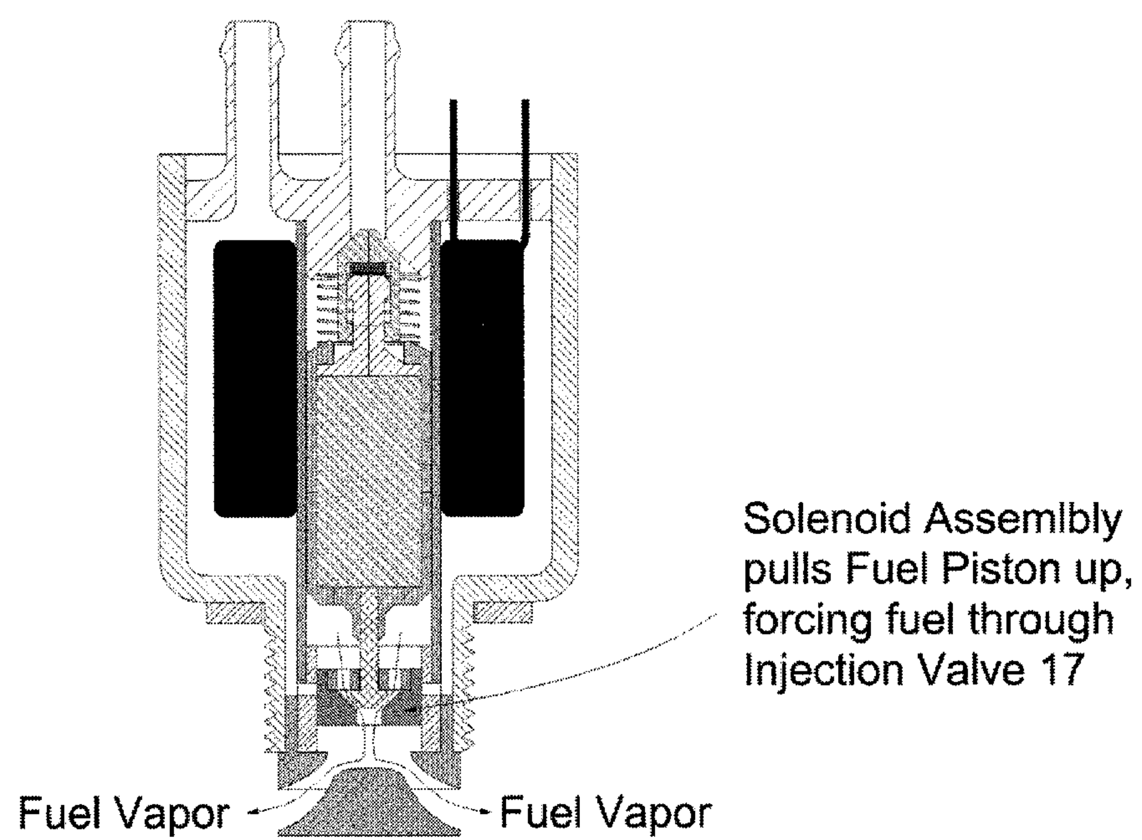
Figure 7 Fuel Injection
