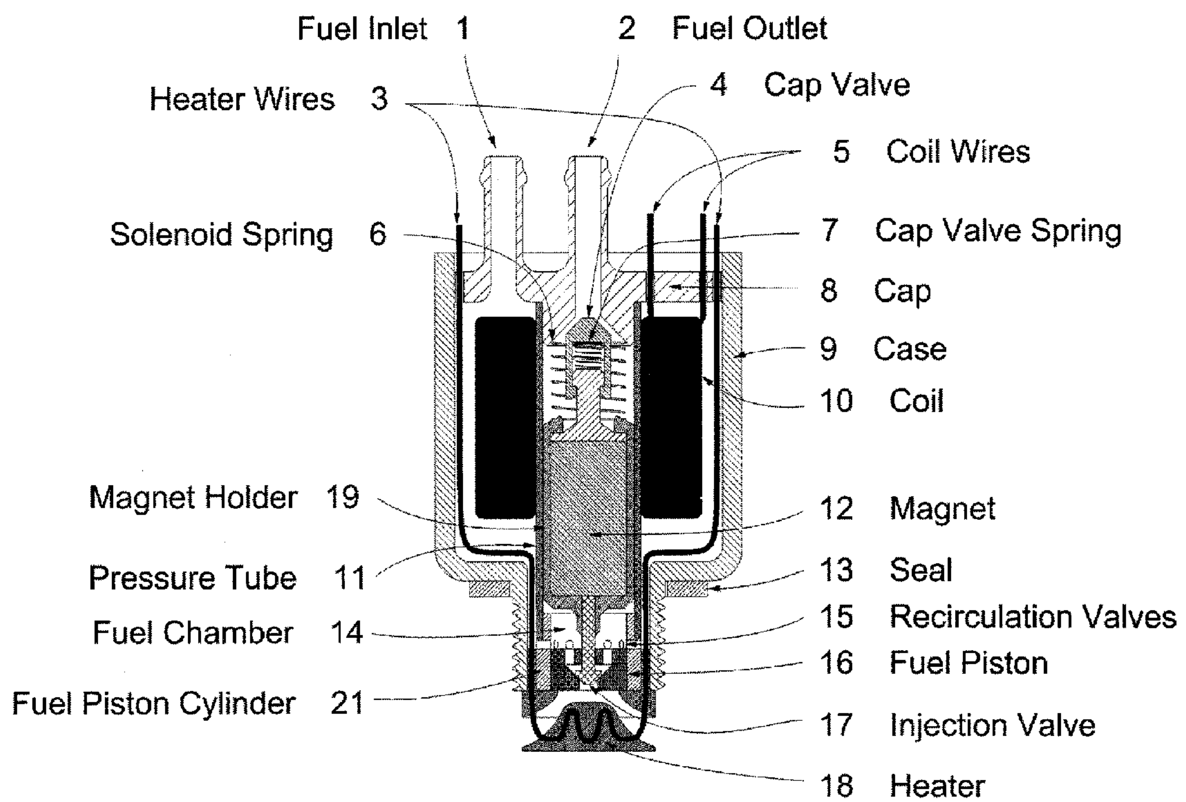
Figure 2 Injector Assembly
