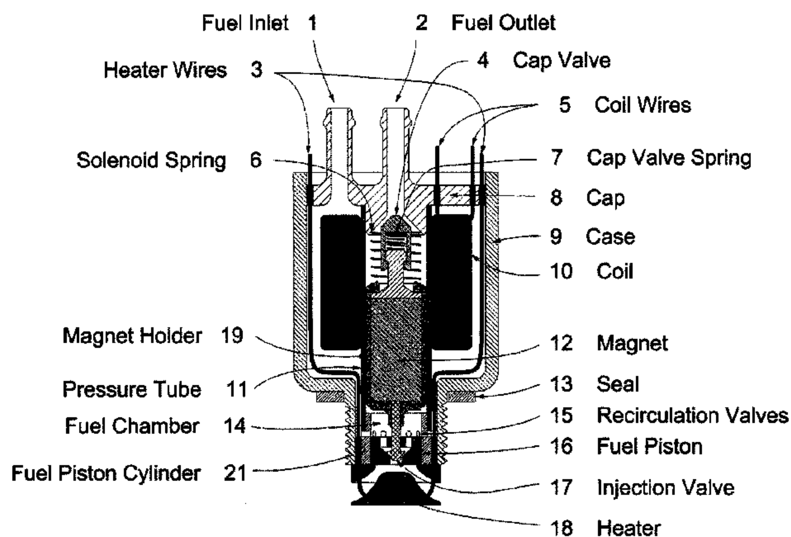
Injector Assembly
