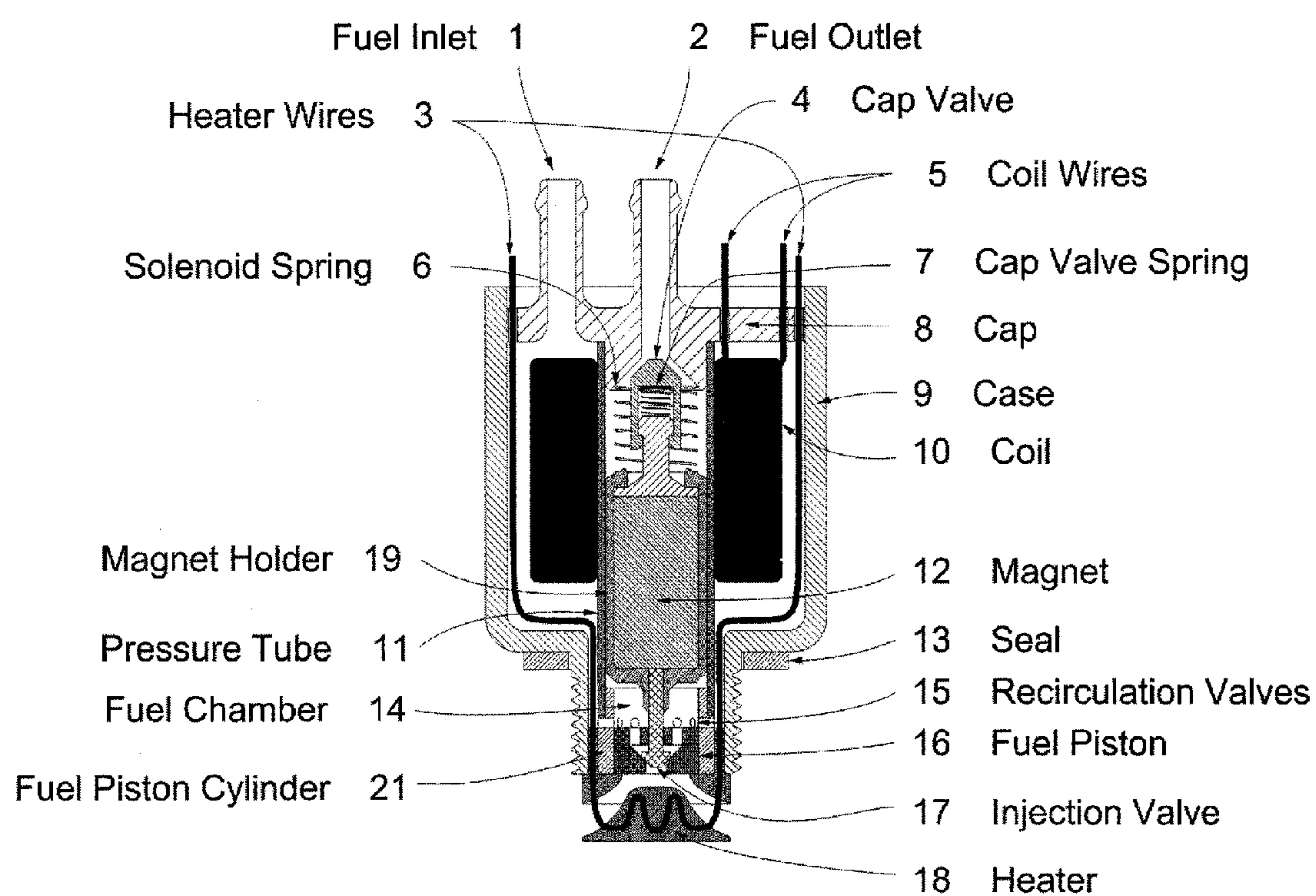
Figure 2 Injector Assembly
