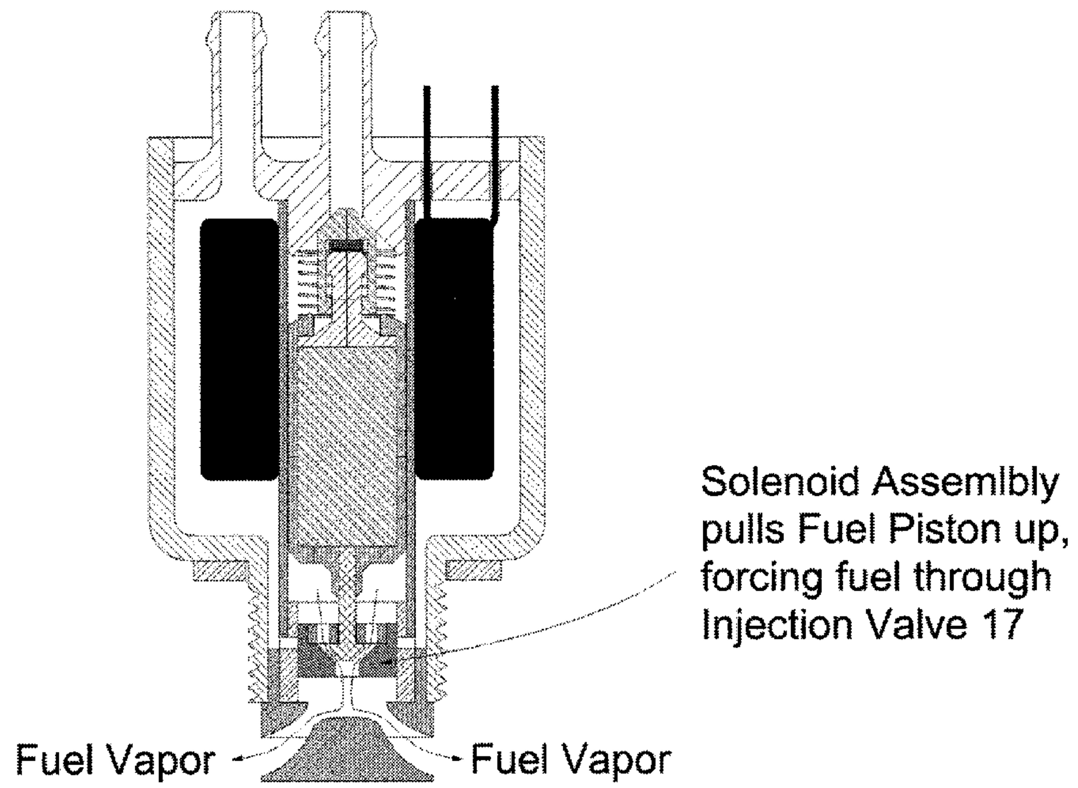
Figure 7 Fuel Injection
