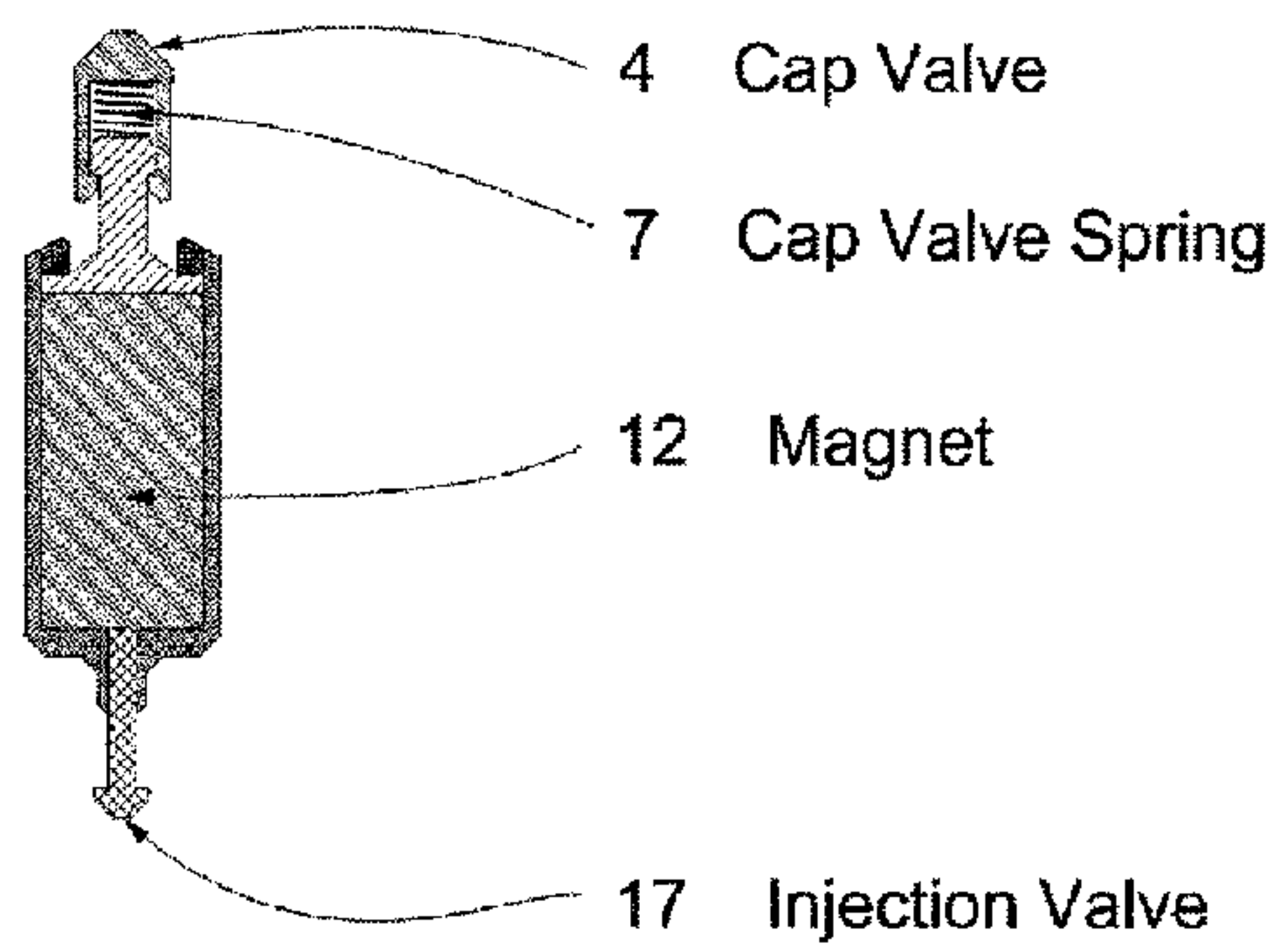
Figure 3A Solenoid Assembly
