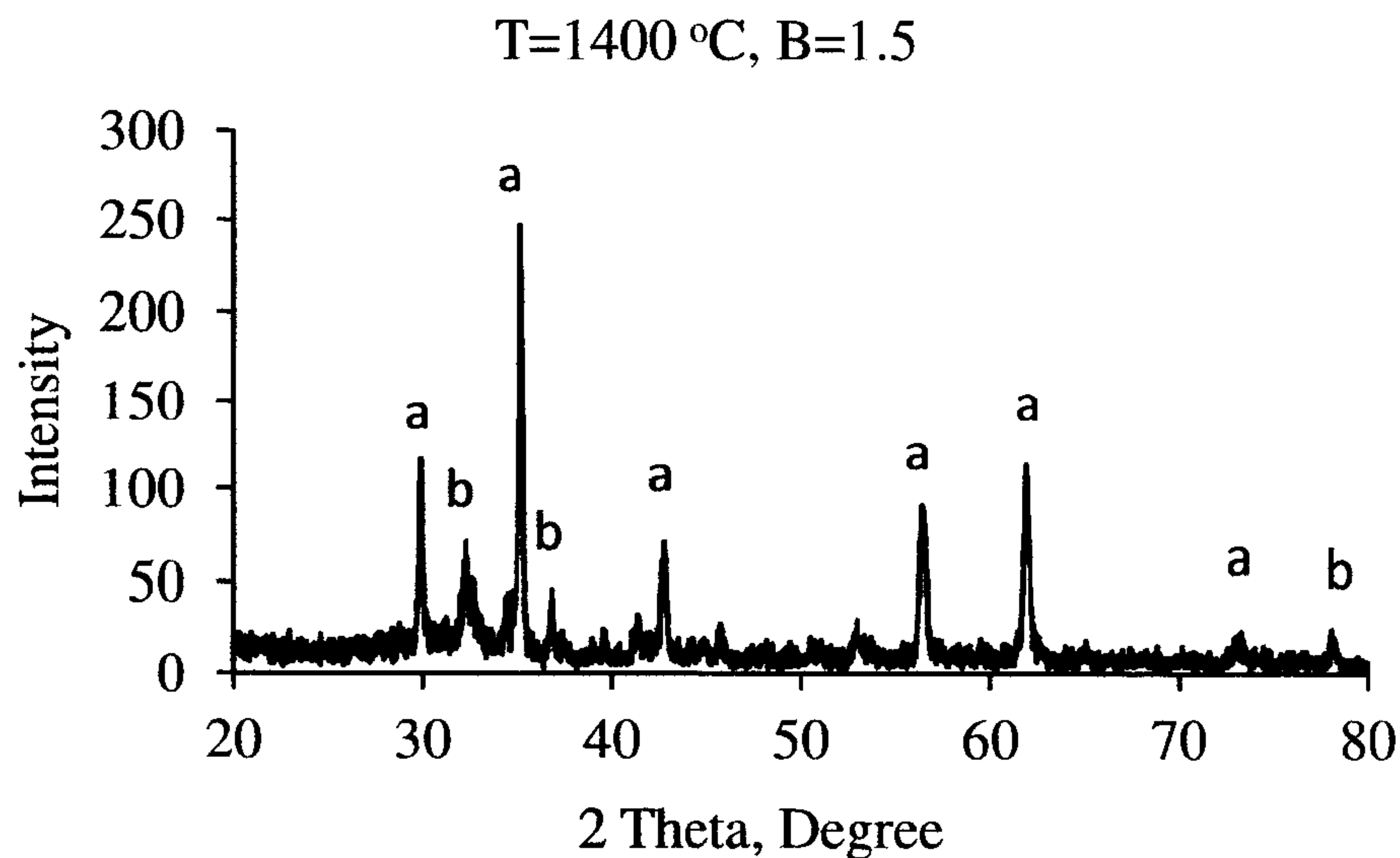
XRD pattern, a - manganese ferrite, b - calcium silicate
