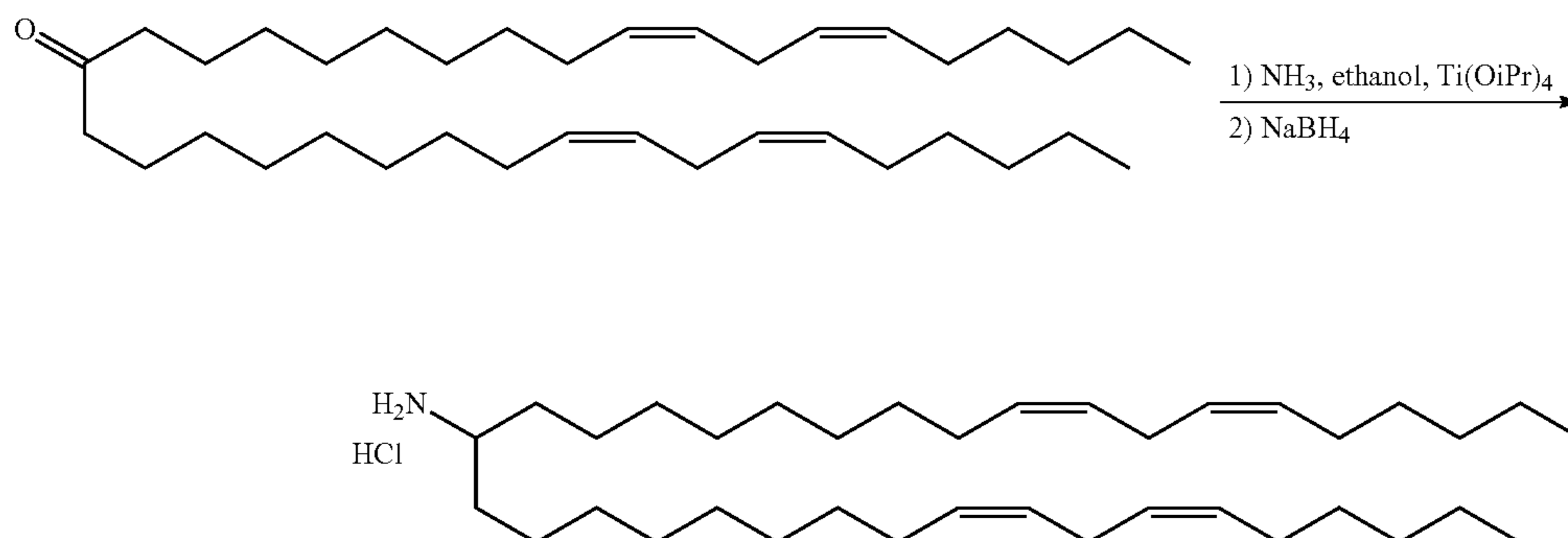
Scheme 10
