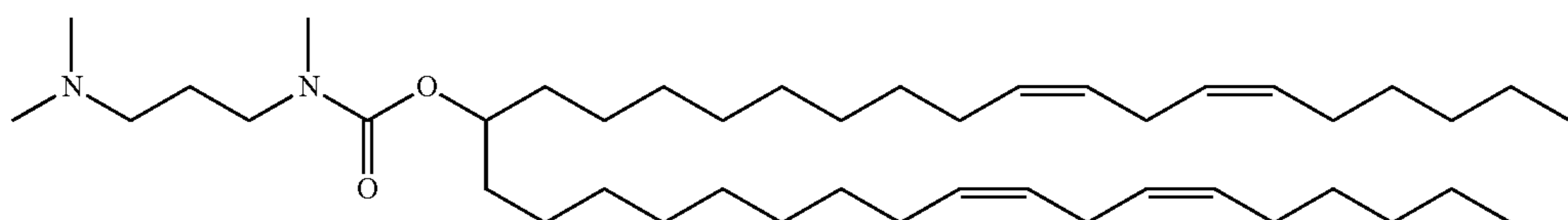
MC3MC
