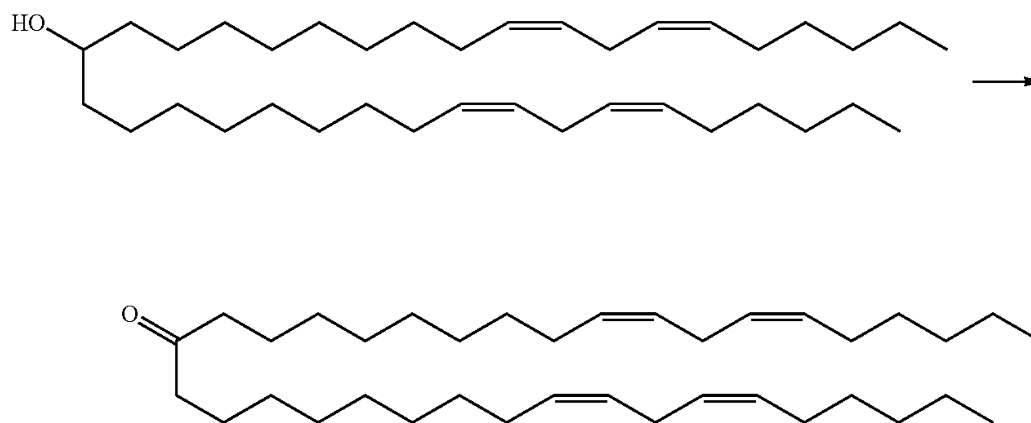
Scheme 9
