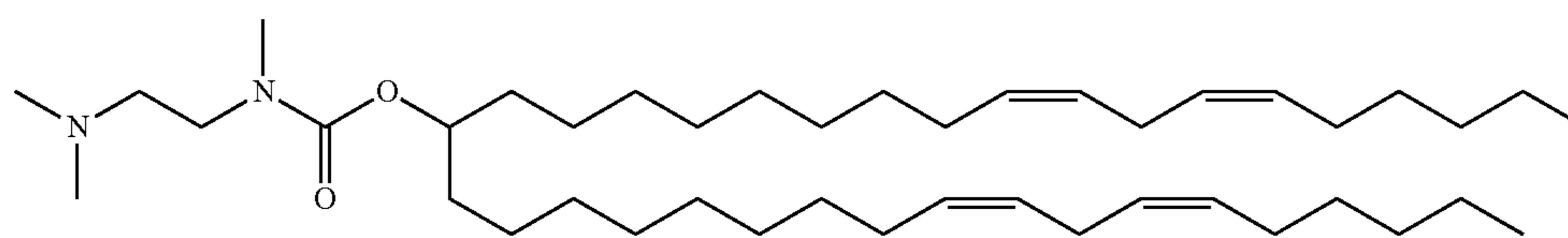
MC2MC
