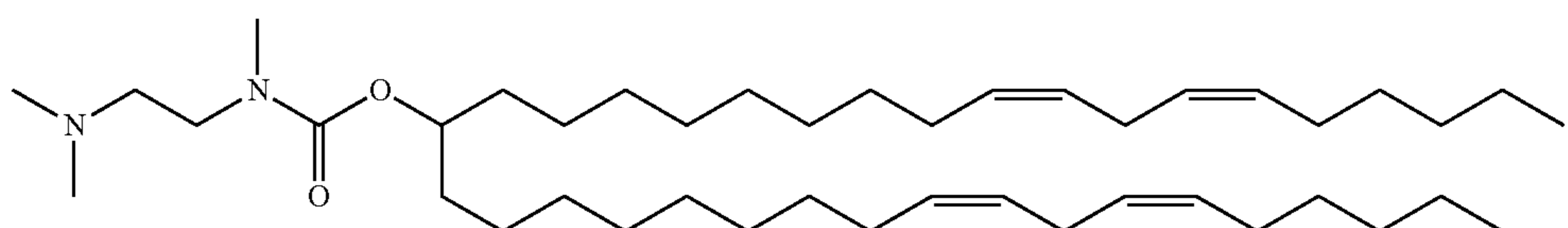
MC2MC
