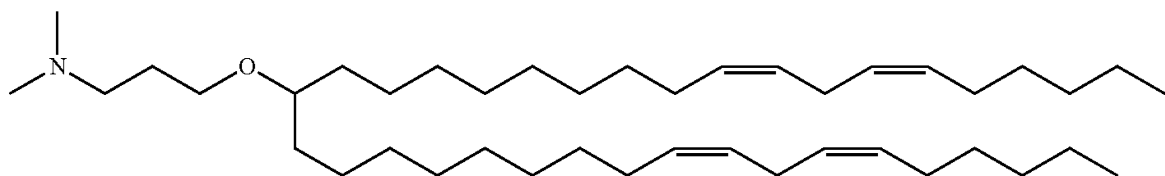
MC3 Ether
