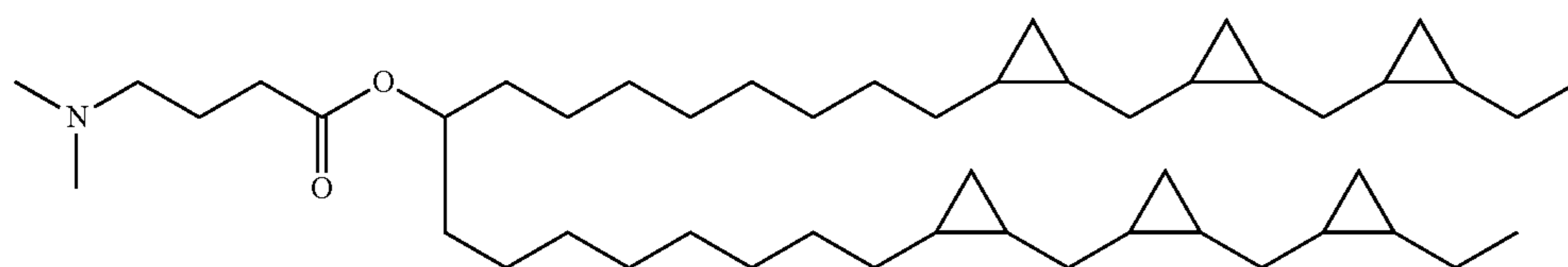
CP-LenMC3
