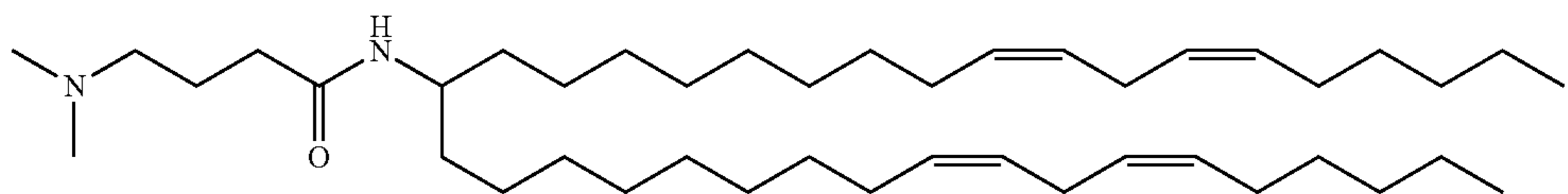
MC3 Amide
