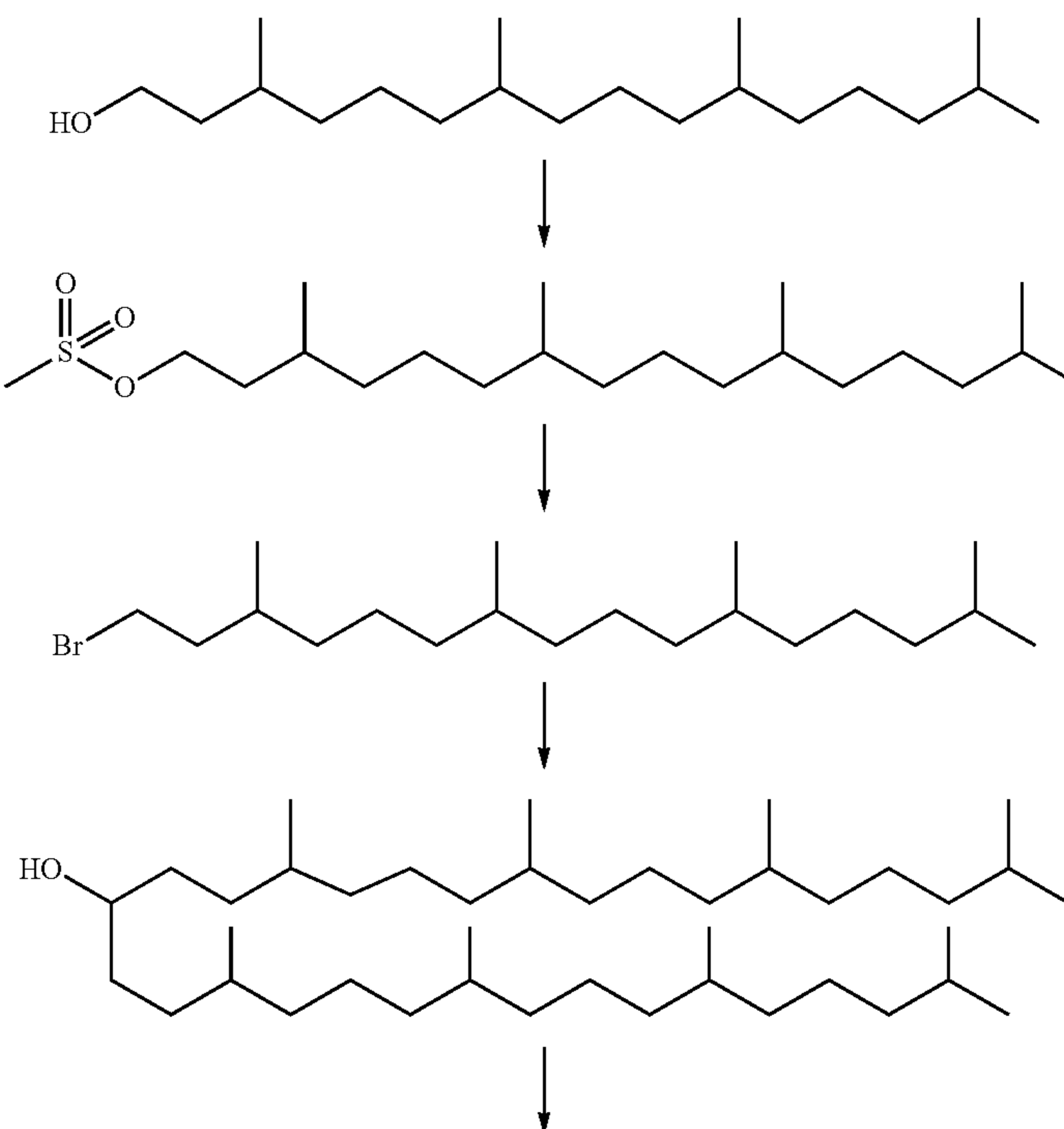
Scheme 12
