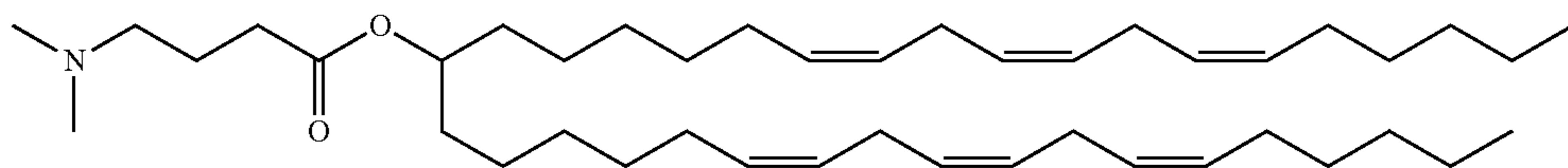
\gamma -LenMC3
