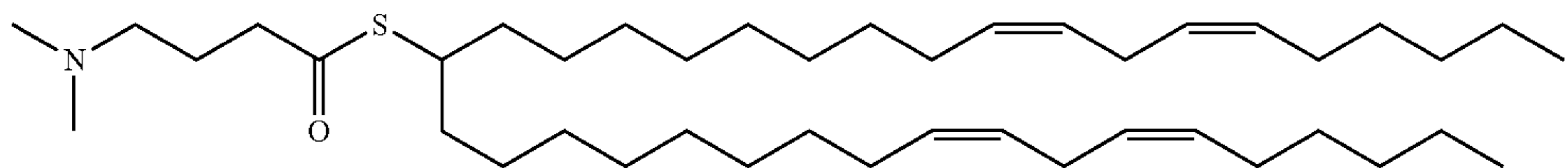
MC3 Thioester
