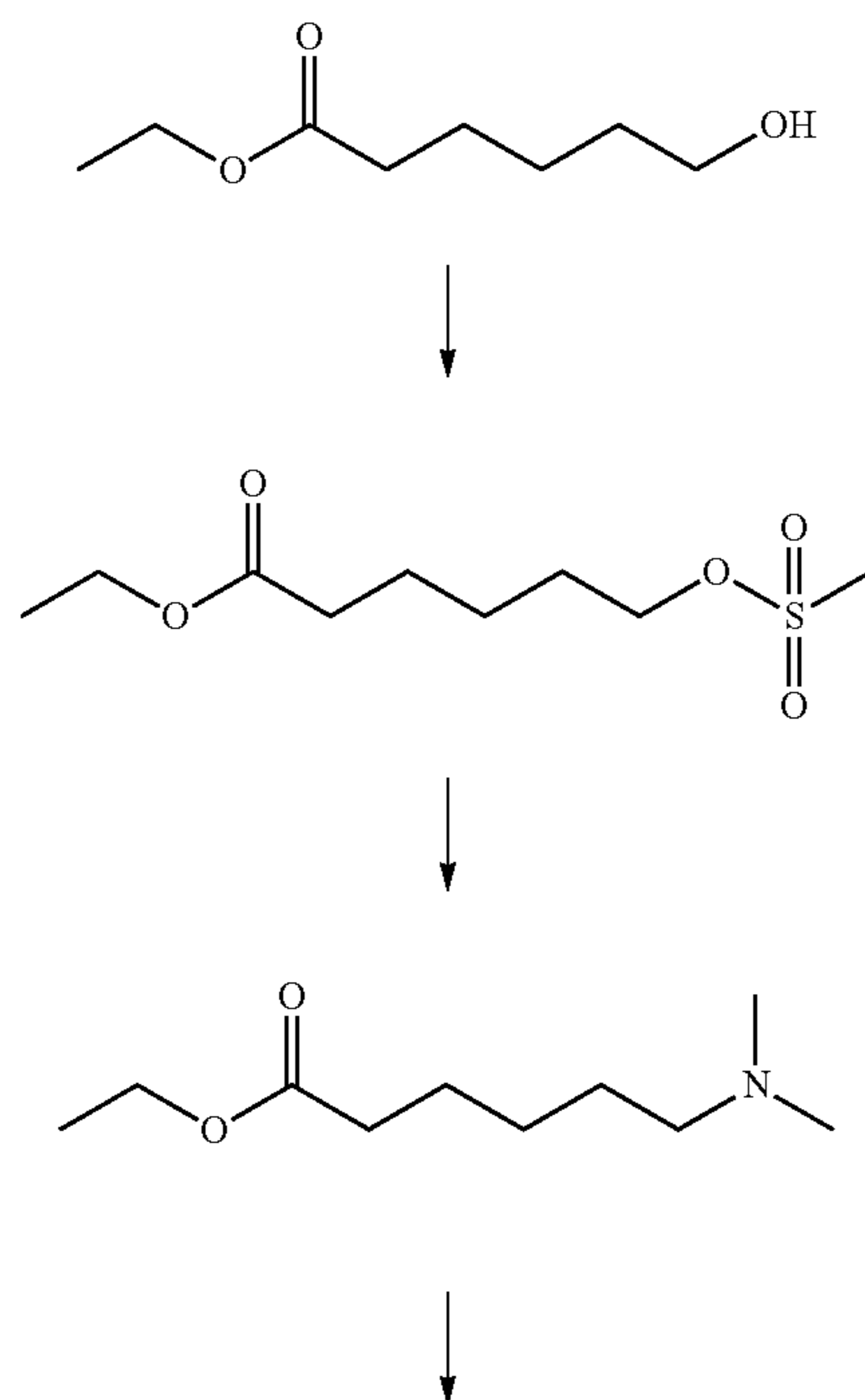
Scheme 14
