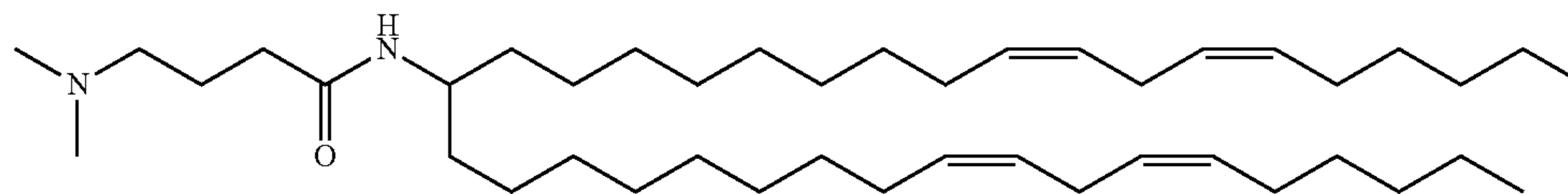
MC3 Amide
