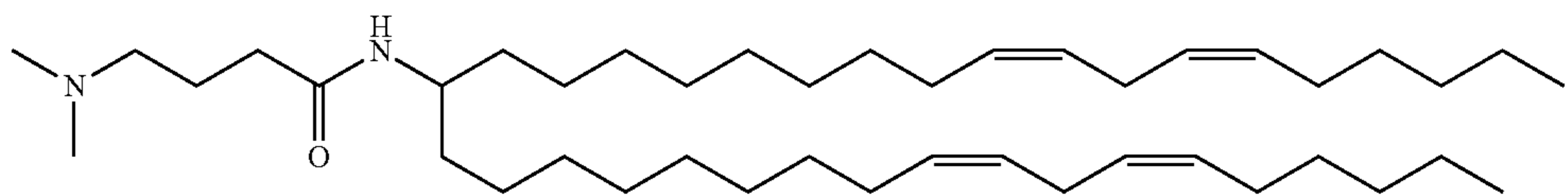
MC3 Amide
