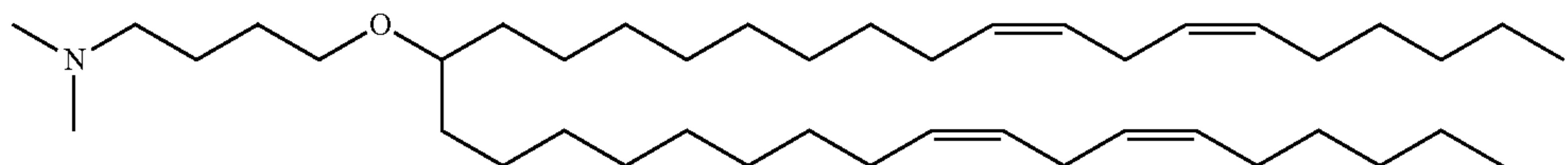
MC4 Ether
