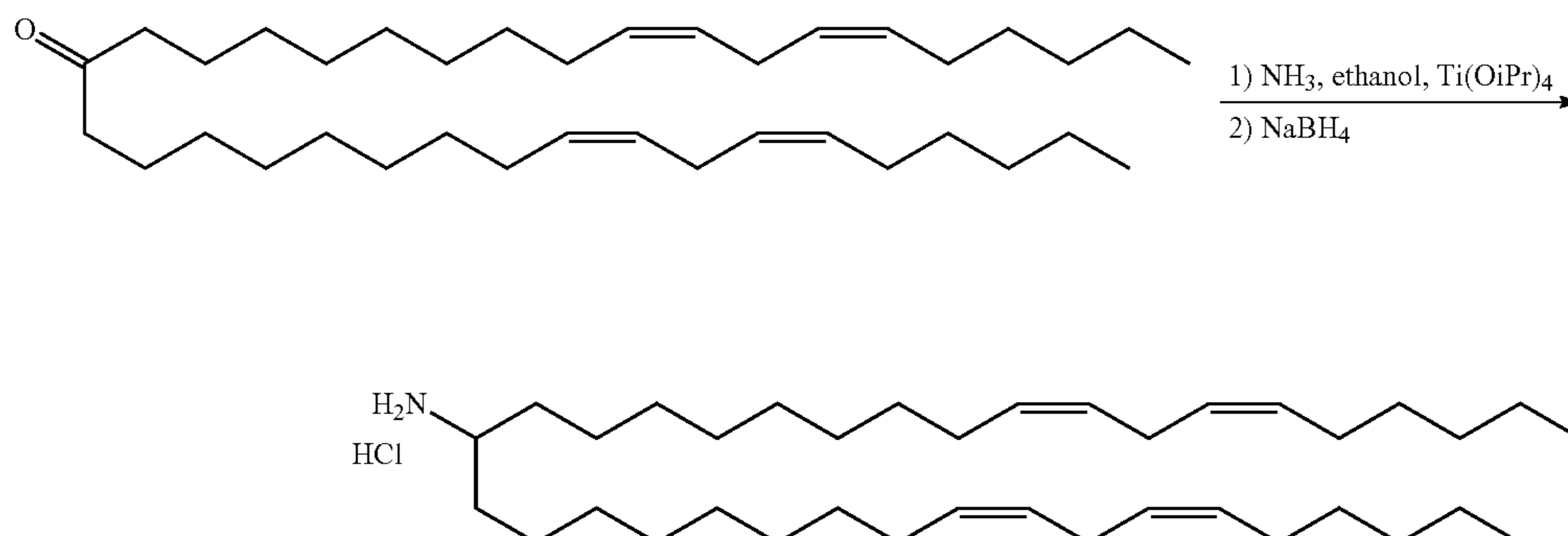
Scheme 10
