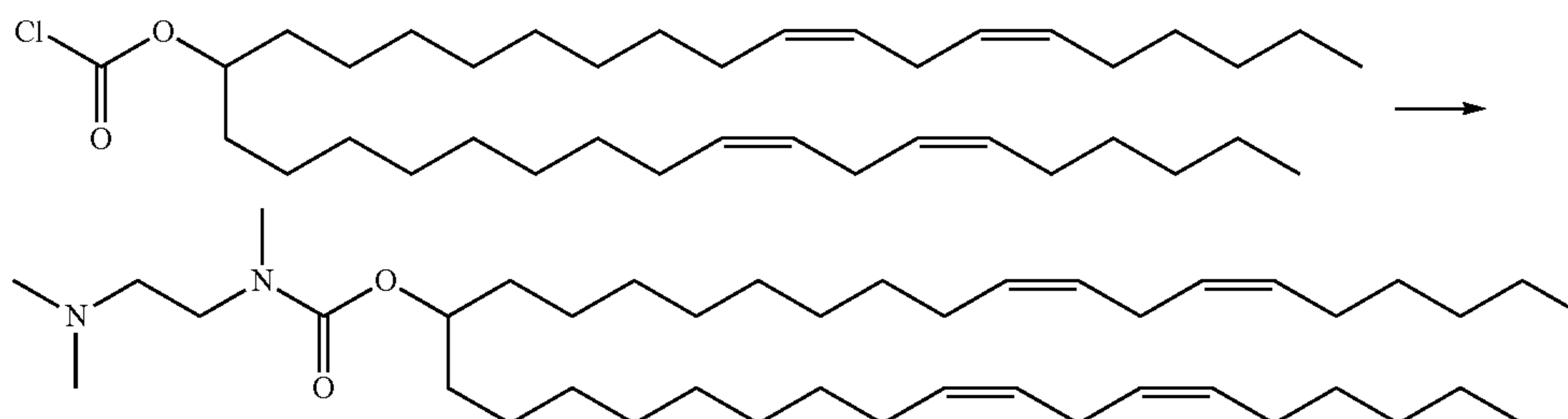
Scheme 6
