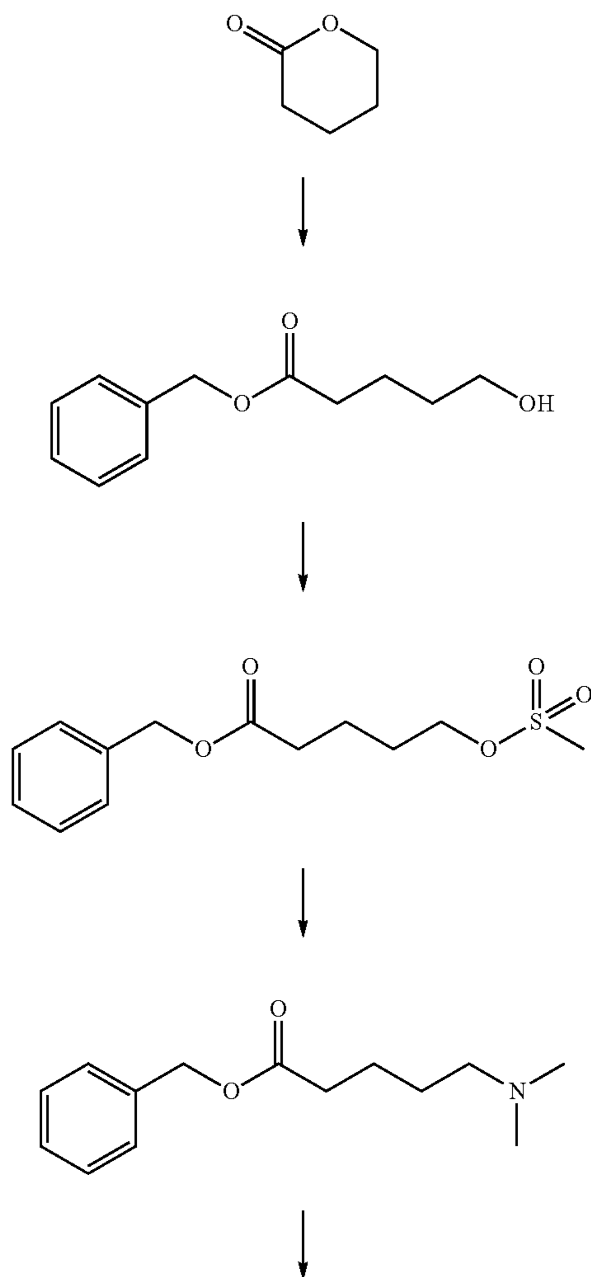
Scheme 13
