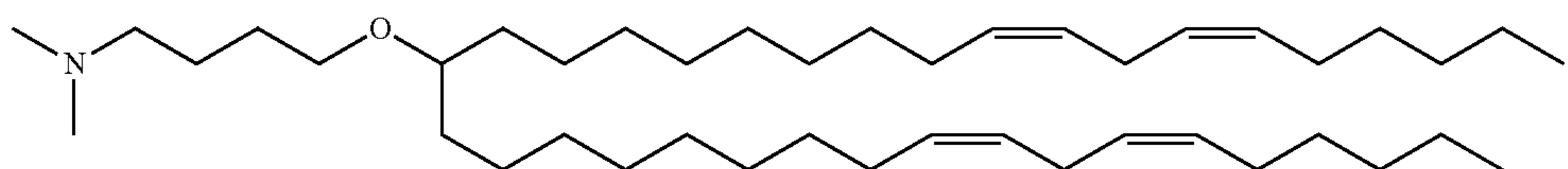
MC4 Ether
