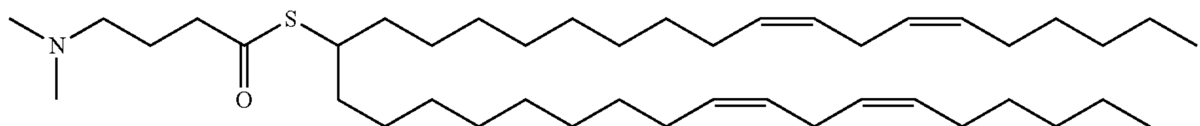
MC3 Thioester
