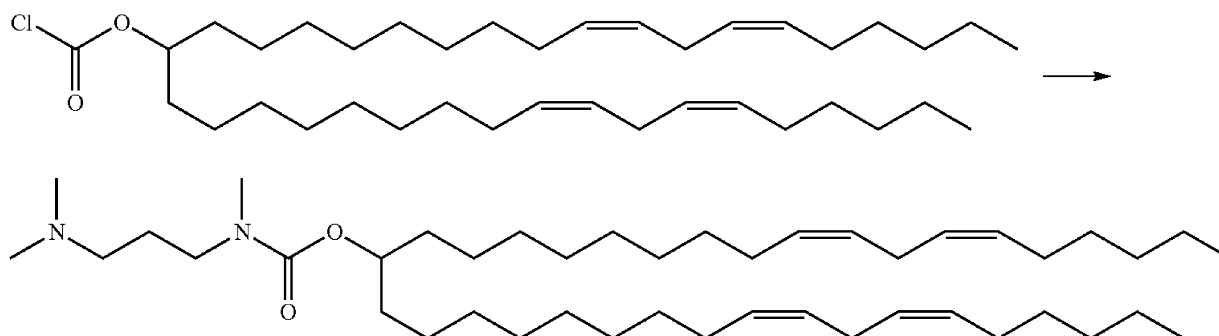
Scheme 5
