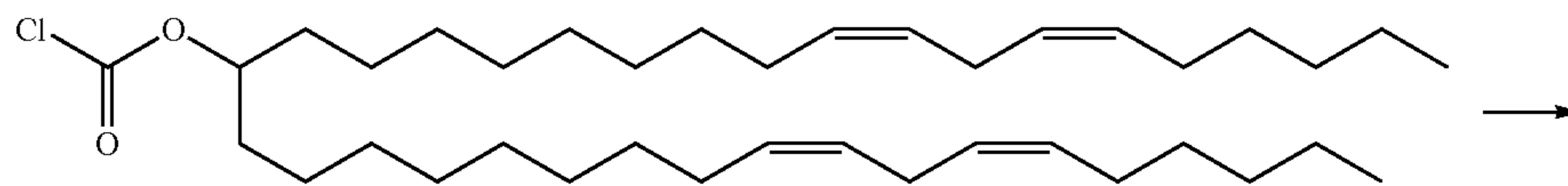
Scheme 7
