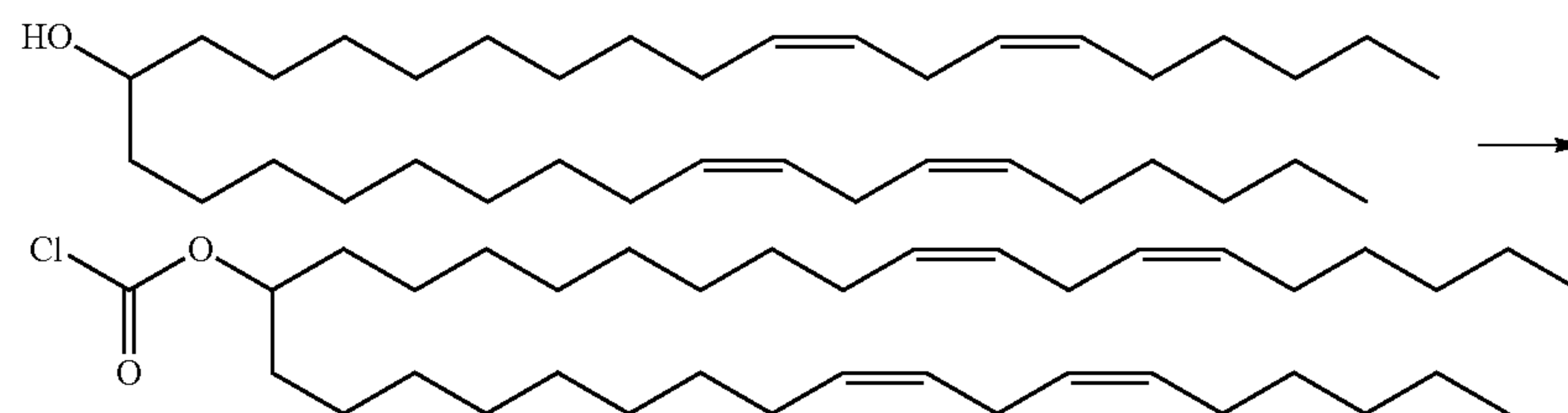
Scheme 4
