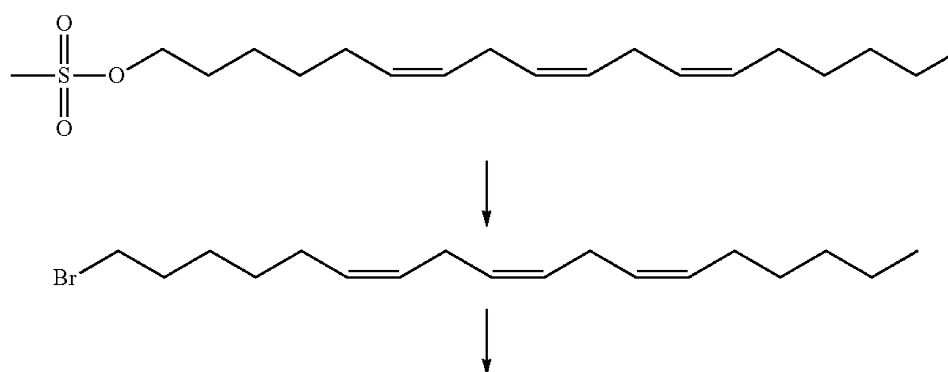
Scheme 3
