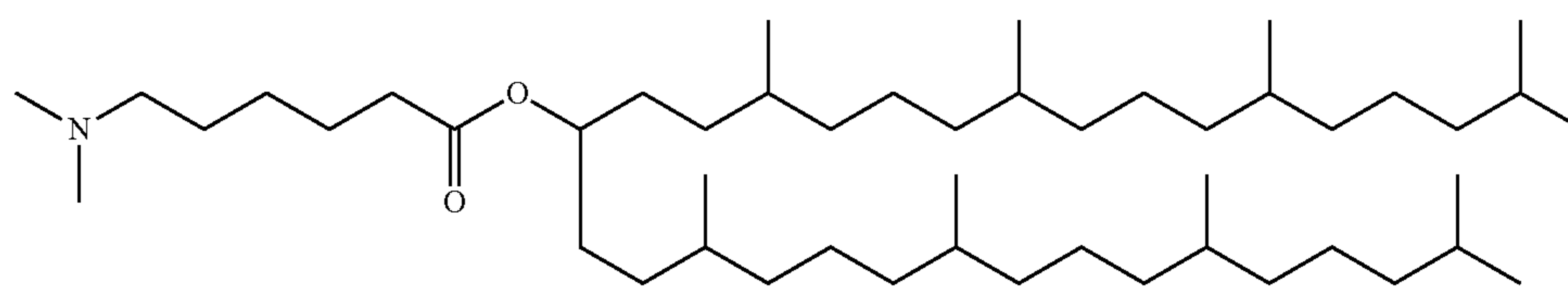
Pan-MC5
