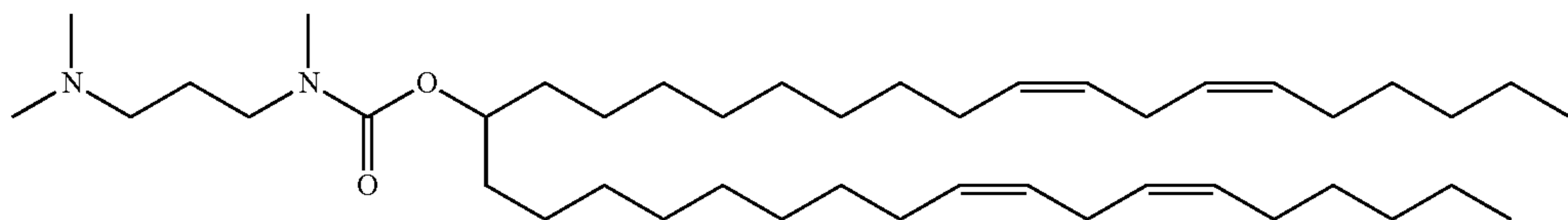
MC3MC
