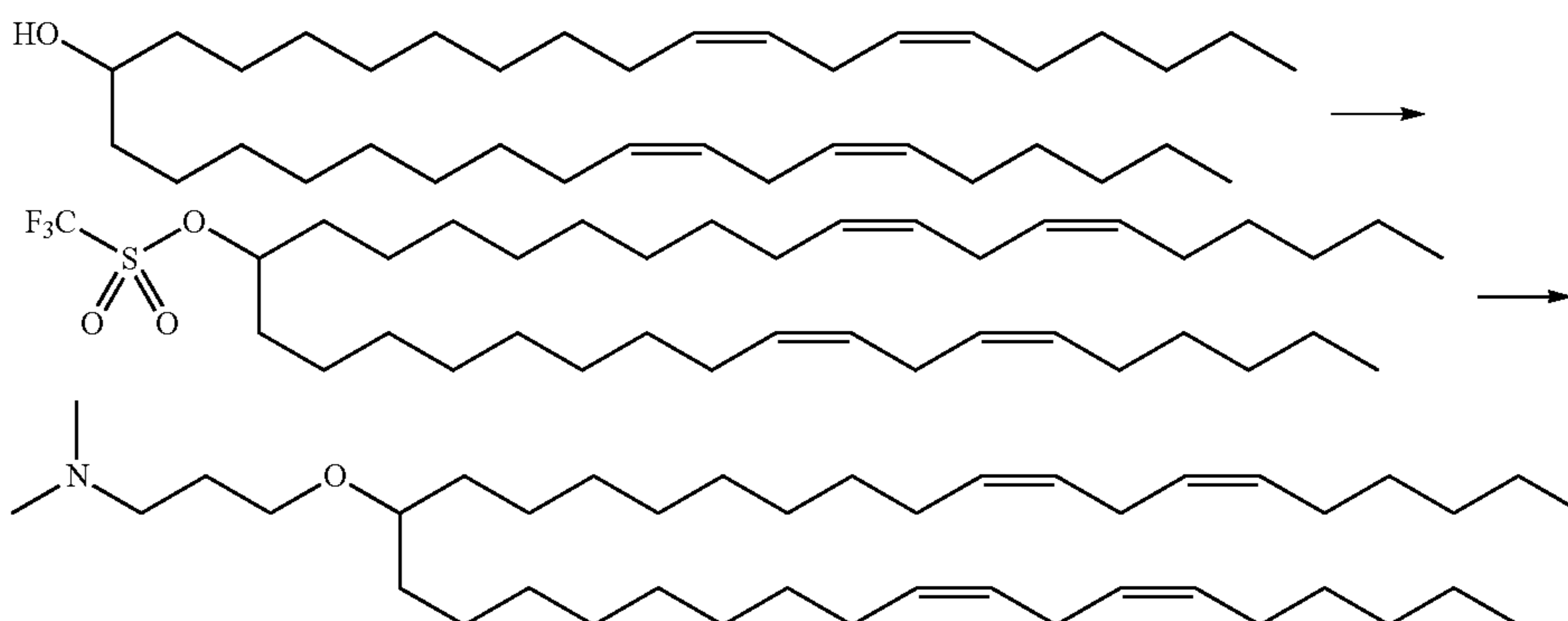
Scheme 8
