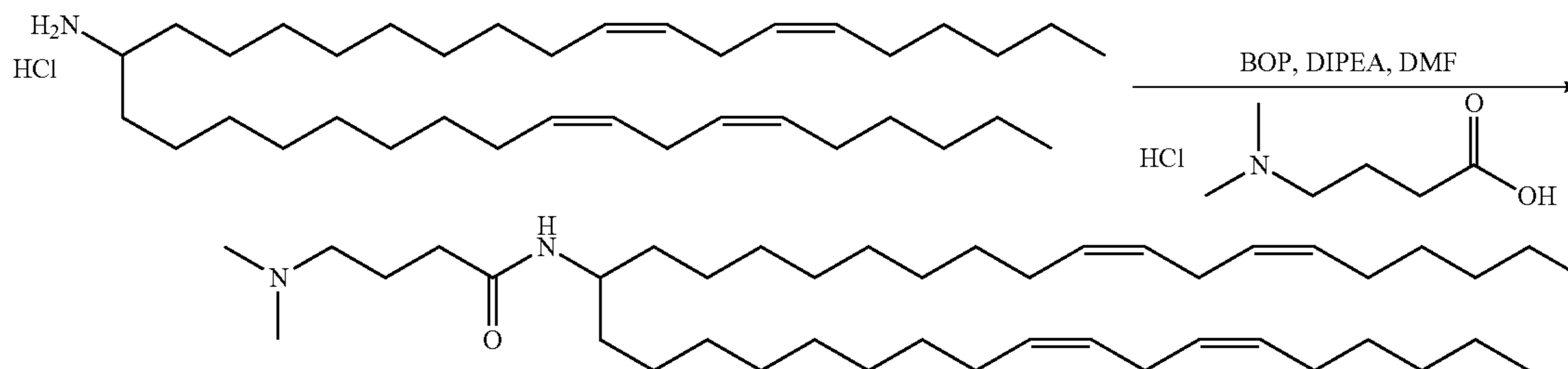
Scheme 11
