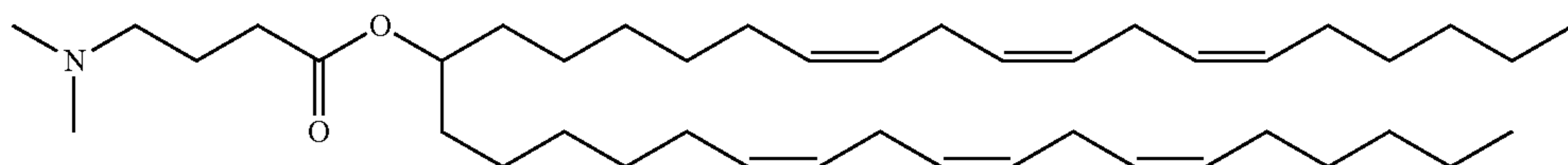
\gamma -LenMC3
