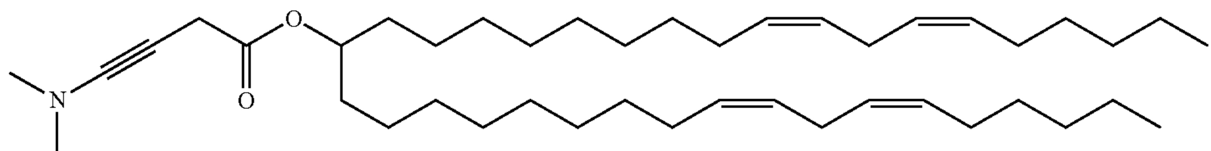
MC3 Alkyne
