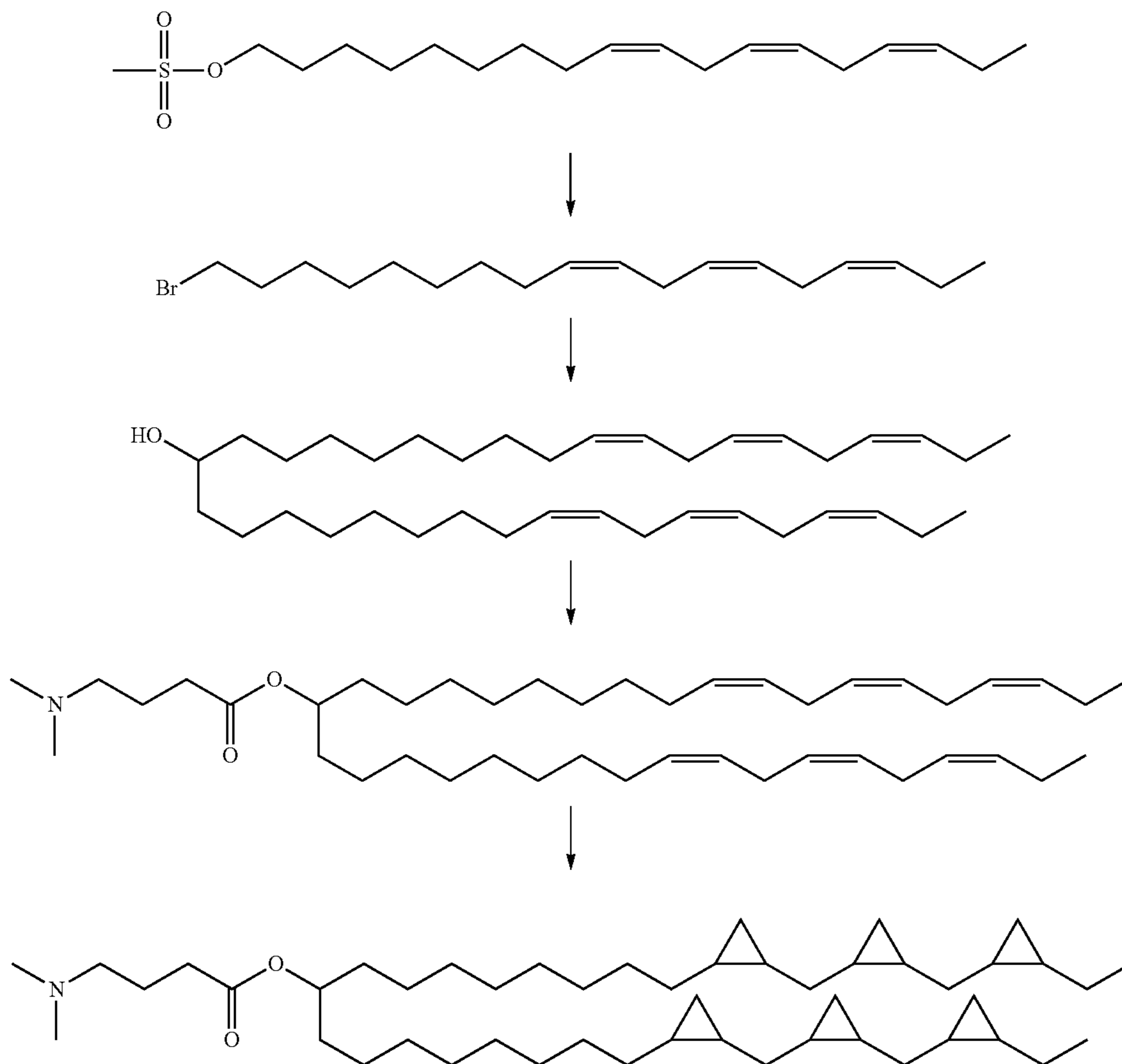
Scheme 2
