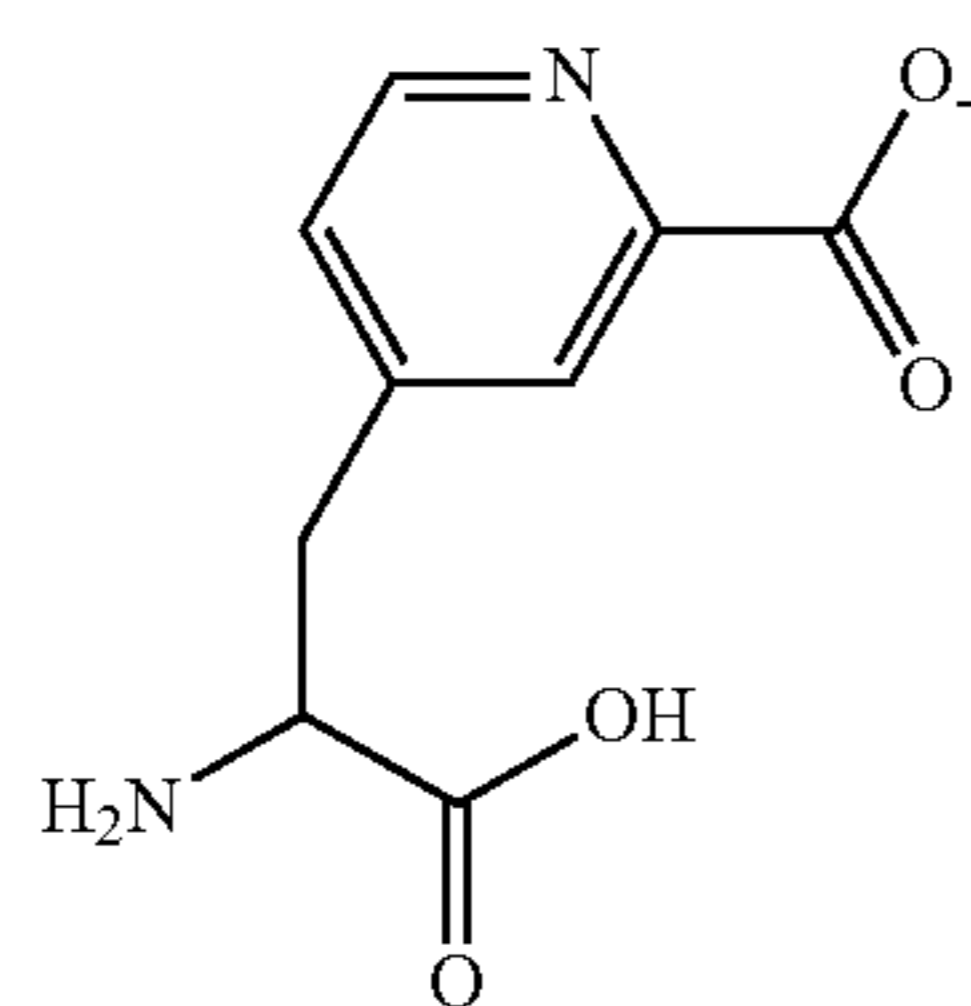
(2-carboxy-4-pyridyl)-DL-alanine
