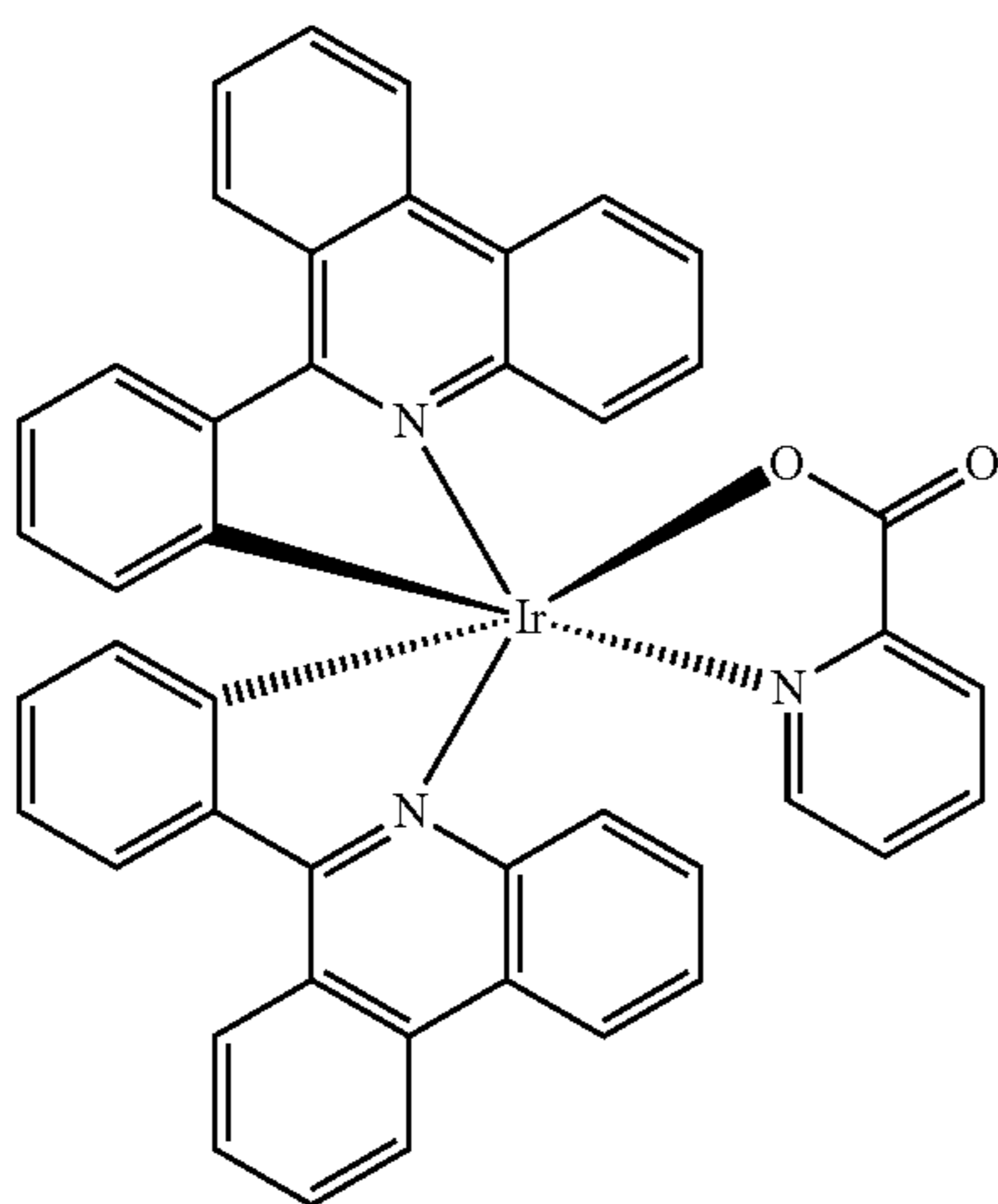
\text{Ir}(\text{6-phenylphenanthridine})_2 pyridine-2-carboxylic acid
