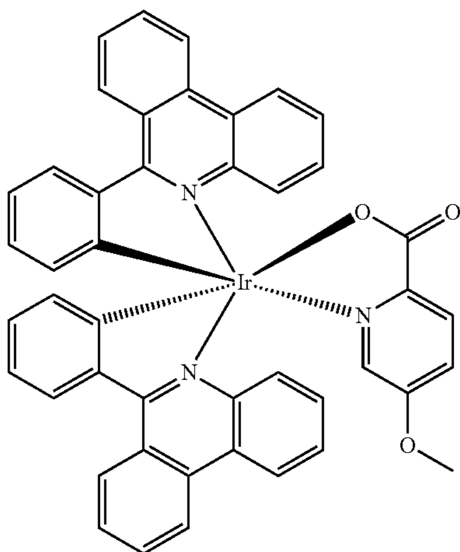
\text{Ir}(\text{6-phenylphenanthridine})_2 5-(methoxy)pyridine-2-carboxylic acid
