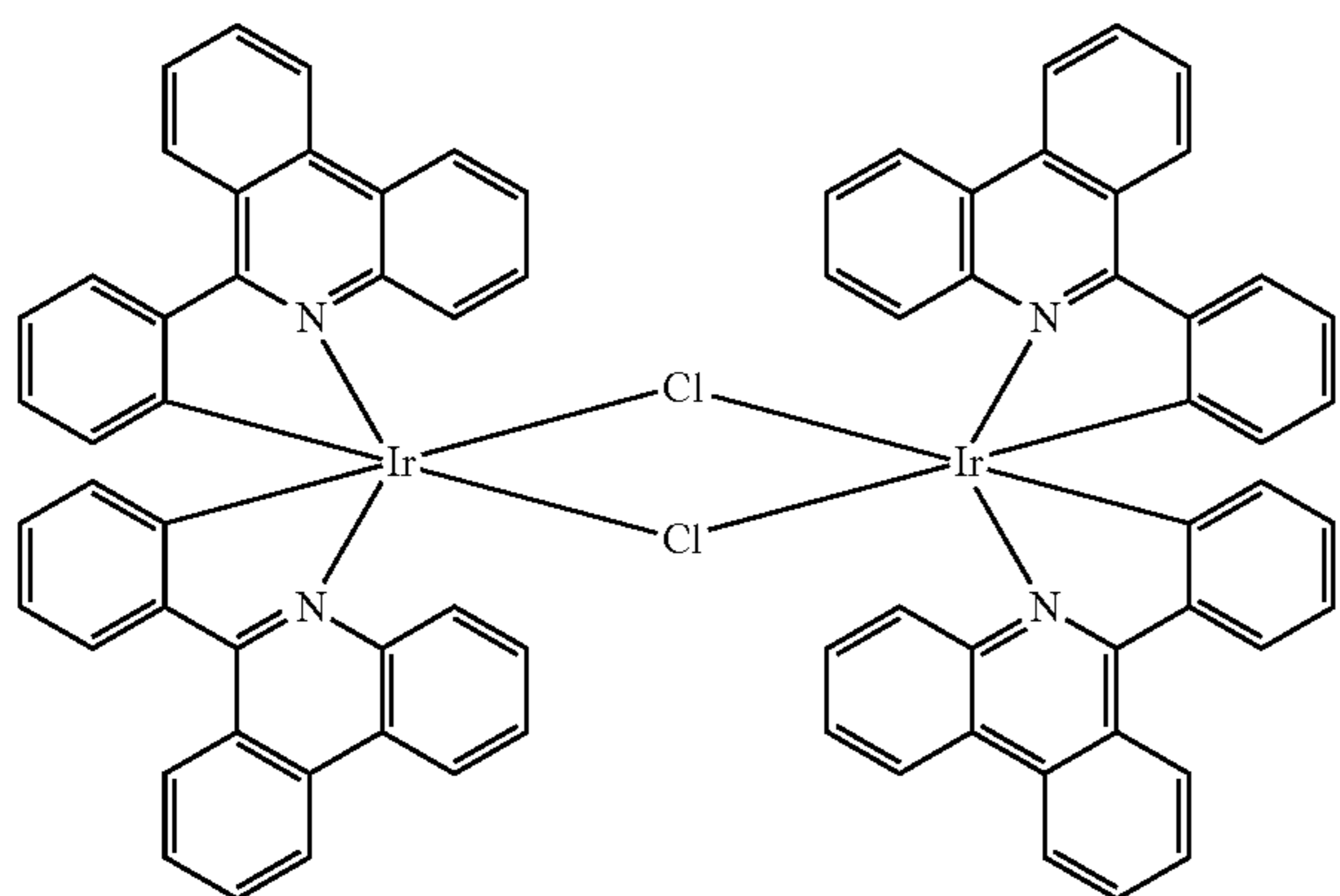
[(6\text{-phenylphenanthridine})_2\text{IrCl}]_2
