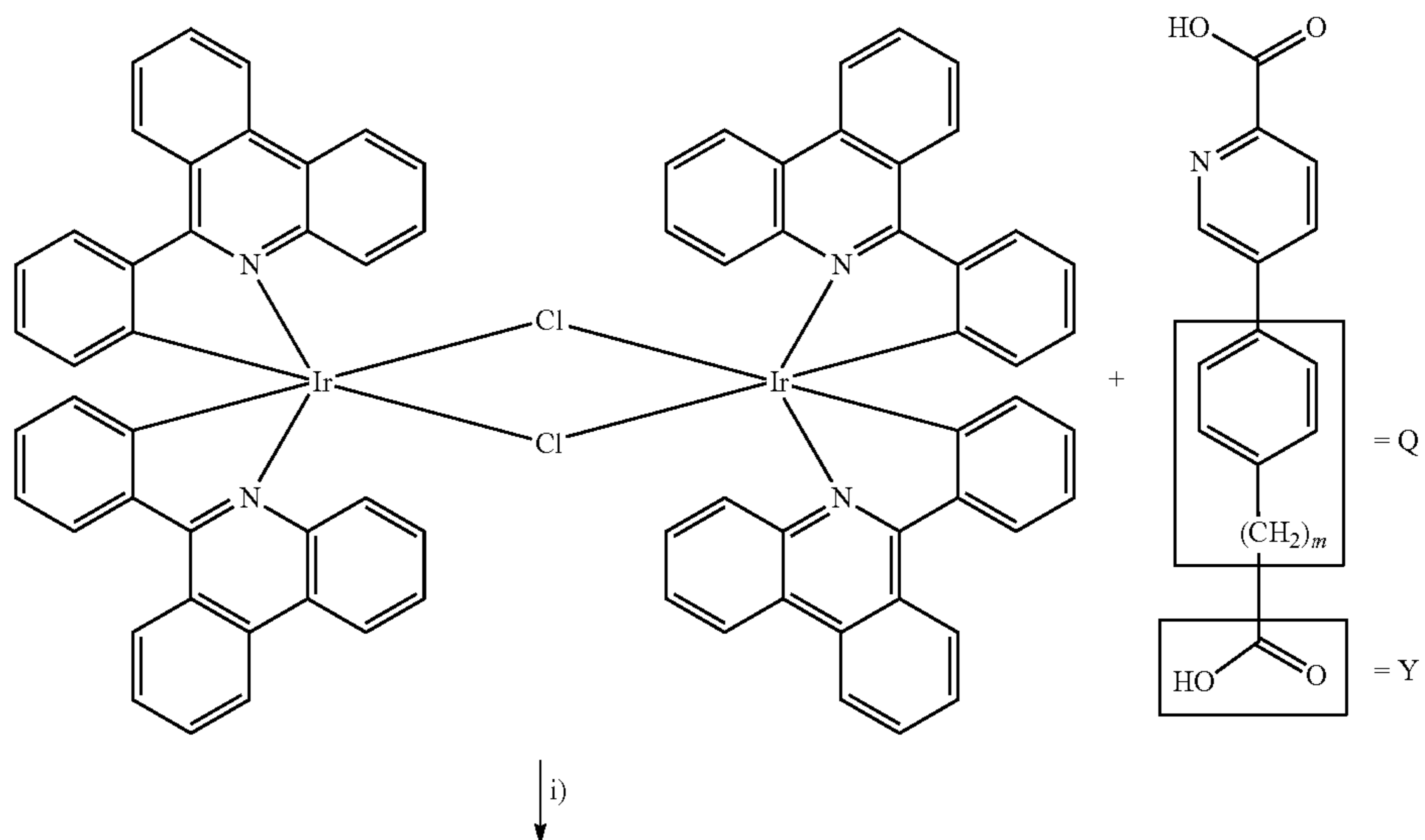
Scheme 1: Synthesis of a compound of Formula I.
