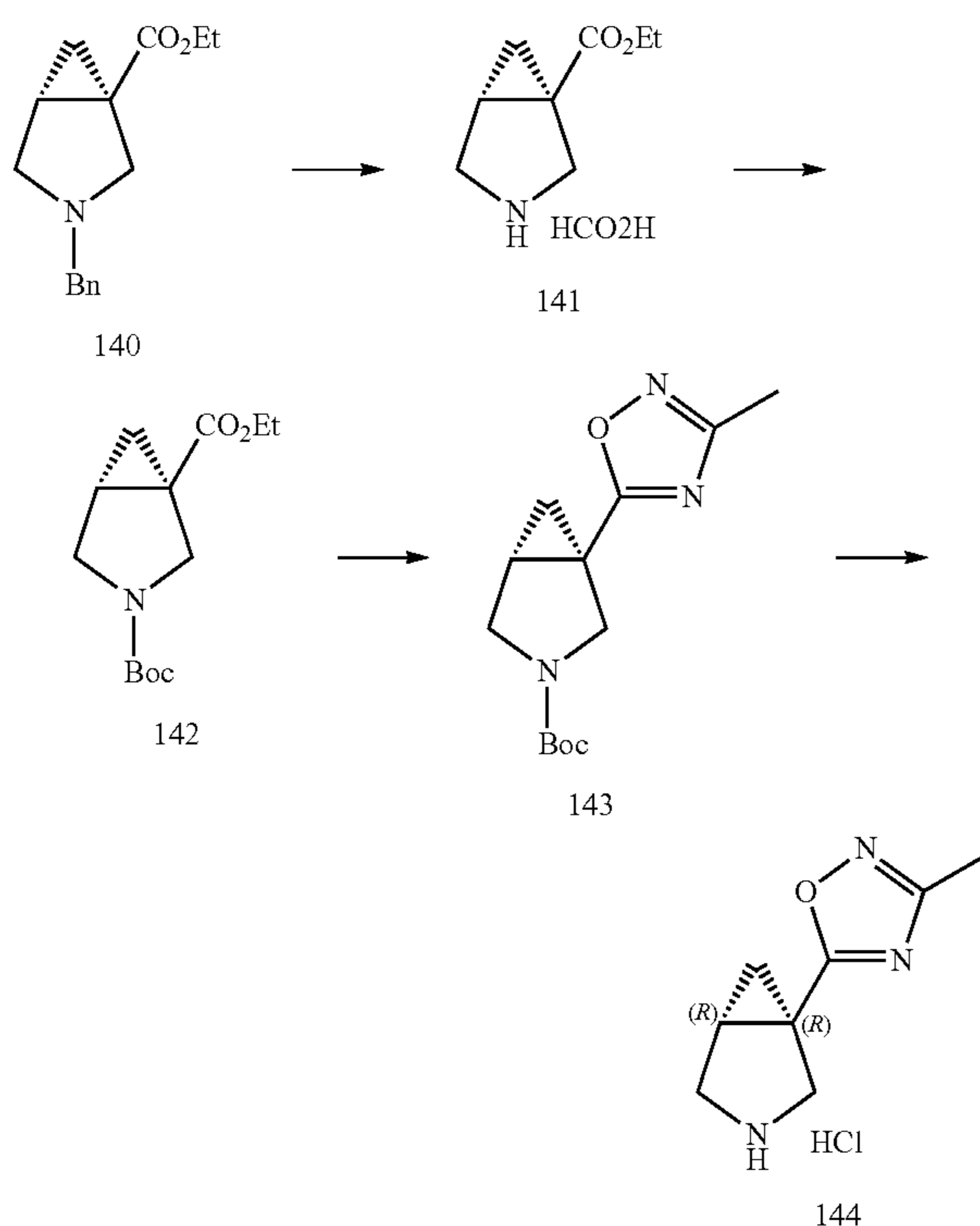
Scheme 104: Enantiospecific synthesis of azabicyclo compounds.
