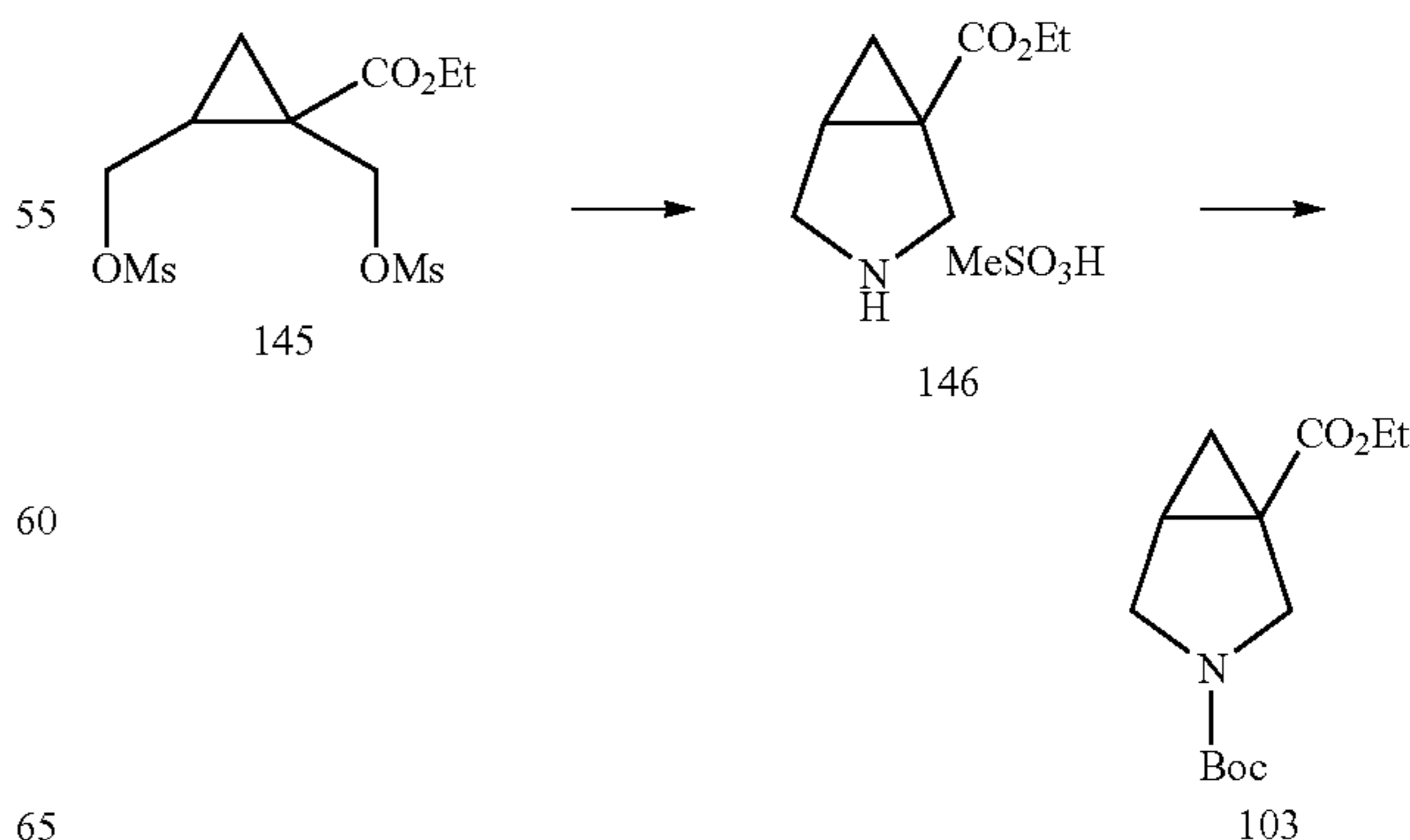
Scheme 105: Direct formation of N-H azabicyclo compound with ammonia.
