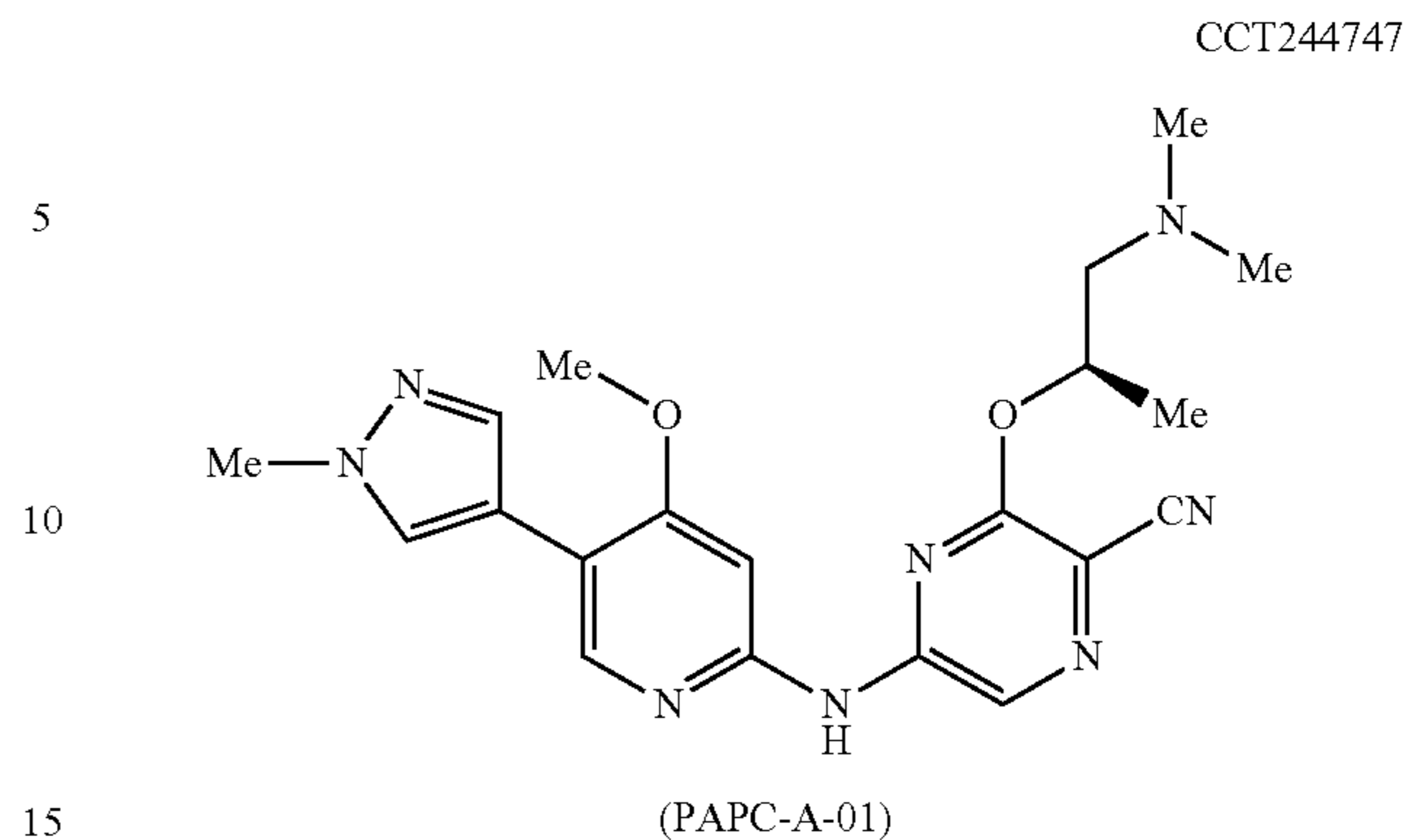
Compound 7i
