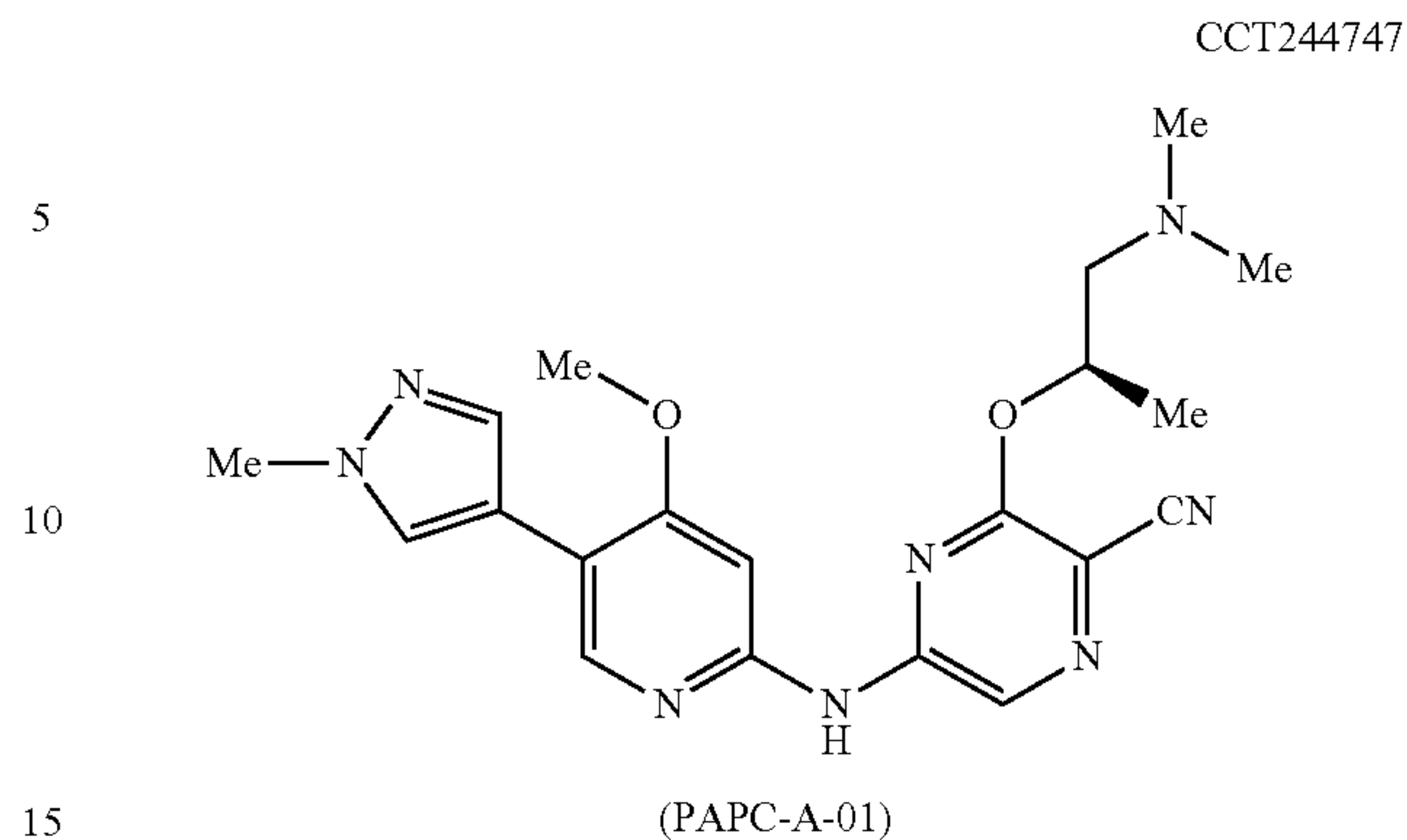
Compound 7i
