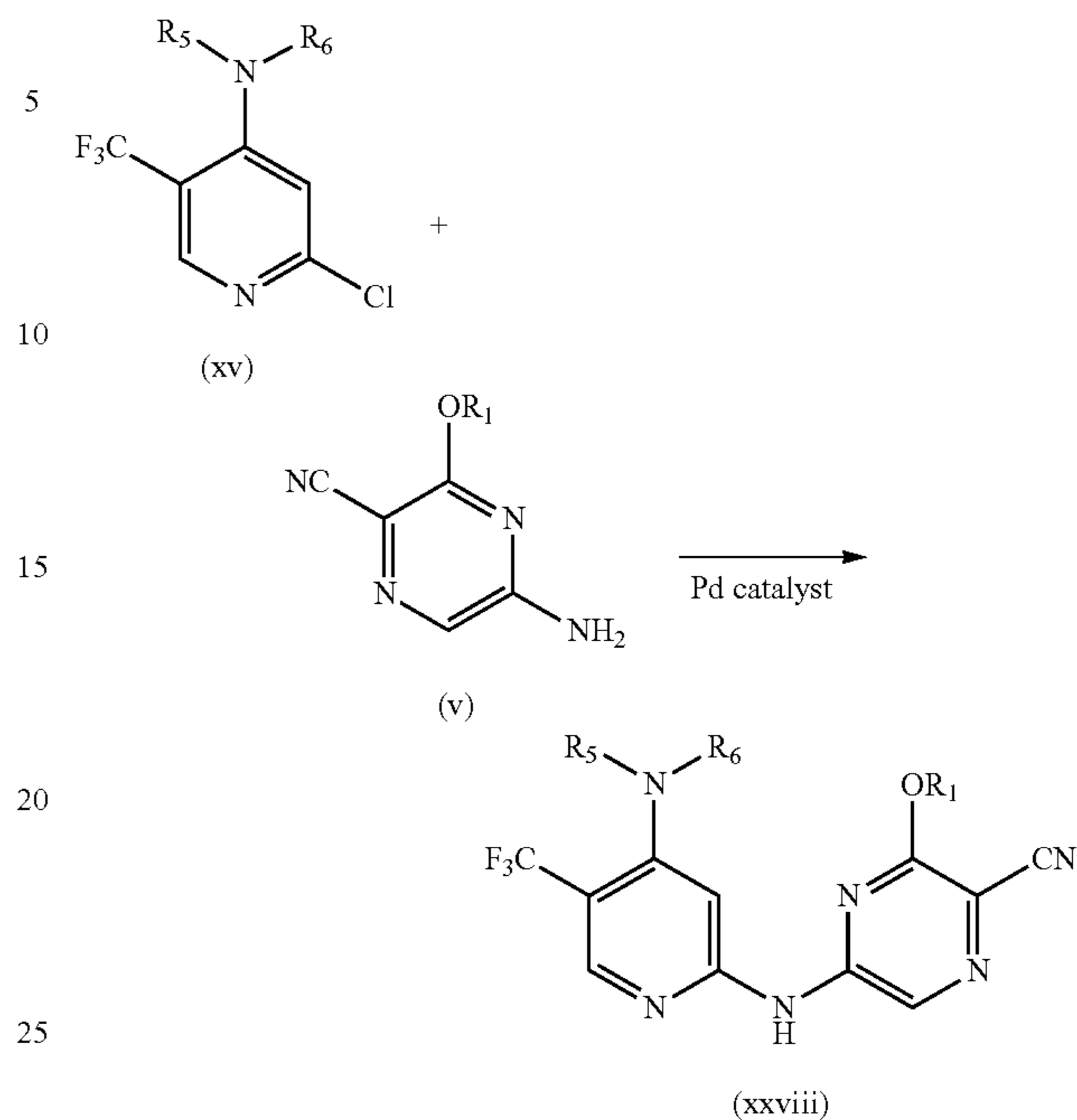
Scheme 12
