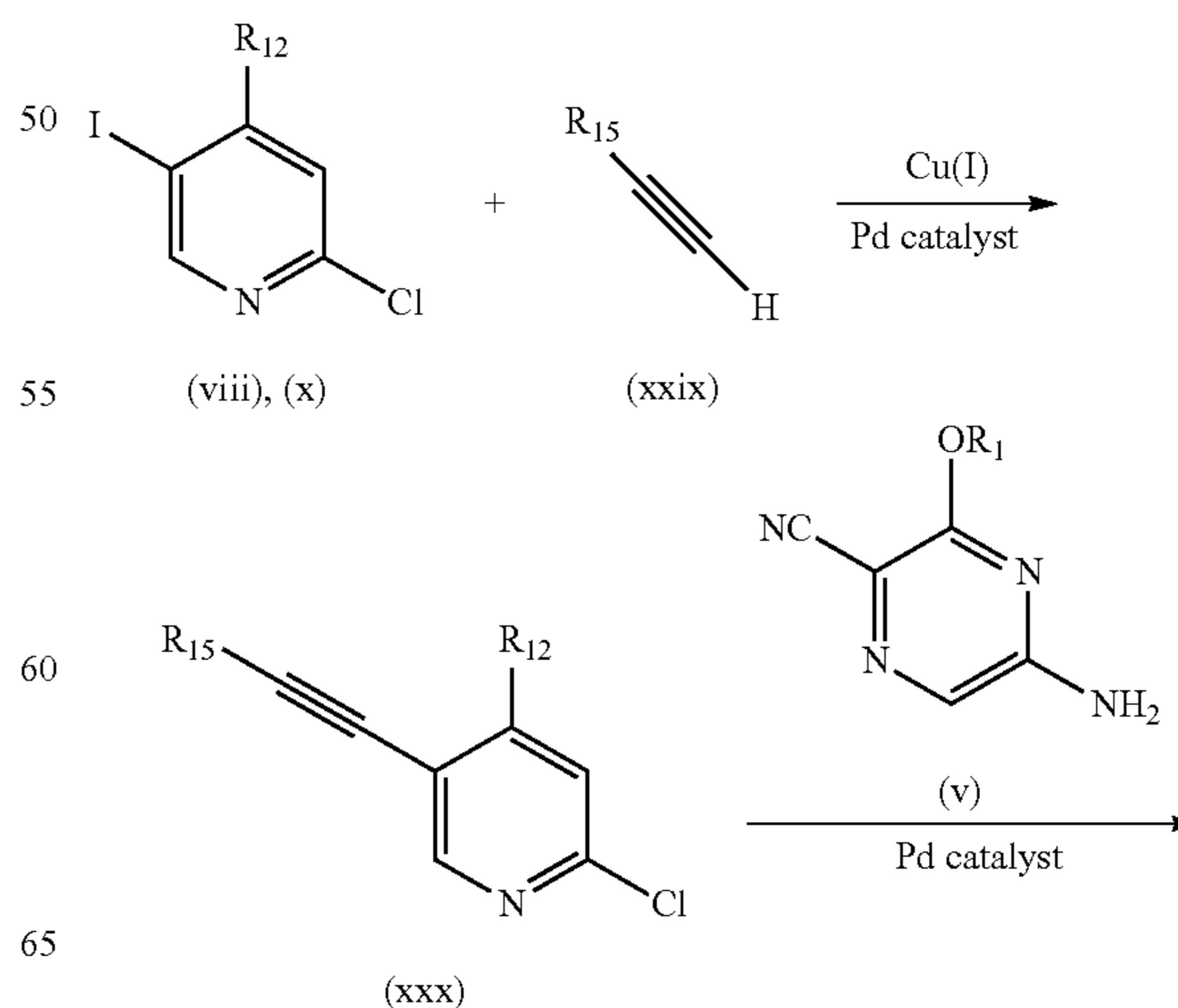
Scheme 13
