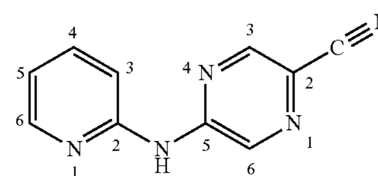
5-(Pyridin-2-yl-amino)-pyrazine-2-carbonitrile
