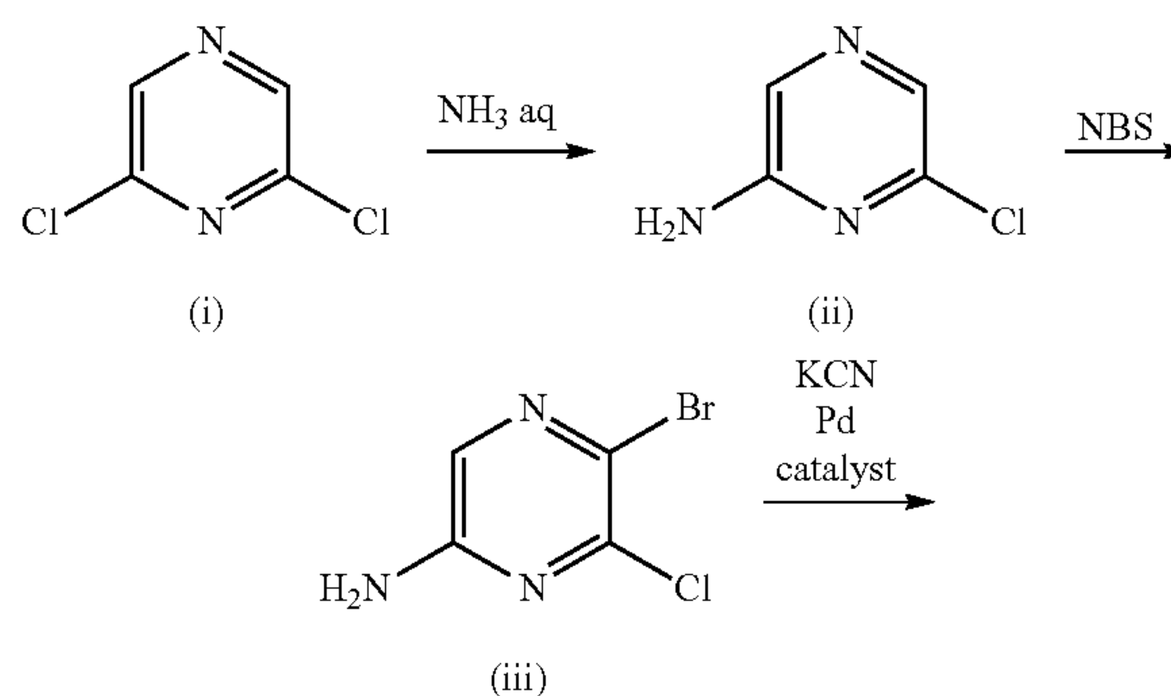
Scheme 1
