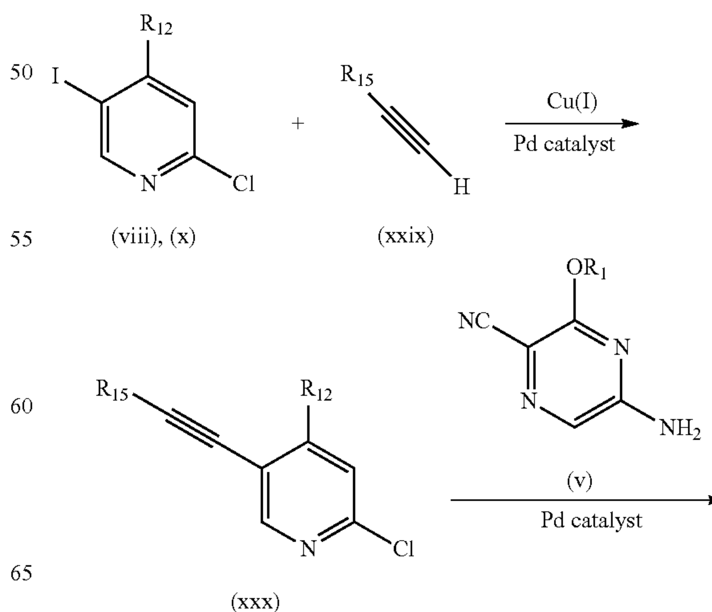
Scheme 13
