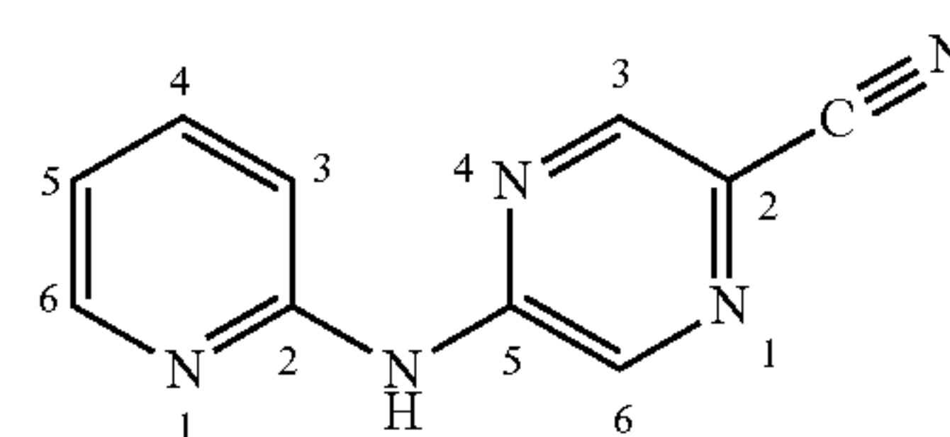
5-(Pyridin-2-yl-amino)-pyrazine-2-carbonitrile
