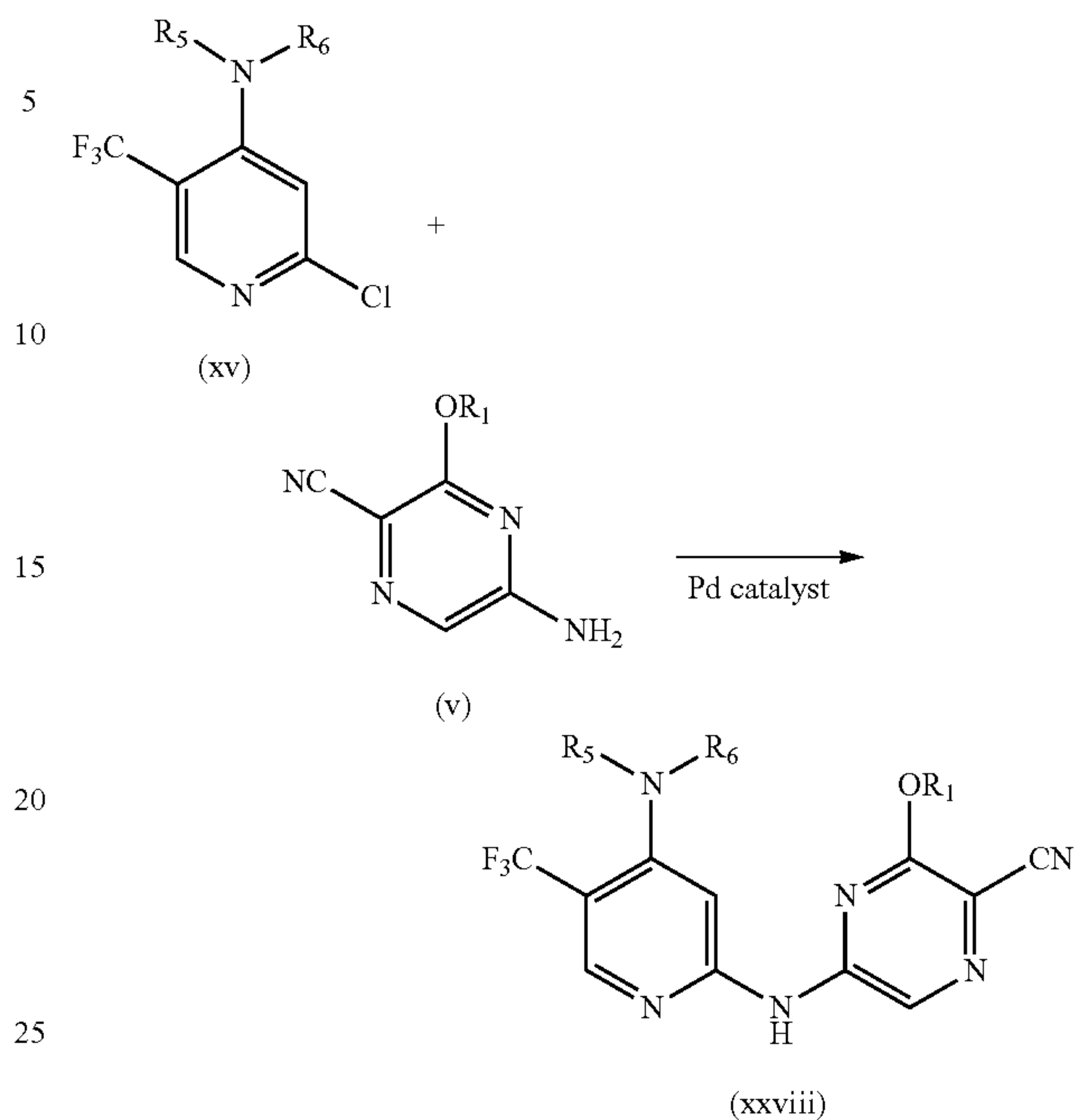
Scheme 12
