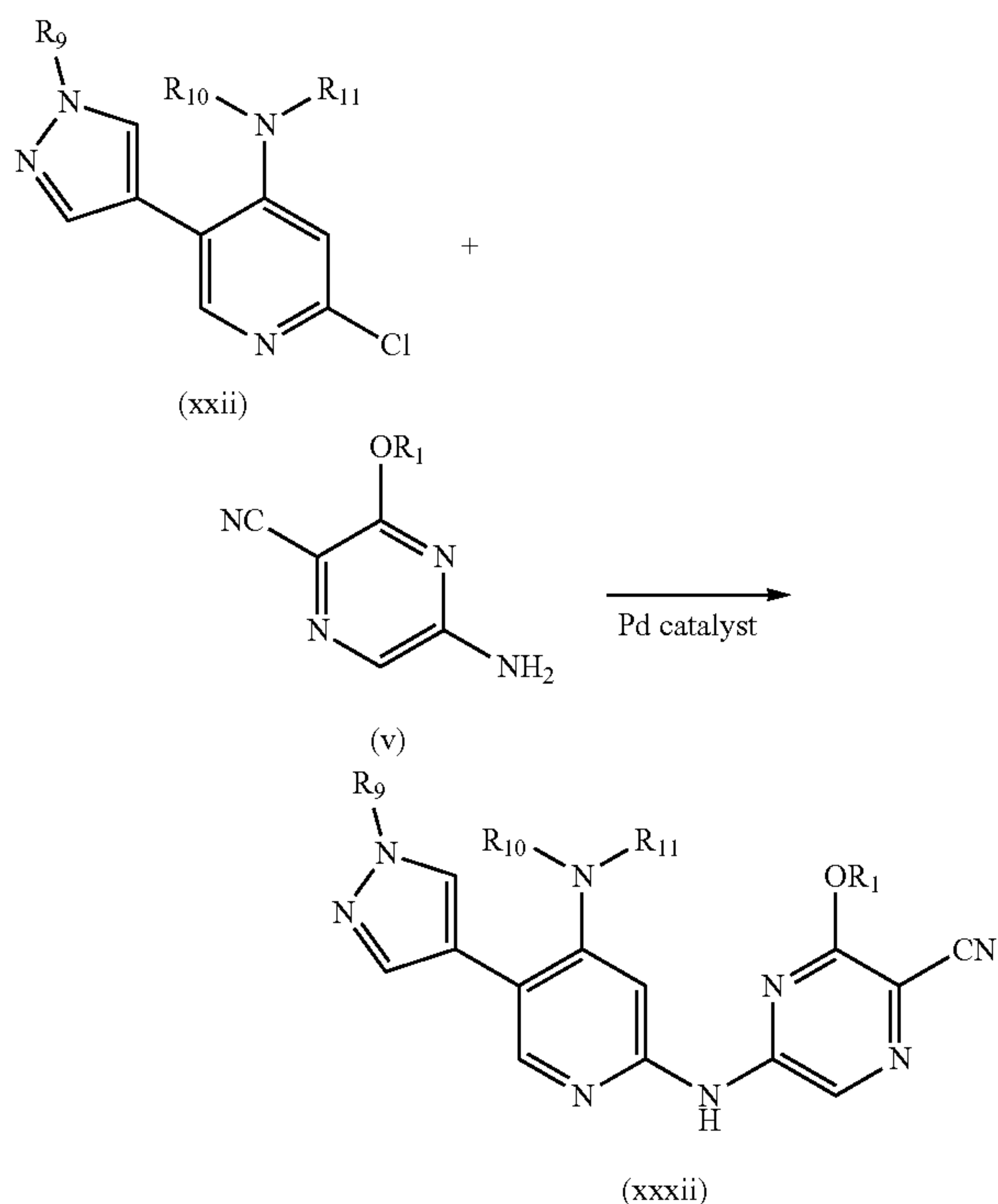
Scheme 14
