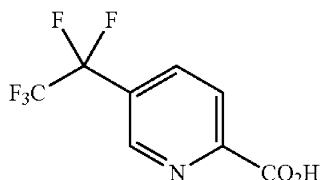
5-pentafluoropyridin-2-carboxylic acid
