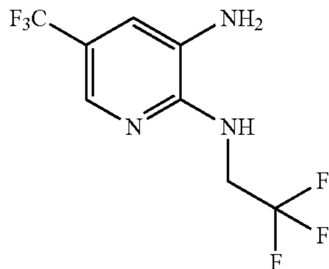
N 2 -(2,2,2-trifluoroethyl)-5-trifluoromethylpyridin-2,3-diamine
