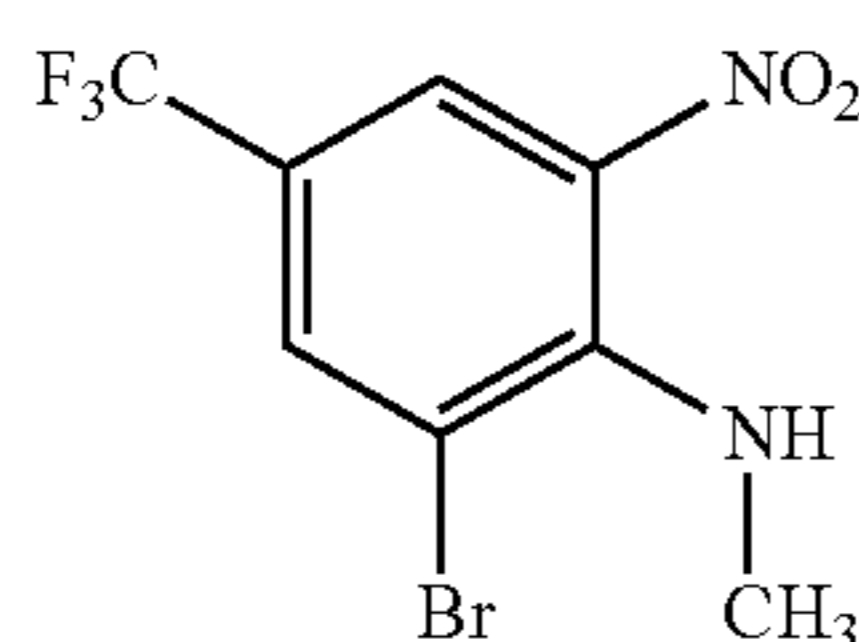
(2-bromo-6-nitro-4-trifluoromethyl-phenyl)-methyl-amine
