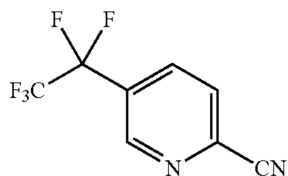
2-cyano-5-pentafluoroethyl pyridine
