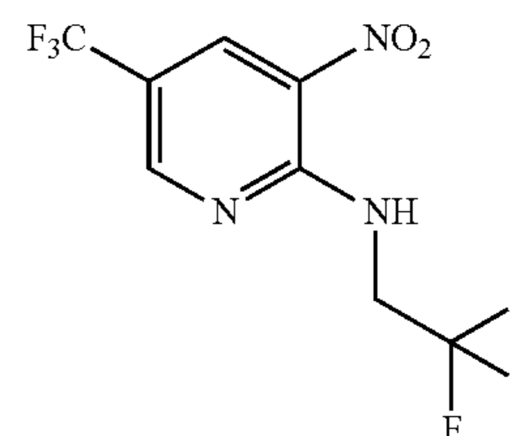
(3-nitro-5-trifluoromethylpyridin-2-yl)-(2,2,2-trifluoroethyl)amine
