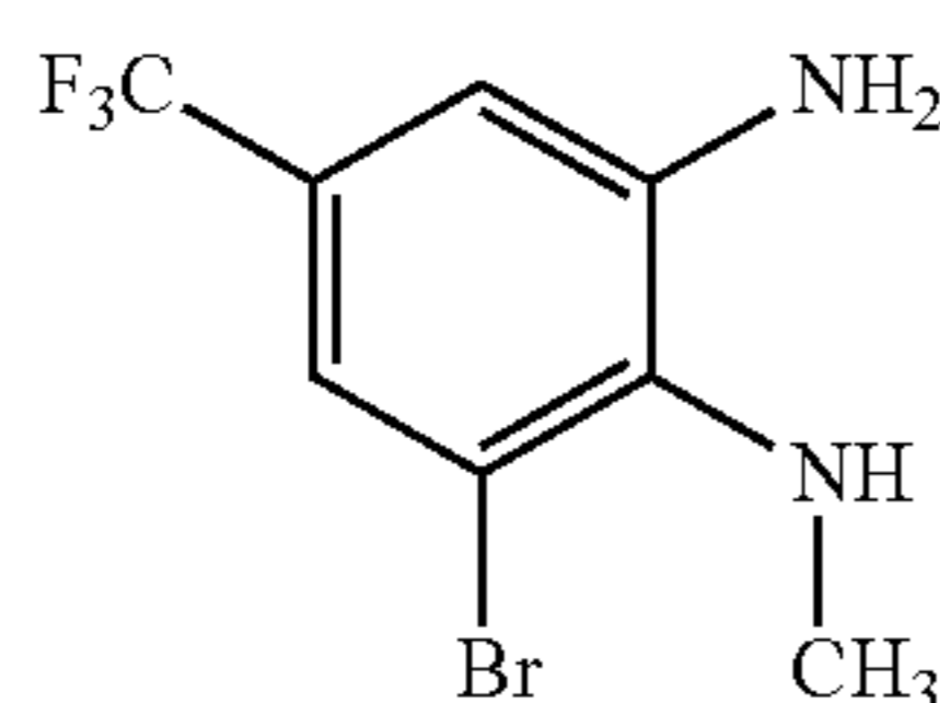
3-bromo-N 2 -methyl-5-trifluoromethyl-benzene-1,2-diamine
