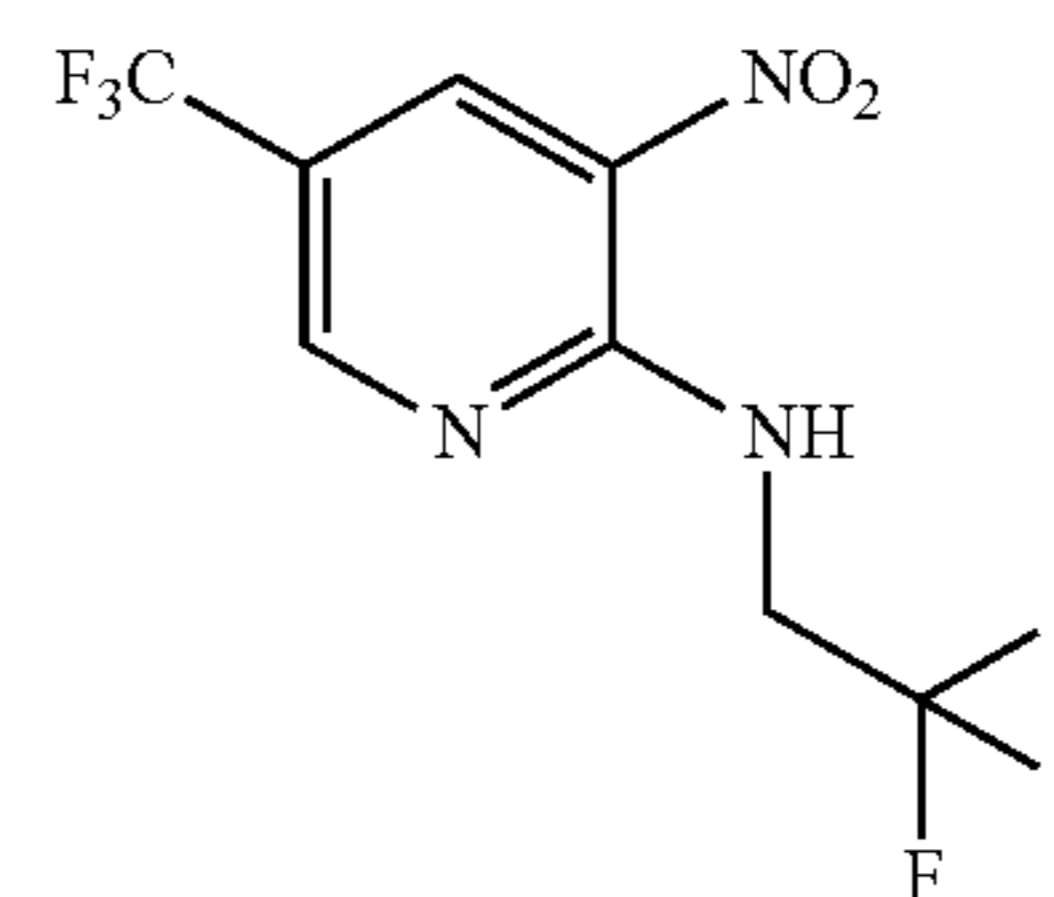
(3-nitro-5-trifluoromethylpyridin-2-yl)-(2,2,2-trifluoroethyl)amine
