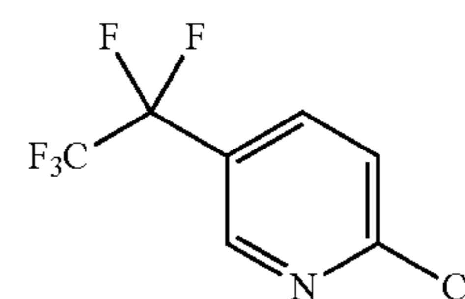
2-chloro-5-pentafluoroethyl pyridine
