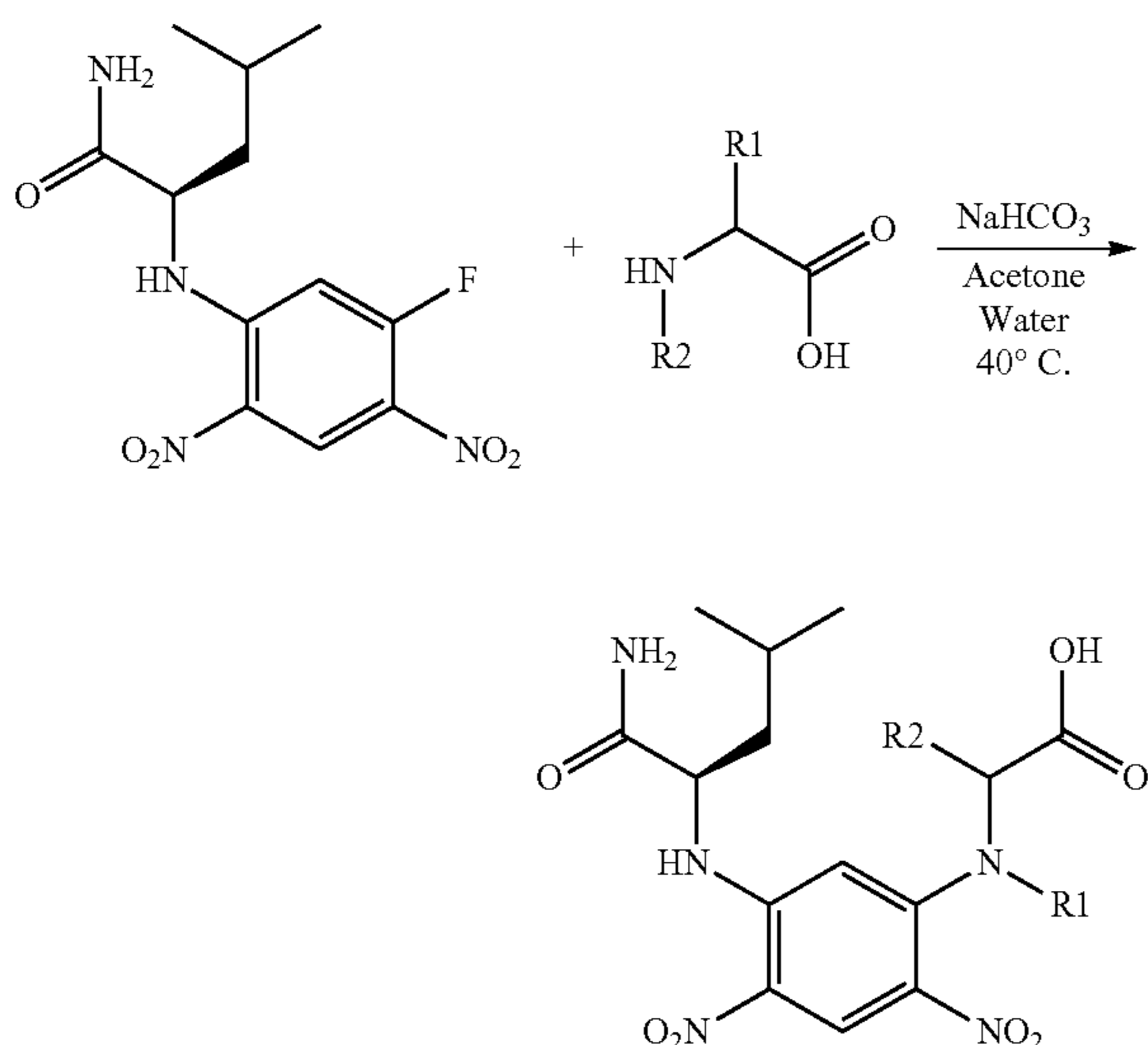
Scheme 5
