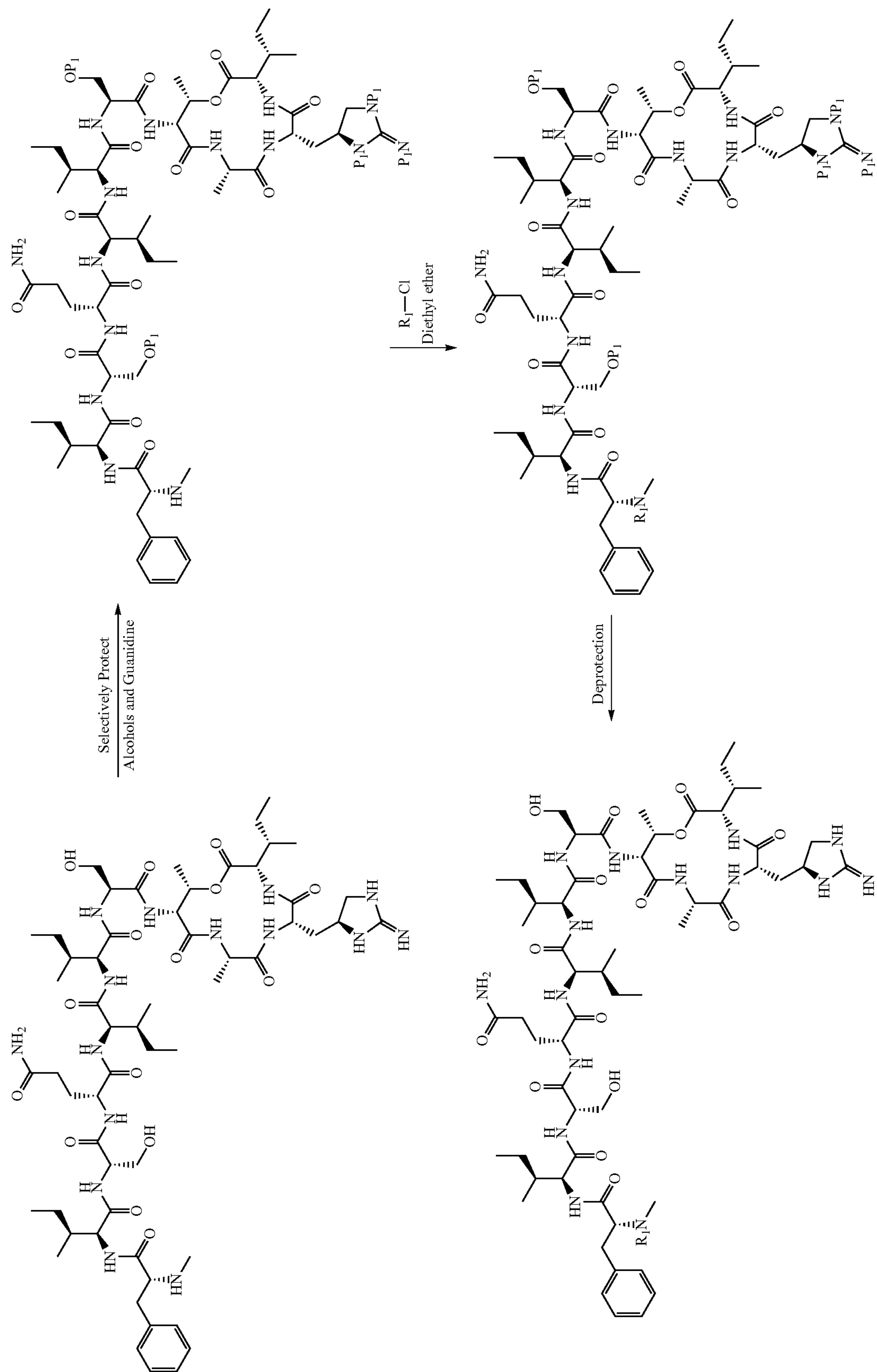
Scheme 2.
