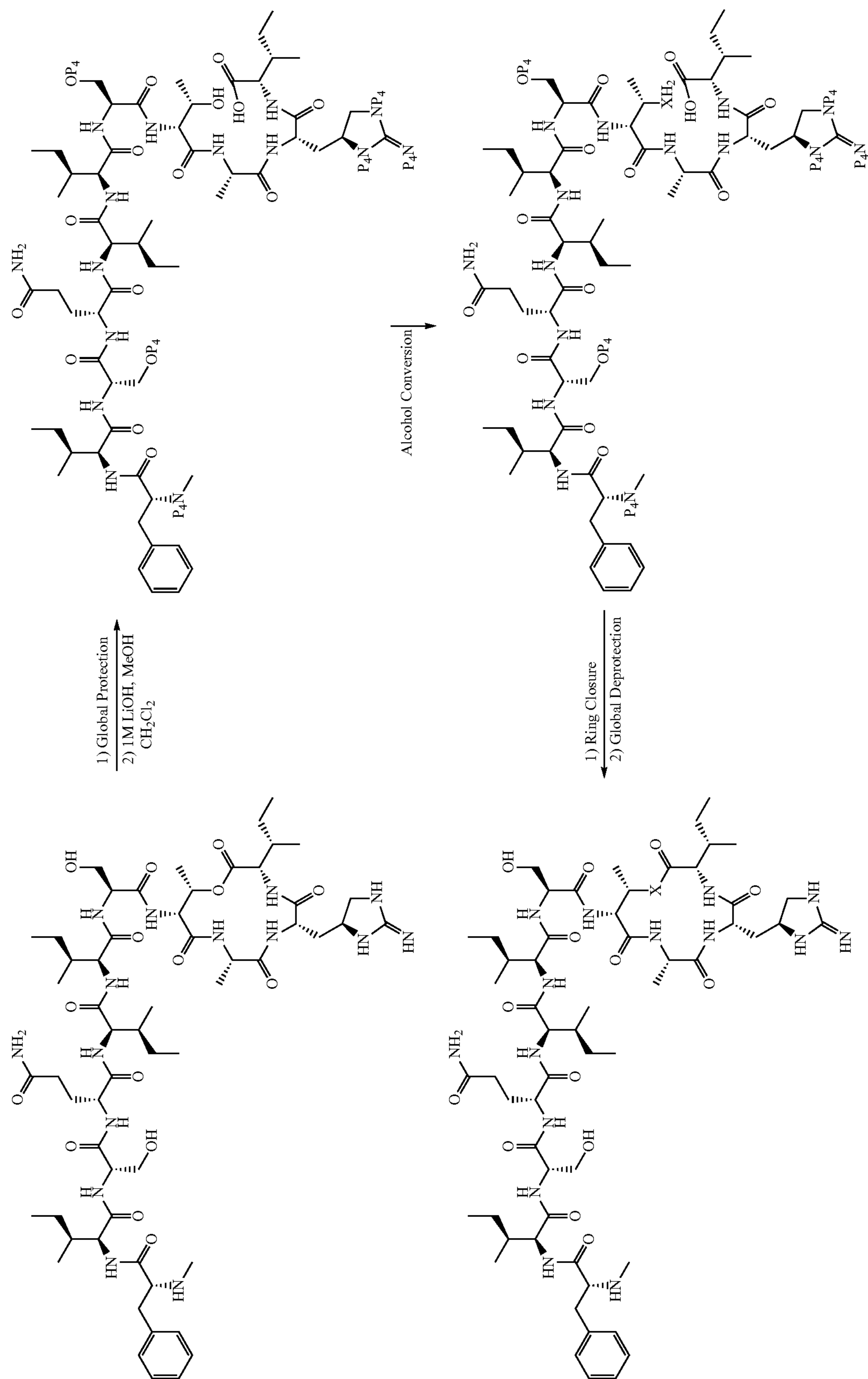
Scheme 4.
