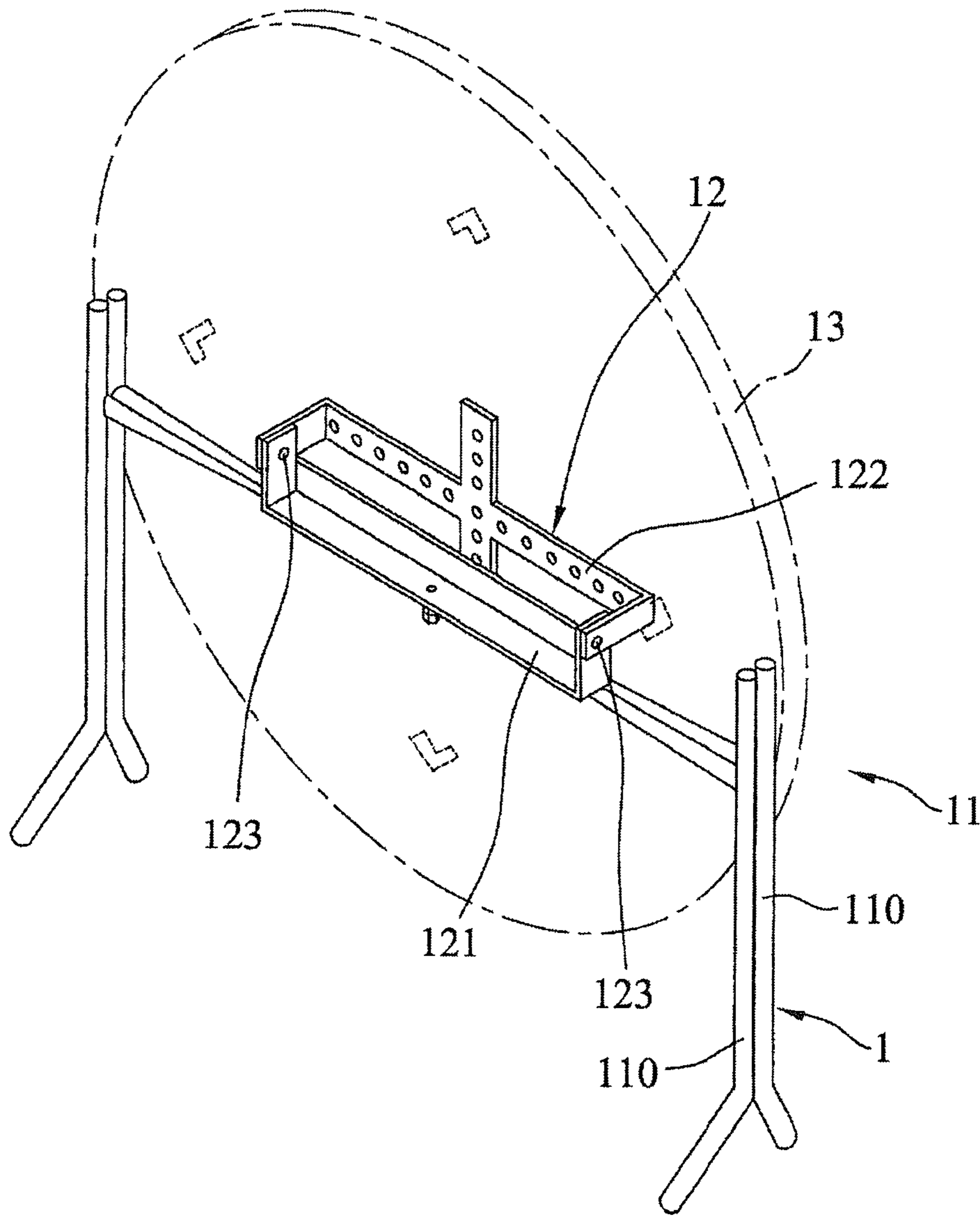
FIG. 2 PRIOR ART
