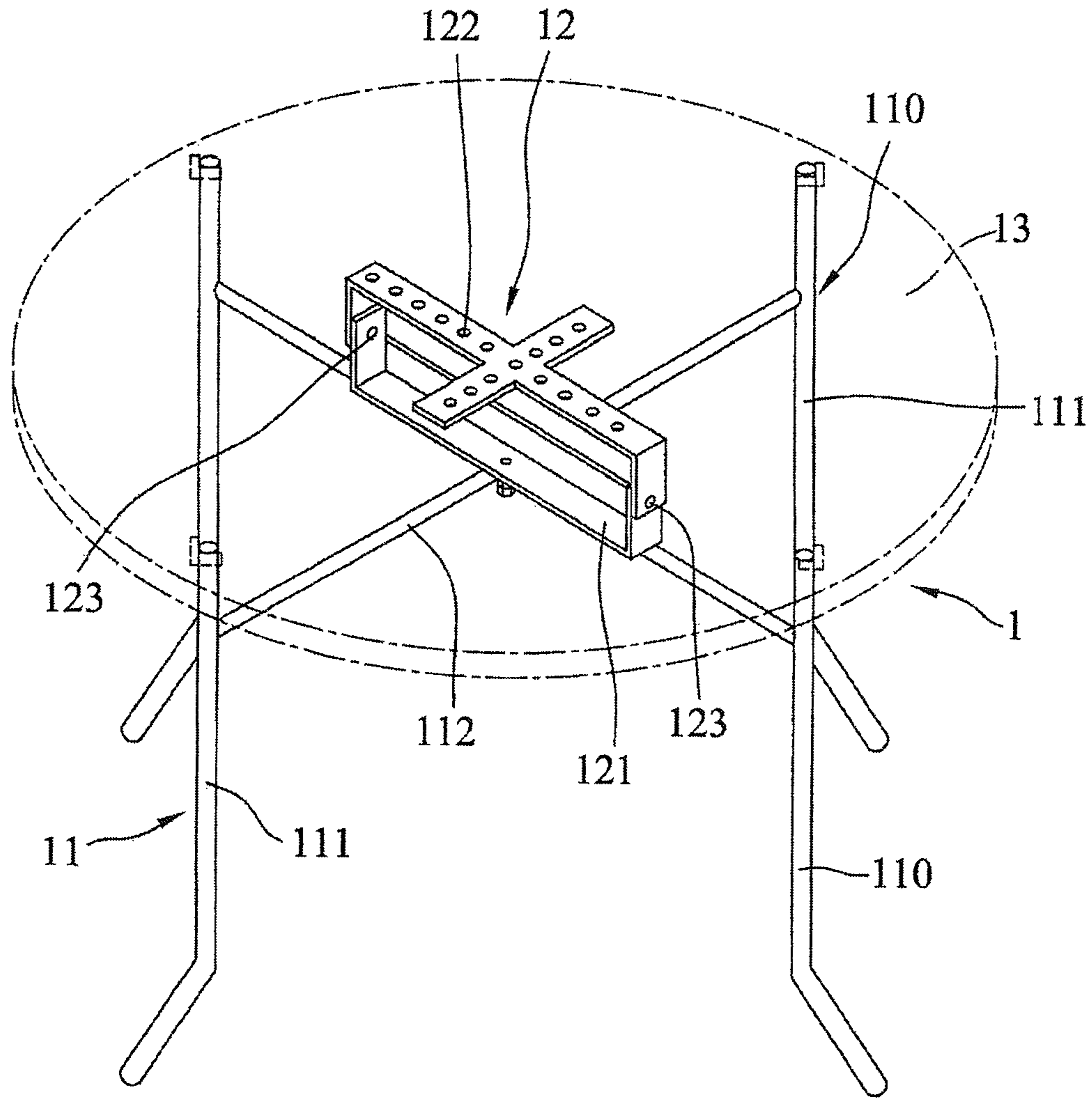
FIG. 1 PRIOR ART
