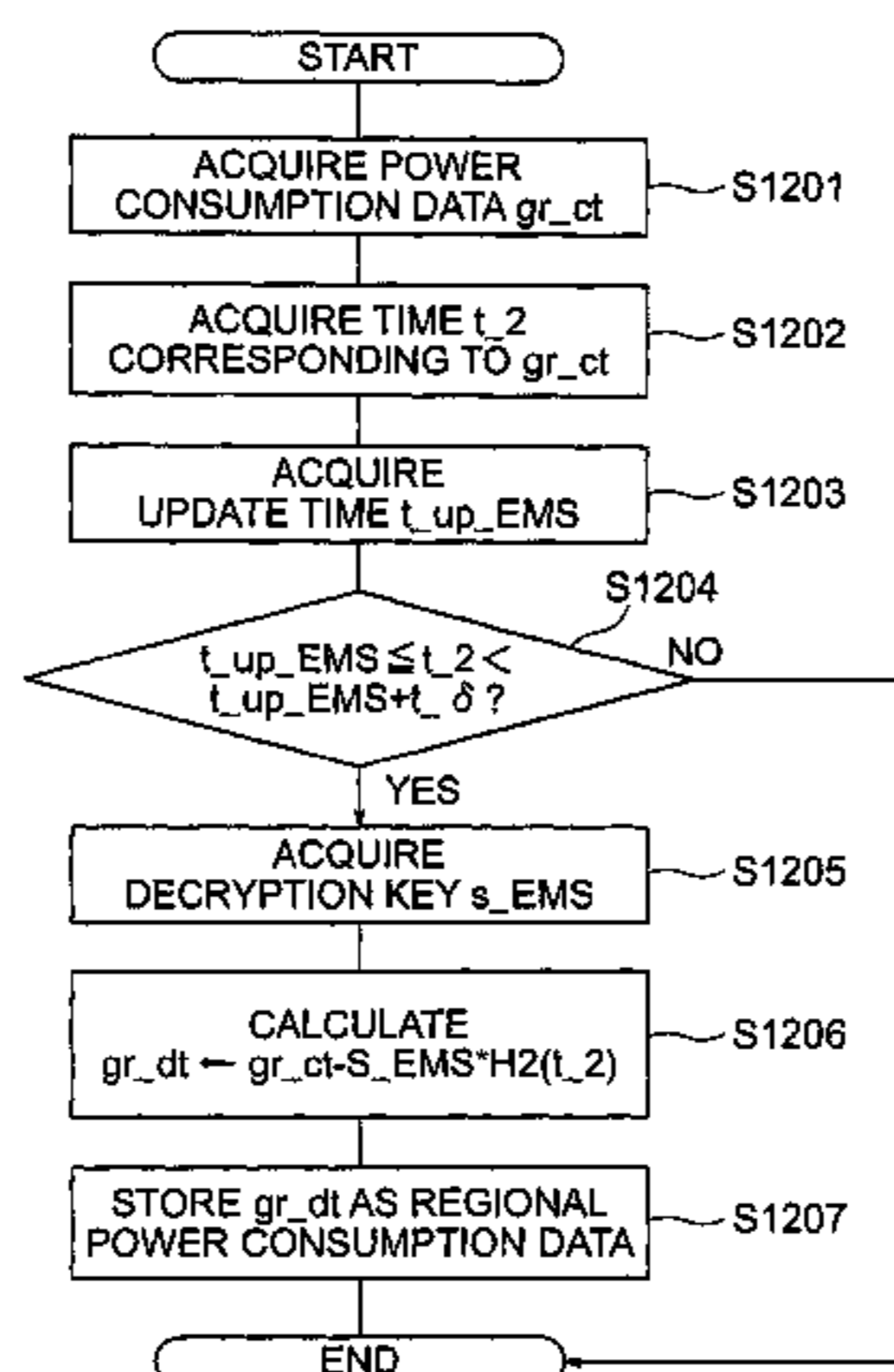
PROCESS PERFORMED BY EMS TO DECODE TOTAL POWER CONSUMPTION DATA
