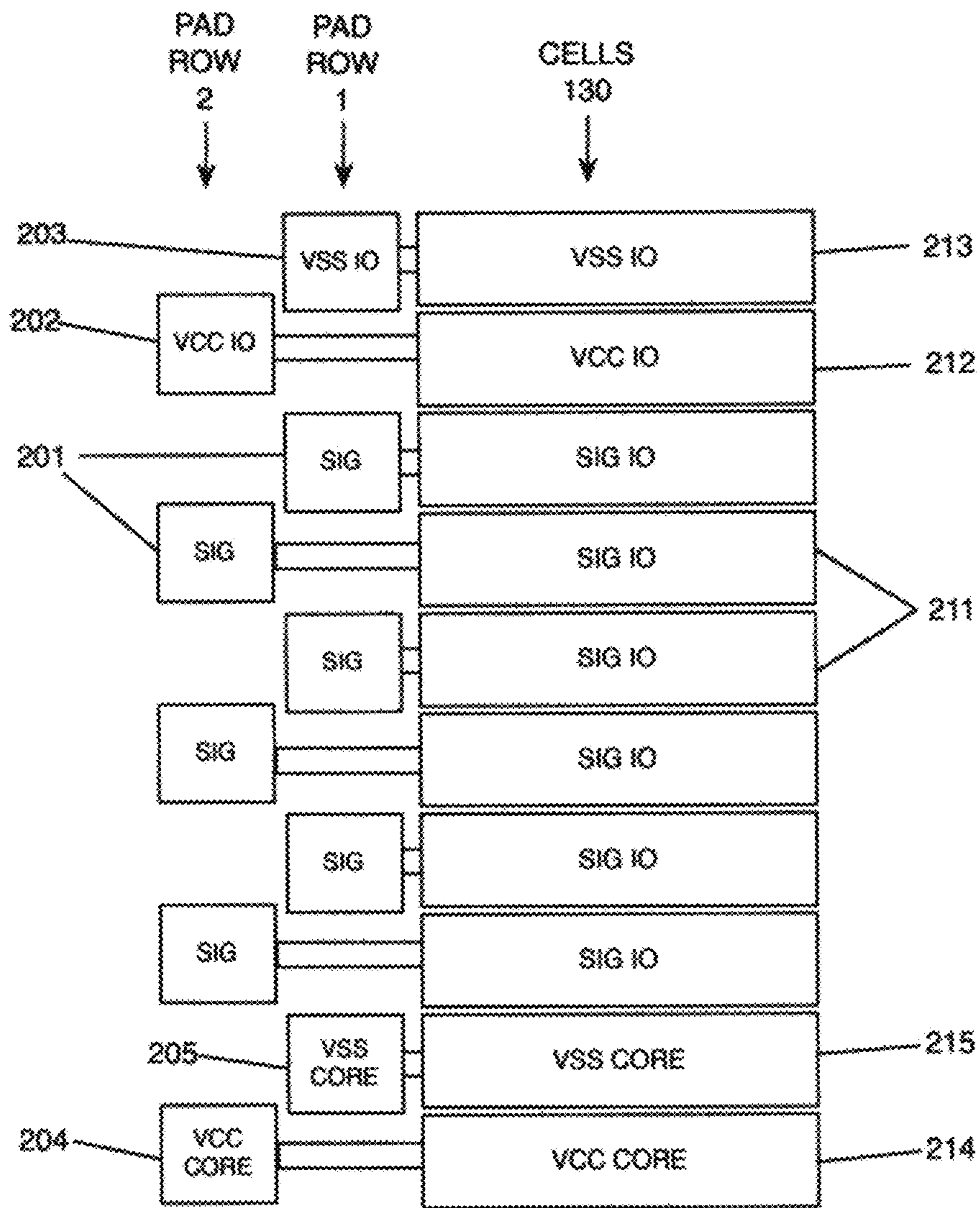
Fig. 1 (Prior Art)
