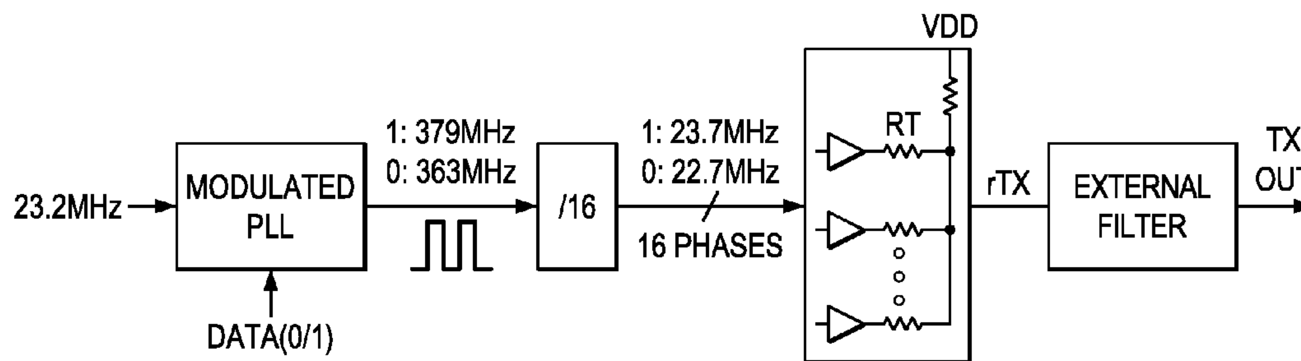
FIG. 3 (PRIOR ART)
