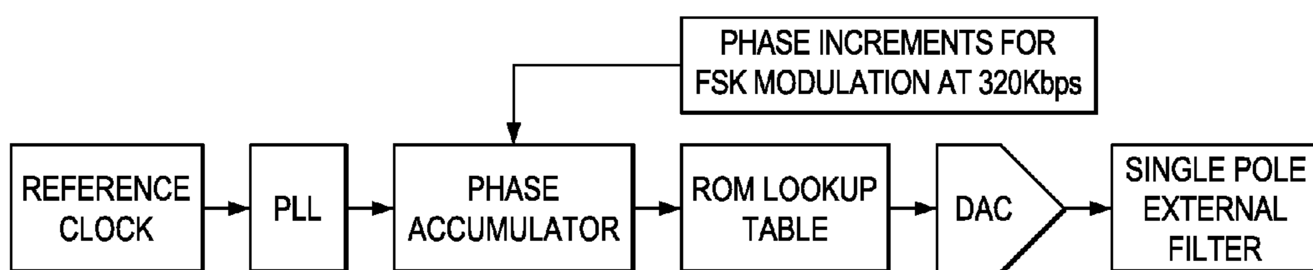
FIG. 2 (PRIOR ART)
