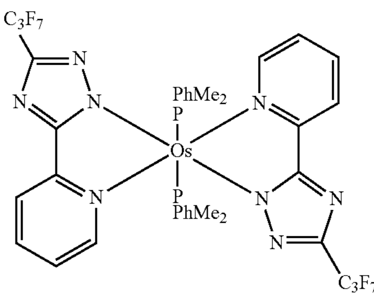
Os(hptz) 2 (PPhMe 2 ) 2
