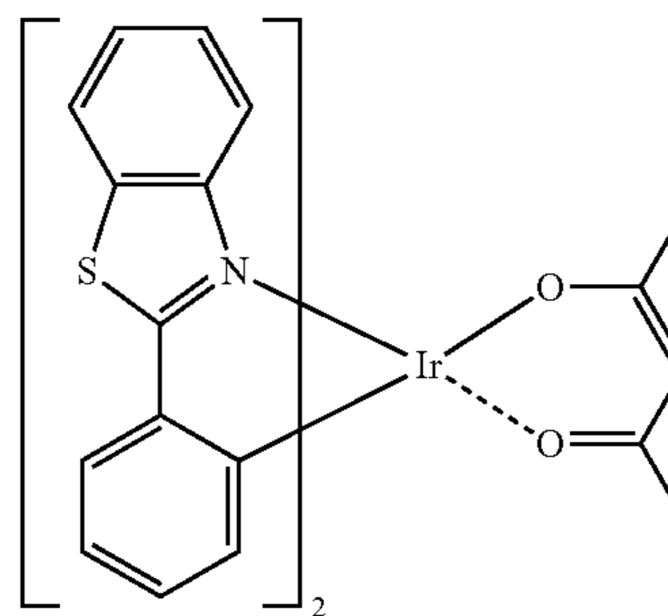
Ir(BT) 2 (acac)
