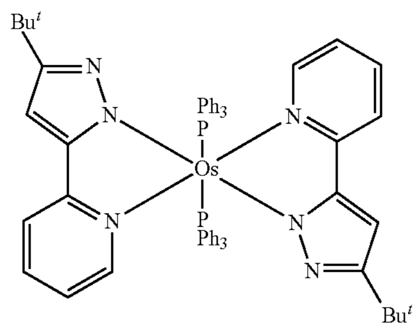
Os(bppz) 2 (PPh 3 ) 2
