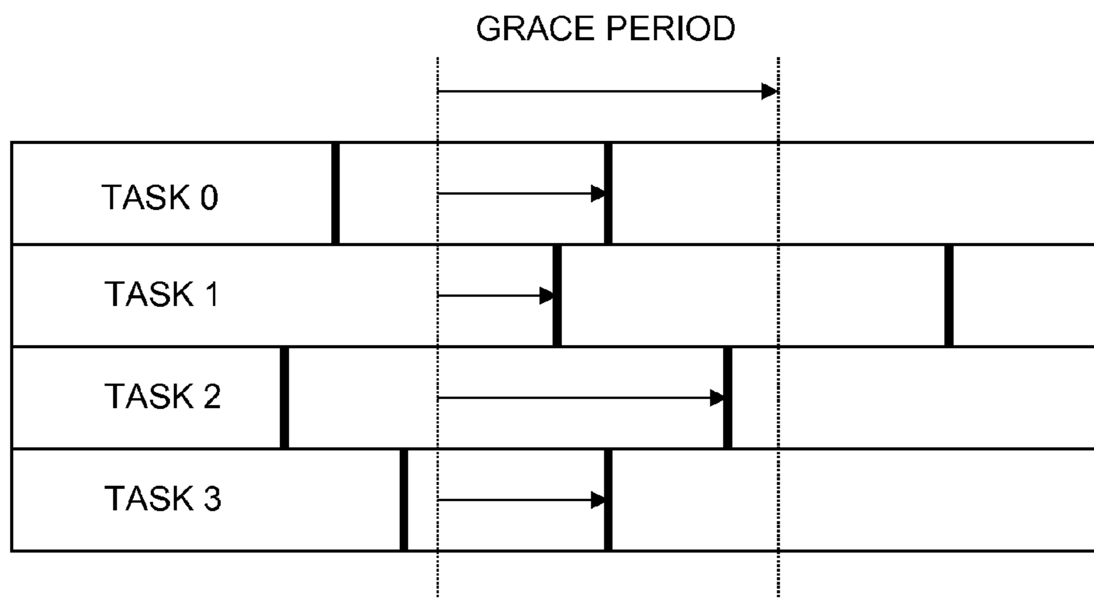
FIG. 3 (PRIOR ART)
