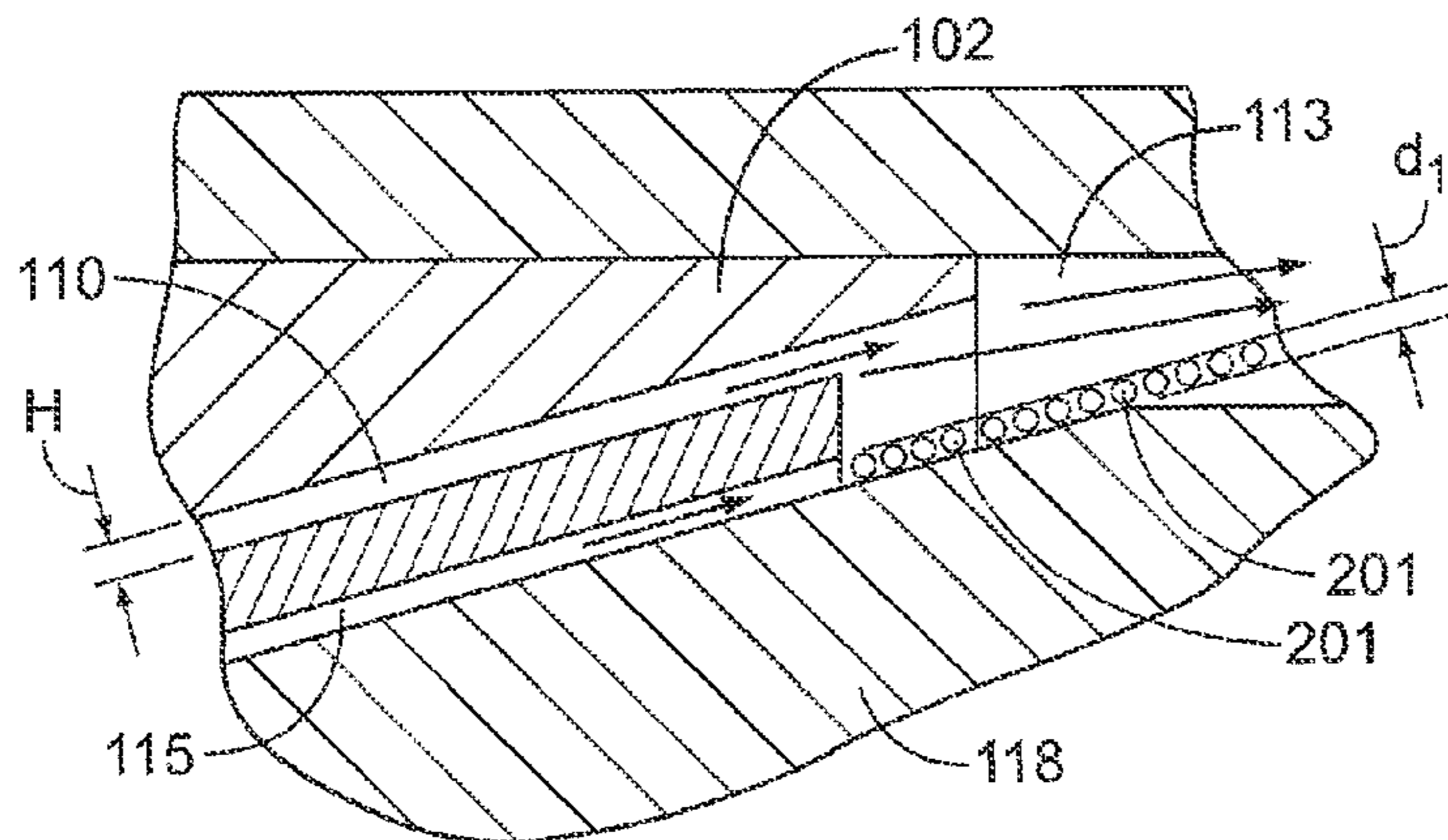
FIG. 2D
