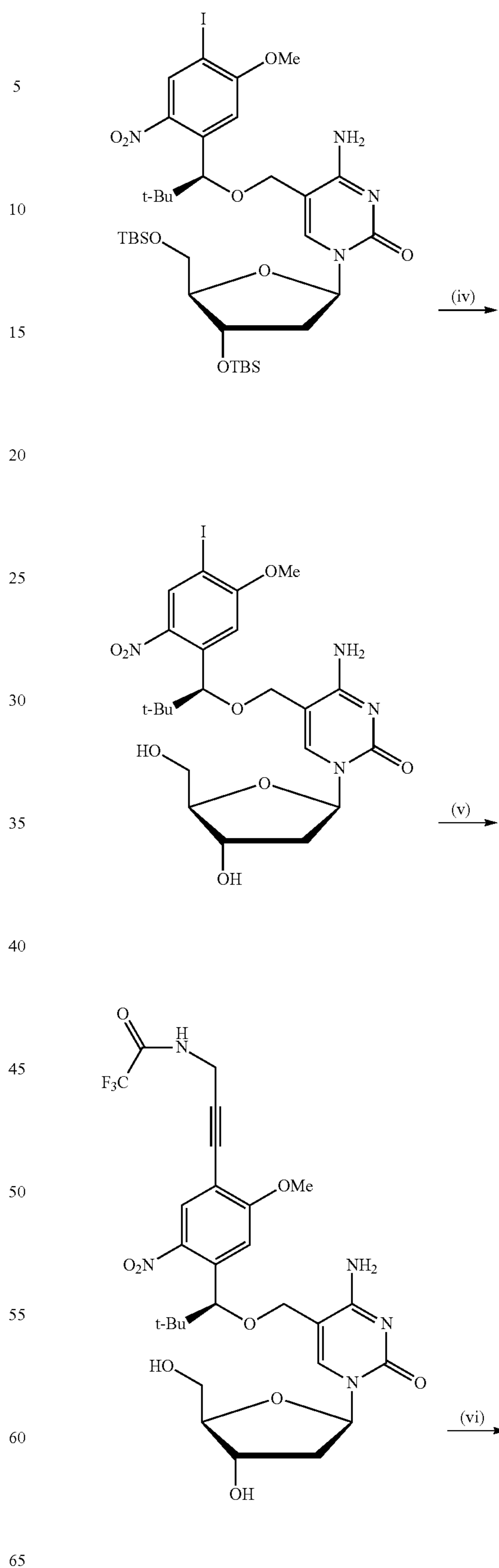
Scheme 5a. Synthesis of dye labeled 5-[(S)-1-(5-methoxy-2-nitrophenyl)-2,2-dimethyl-propyloxy]methyl-2'-deoxycytidine-5'-triphosphate.
