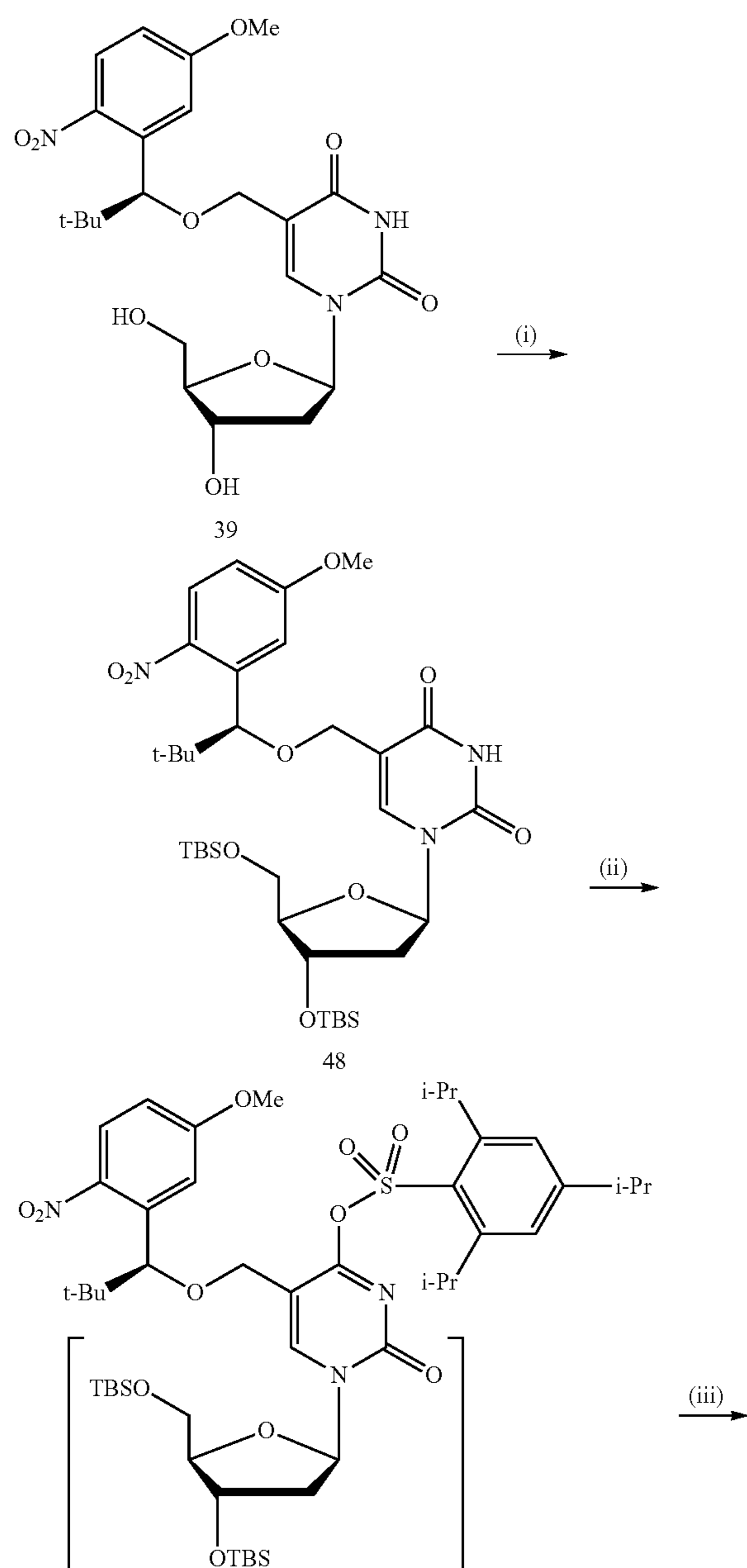
Scheme S22. Synthesis of 5-[(S)-1-(5-methoxy-2-nitrophenyl)-2,2-dimethyl-propyloxy]methyl-2'-deoxycytidine-5'-triphosphate.
