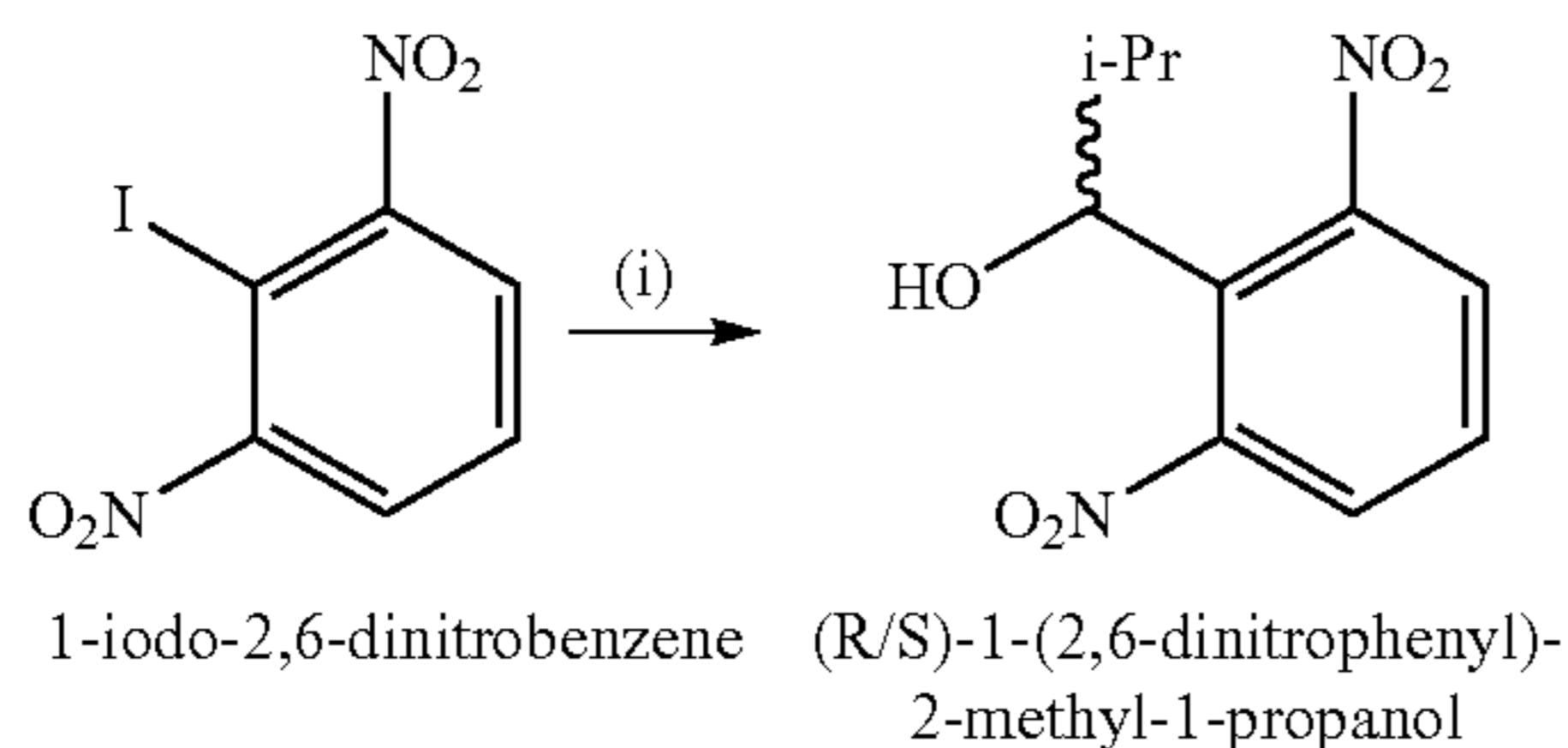
Scheme S1. Synthesis of (R/S)-1-(2,6-dinitrophenyl)-2-methyl-1-propanol.
