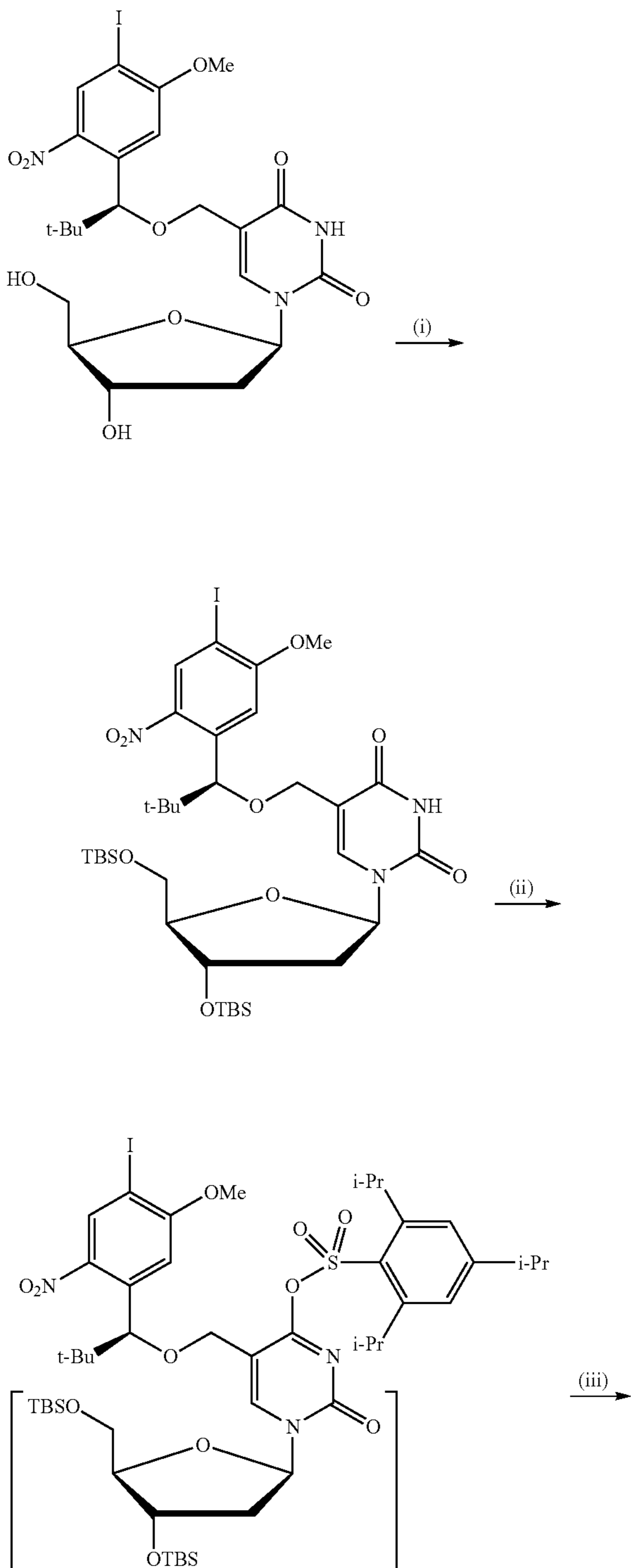
Scheme 5a. Synthesis of dye labeled 5-[(S)-1-(5-methoxy-2-nitrophenyl)-2,2-dimethyl-propyloxy]methyl-2'-deoxycytidine-5'-triphosphate.
