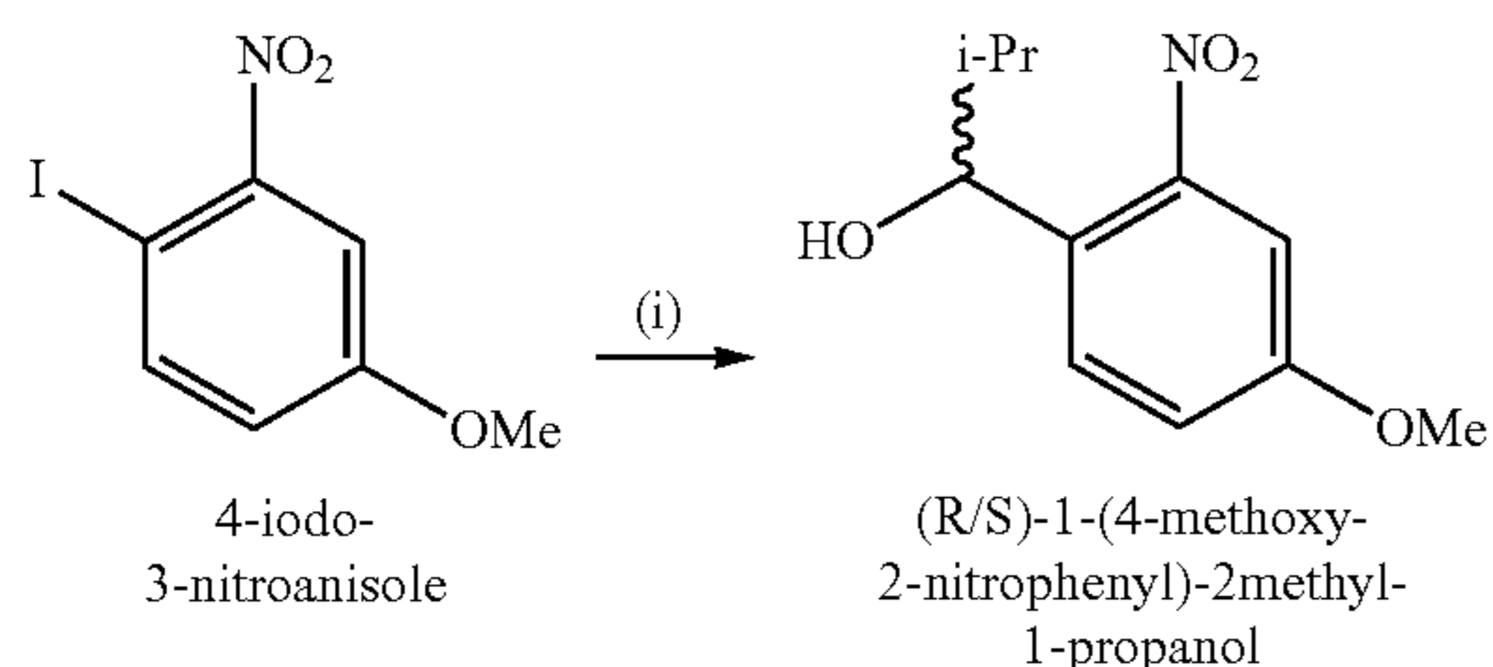
Scheme S2. Synthesis of (R/S)-1-(4-methoxy-2-nitrophenyl)-2-methyl-1-propanol.
