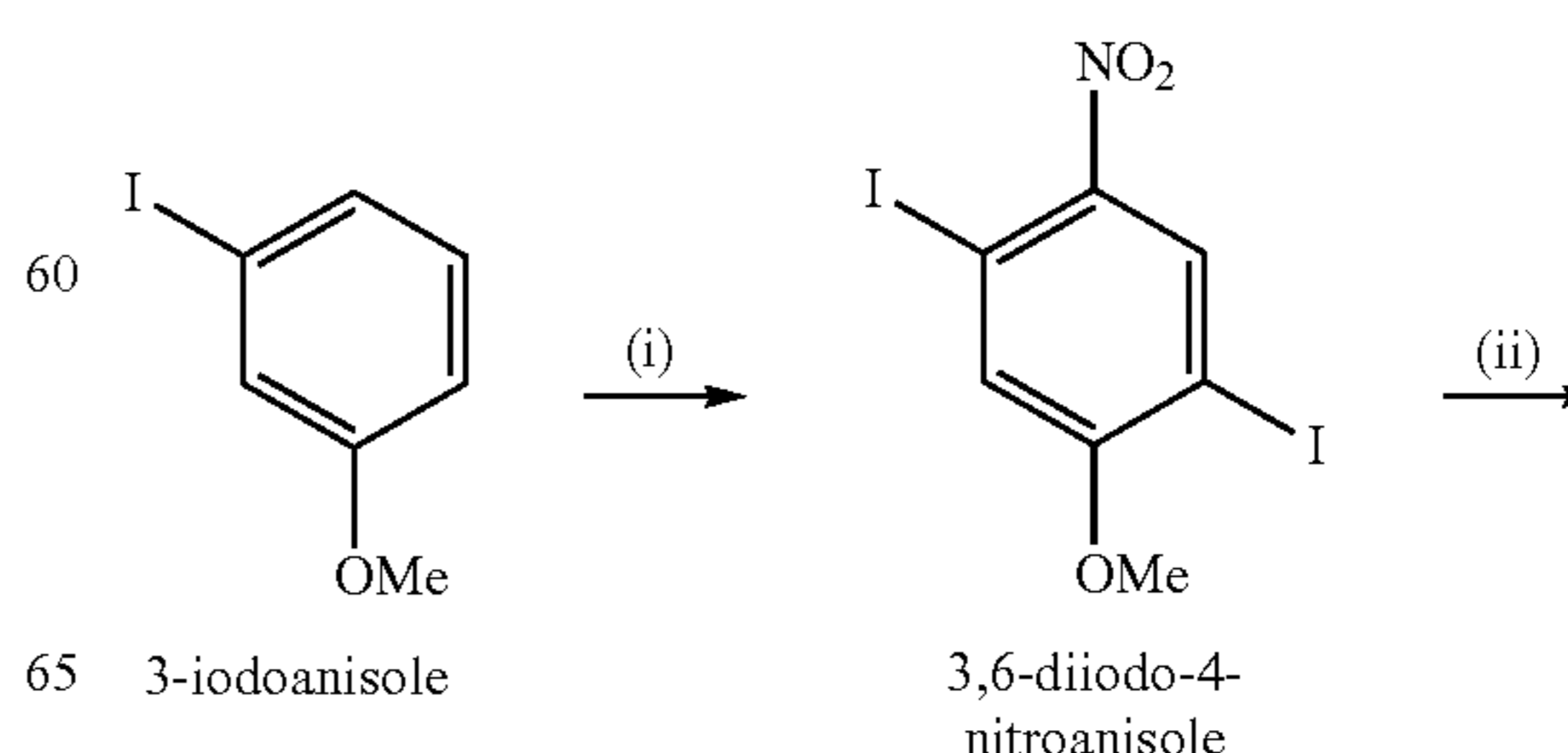
Scheme S24.
