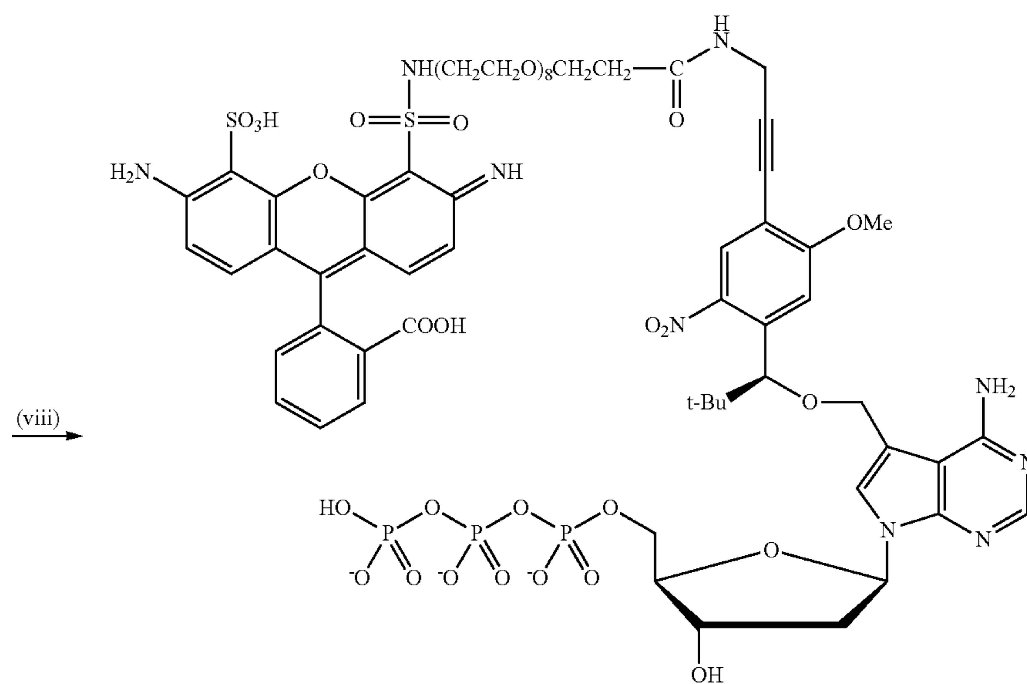
Scheme 2d.
