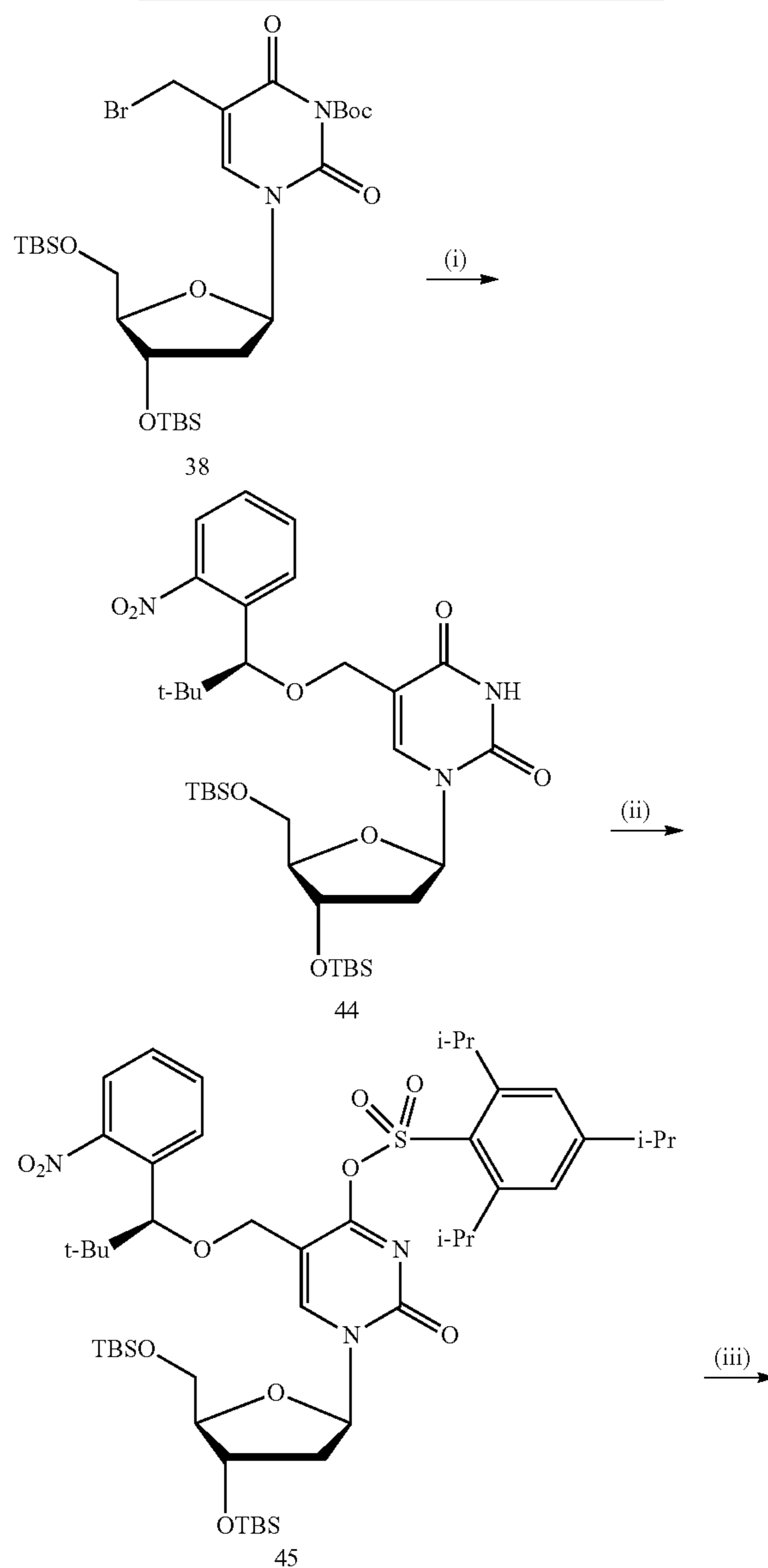
Scheme S21. Synthesis of 5-[(S)-1-(2-nitrophenyl)-2,2-dimethyl-propyloxy]methyl-2'-deoxycytidine-5'-triphosphate.
