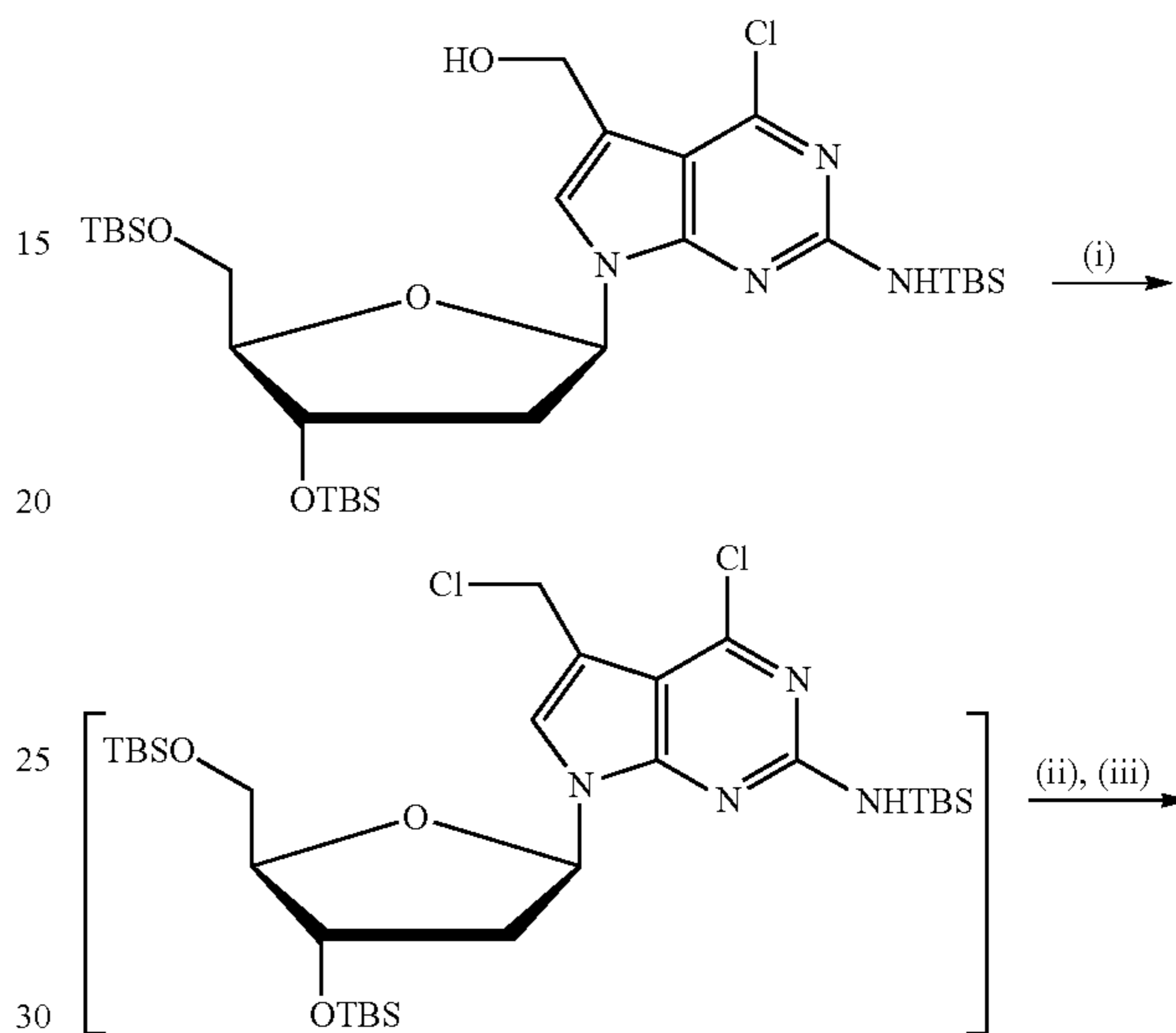
Scheme 4a. Synthesis of dye labeled 7-[(S)-1-(5-methoxy-2-nitrophenyl)-2,2-dimethyl-propyloxy]methyl-7-deaza-2'-deoxyguanosine-5'-triphosphate.
