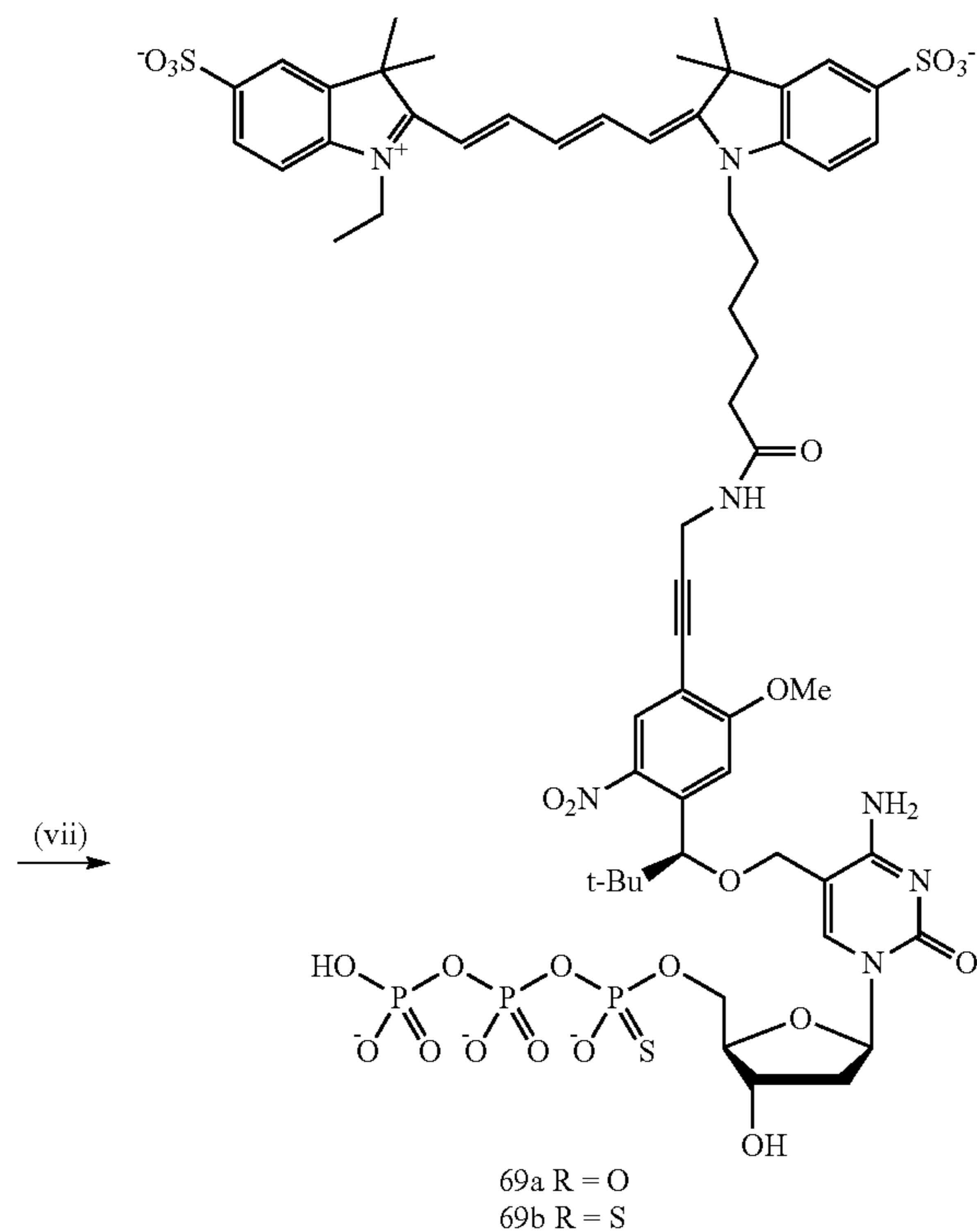
Scheme S28b.
