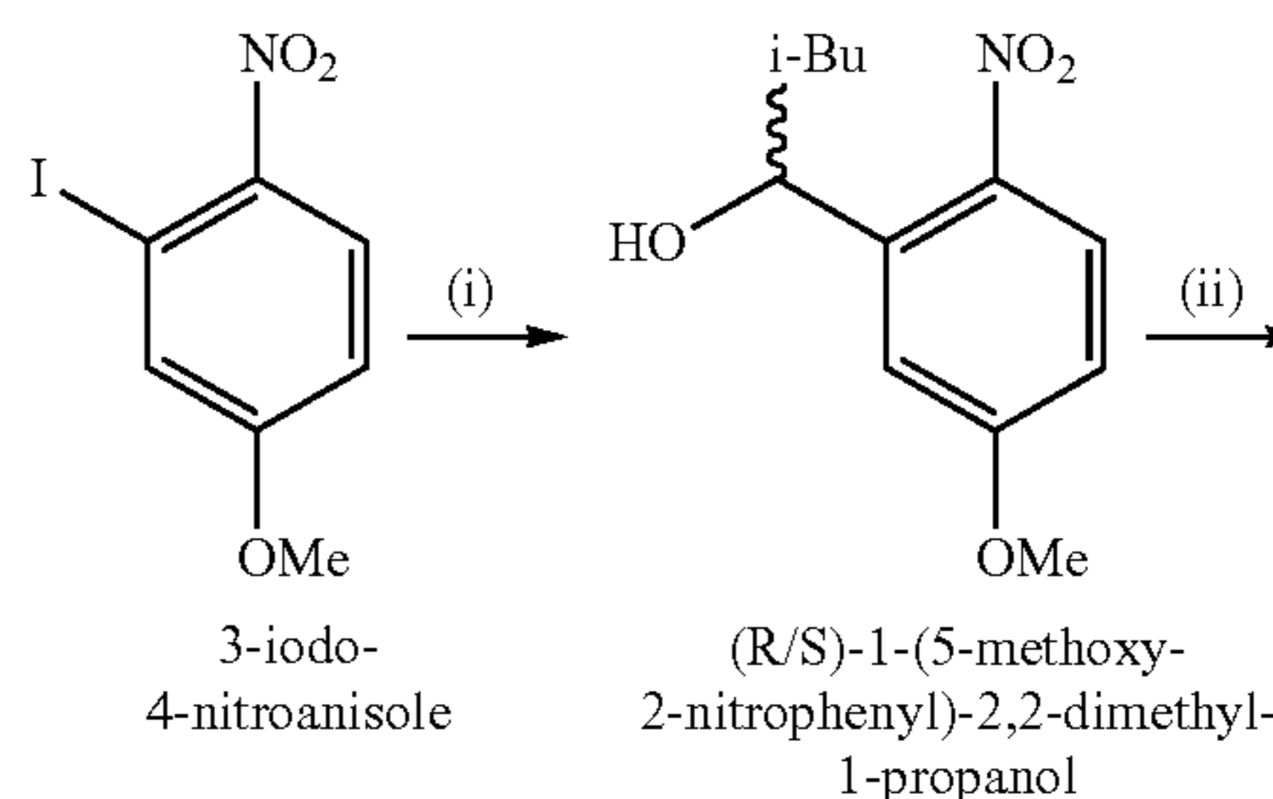
Scheme S4. Synthesis of (R/S)-1-(5-methoxy-2-nitrophenyl)-2,2-dimethyl-1-propanol and (S)-1-(5-methoxy-2-nitrophenyl)-2,2-dimethyl-1-propanol.
