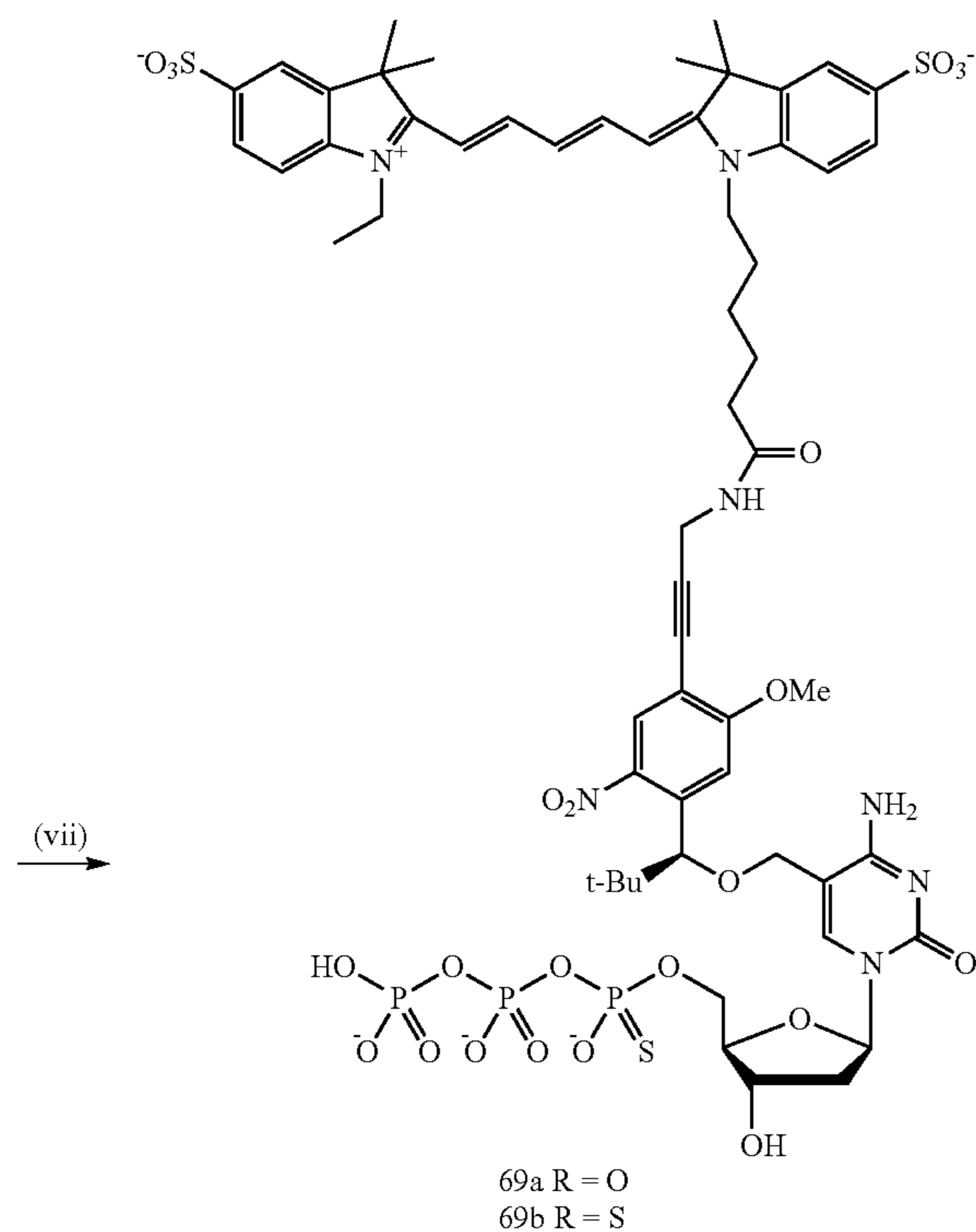
Scheme S28b.
