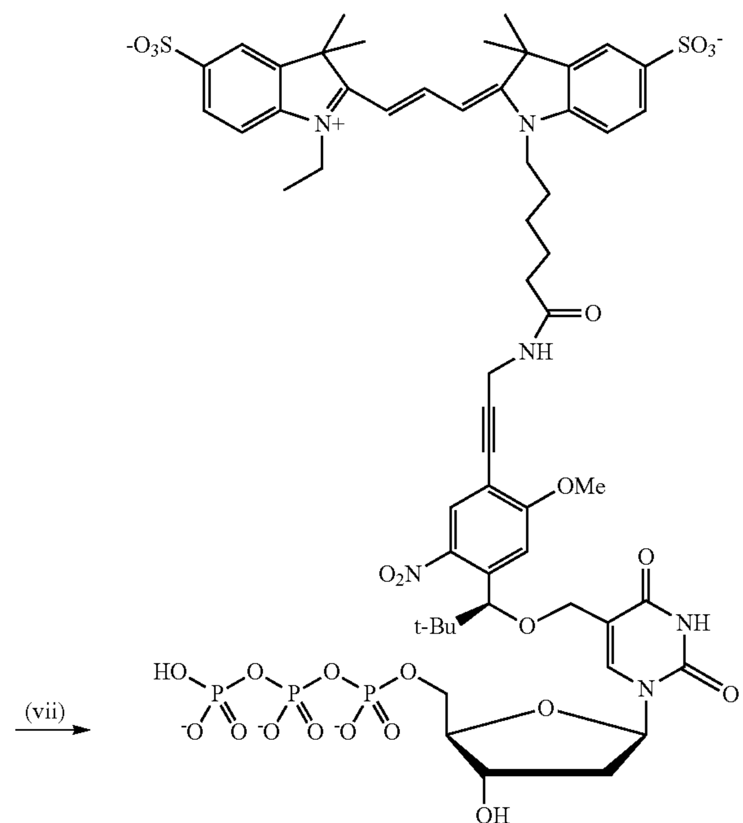
Scheme 3d.
