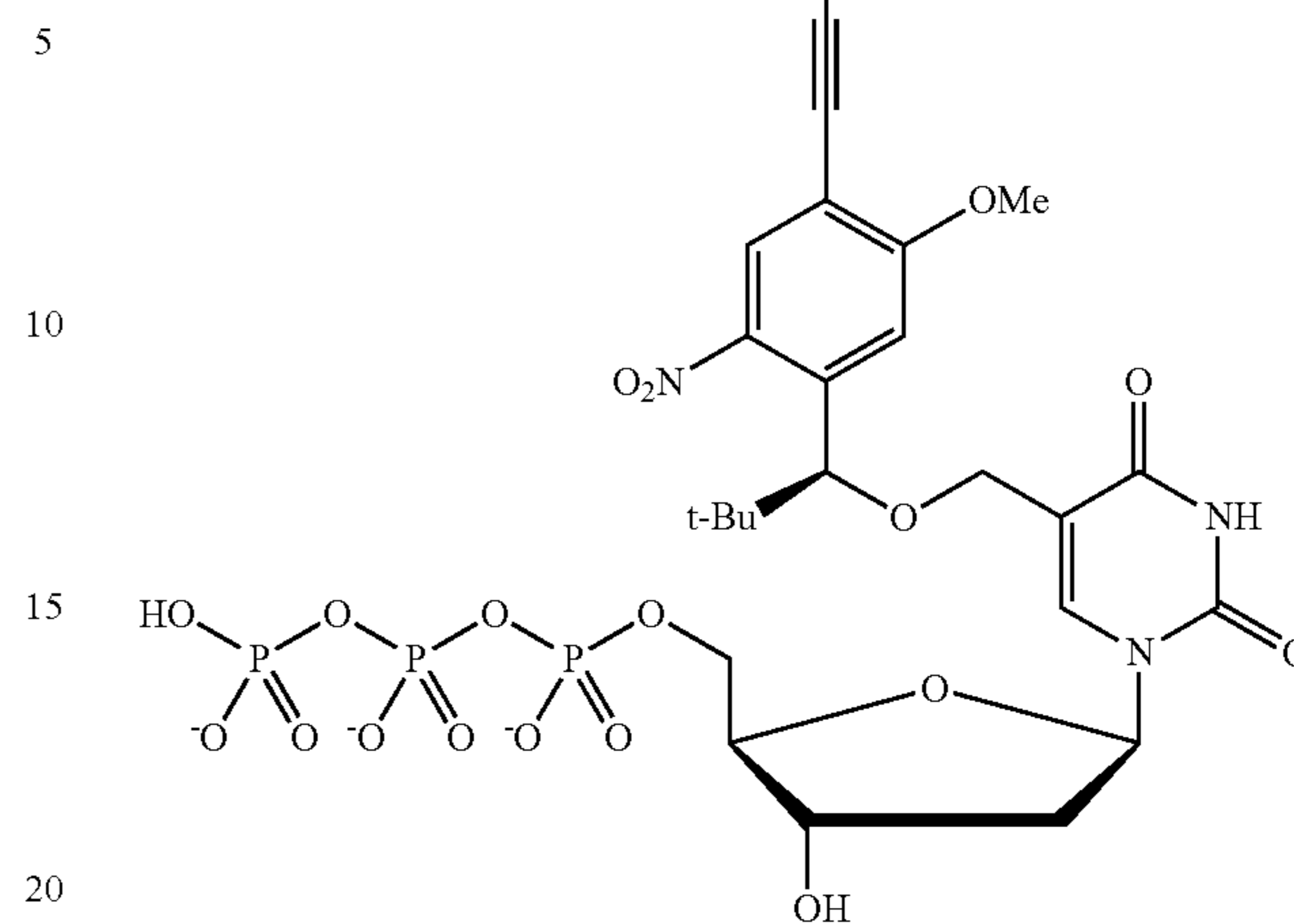
Scheme 3a. Synthesis of dye labeled 5-[(S)-1-(5-methoxy-2-nitrophenyl)-2,2-dimethyl-propyloxy]methyl-2'-deoxyuridine-5'-triphosphate.
