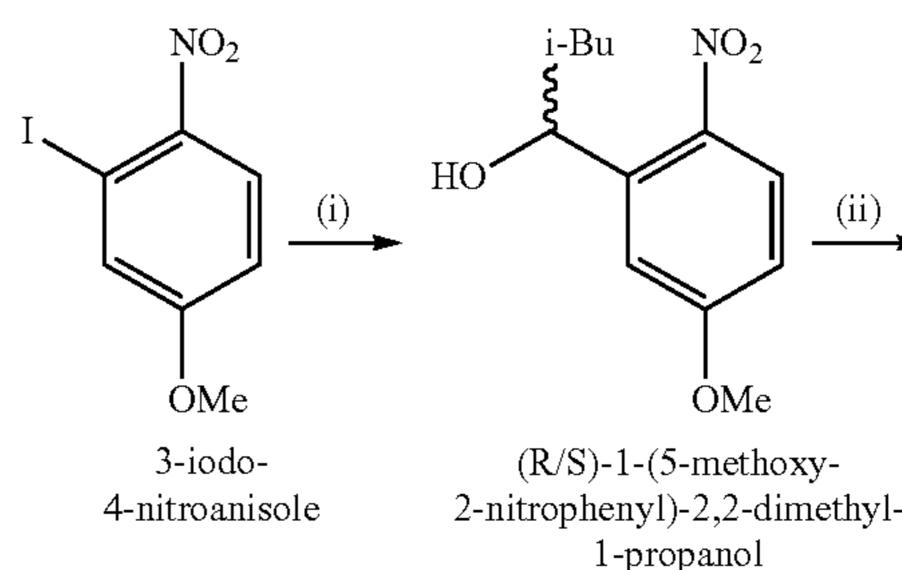
Scheme S4. Synthesis of (R/S)-1-(5-methoxy-2-nitrophenyl)-2,2-dimethyl-1-propanol and (S)-1-(5-methoxy-2-nitrophenyl)-2,2-dimethyl-1-propanol.
