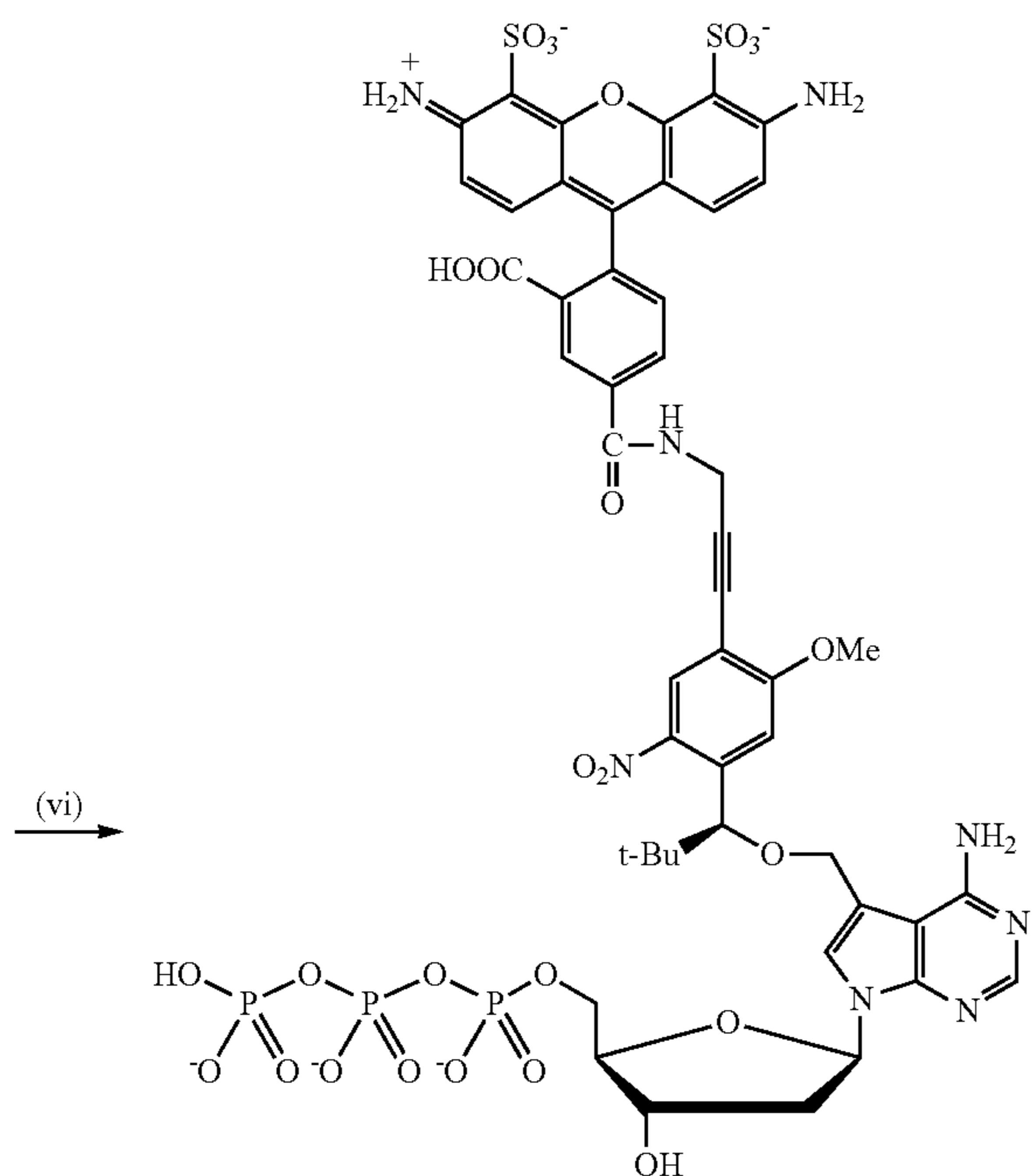
Scheme 2b.
