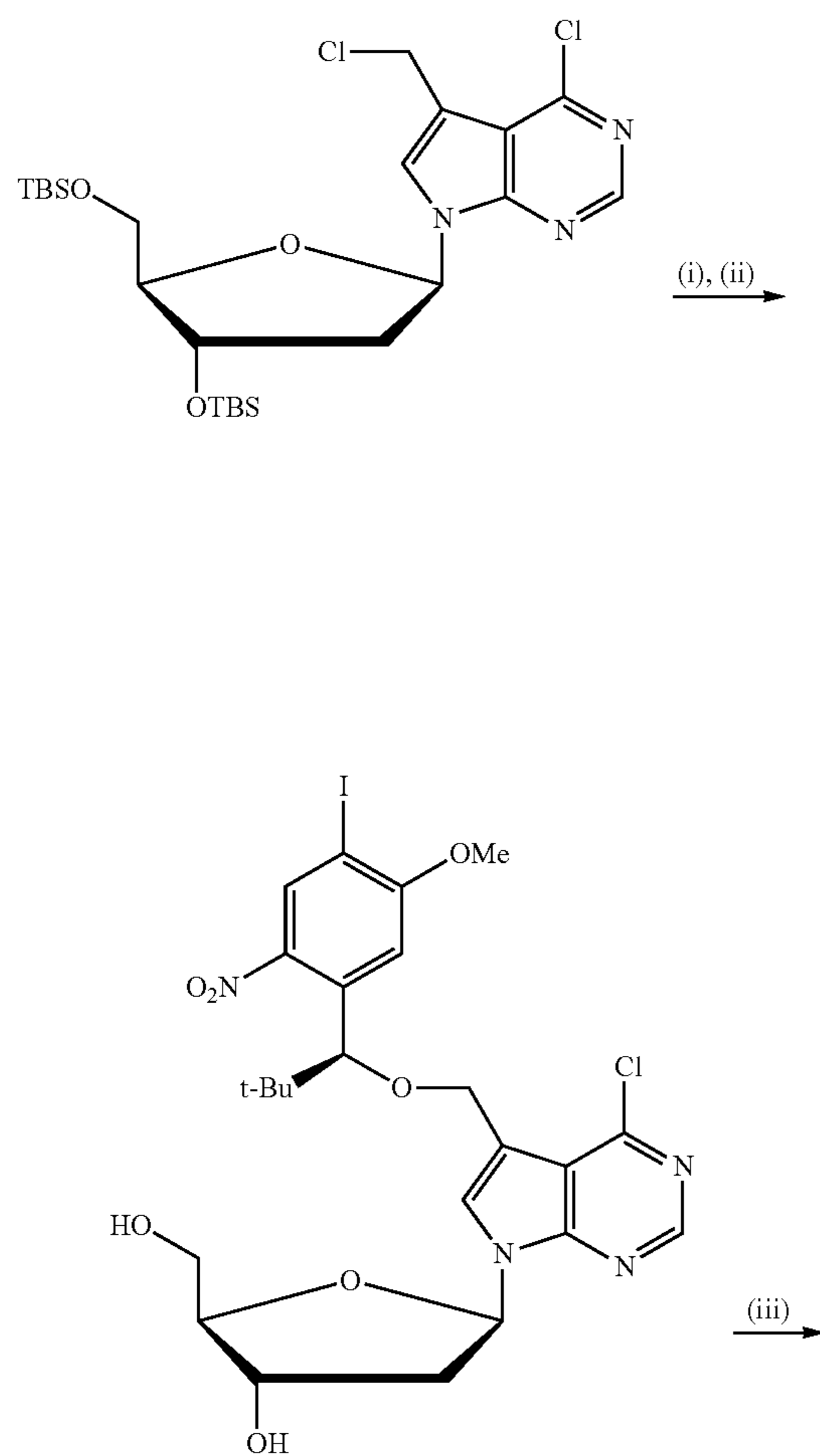
Scheme 2a. Synthesis of dye labeled 7-[(S)-1-(5-methoxy-2-nitrophenyl)- 2,2-dimethyl-propyloxy]methyl-7-deaza-2'-deoxyadenosine-5'- triphosphate.
