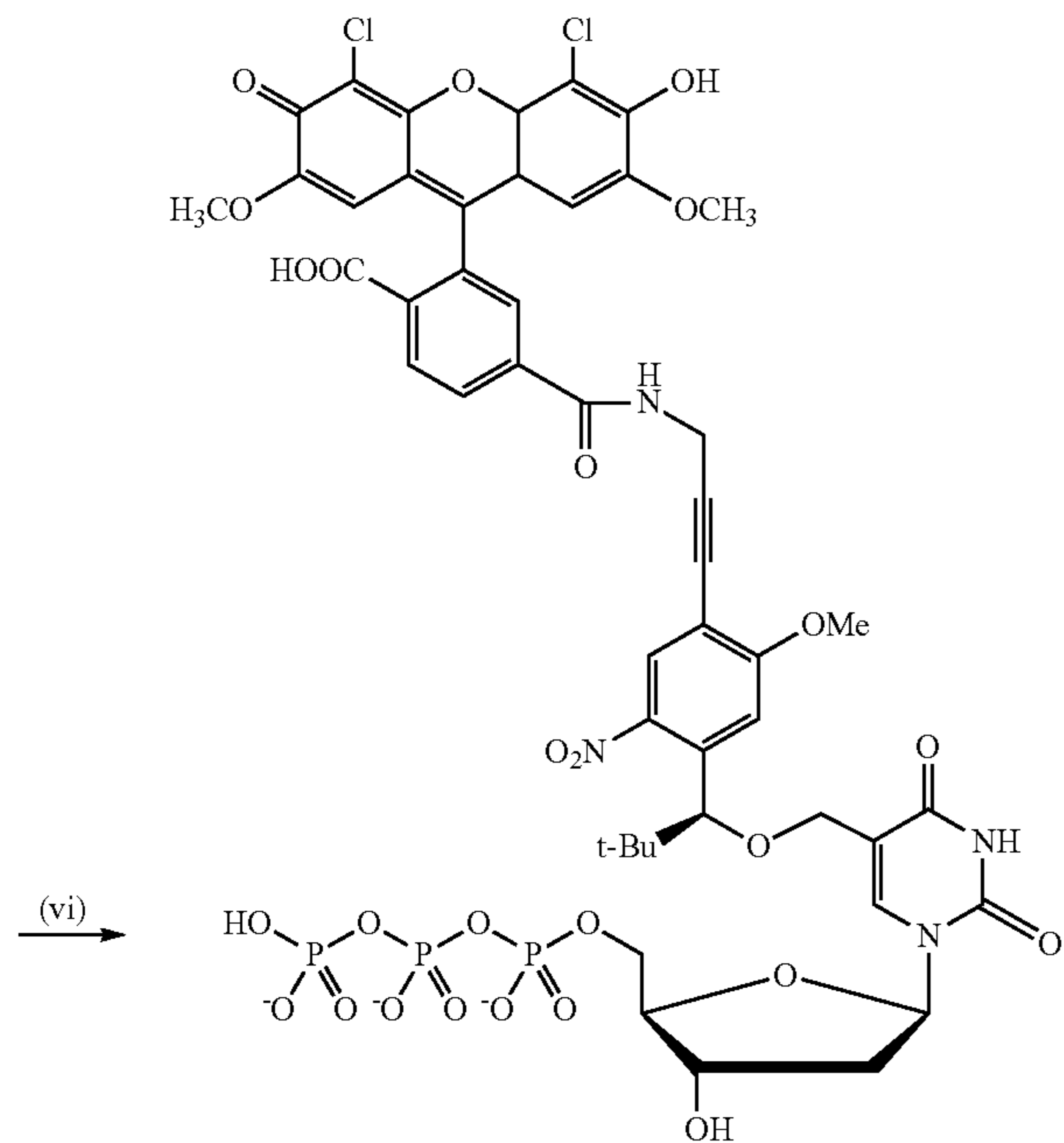
Scheme 3c.
