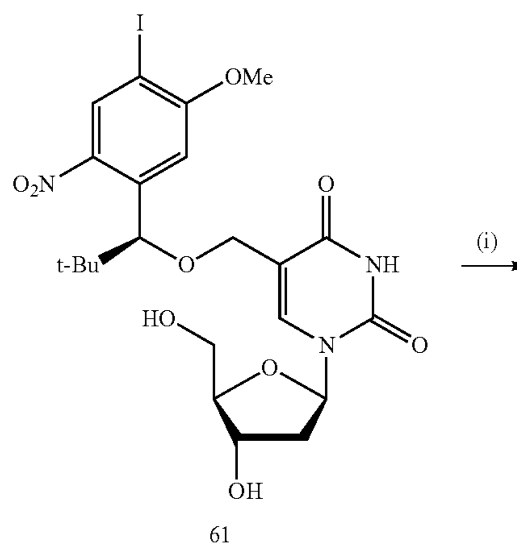
Scheme S28a. Synthesis of dye labeled 5-{(S)-1-[4-(3-amino-1-propynyl)-5-methoxy-2-nitrophenyl]-2,2-dimethyl-propyloxy}methyl-2'-deoxycytidine-5'-triphosphate.
