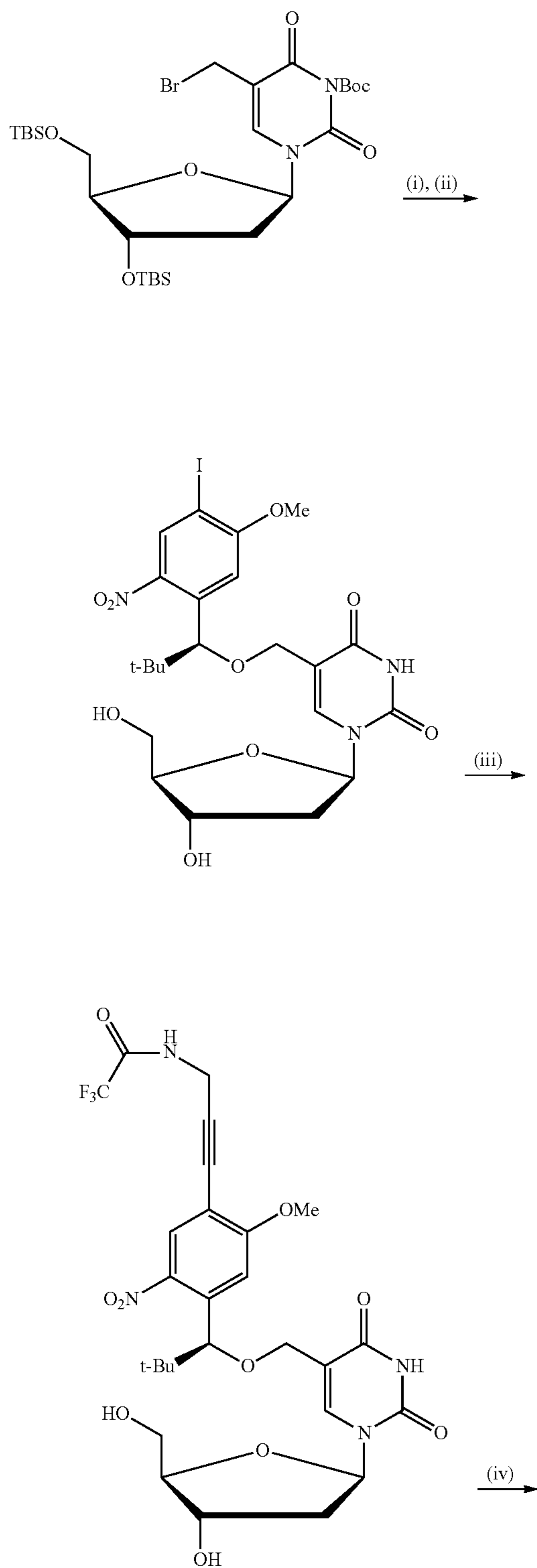
Scheme 3a. Synthesis of dye labeled 5-[(S)-1-(5-methoxy-2-nitrophenyl)-2,2-dimethyl-propyloxy]methyl-2'-deoxyuridine-5'-triphosphate.
