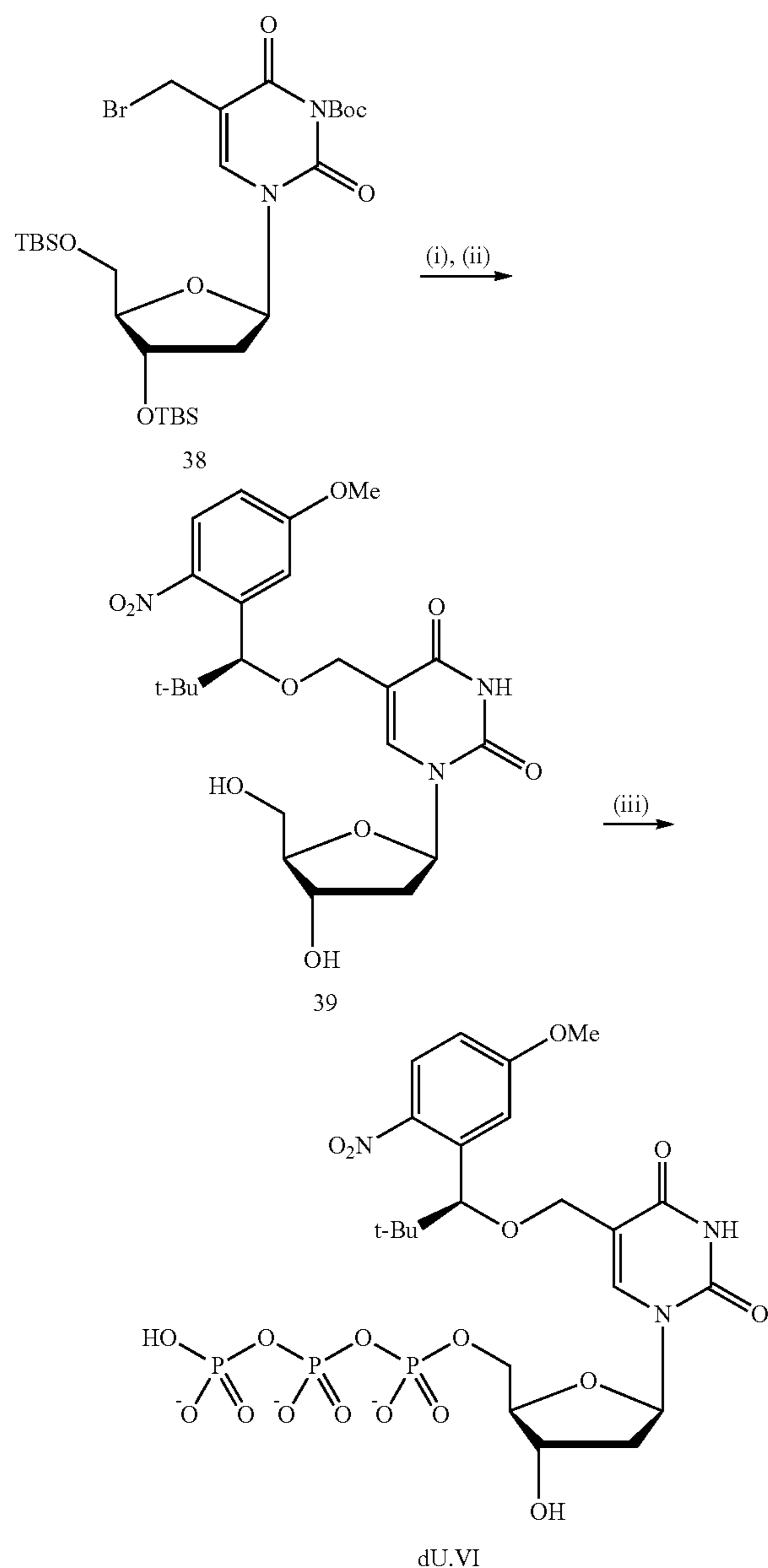
Scheme S19. Synthesis of 5-[(S)-1-(5-methoxy-2-nitrophenyl)-2,2-dimethyl-propyloxy]methyl-2'-deoxyuridine-5'-triphosphate.
