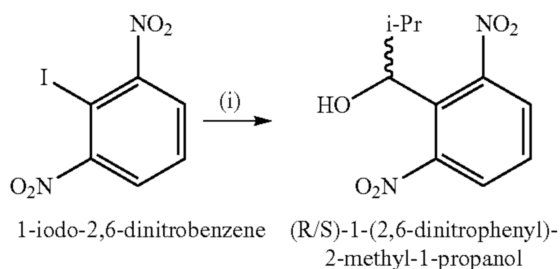
Scheme S1. Synthesis of (R/S)-1-(2,6-dinitrophenyl)-2-methyl-1-propanol.
