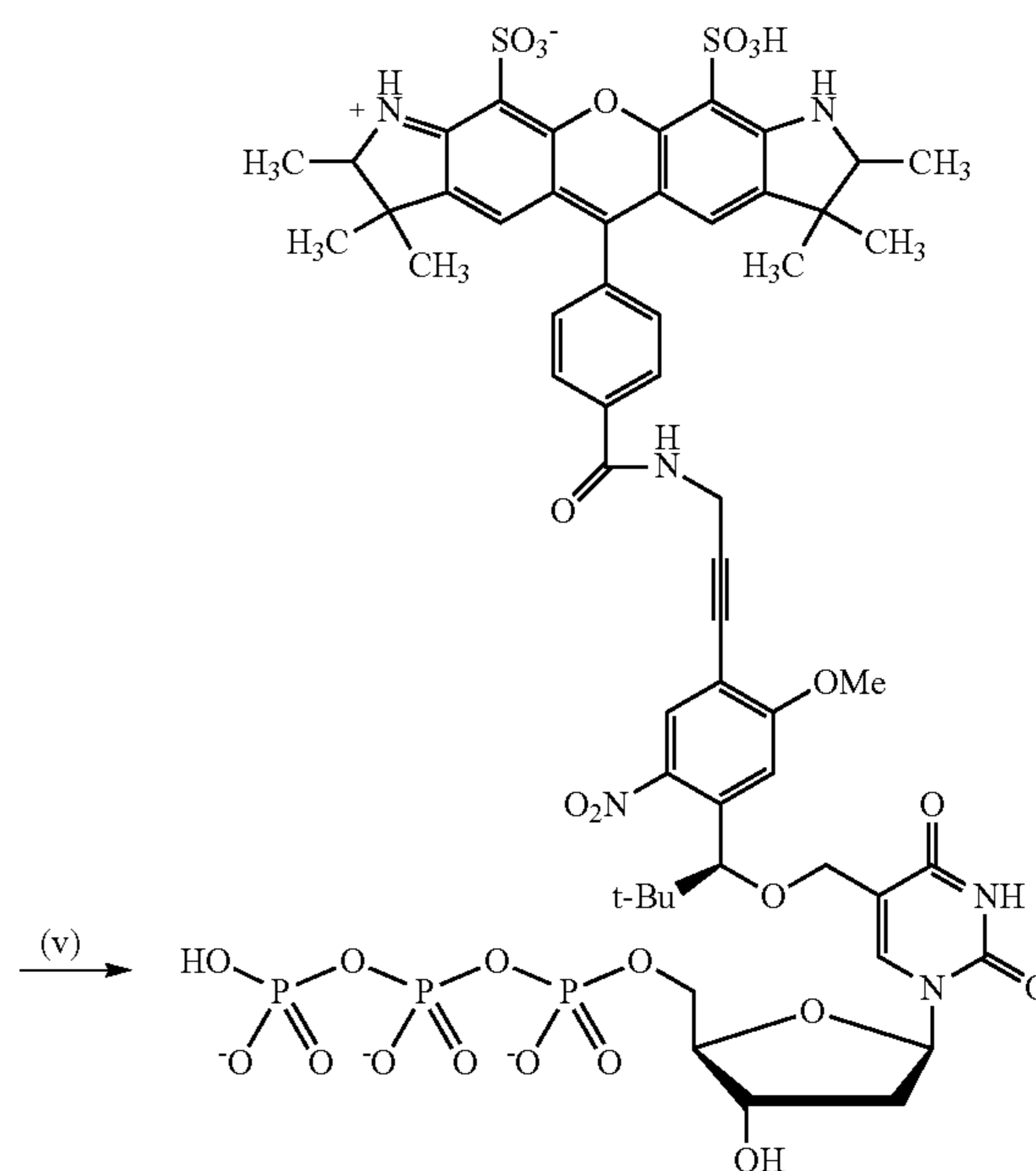
Scheme 3b.
