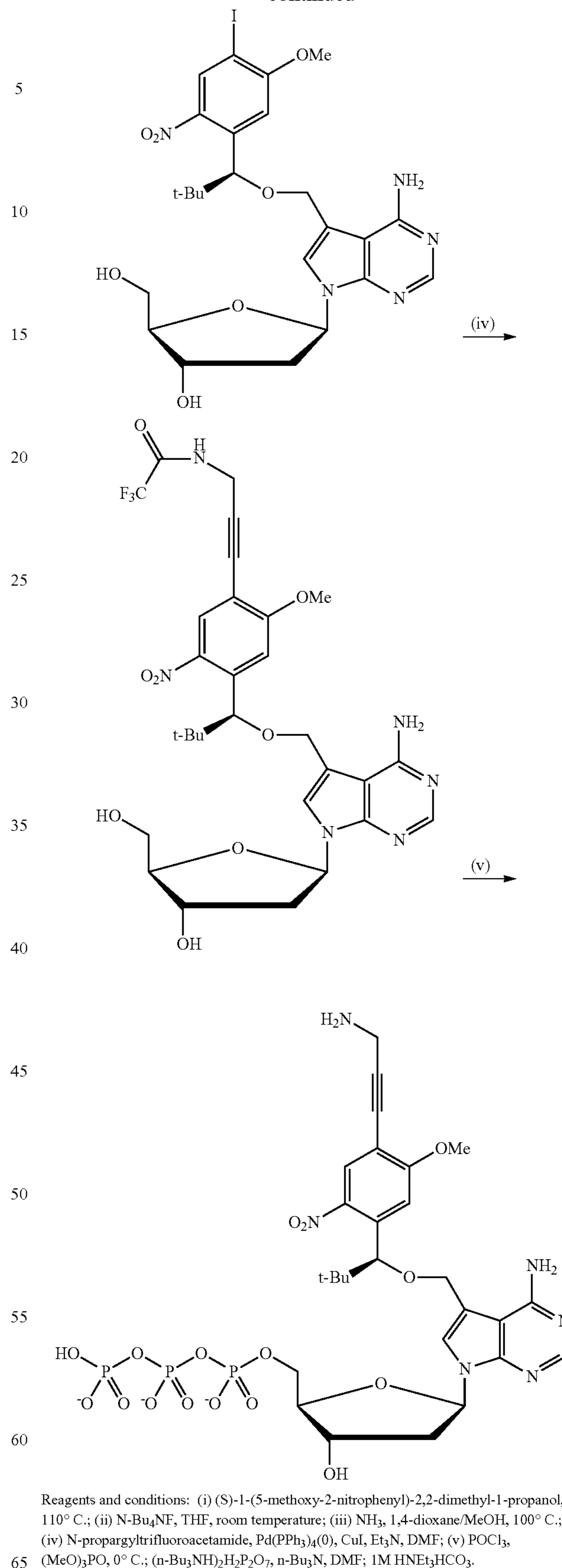
Scheme 2a. Synthesis of dye labeled 7-[(S)-1-(5-methoxy-2-nitrophenyl)- 2,2-dimethyl-propyloxy]methyl-7-deaza-2'-deoxyadenosine-5'- triphosphate.
