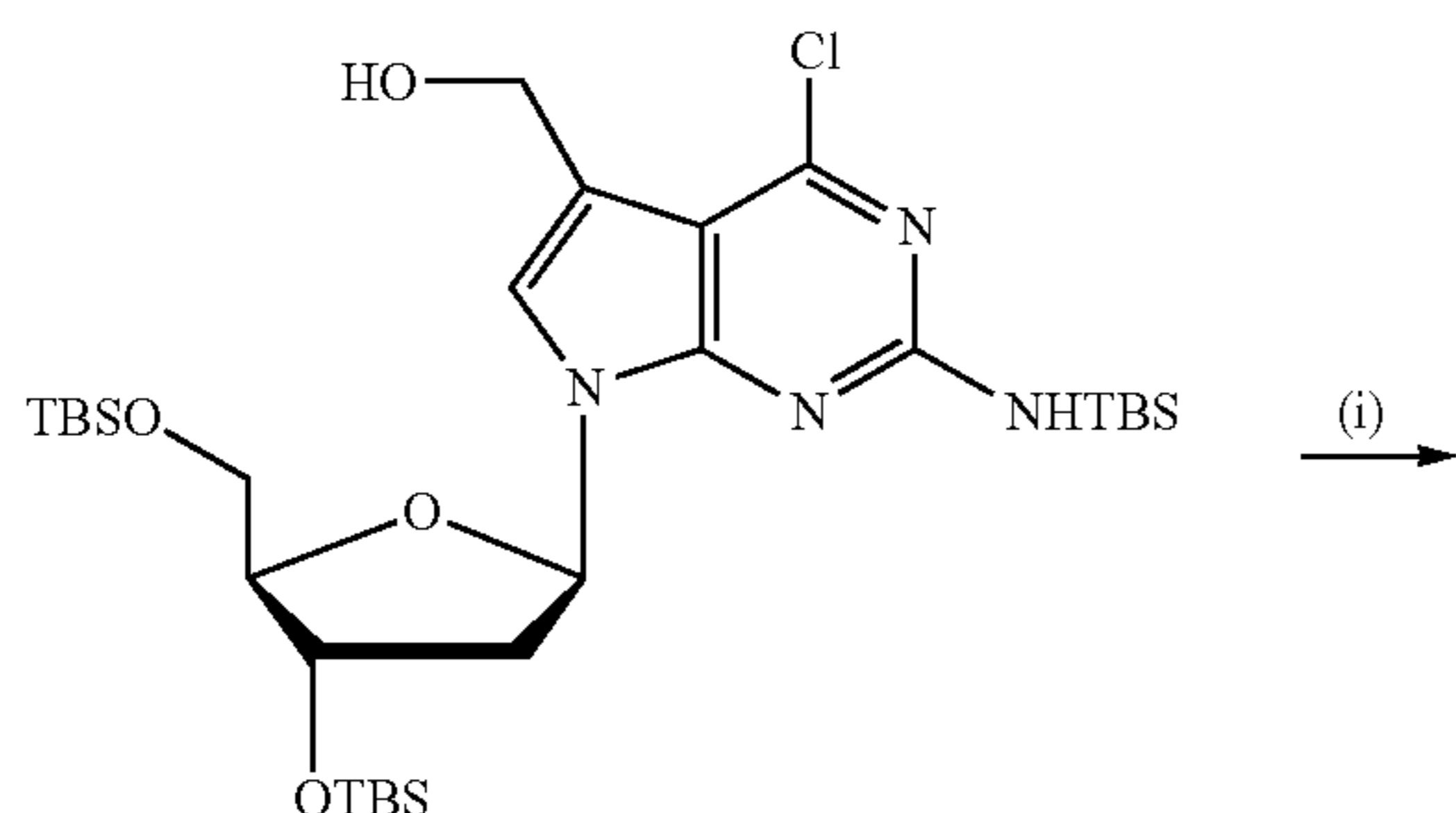
Scheme S17. Synthesis of 7-[1-(4,5-dimethoxy-2-nitrophenyl)-2,2-dimethyl-propyloxy]methyl-7-deaza-2'-deoxyguanosine-5'-triphosphate.
