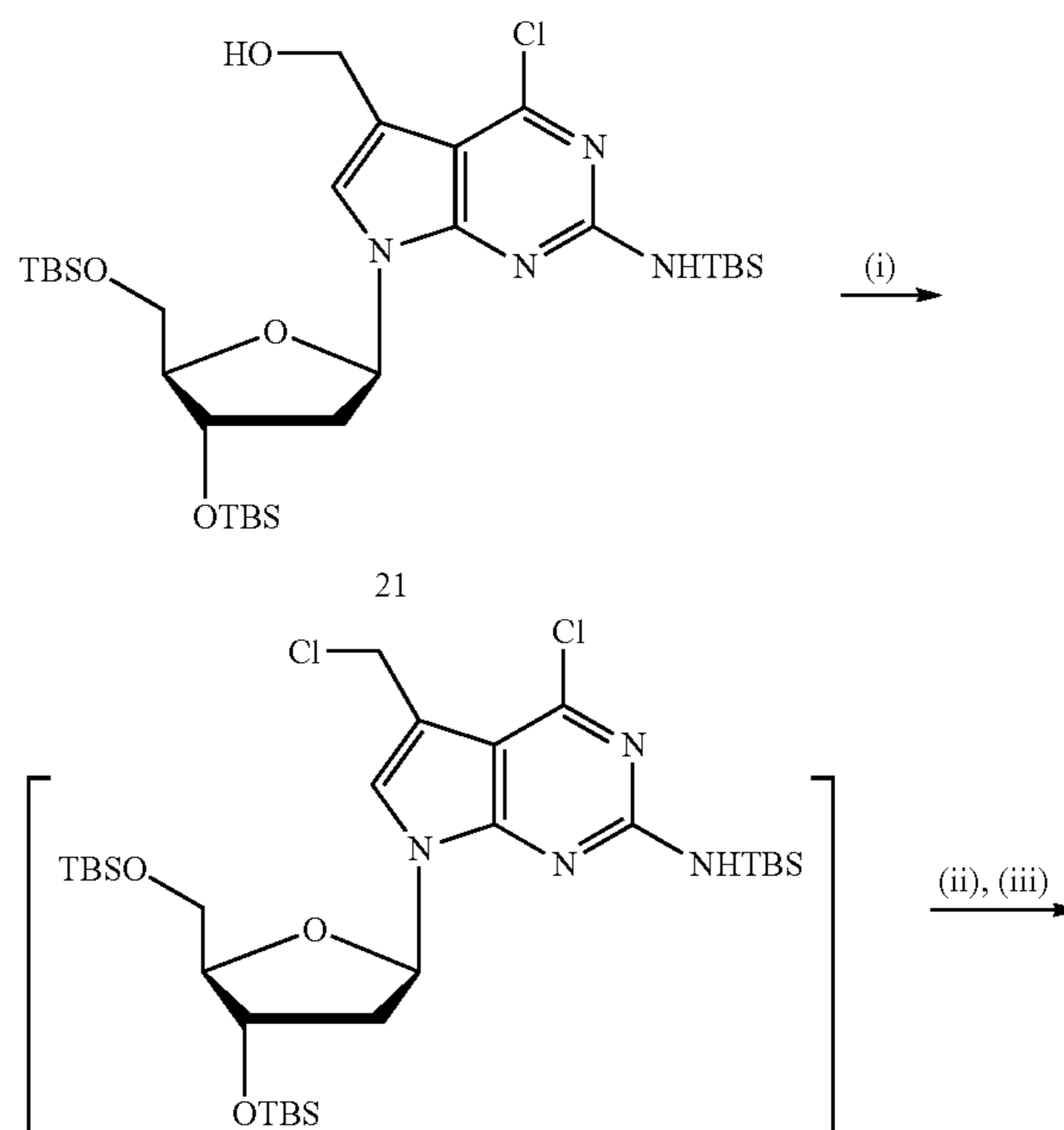
Scheme S18. Synthesis of 7-[(S)-1-(5-methoxy-2-nitrophenyl)-2,2-dimethyl-propyloxy]methyl-7-deaza-2'-deoxyguanosine-5'-triphosphate.
