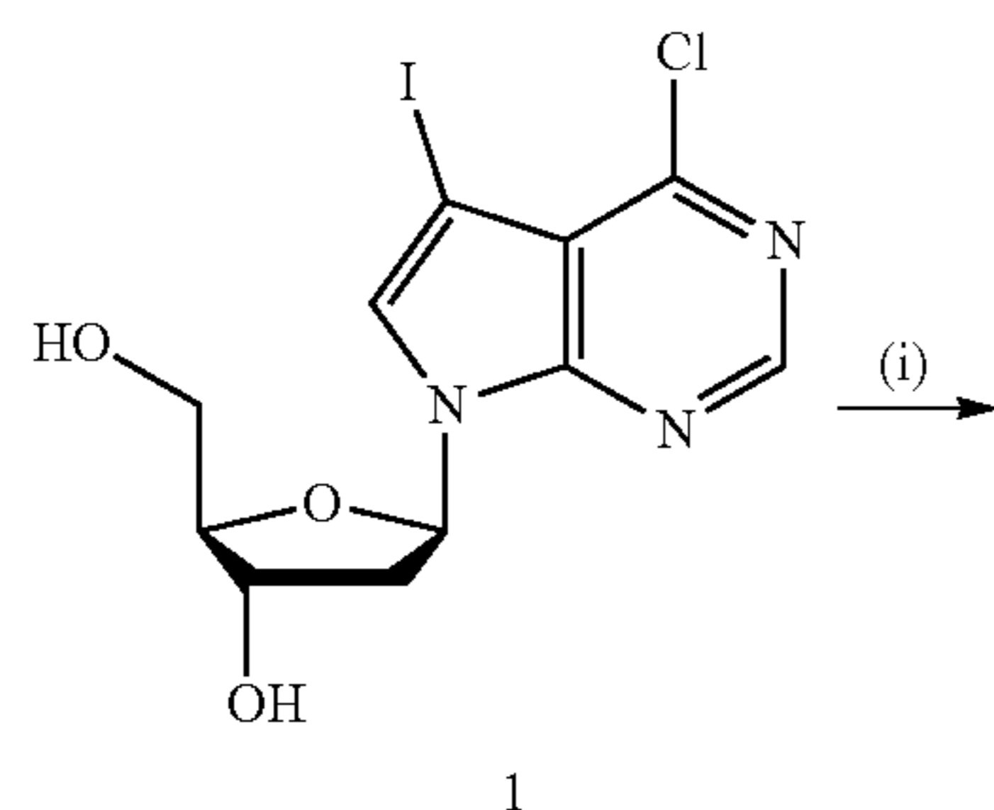
Scheme S6. Synthesis of 7-(2-nitrobenzyloxy)methyl-7-deaza-2'-deoxyadenosine-5'-triphosphate.
