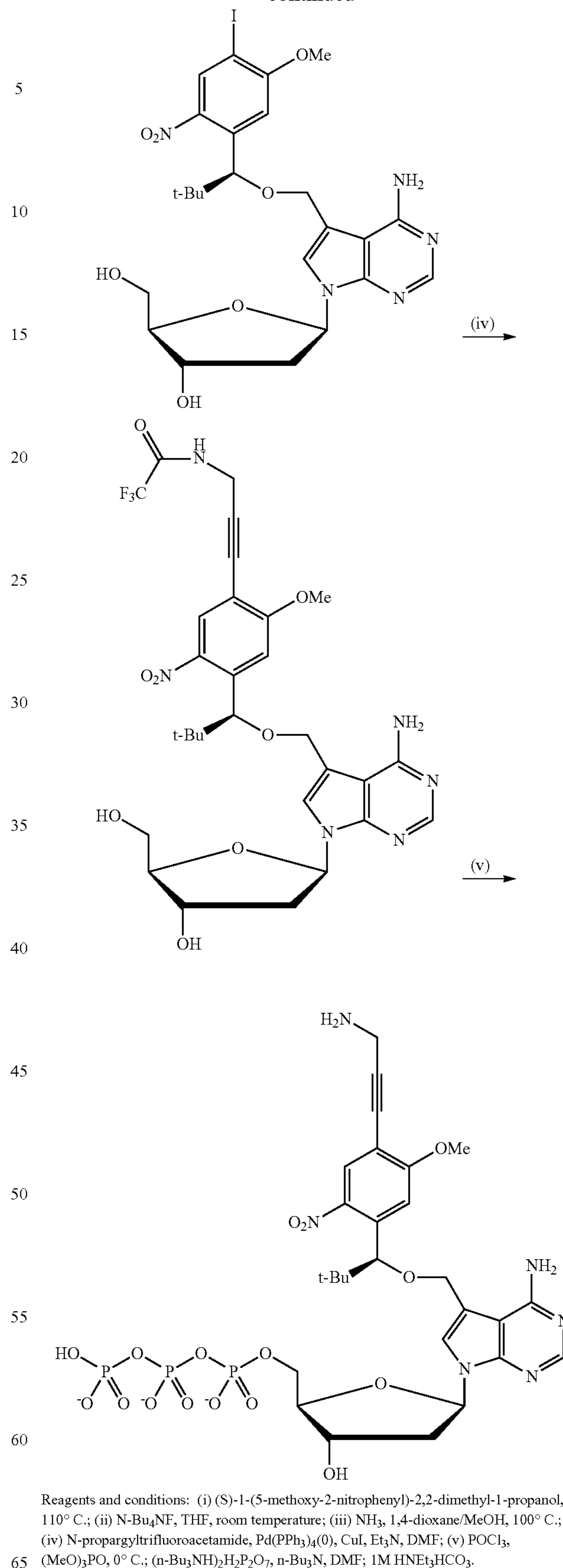
Scheme 2a. Synthesis of dye labeled 7-[(S)-1-(5-methoxy-2-nitrophenyl)- 2,2-dimethyl-propyloxy]methyl-7-deaza-2'-deoxyadenosine-5'- triphosphate.
