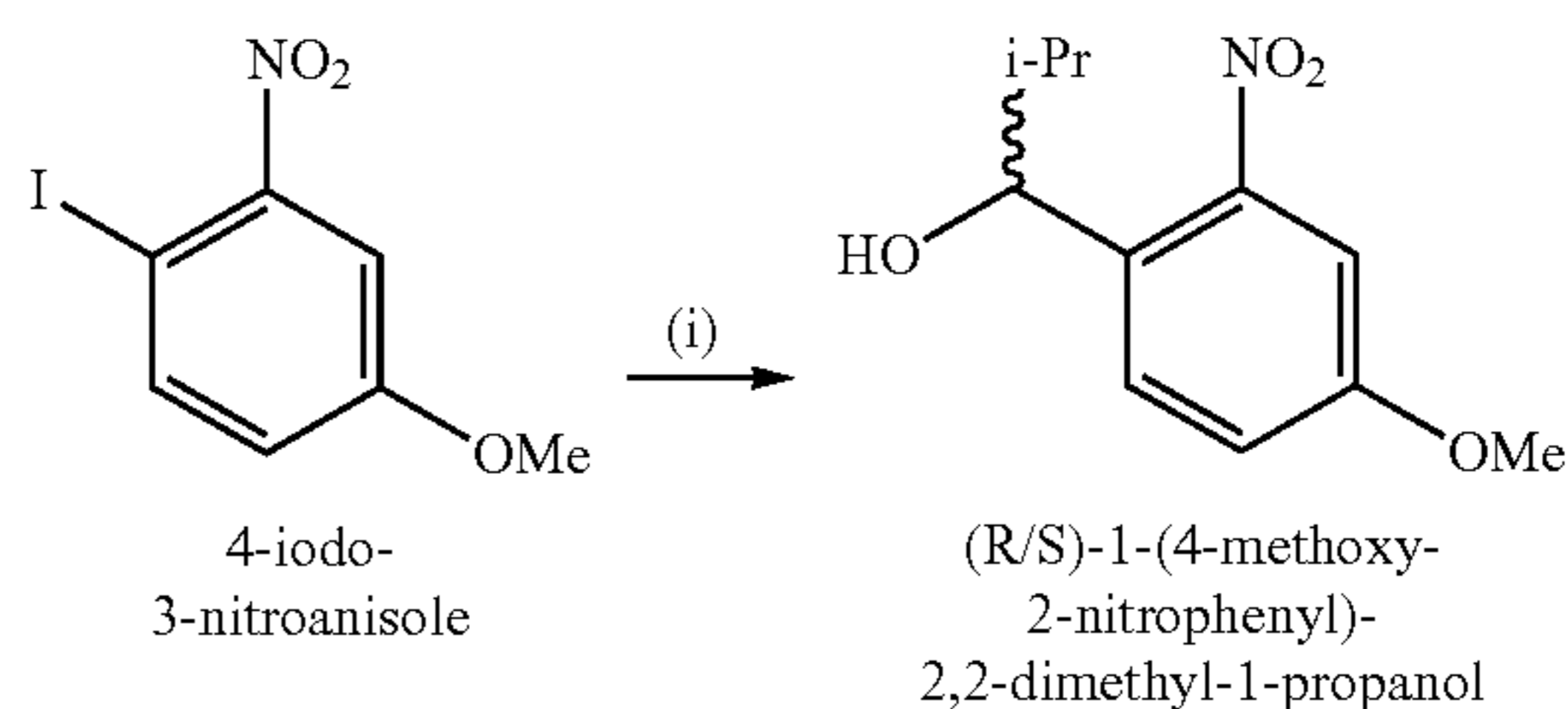
Scheme S3. Synthesis of (R/S)-1-(4-methoxy-2-nitrophenyl)-2,2-dimethyl-1-propanol.
