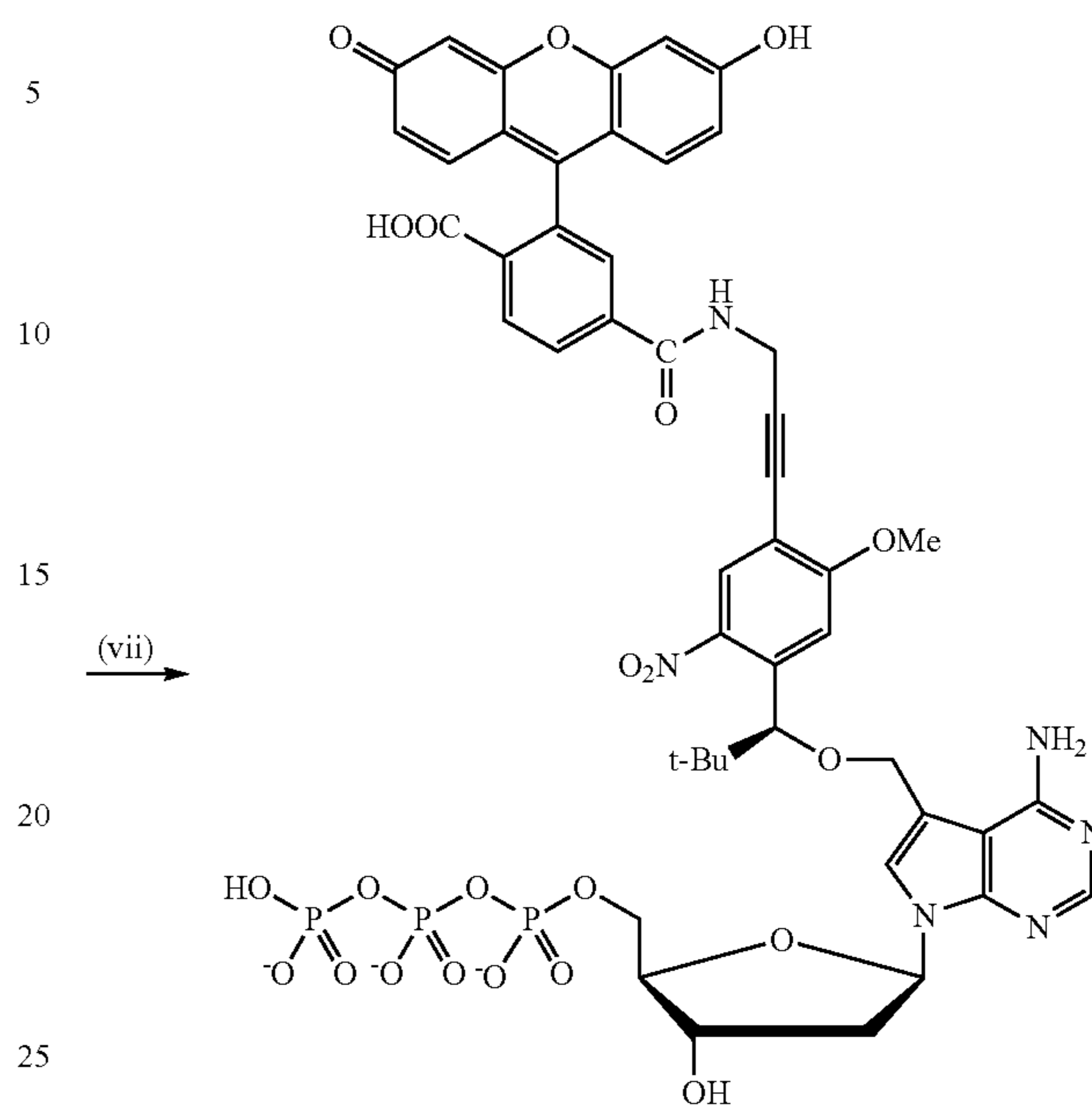
Scheme 2c.
