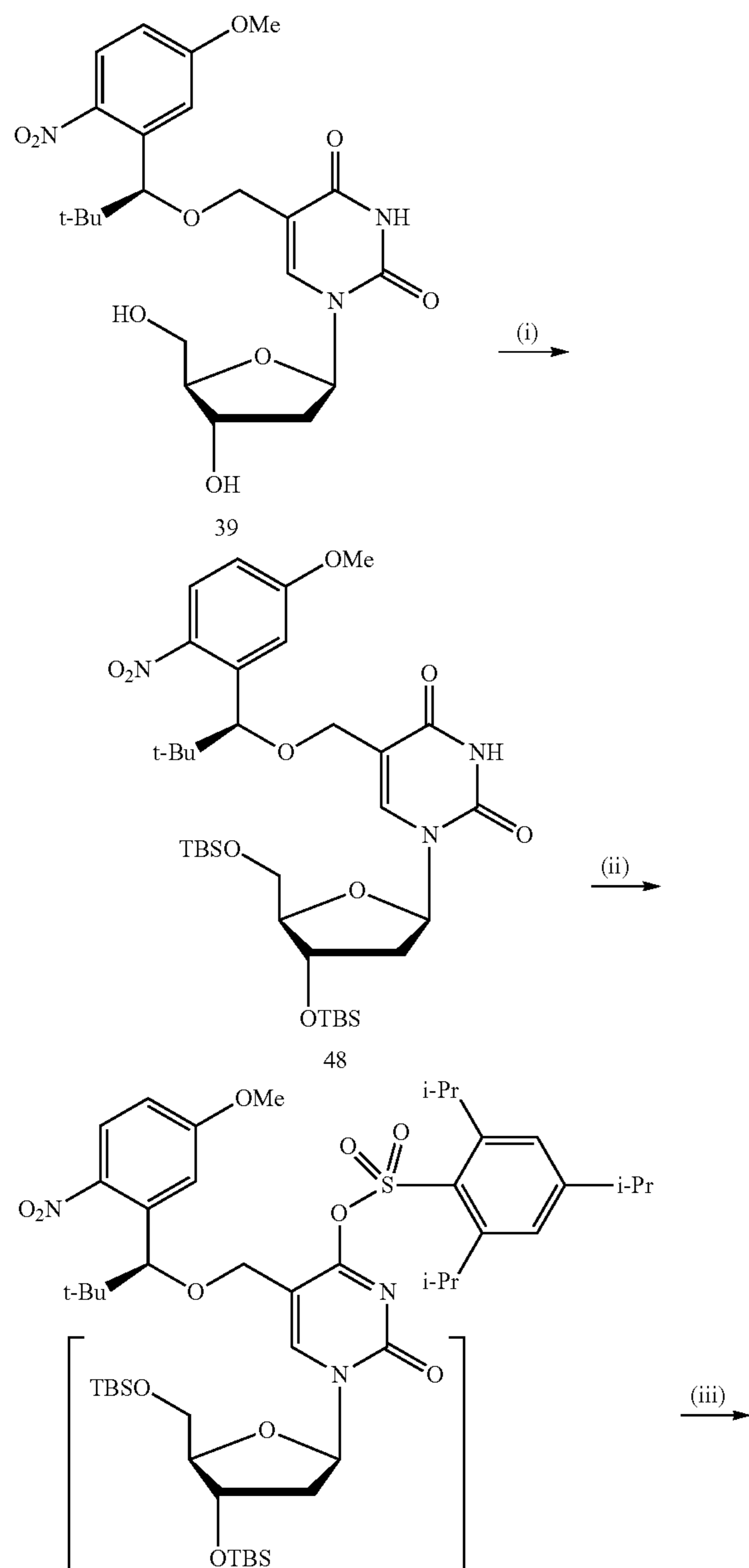
Scheme S22. Synthesis of 5-[(S)-1-(5-methoxy-2-nitrophenyl)-2,2-dimethyl-propyloxy]methyl-2'-deoxycytidine-5'-triphosphate.
