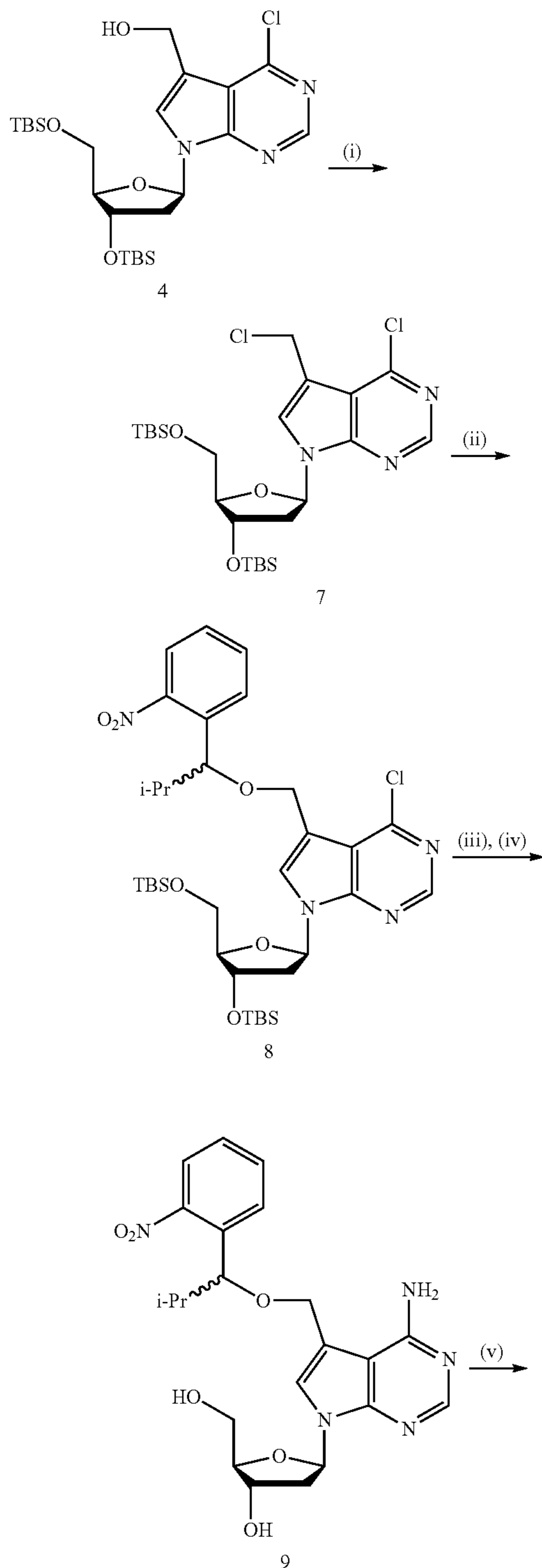
Scheme S7. Synthesis of 7-[1-(2-nitrophenyl)-2-methyl-propyloxy]methyl-7-deaza-2'-deoxyadenosine-5'-triphosphate.
