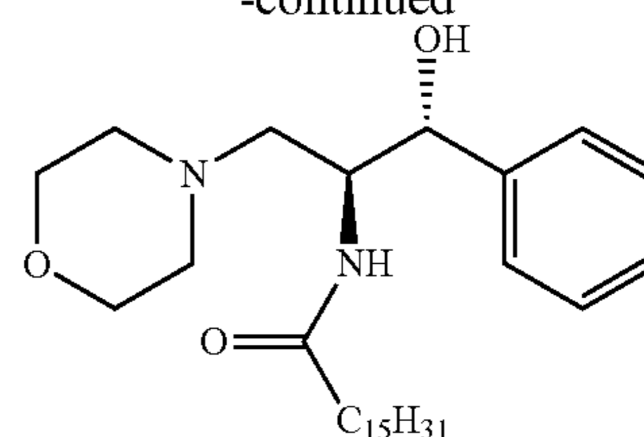
D-erythro-PPMP
