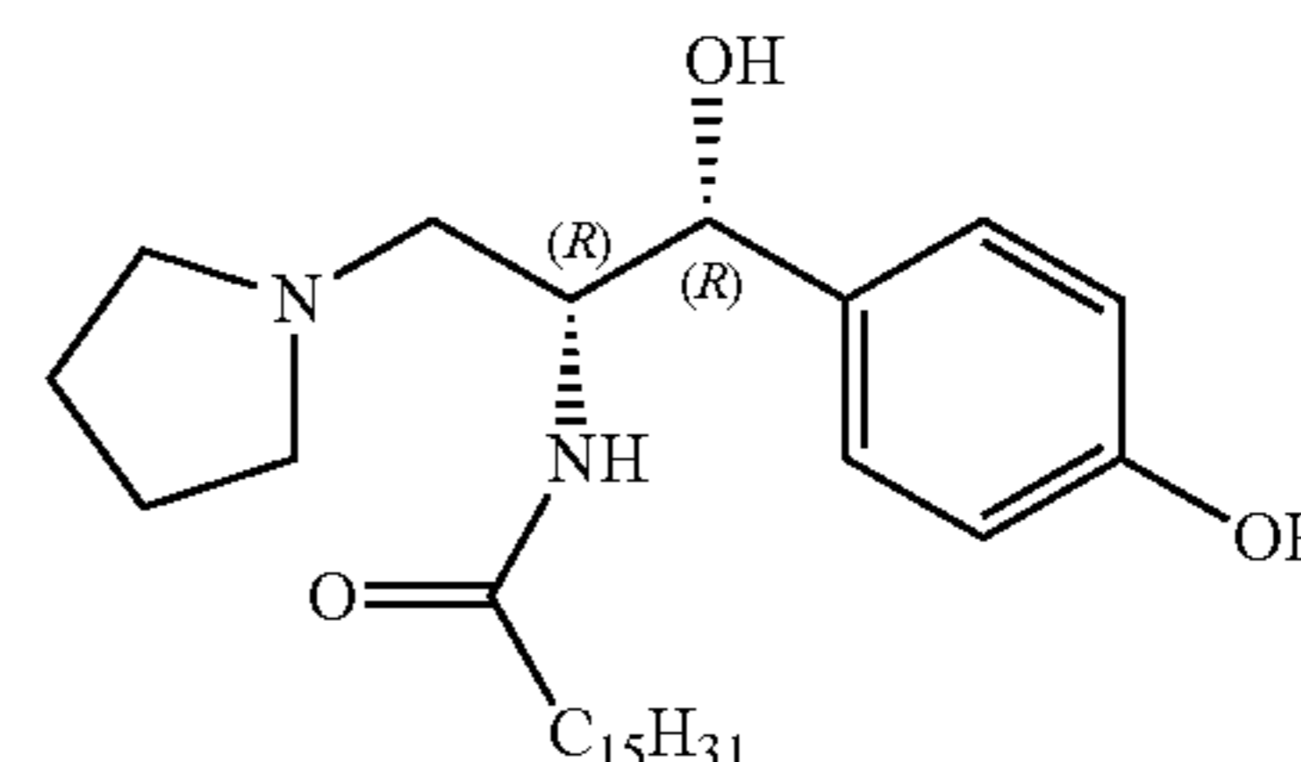
D-threo-4'-hydroxy-P4
