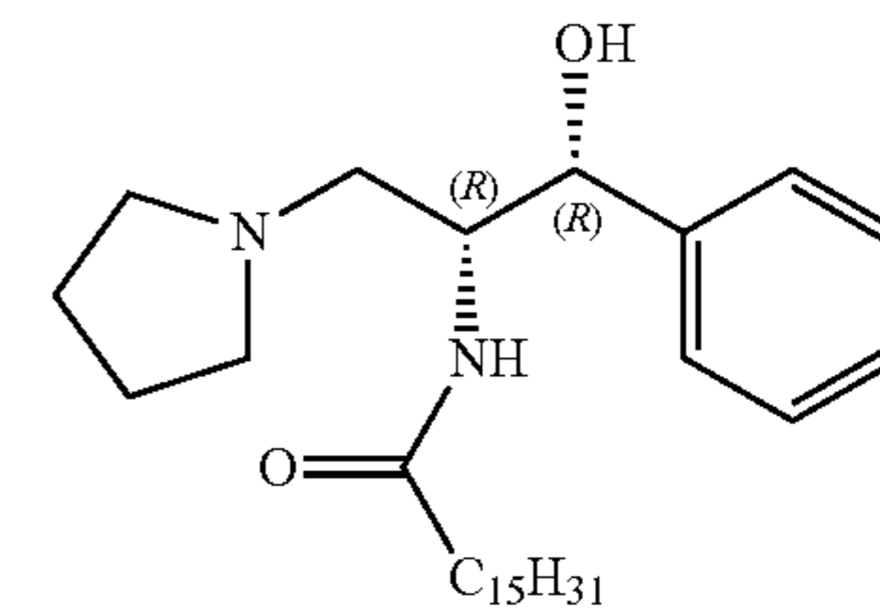
D-threo-P4
