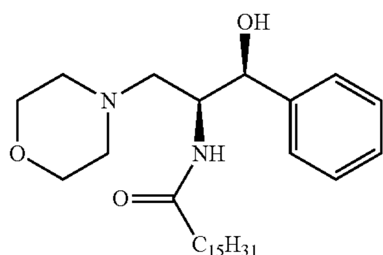
L-threo-PPMP
