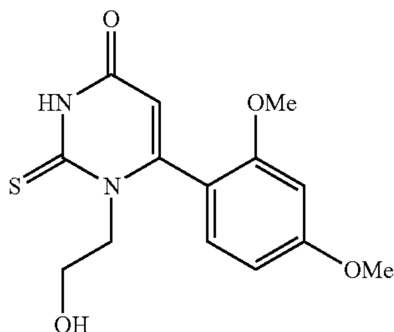
6-(2,4-Dimethoxyphenyl)-1-(2-hydroxyethyl)-2-thioxo-2,3-dihydropyrimidin-4(1H)-one
