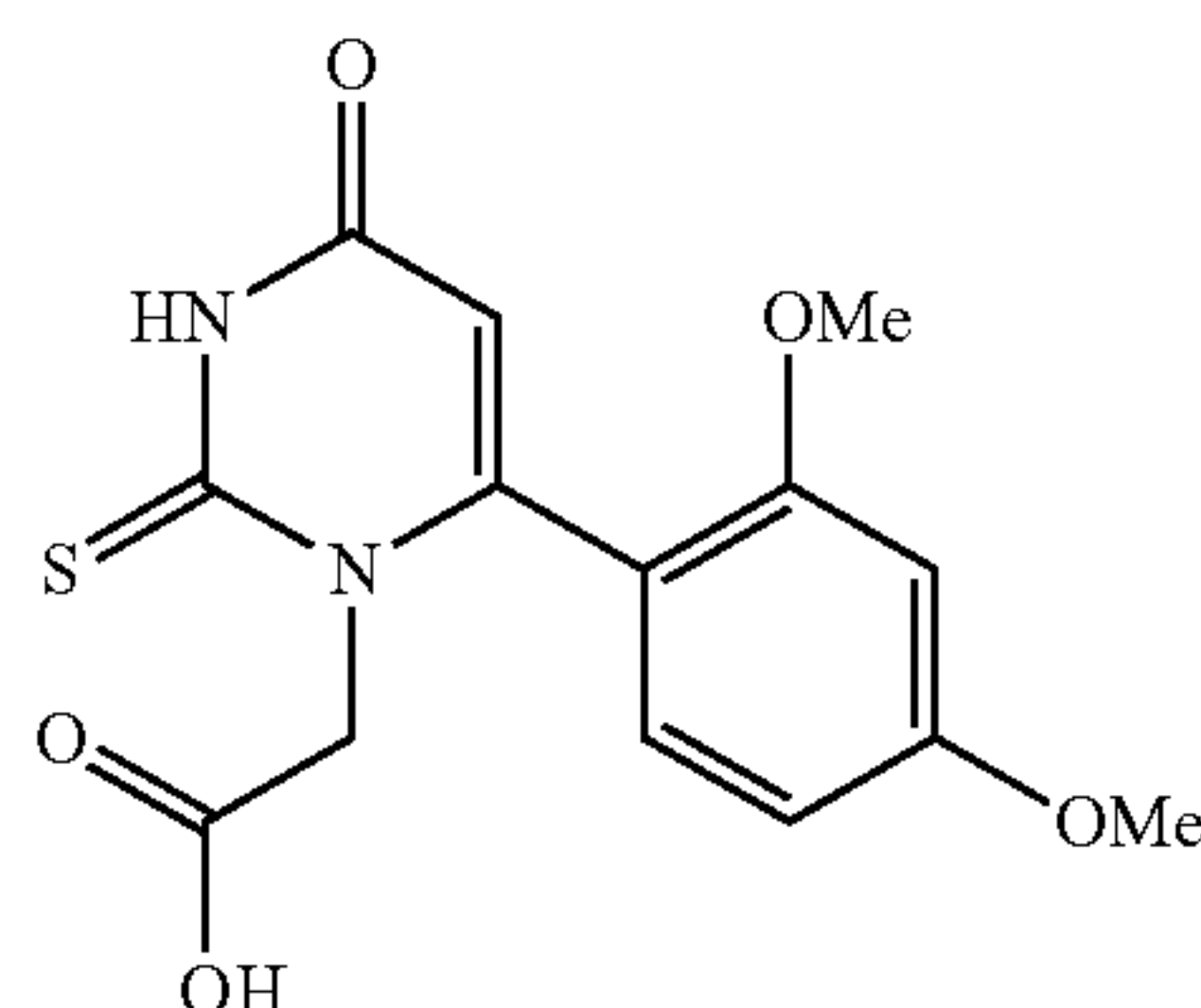
2-(6-(2,4-dimethoxyphenyl)-4-oxo-2-thioxo-3,4-dihydropyrimidin-1(2H)-yl)acetic acid
