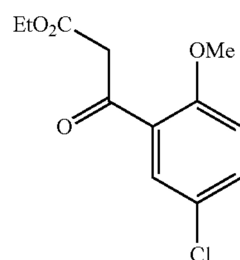
Ethyl 3-(5-chloro-2-methoxyphenyl)-3-oxopropanoate
