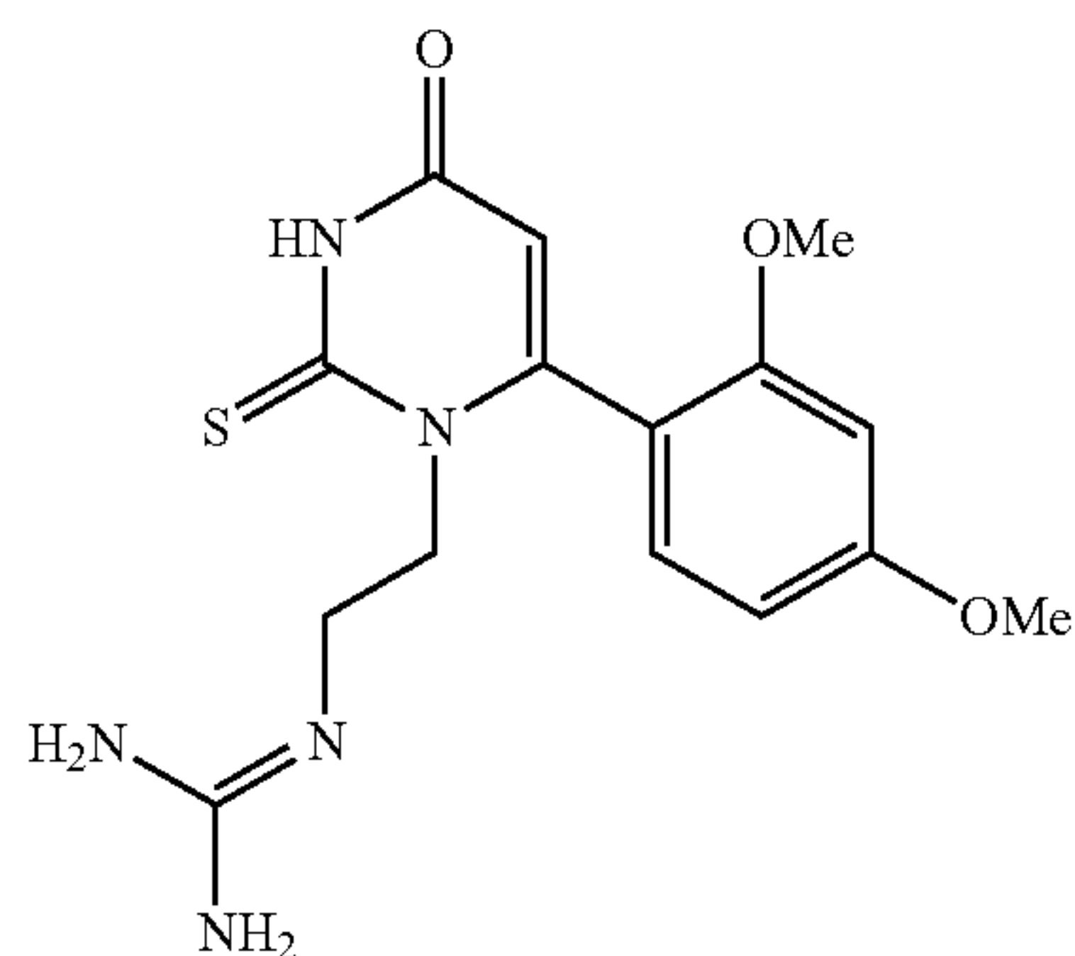
2-(2-(6-(2,4-dimethoxyphenyl)-4-oxo-2-thioxo-3,4-dihydropyrimidin-1(2H)-yl)ethyl)guanidine
