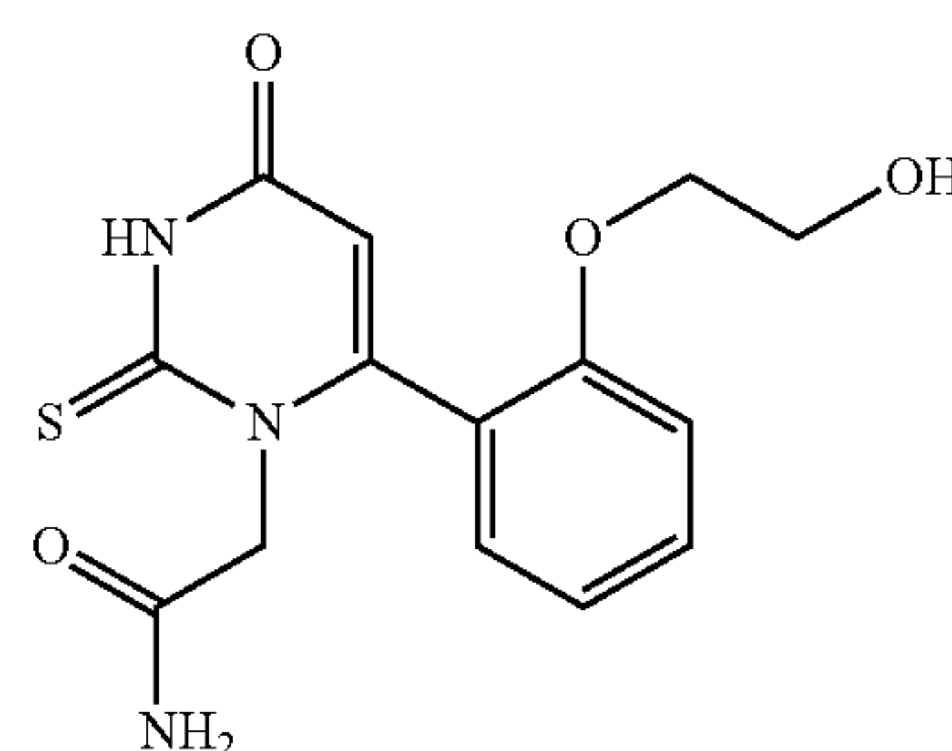
2-(6-(2-(2-Hydroxyethoxy)phenyl)-4-oxo-2-thioxo-3,4-dihydropyrimidin-1(2H)-yl)acetamide
