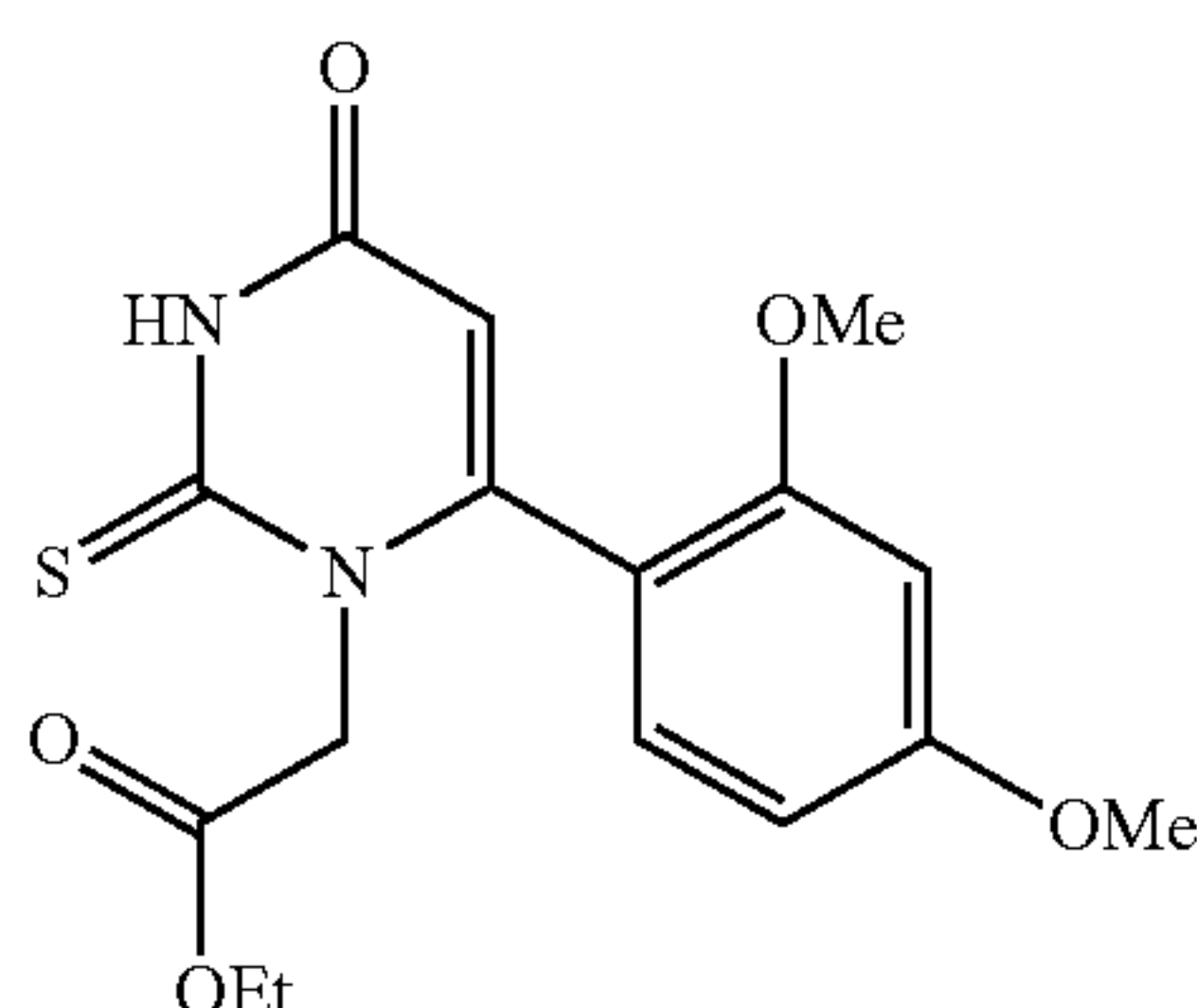
Ethyl 2-(6-(2,4-dimethoxyphenyl)-4-oxo-2-thioxo-3,4-dihydropyrimidin-1(2H)-yl)acetate
