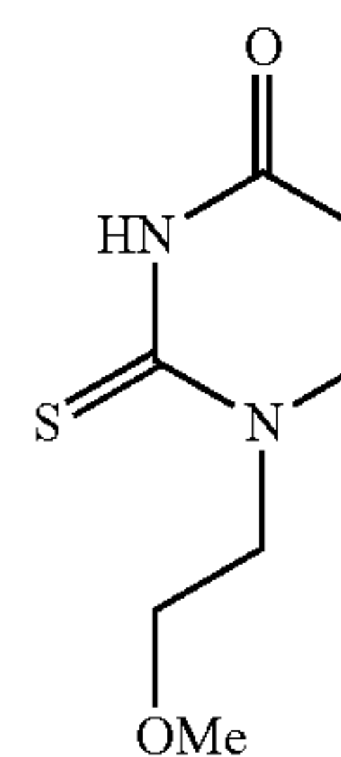
1-(2-Methoxyethyl)-2-thioxo-2,3-dihydropyrimidin-4(1H)-one
