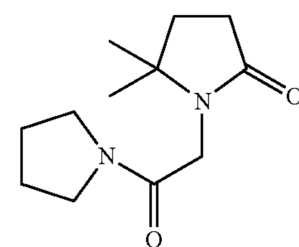
N-[(5,5-dimethyl-2-oxo-pyrrolidino)-acetyl]-pyrrolidine;
