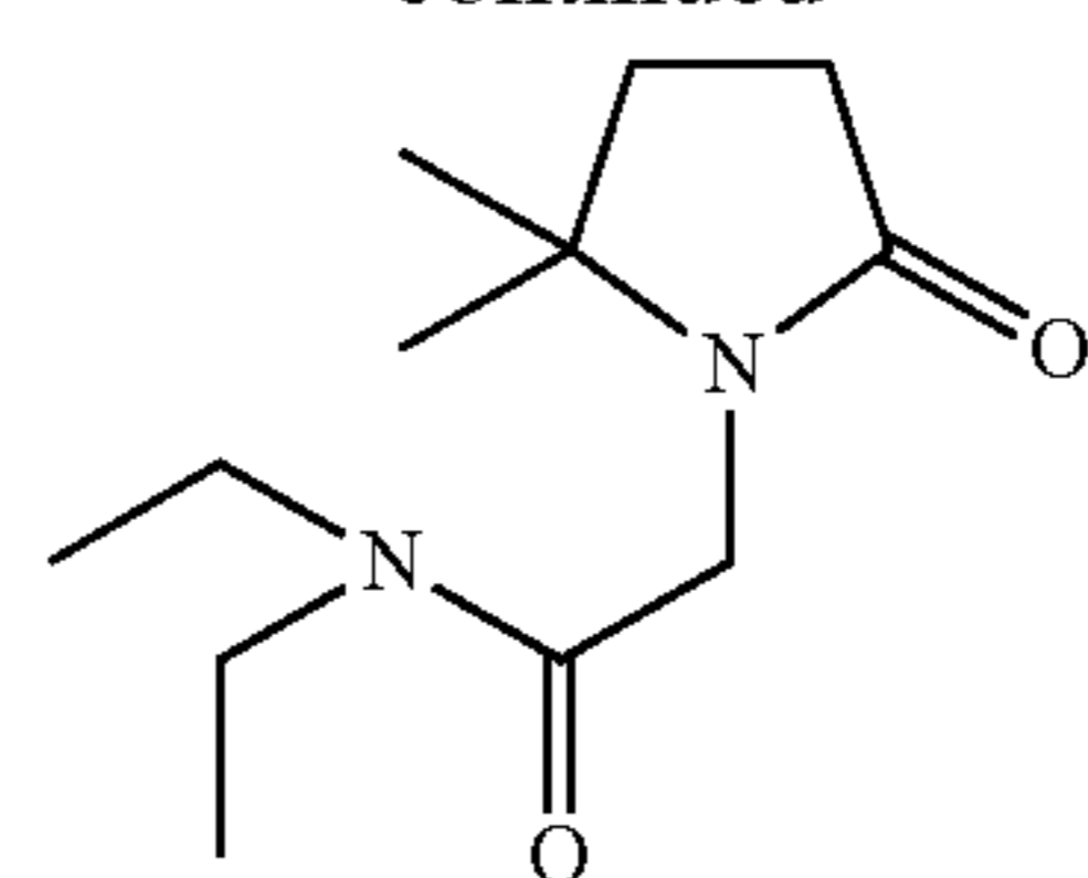
(5,5-dimethyl-2-oxo-pyrrolidino)-N,N-diethylacetamide;
