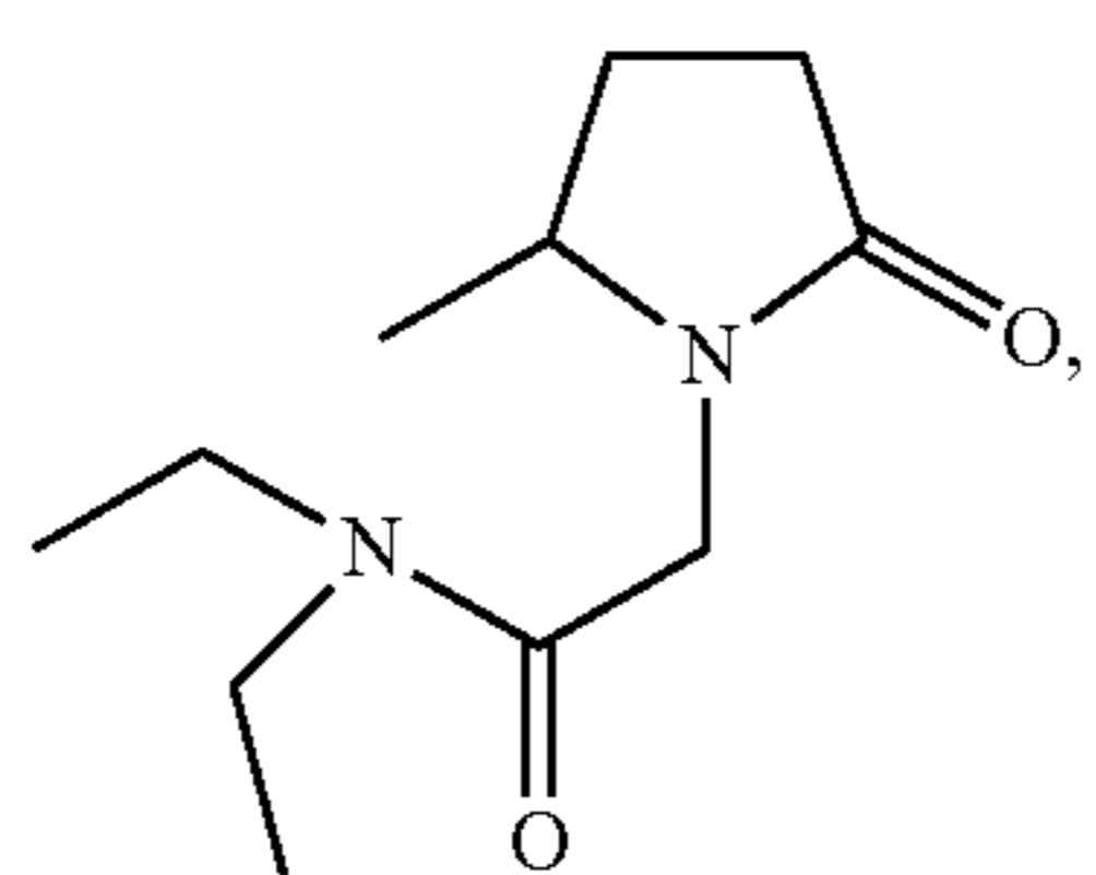
(5-methyl-2-oxo-pyrrolidino)-N,N-diethylacetamide;
