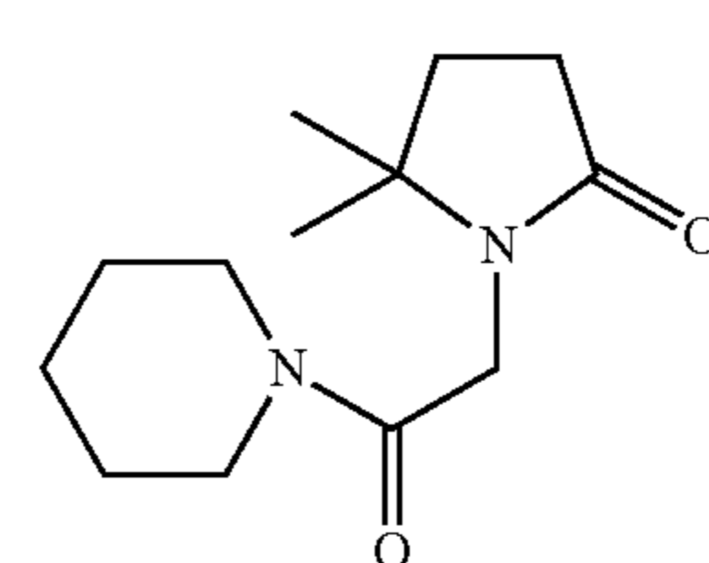
N-[(5,5-dimethyl-2-oxo-pyrrolidino)-acetyl]-pyrrolidine; and
