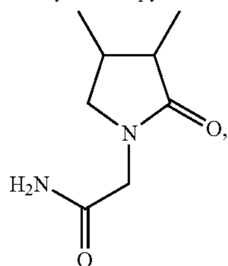
(3,4-dimethyl-2-oxo-pyrrolidino)-acetamide;
