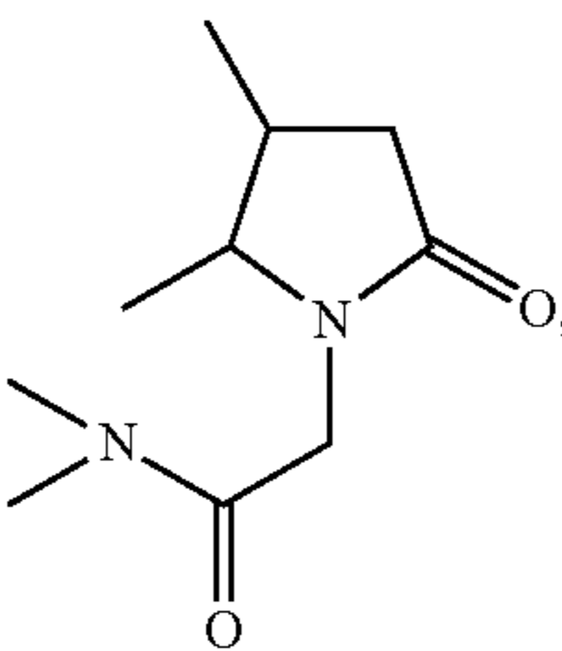
(4,5-dimethyl-2-oxo-pyrrolidino)-N,N-dimethylacetamide;
