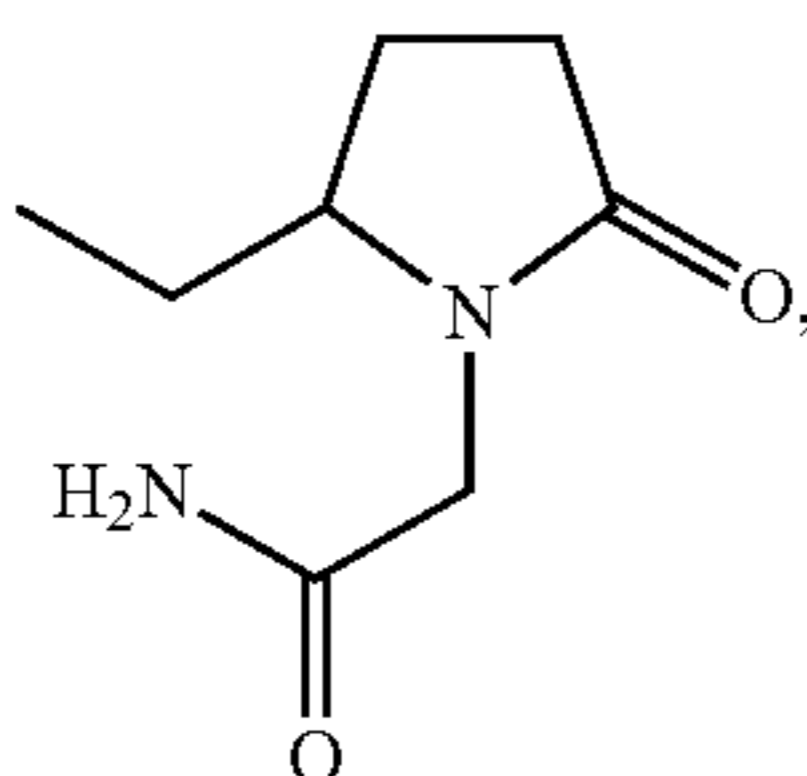
(5-ethyl-2-oxo-pyrrolidino)-acetamide;
