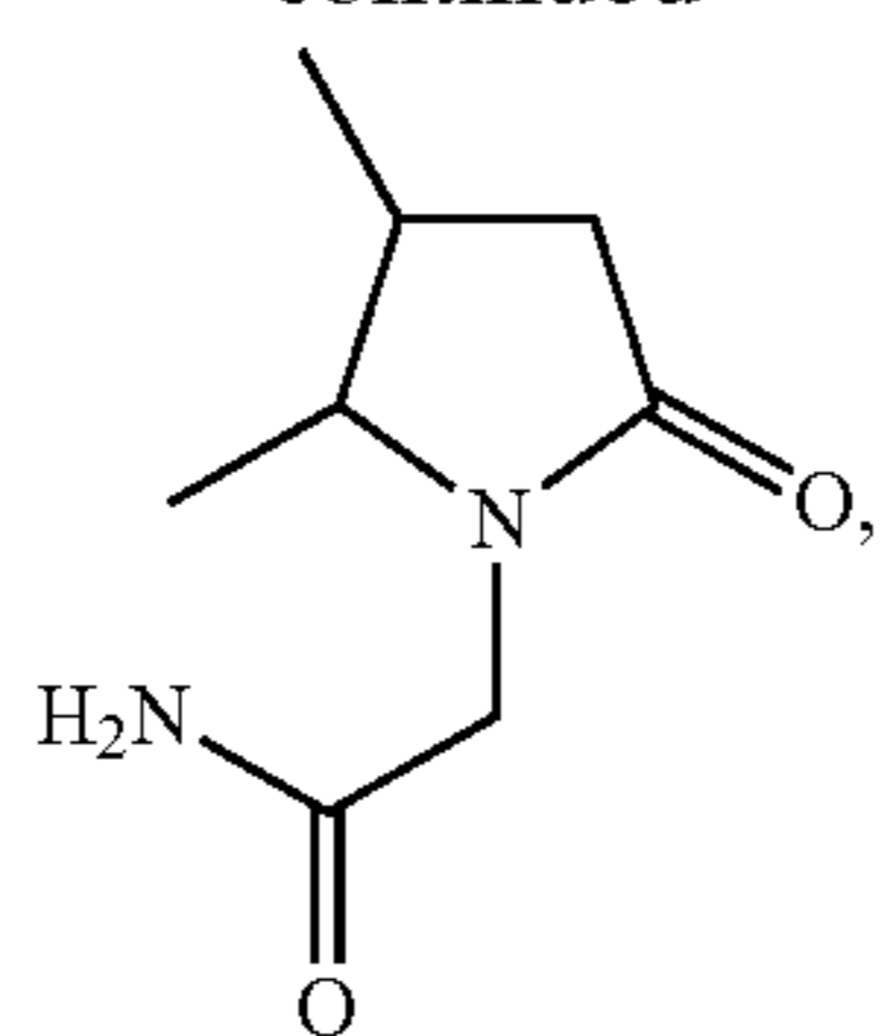
(4,5-dimethyl-2-oxo-pyrrolidino)-acetamide;
