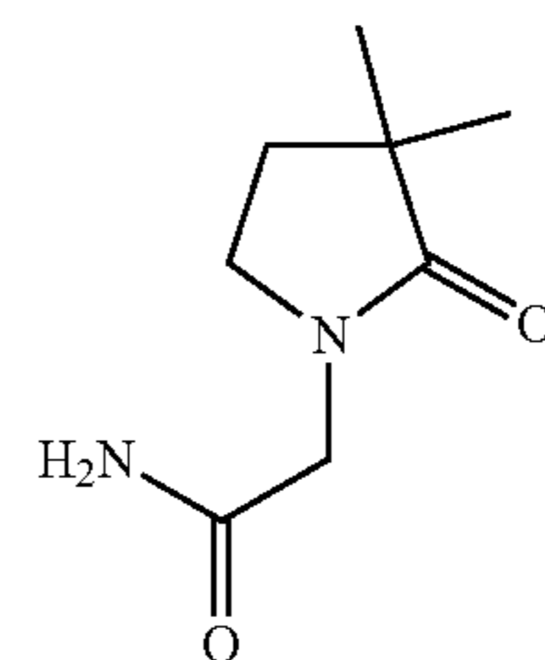
(3,3-dimethyl-2-oxo-pyrrolidino)-acetamide;
