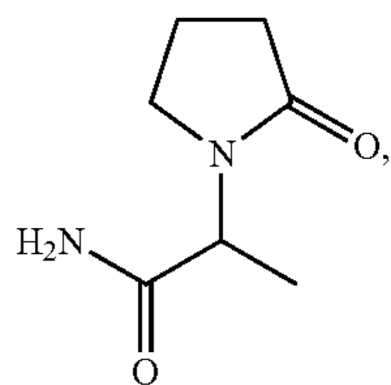
2-(2-oxo-pyrrolidino)-propionamide;
