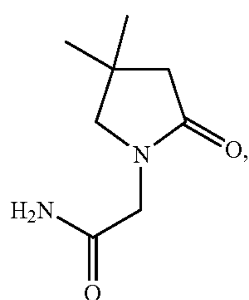
(4,4-dimethyl-2-oxo-pyrrolidino)-acetamide;
