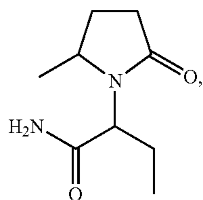
2-(5-methyl-2-oxo-pyrrolidino)-butyramide;
