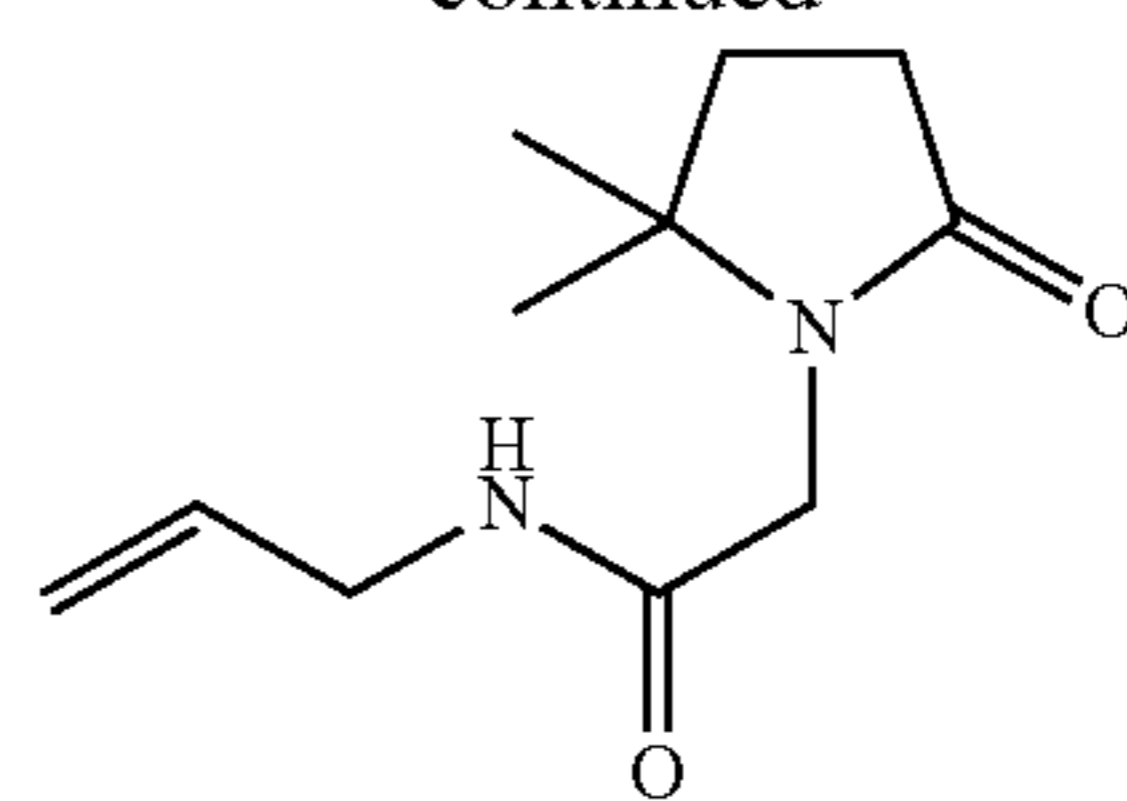
N-allyl-(5,5-dimethyl-2-oxo-pyrrolidino)-acetamide;
