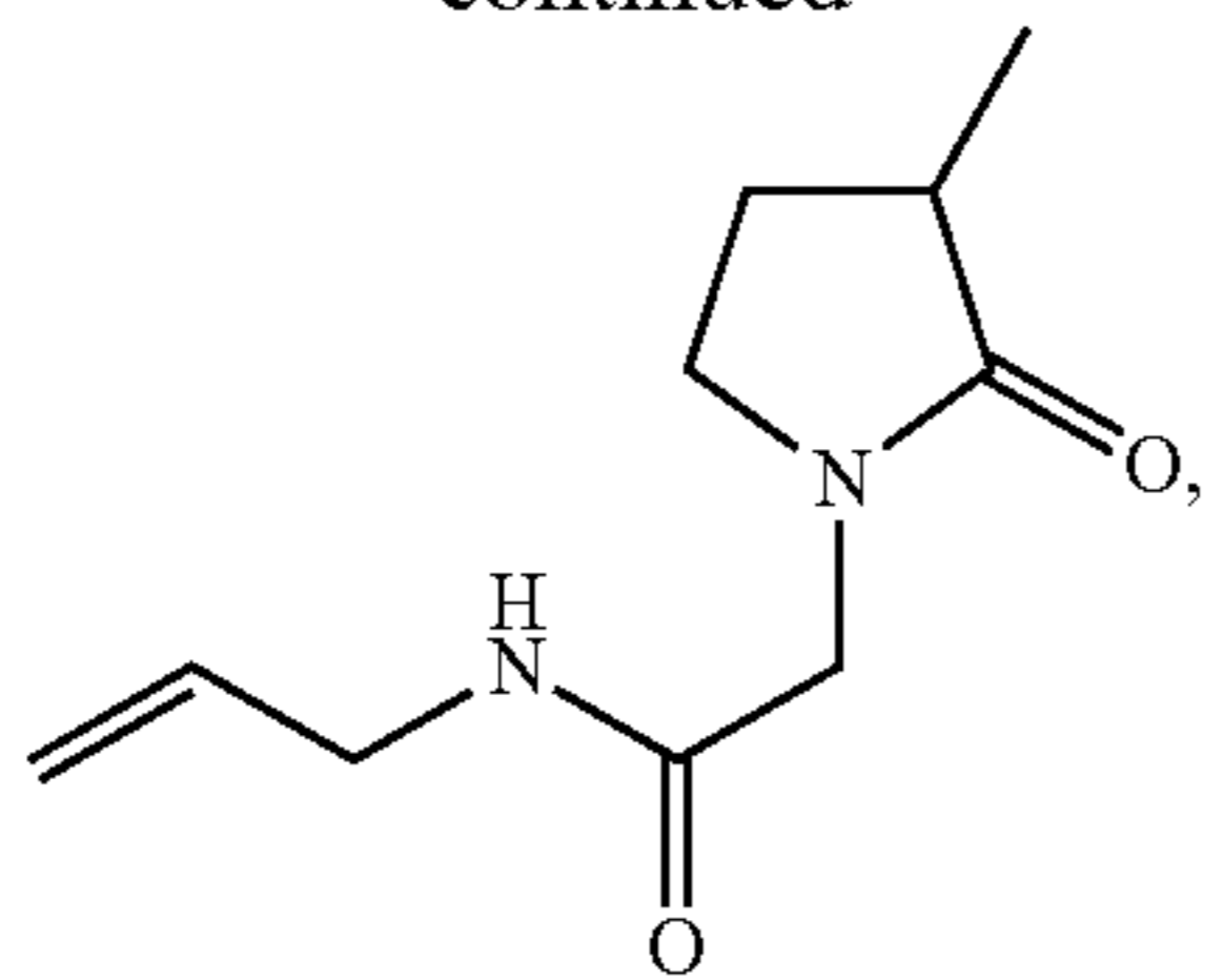
N-allyl-(3-methyl-2-oxo-pyrrolidino)-acetamide;
