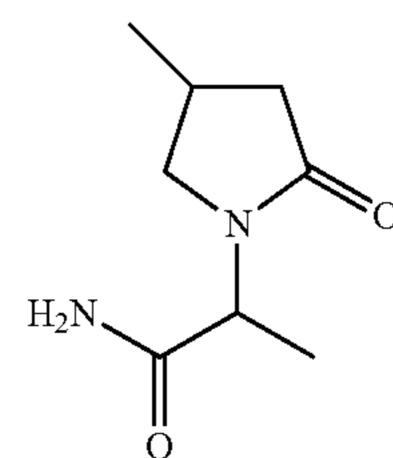
2-(4-methyl-2-oxo-pyrrolidino)-propionamide;
