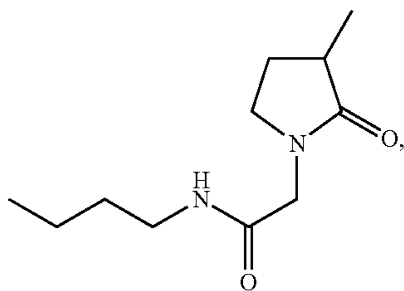
N-n-butyl-(3-methyl-2-oxo-pyrrolidino)-acetamide;
