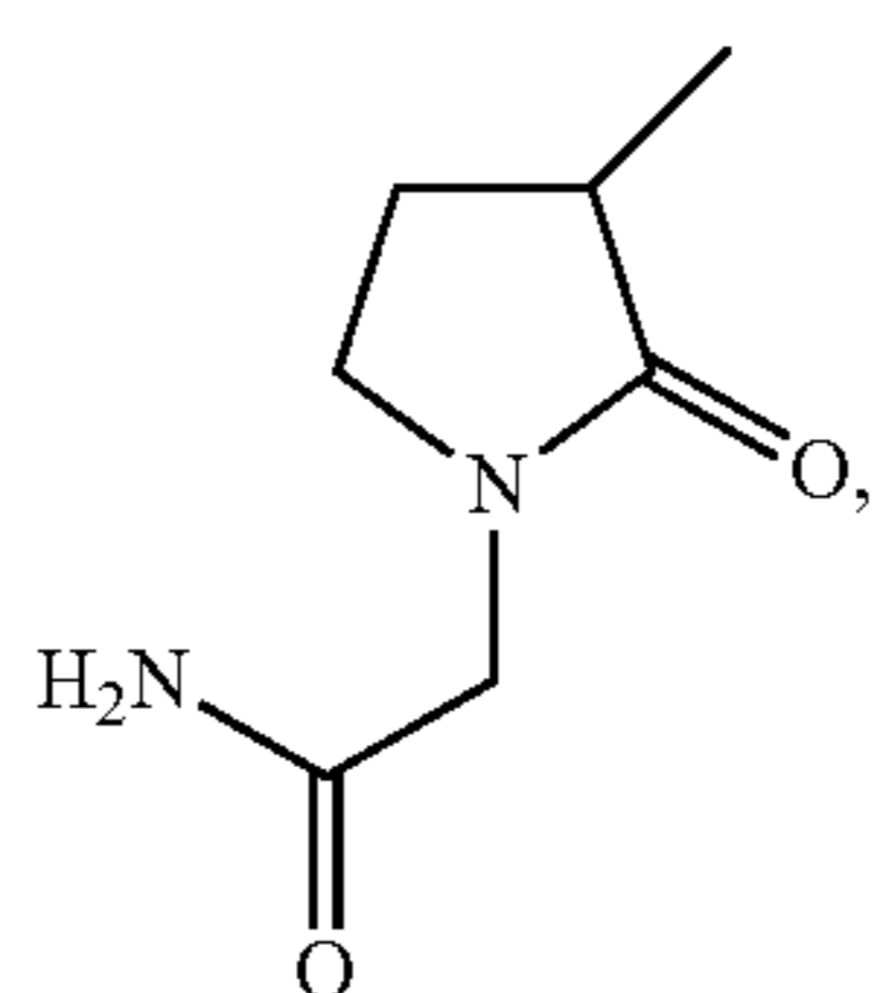
(3-methyl-2-oxo-pyrrolidino)-acetamide;
