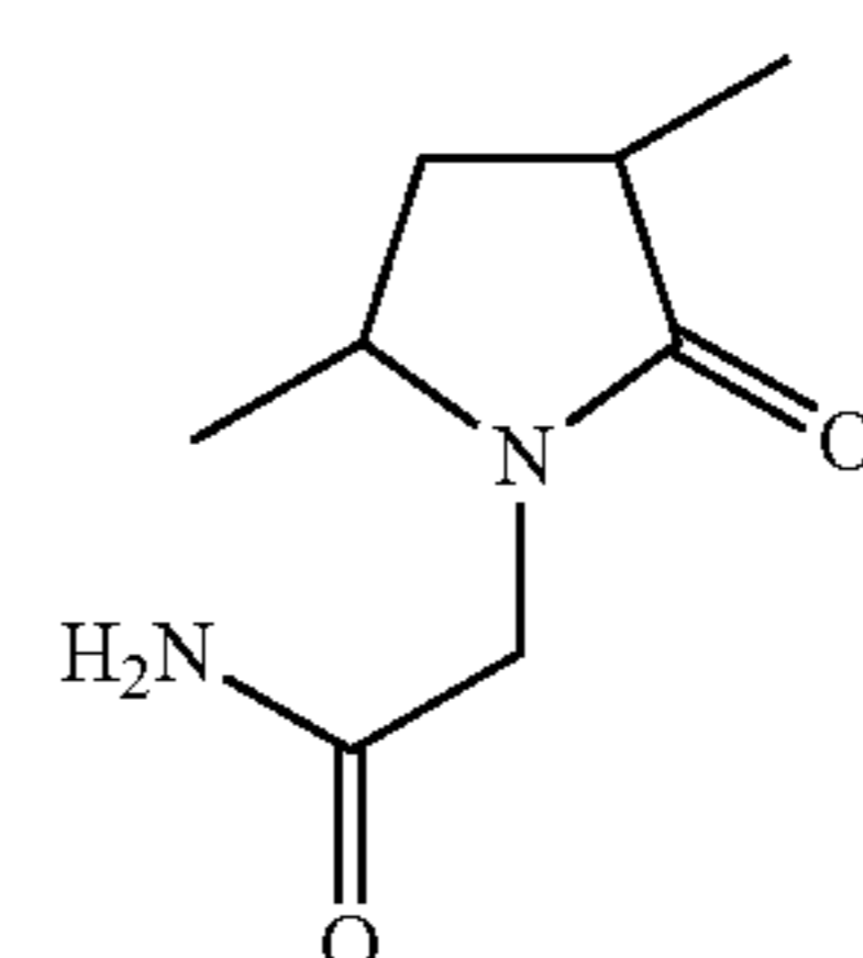
(3,5-dimethyl-2-oxo-pyrrolidino)-acetamide;
