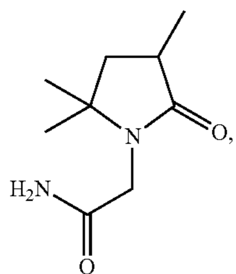
(3,5,5-trimethyl-2-oxo-pyrrolidino)-acetamide;
