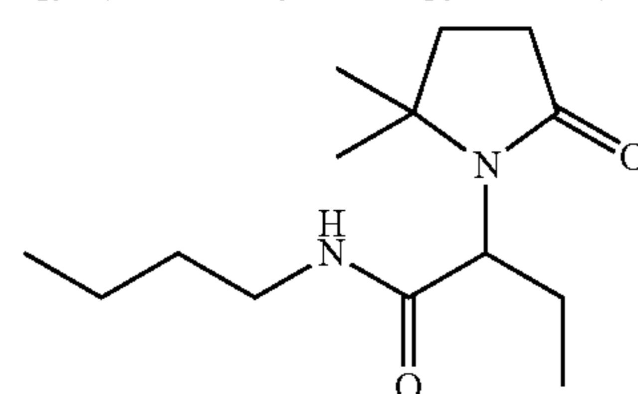
N-n-butyl-2-(5,5-dimethyl-2-oxo-pyrrolidino)-butyramide;
