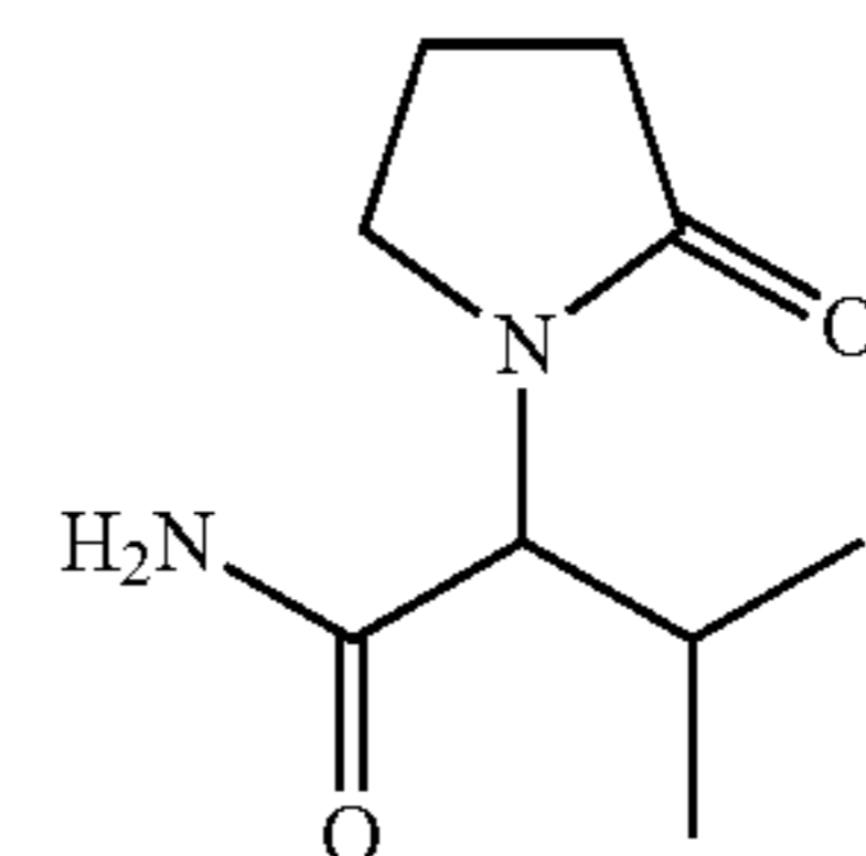
2-(2-oxo-pyrrolidino)-3-methyl-butyramide;
