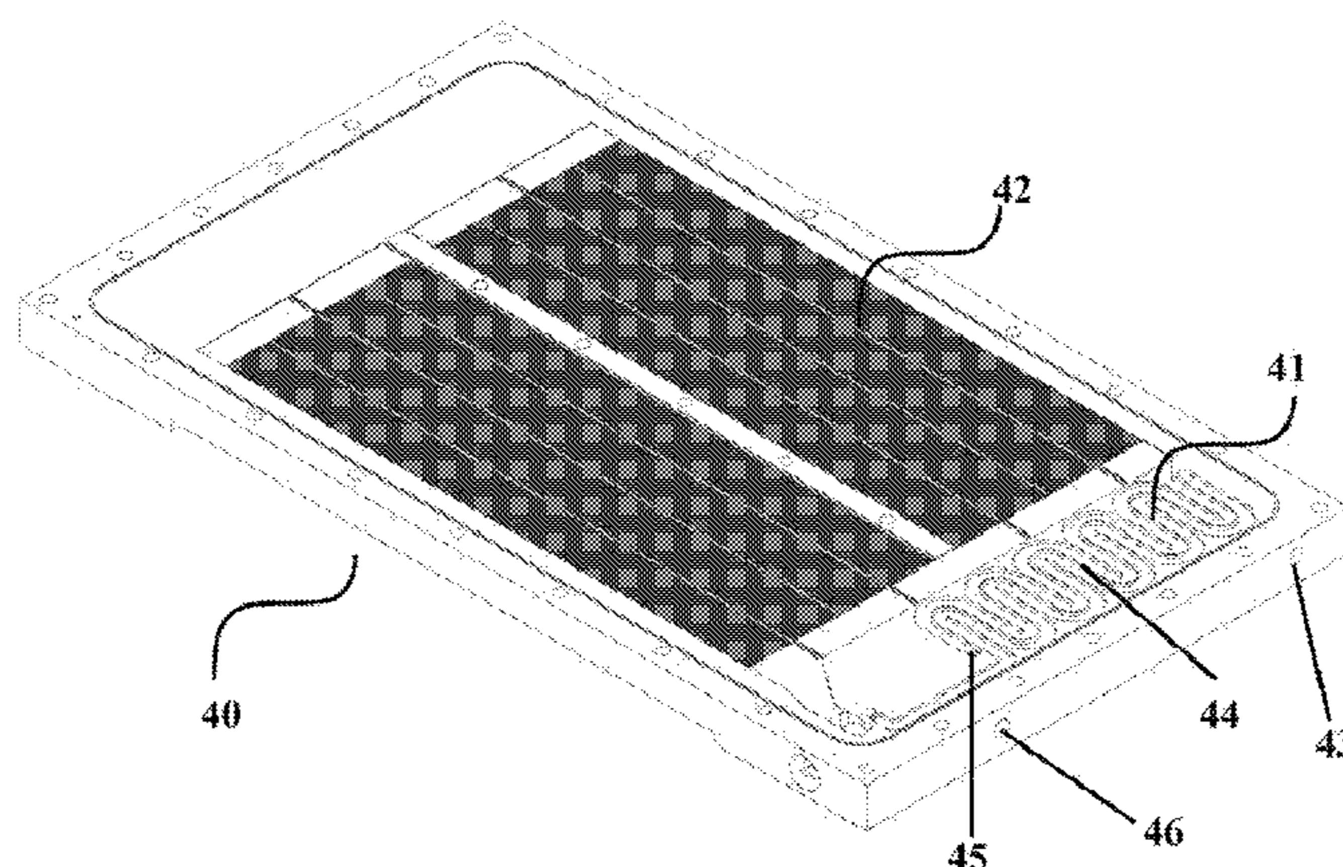
Alternative embodiment of the Current Invention of Integrating the TXV and Sensing Bulb within Each of a Plurality of Evaporative Cold Plates with a recuperative heat exchanger
