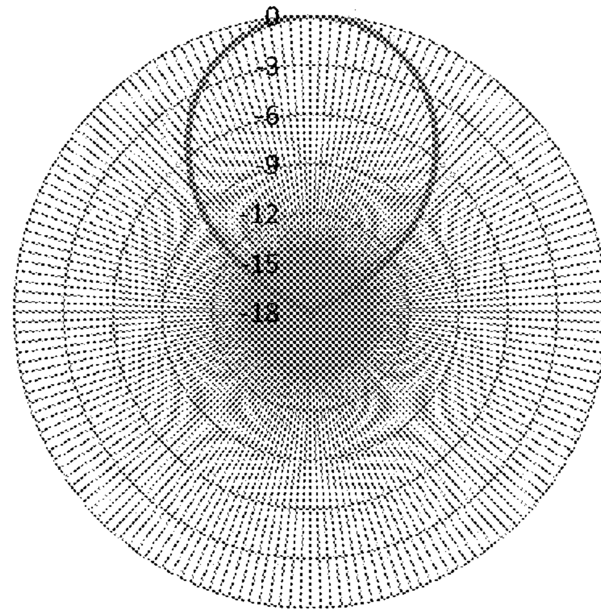
Normalized Azimuth Pattern - Vertically Polarized in dB
