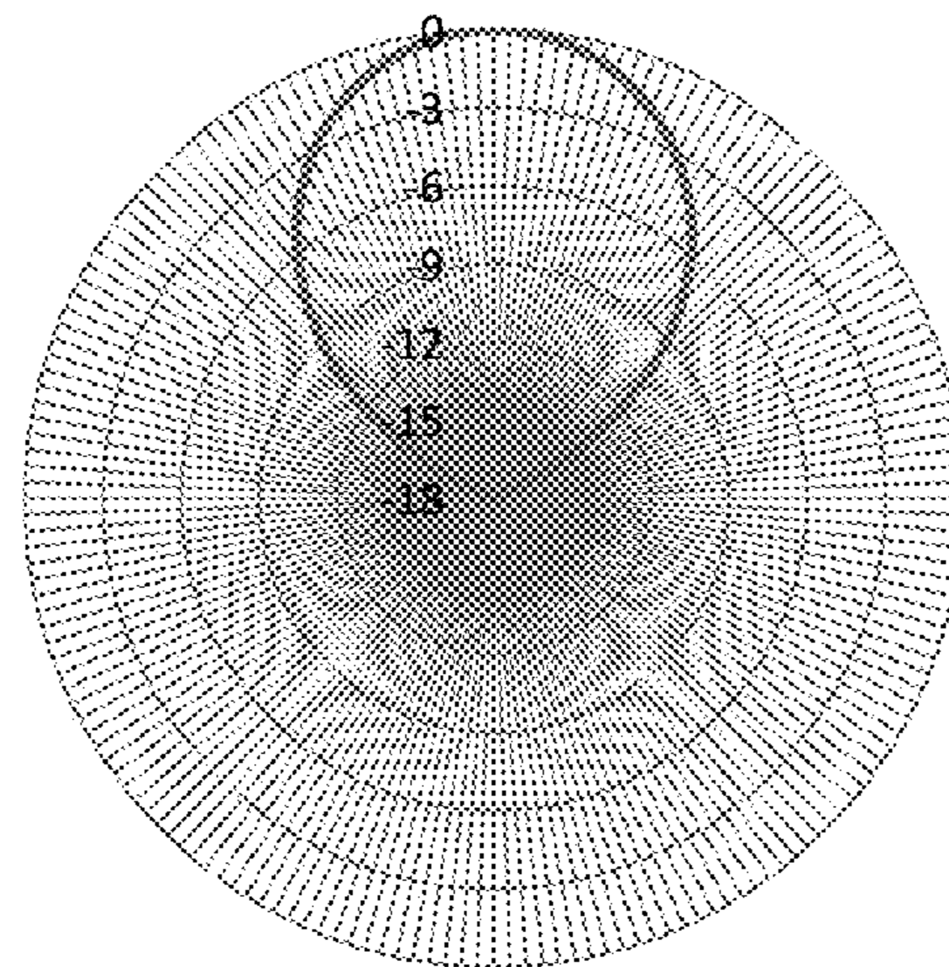
Normalized Elevation Pattern - Horizontally Polarized in dB
