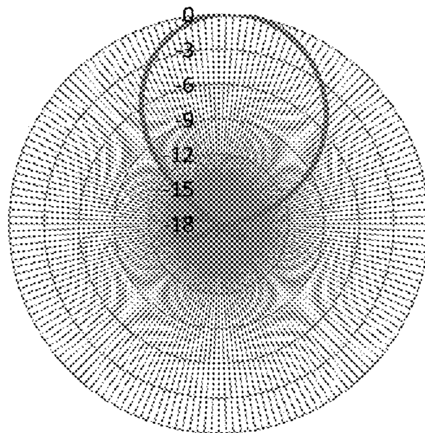
Normalized Elevation Pattern - Vertically Polarized in dB
