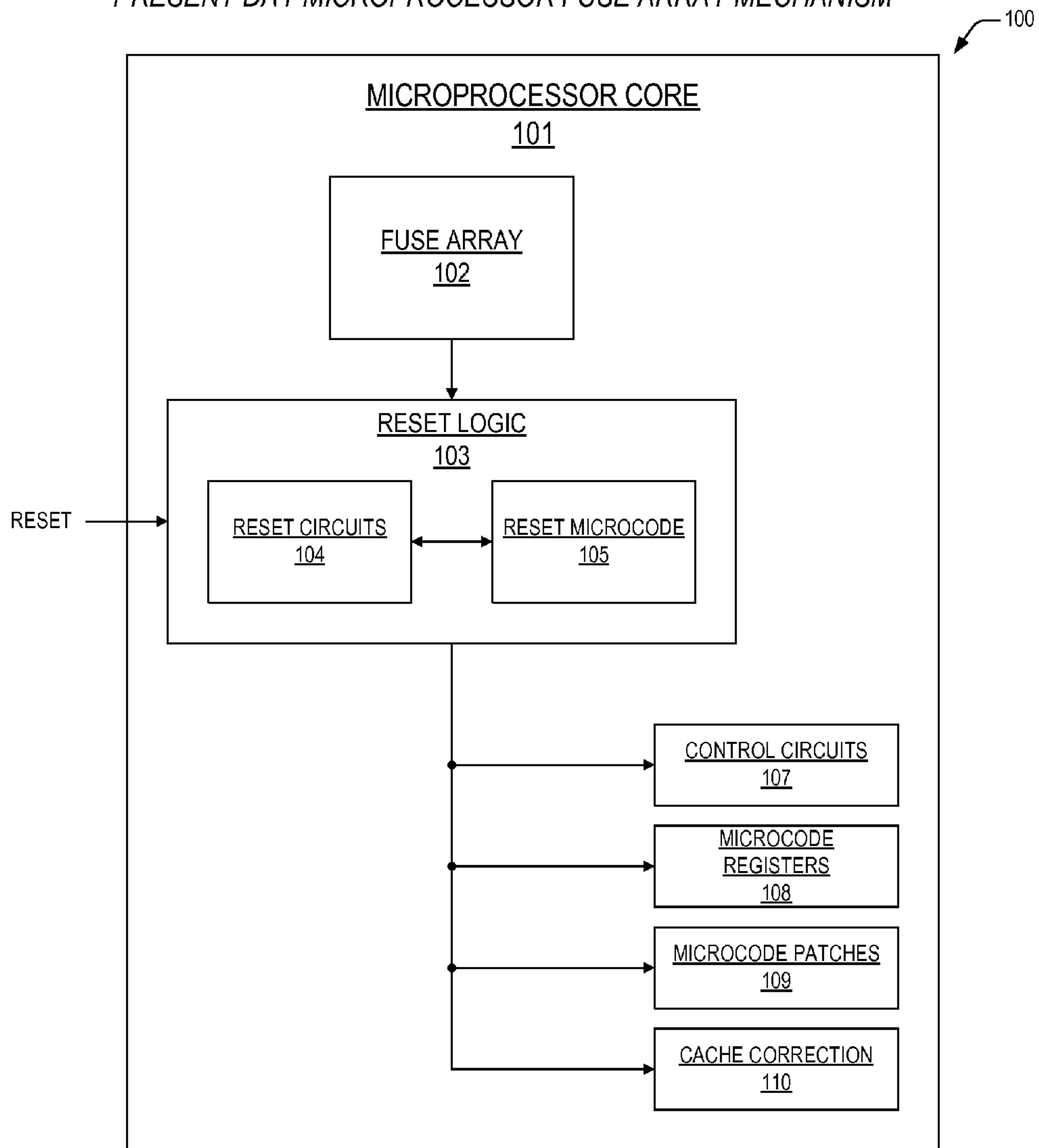
PRESENT DAY MICROPROCESSOR FUSE ARRAY MECHANISM
