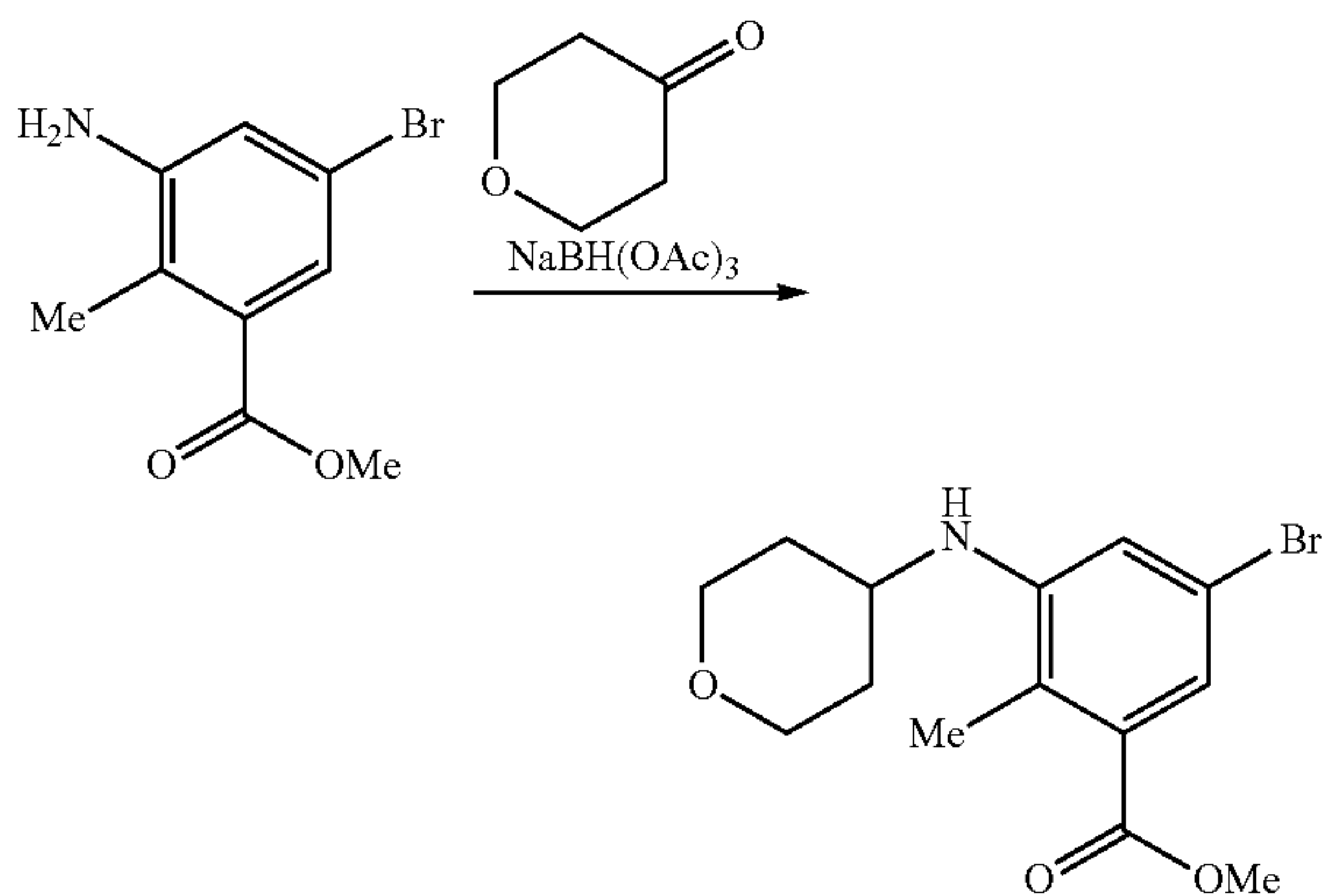
Methyl 5-bromo-3-(ethyl(tetrahydro-2H-pyran-4-yl)amino)-2-methylbenzoate (3)
