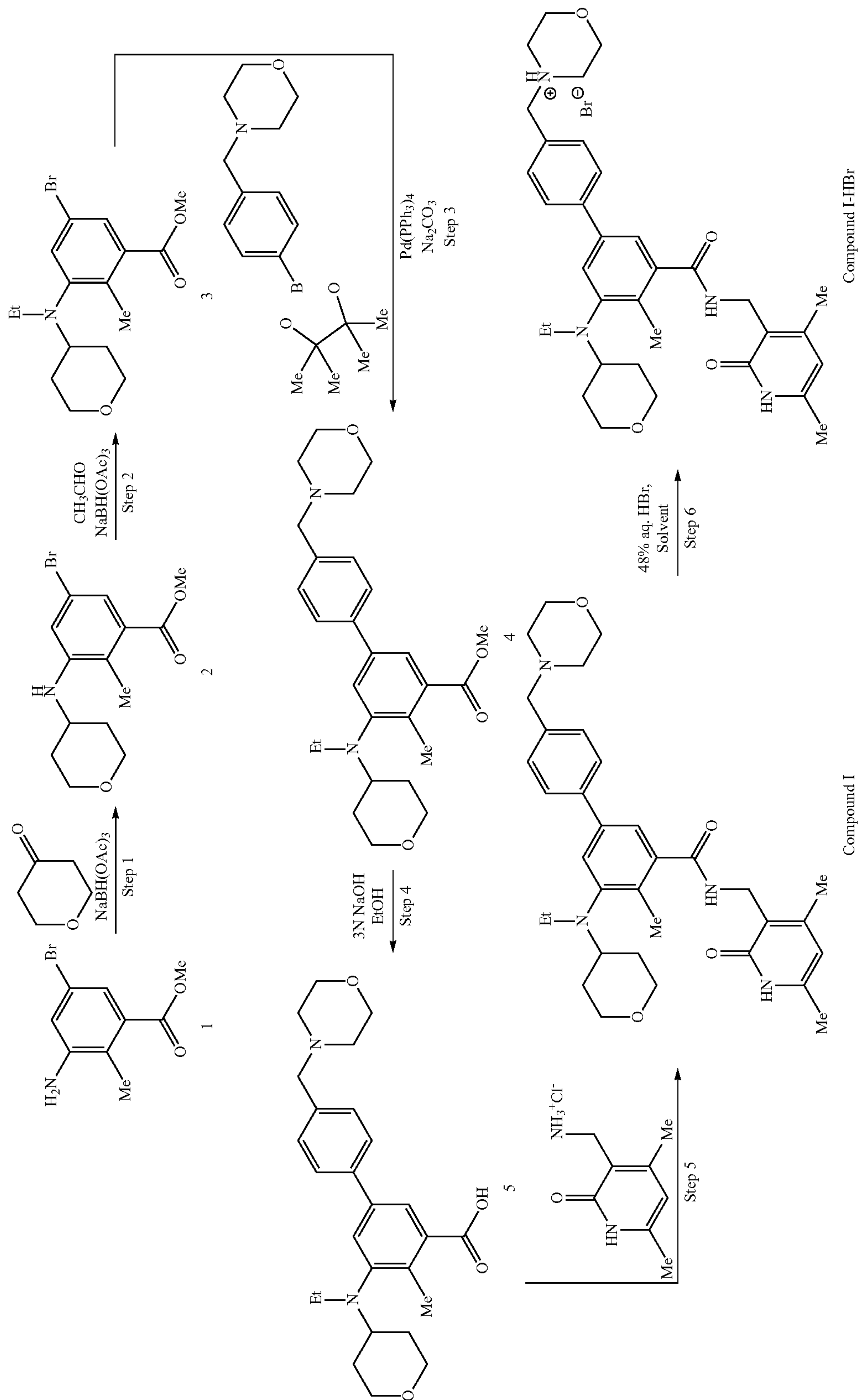
Scheme 1
